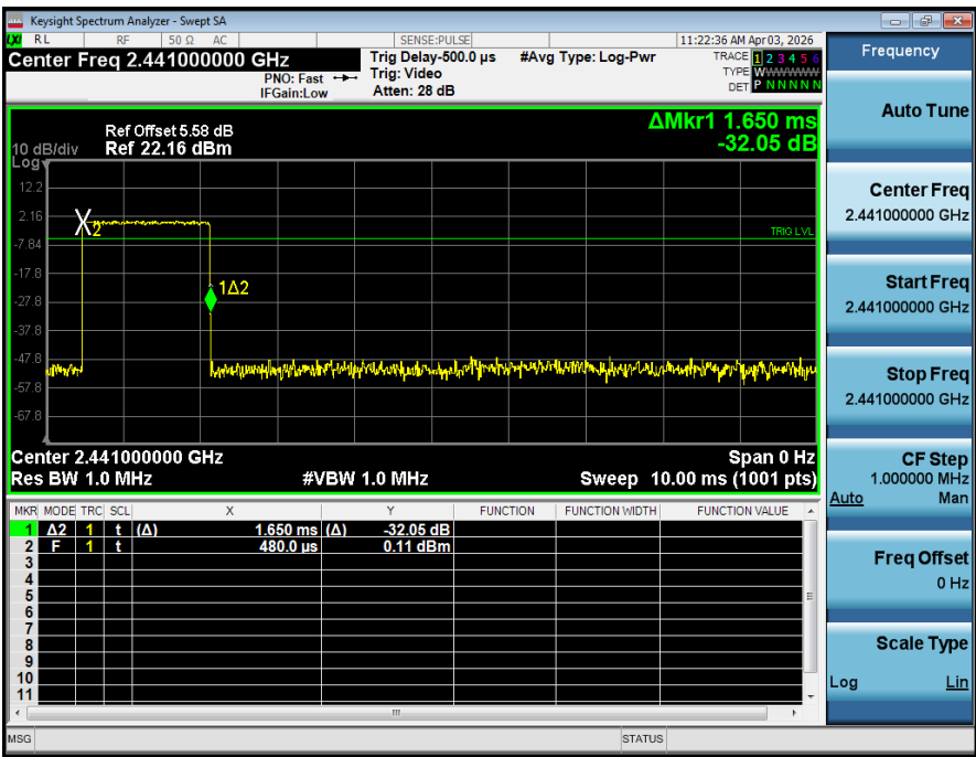
Dwell_Time_(Hopping)_NVNT_ANT1_2-DH3_2441_00_Accumulated
