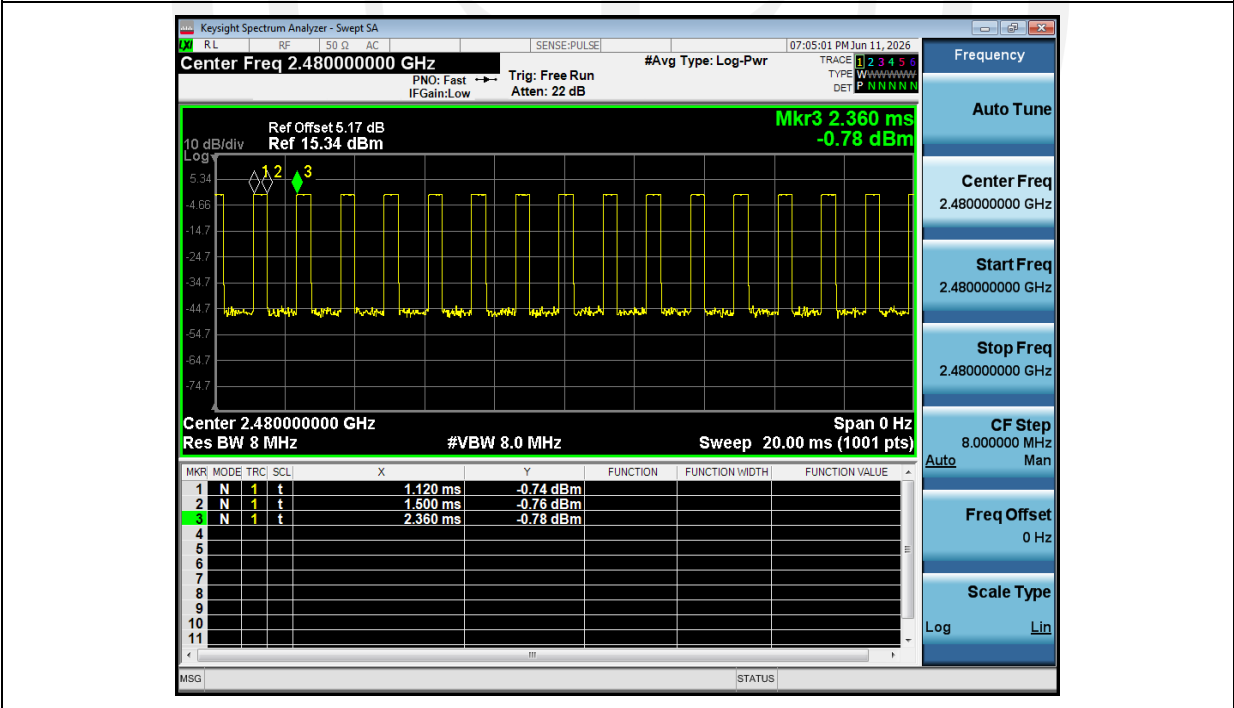
Duty_Cycle_NVNT_ANT1_1-DH1_2480
