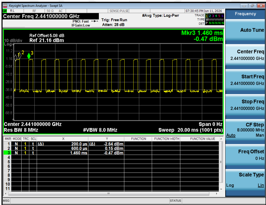
Duty_Cycle_NVNT_ANT1_2-DH1_2441
