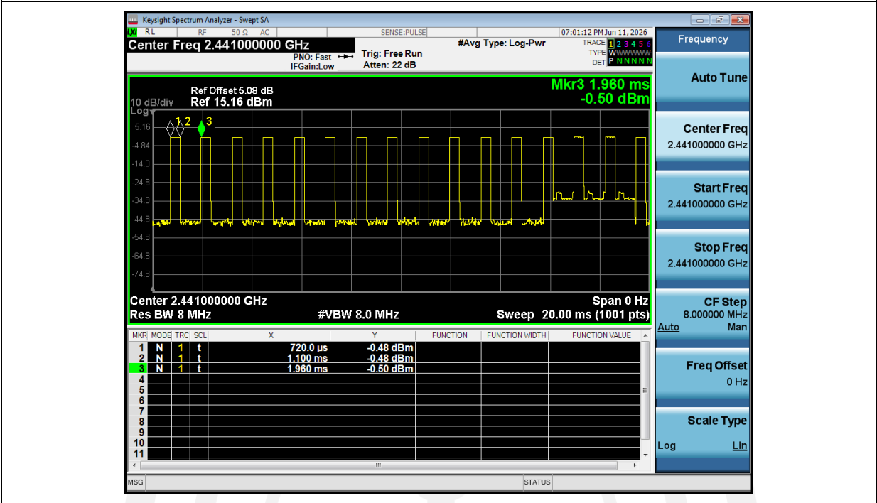
Duty_Cycle_NVNT_ANT1_1-DH1_2441
