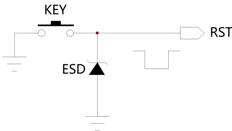
Figure 9 : Push button reset reference circuit
