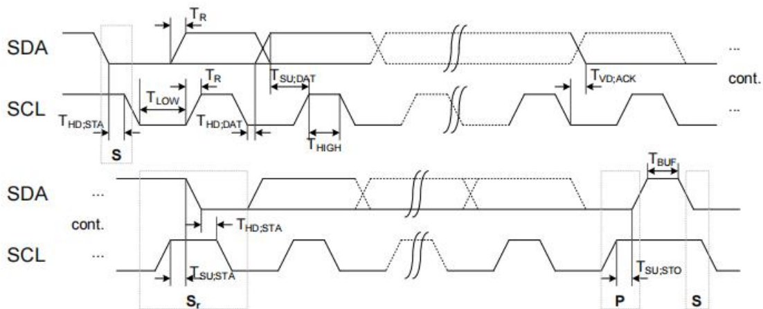
Figure 11 : I2C slave timing diagram
