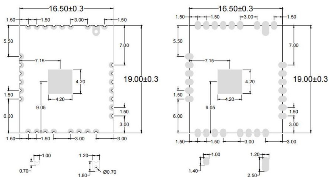
Figure 22 : Recommended package dimensions, top and bottom views
