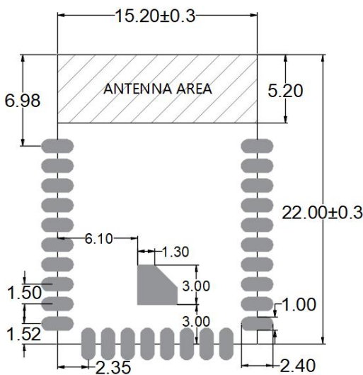
Figure 19 : Recommended package dimensions
