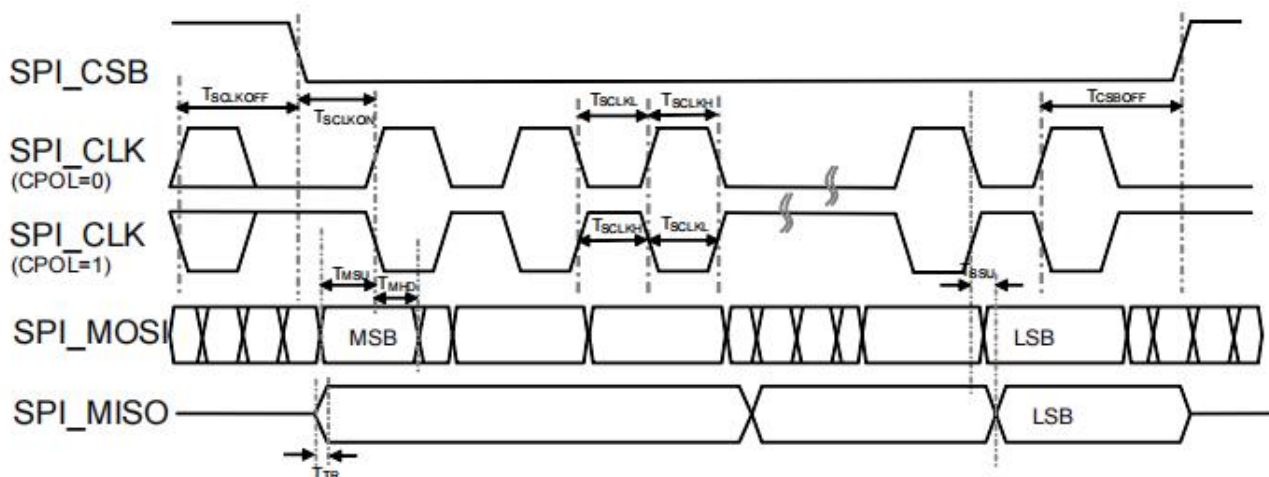
Figure 15 : SPI slave timing diagram
