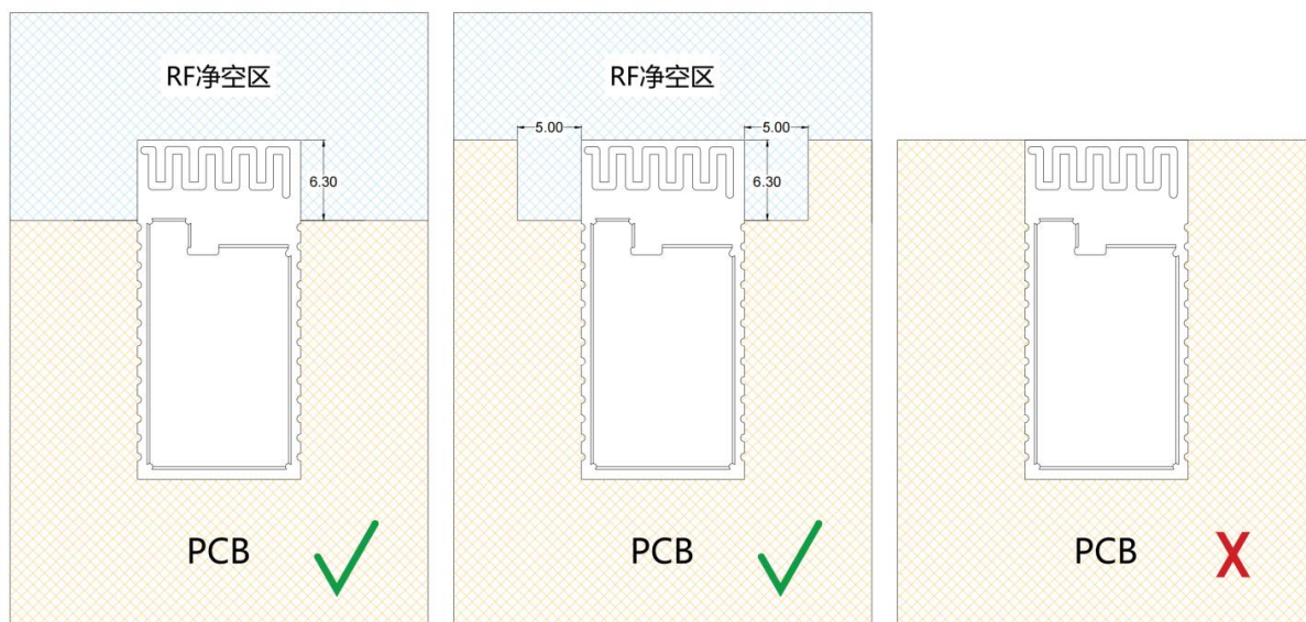
Figure 21 : Module placement reference position
