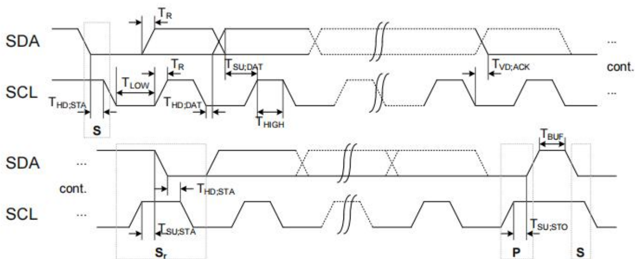
Figure 10 : I2C slave timing diagram
