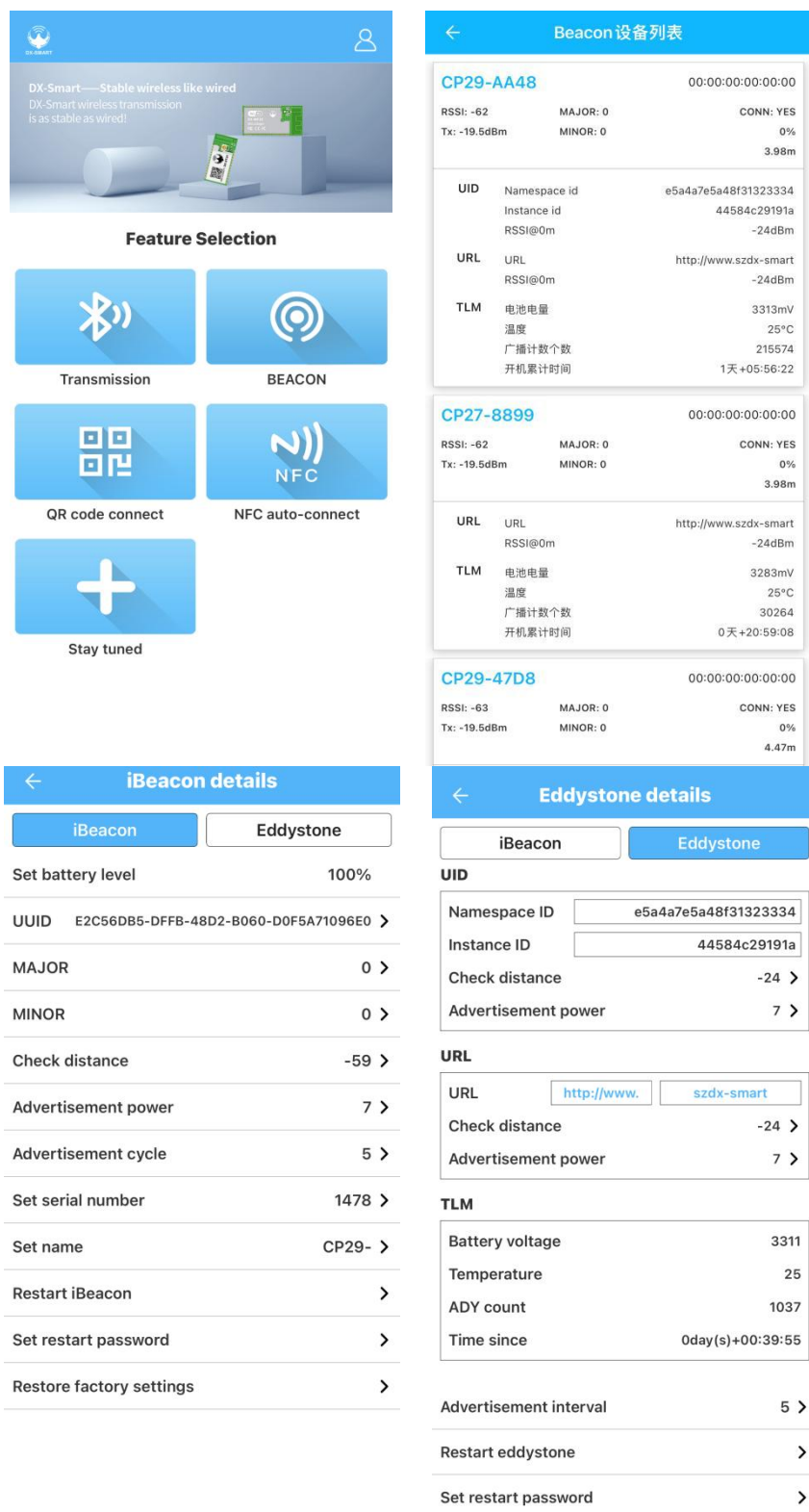
Figure 3: IOS APP interface
