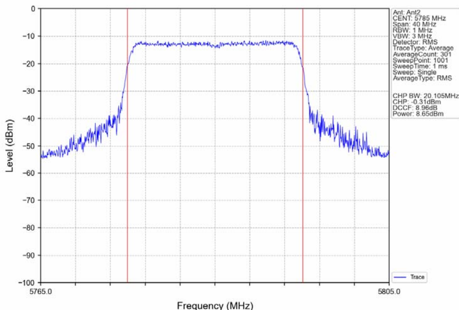
802.11ax(HEW20)_MCH_5785MHz_RU242_Left_Ant2_NTNV
