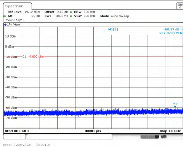
DH5_Ant1_2441_30~1000
