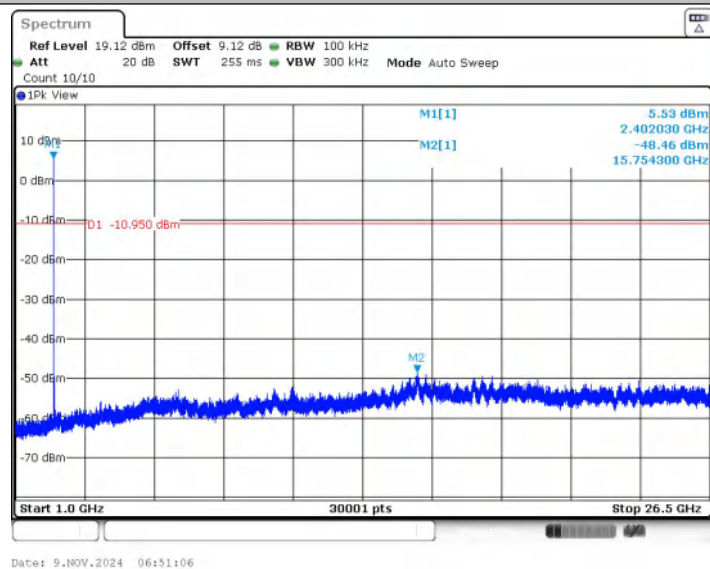
3DH5_Ant1_2402_1000~26500
