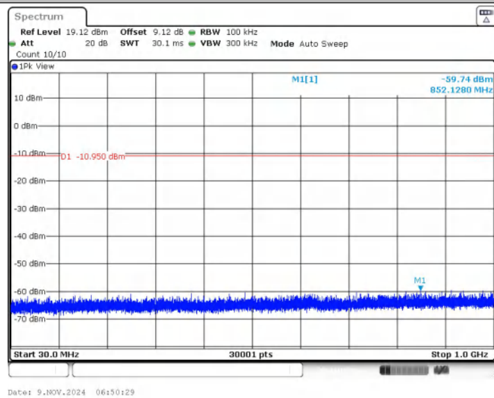
3DH5_Ant1_2402_30~1000
