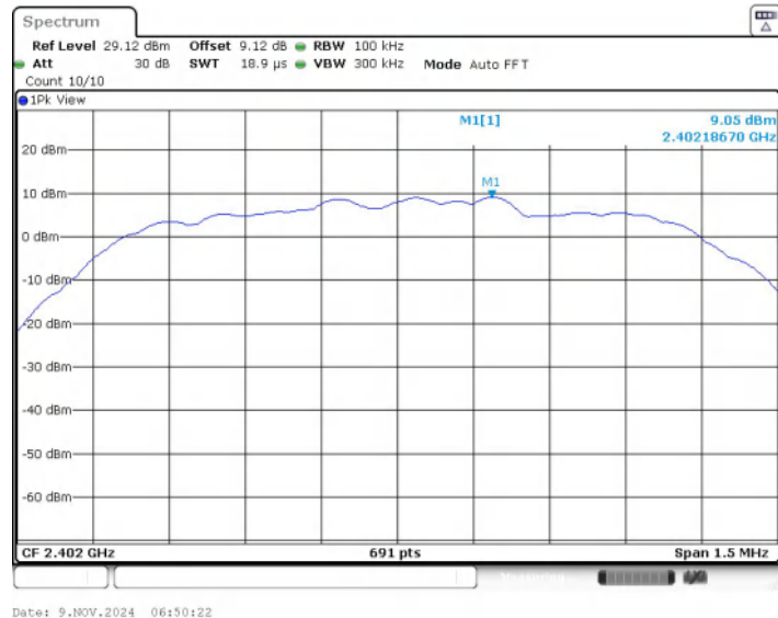
3DH5_Ant1_2402_0~Reference
