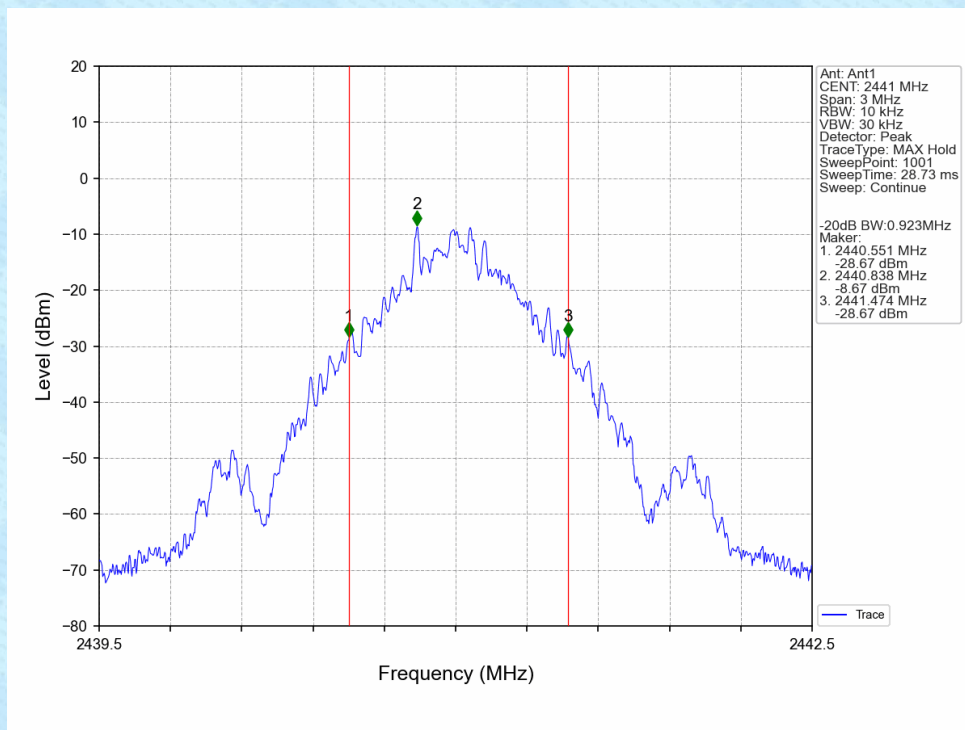
GFSK_DH5_MCH_2441MHz_Ant1_NTNV
