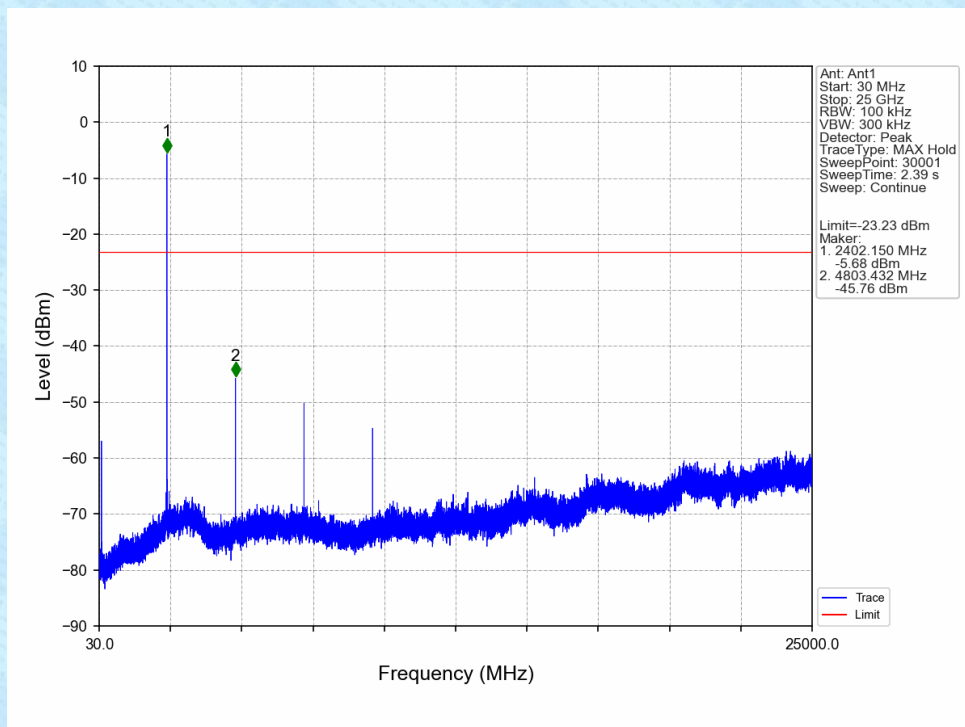
GFSK_DH5_LCH_2402MHz_Ant1_NTNV
