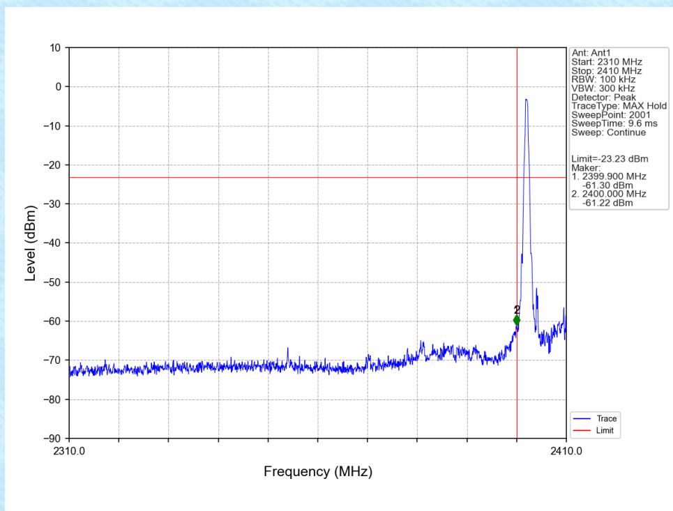
GFSK_DH5_LCH_2402MHz_Ant1_NTNV
