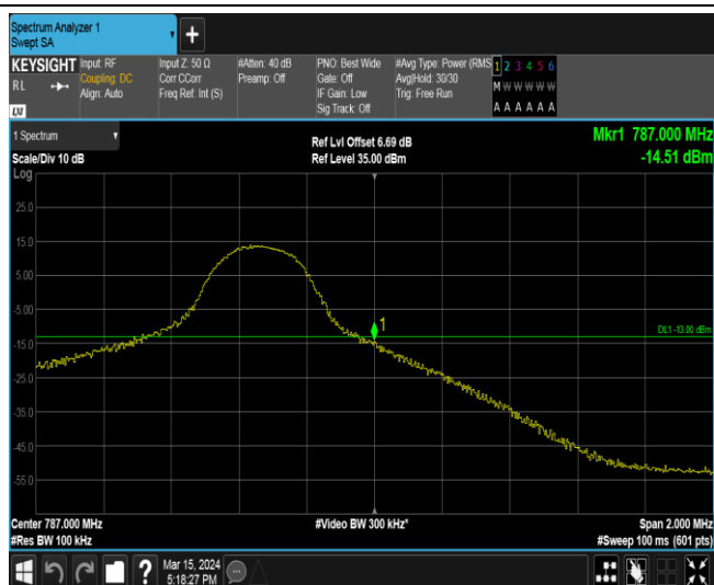
Band13-5MHz-16QAM-23255-25RB#0
