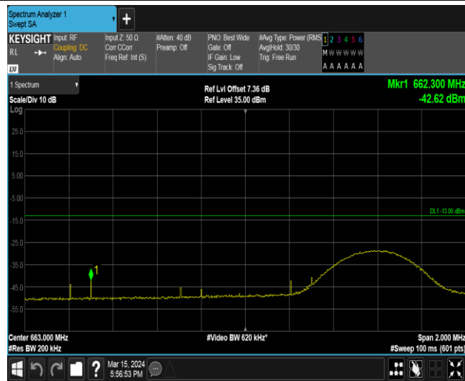
Band71-10MHz-16QAM-133172-50RB#0
