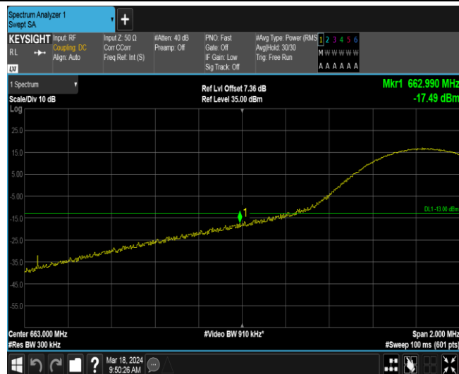
Band71-15MHz-16QAM-133197-1RB#74
