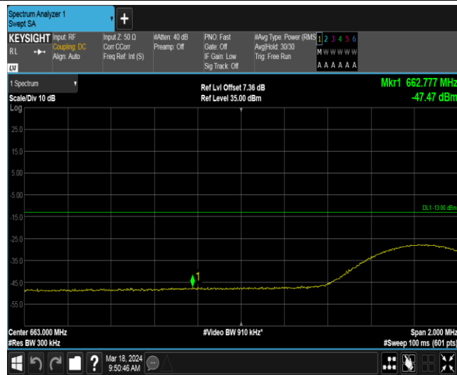
Band71-15MHz-16QAM-133197-75RB#0
