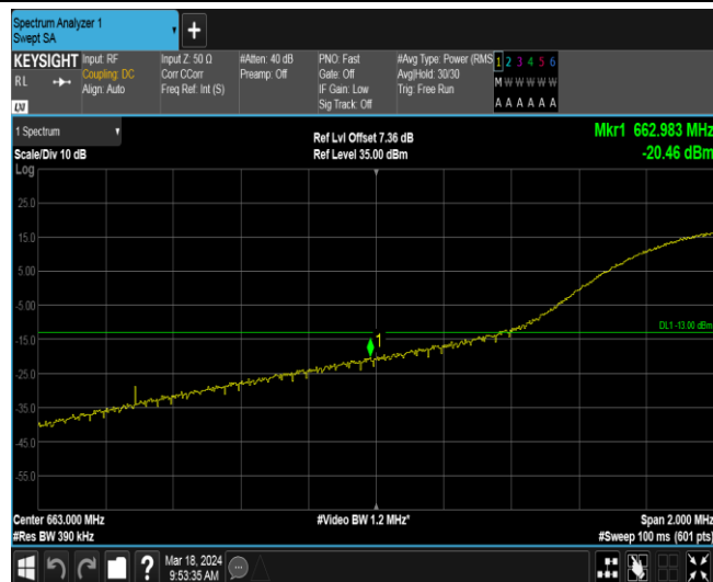
Band71-20MHz-16QAM-133222-1RB#99
