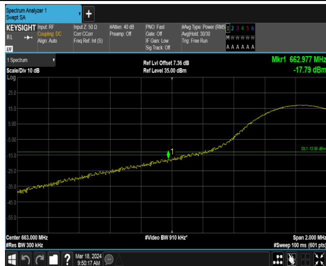
Band71-15MHz-QPSK-133197-1RB#74
