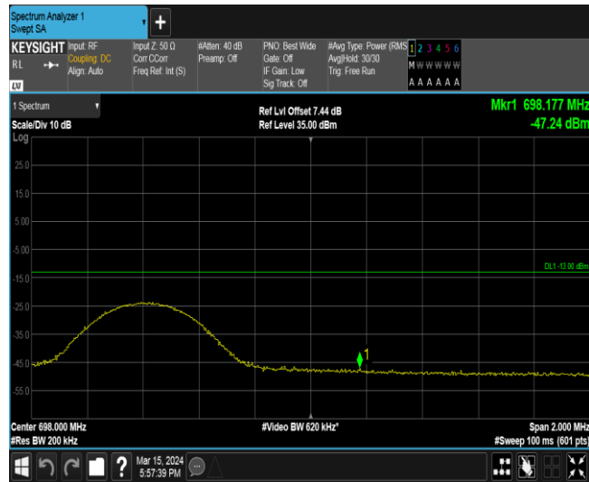
Band71-10MHz-16QAM-133422-1RB#49
