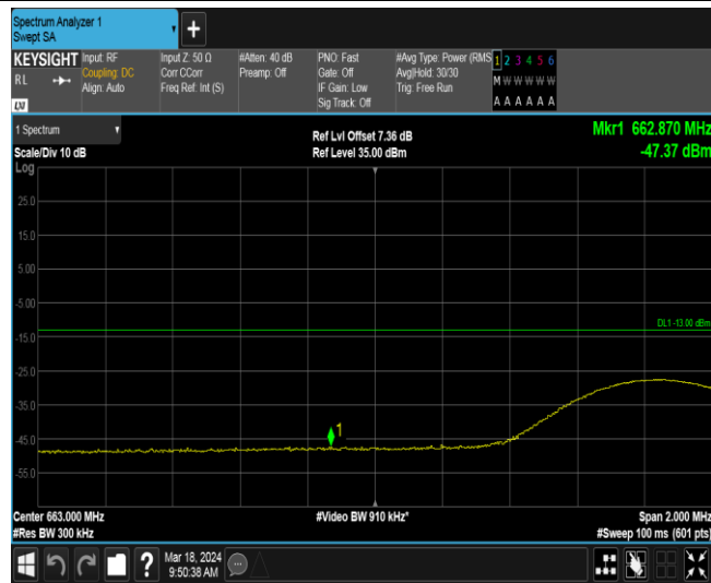
Band71-15MHz-QPSK-133197-75RB#0
