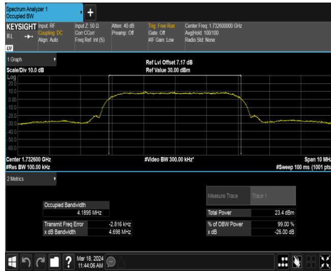
Band4-1413-2
