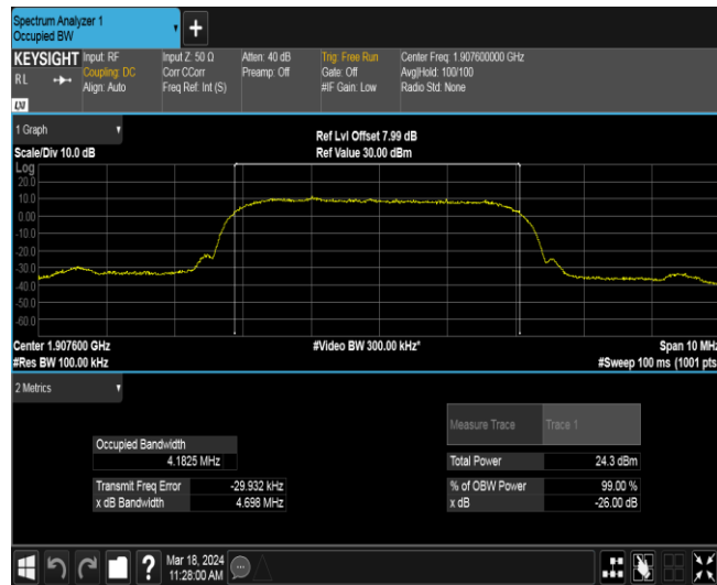
Band2-9538-3
