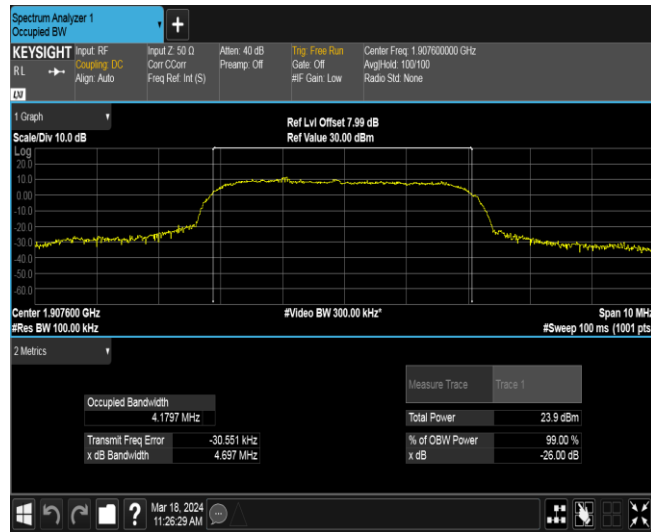
Band2-9538-2
