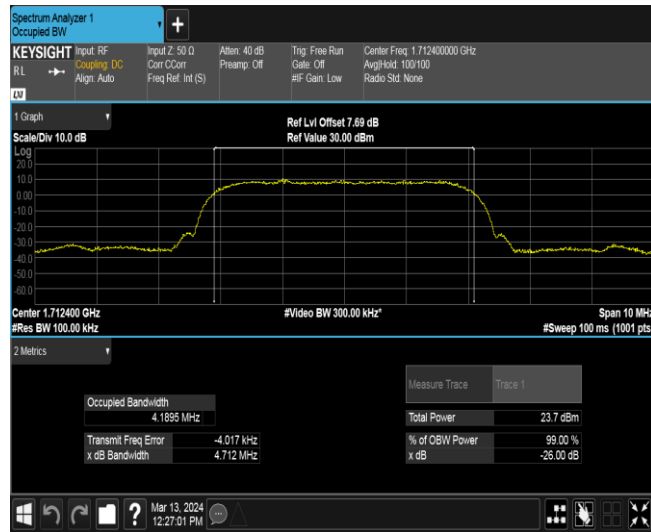
Band4-1312-2
