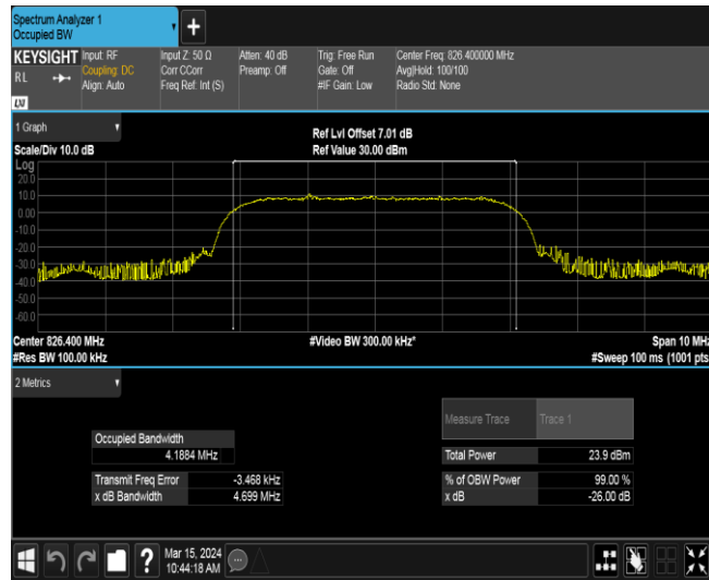
Band5-4132-4
