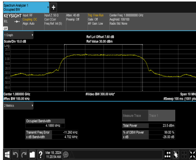
Band2-9400-4
