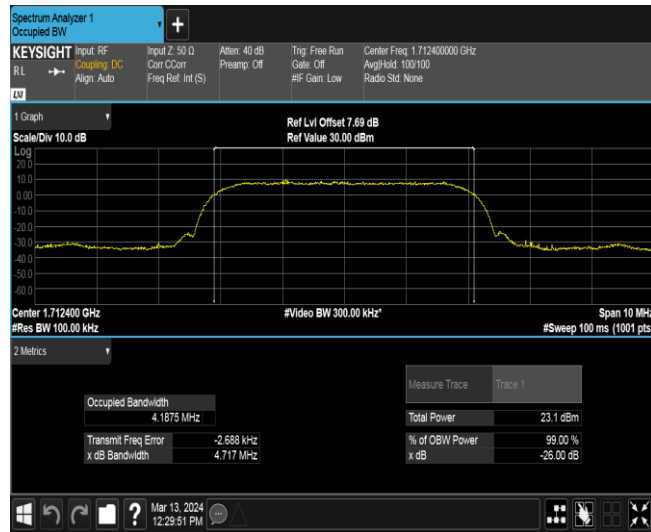
Band4-1312-4
