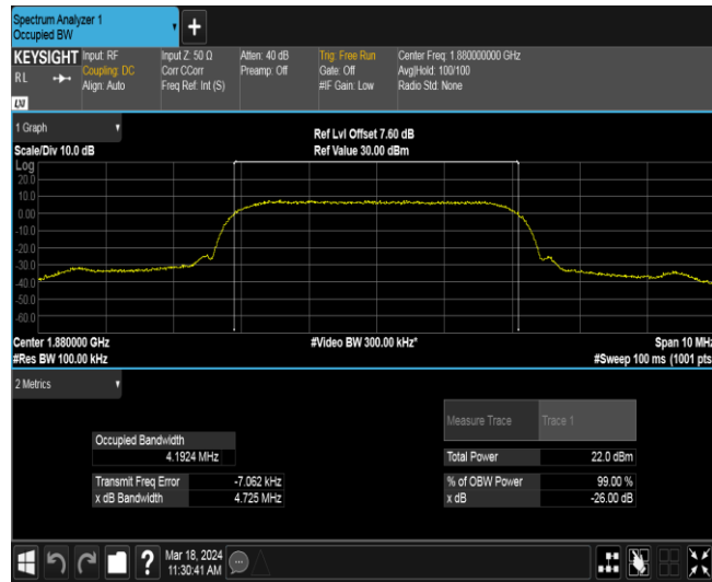
Band2-9400-5
