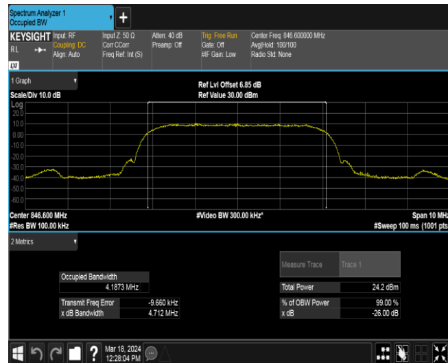
Band5-4233-3
