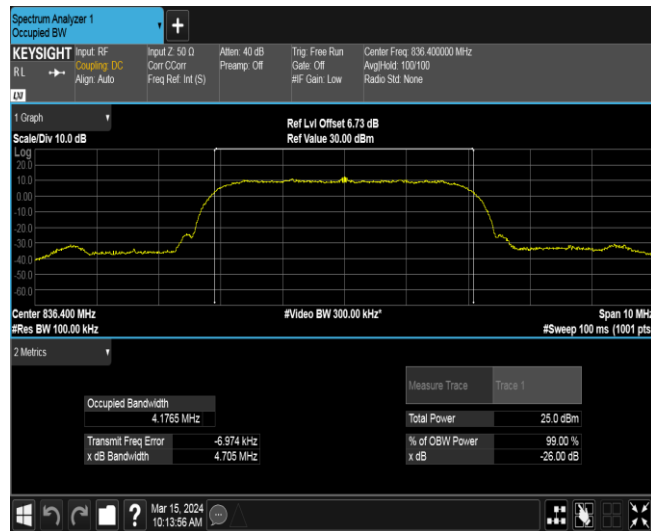
Band5-4233
