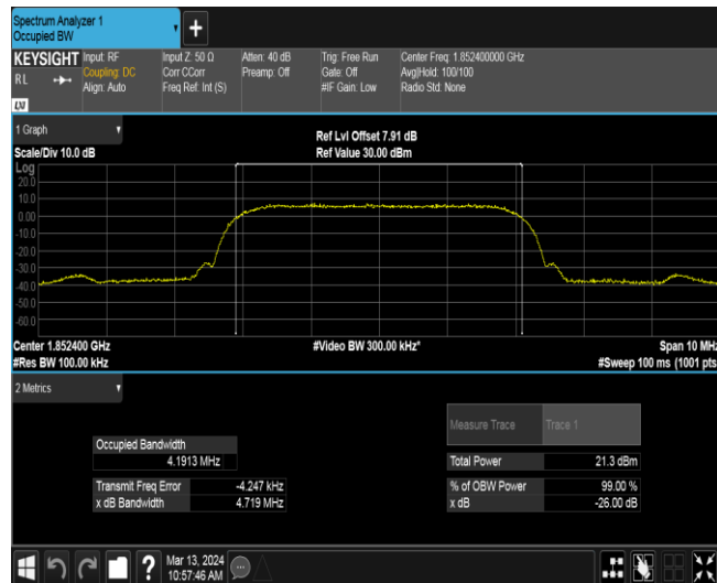
Band2-9262-5
