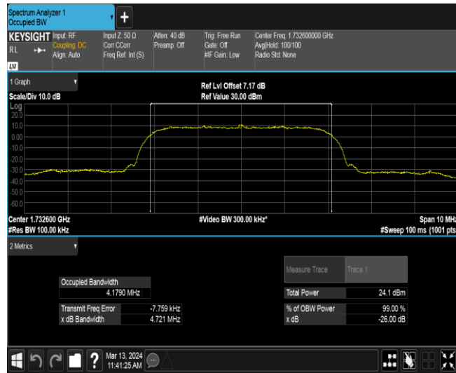
Band4-1513
