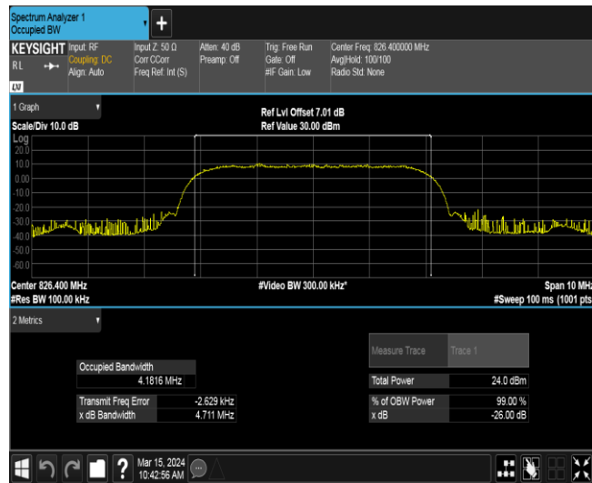
Band5-4132-3
