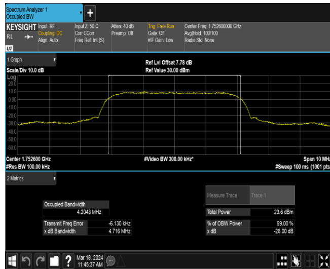
Band4-1513-3
