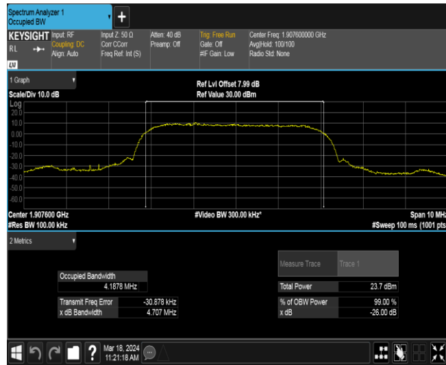
Band2-9538-4
