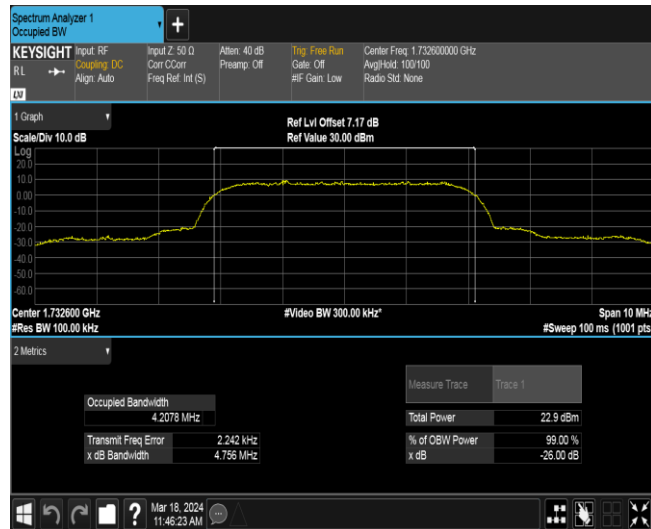
Band4-1413-4
