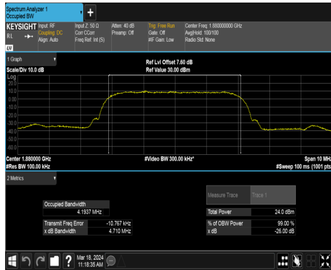
Band2-9400-2
