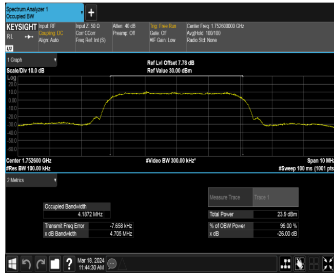
Band4-1513-2
