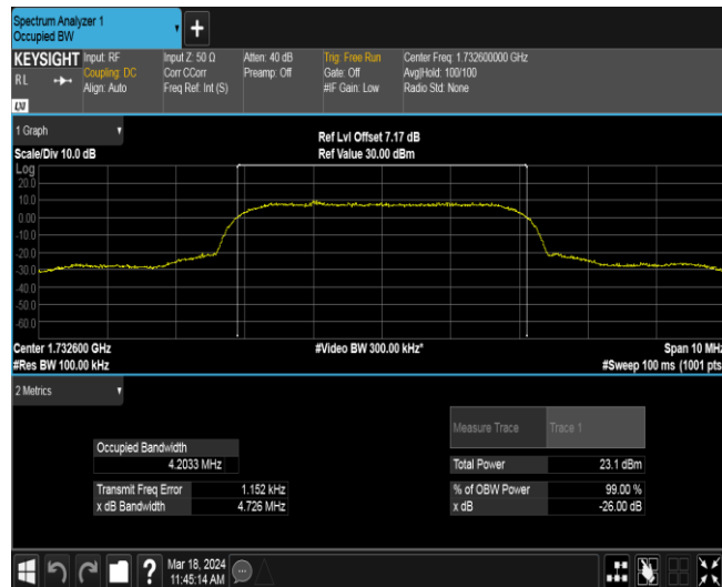
Band4-1413-3
