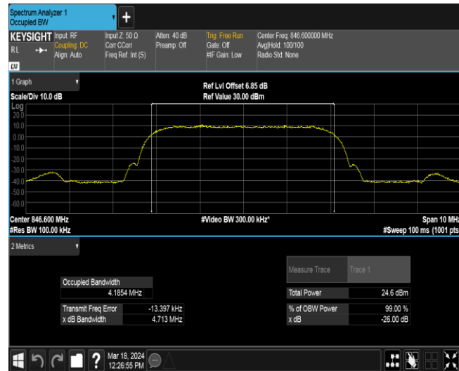
Band5-4233-2
