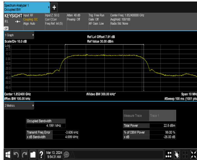
Band2-9262-4
