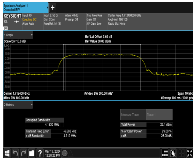
Band4-1312-3
