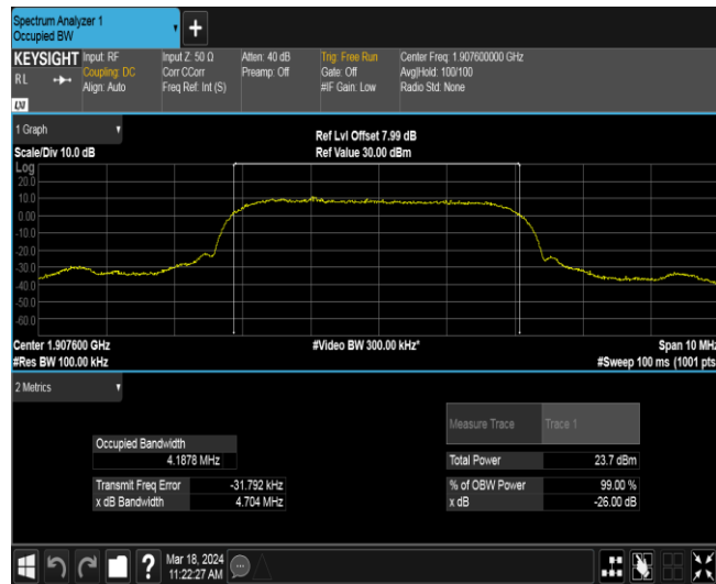
Band4-1312-1
