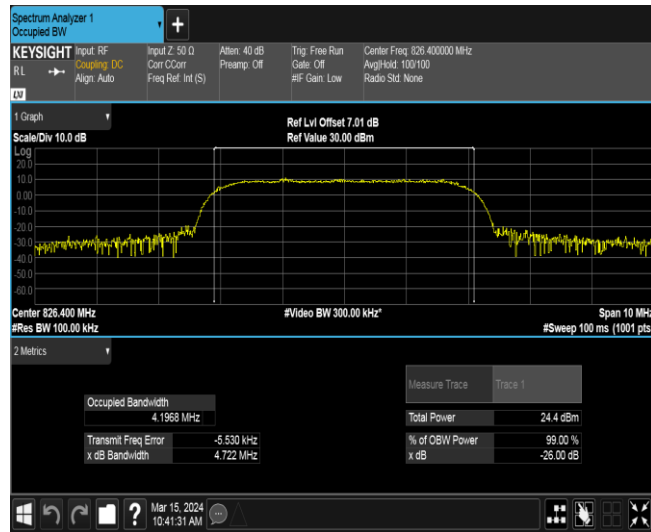
Band5-4132-2
