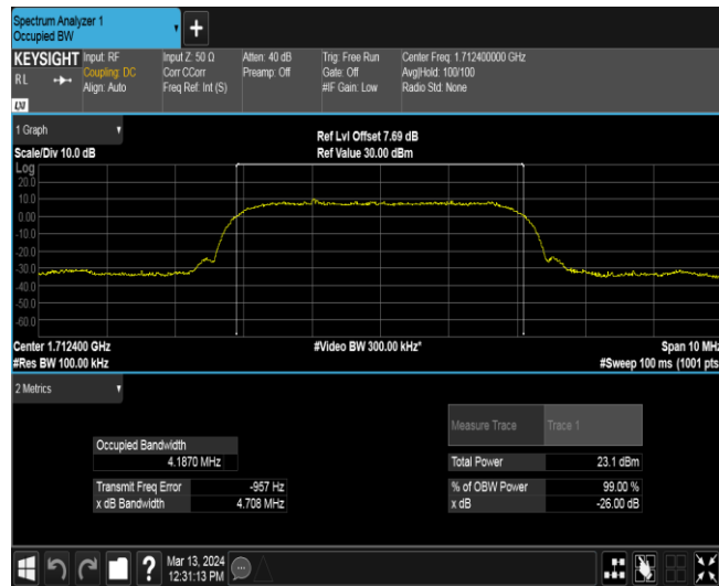
Band4-1413-1
