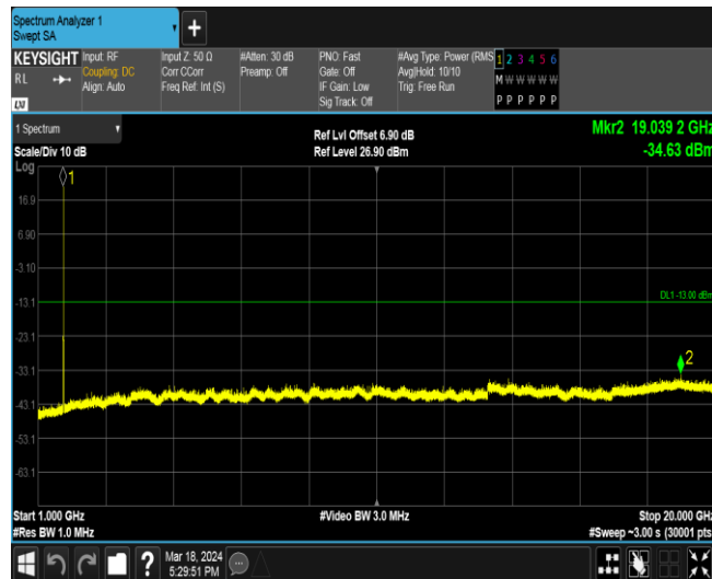
Band4-1312-2-0.15~30MHz
