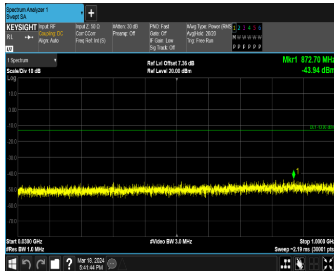
Band4-1413-1-30~1000MHz
