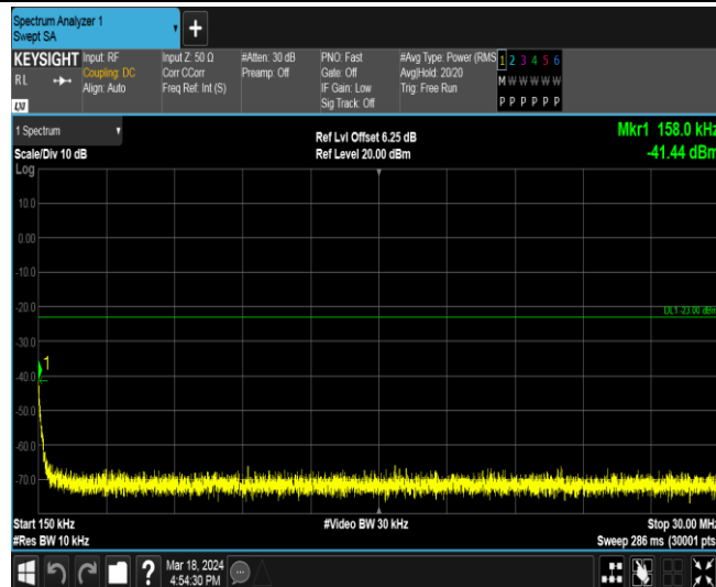
Band2-9400-4-0.15~30MHz
