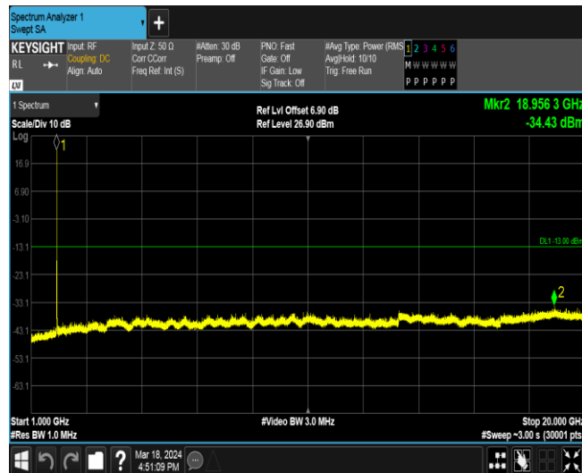
Band2-9400-3-1000~20000MHz
