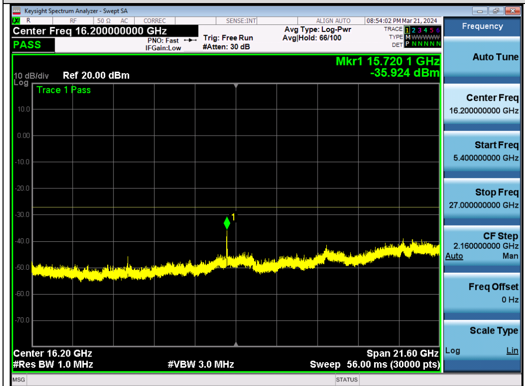
Test_Graph_802.11a_ANT1_5240_6Mbps_Frequency Band 4
