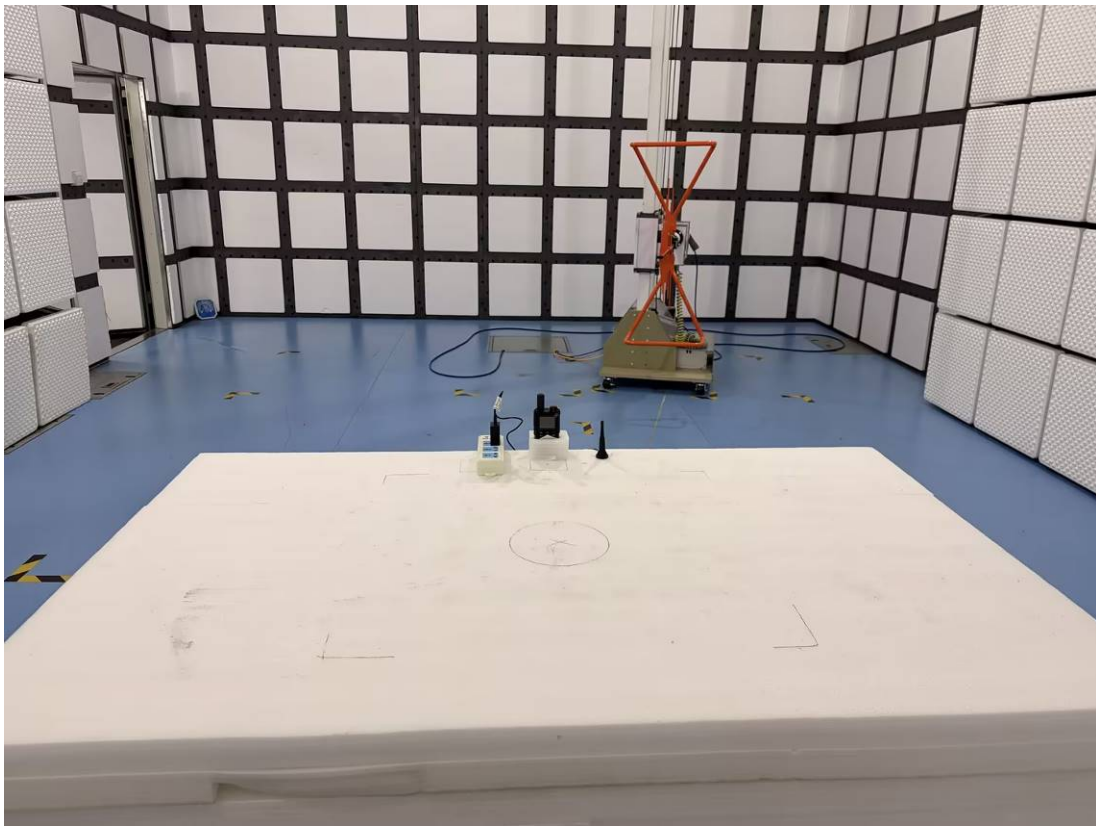
Radiation Emission - Back View (Below 1GHz)
