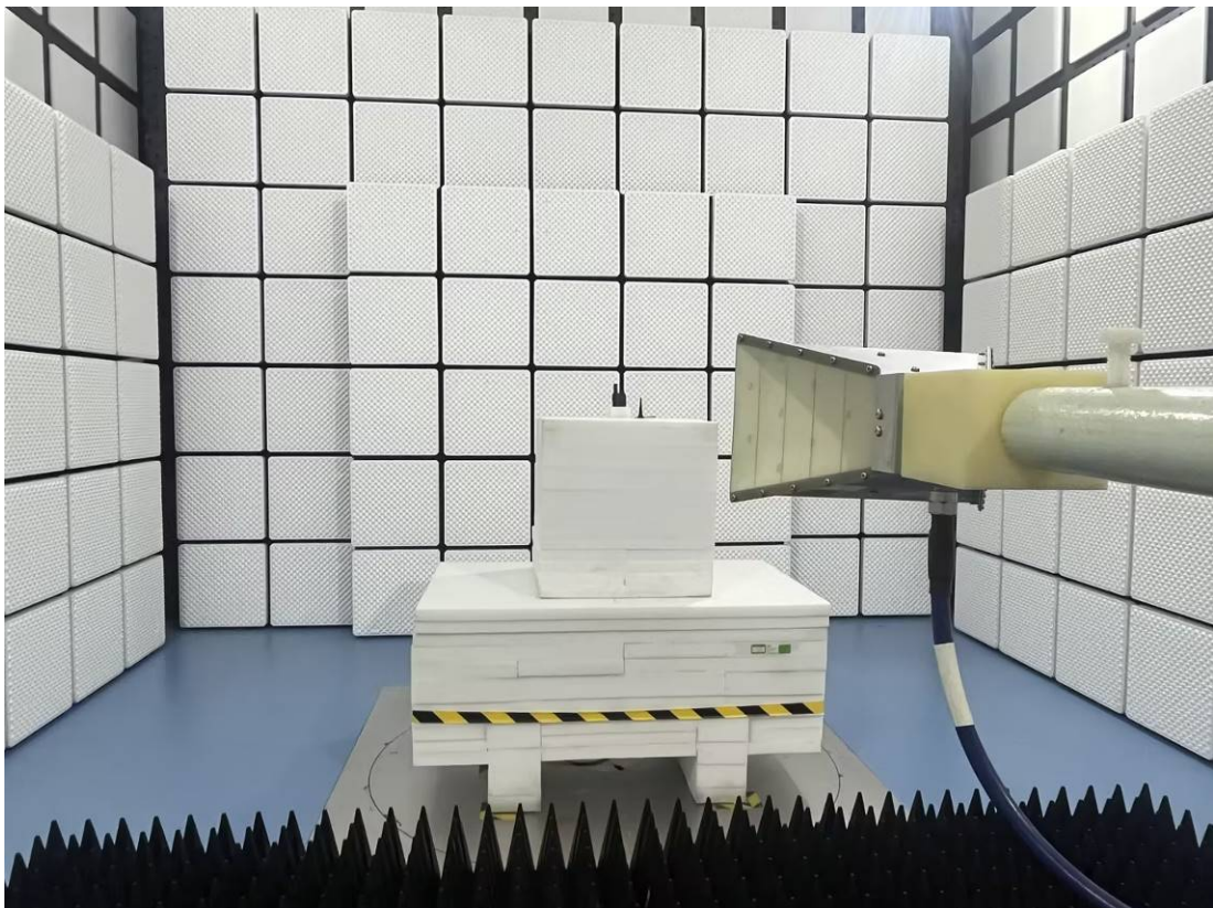
Radiation Emission - Back View (1GHz-18GHz)
