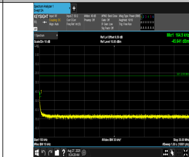
EGPRS850-251-8-0.15~30MHz-PASS
