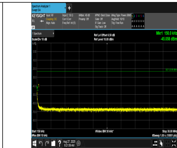
EGPRS850-128-8-0.15~30MHz-PASS
