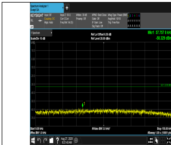
EGPRS850-128-8-0.009~0.15MHz-PASS
