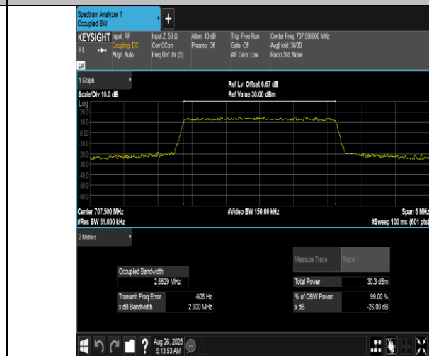
Band12-3MHz-16QAM-23095-15RB#0-PASS
