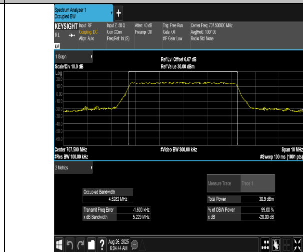
Band12-5MHz-16QAM-23095-25RB#0-PASS
