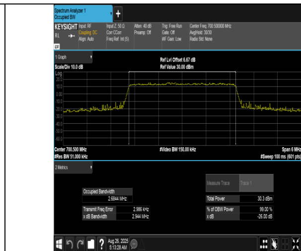
Band12-3MHz-16QAM-23025-15RB#0-PASS
