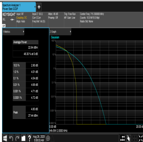
Band12-1.4MHz-16QAM-23173-1RB#0-PASS
