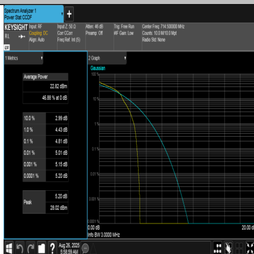
Band12-3MHz-16QAM-23165-1RB#0-PASS
