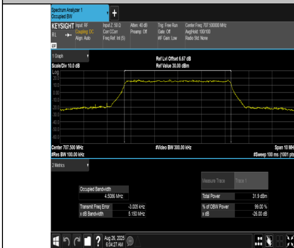
Band12-5MHz-QPSK-23095-25RB#0-PASS
