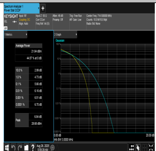
Band12-3MHz-16QAM-23165-15RB#0-PASS
