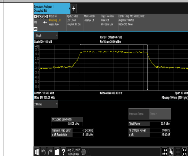
Band12-5MHz-16QAM-23155-25RB#0-PASS
