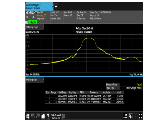
Band12-1.4MHz-16QAM-23017-1RB#0-PASS
