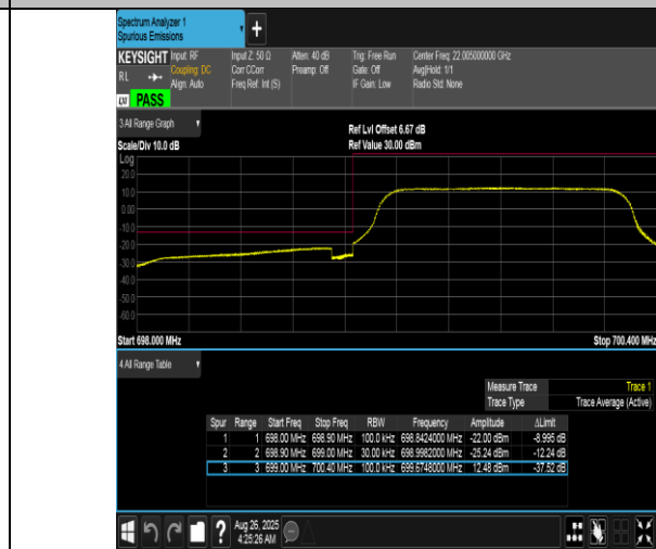
Band12-1.4MHz-16QAM-23017-6RB#0-PASS
