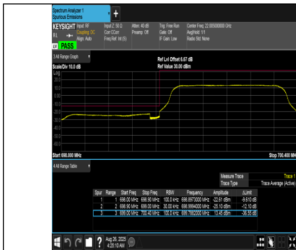
Band12-1.4MHz-QPSK-23017-6RB#0-PASS
