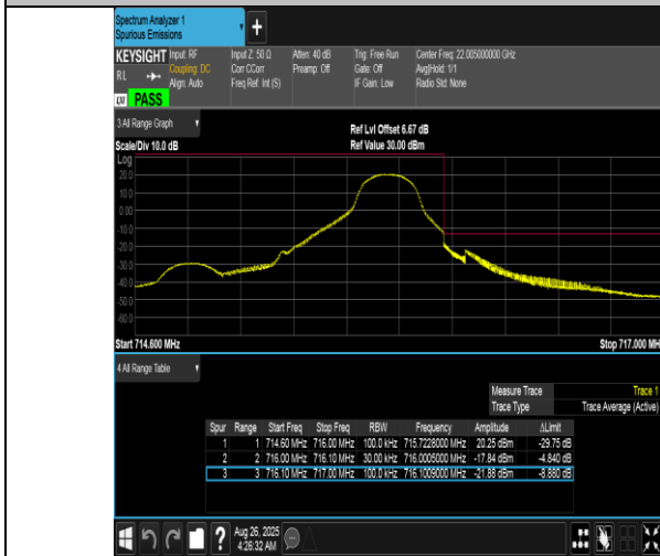
Band12-1.4MHz-16QAM-23173-1RB#5-PASS
