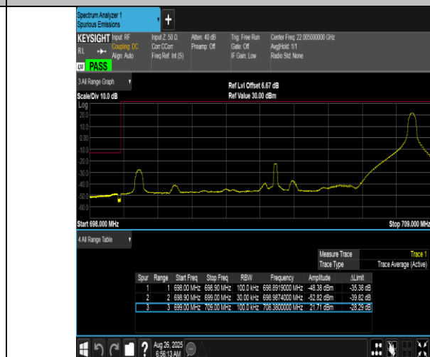
Band12-10MHz-QPSK-23060-1RB#49-PASS
