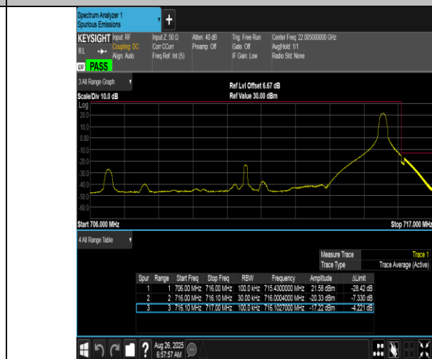
Band12-10MHz-QPSK-23130-1RB#49-PASS
