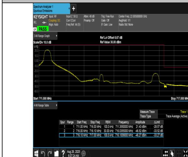
Band12-5MHz-QPSK-23155-1RB#0-PASS
