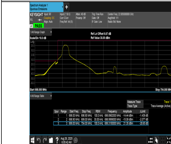
Band12-5MHz-QPSK-23035-1RB#0-PASS
