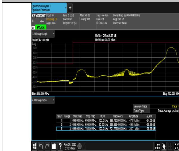
Band12-3MHz-16QAM-23025-1RB#14-PASS
