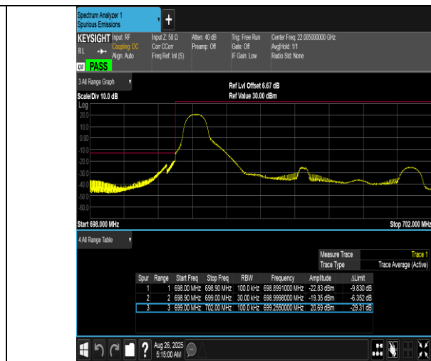
Band12-3MHz-16QAM-23025-1RB#0-PASS
