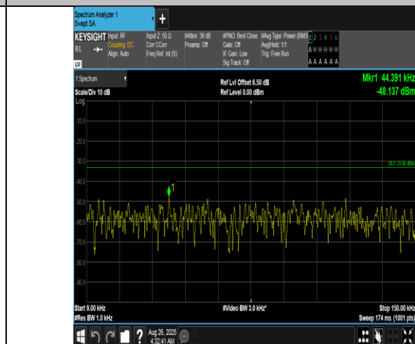
Band12-1.4MHz-16QAM-23017-6RB#0-0.009~0.15-PASS
