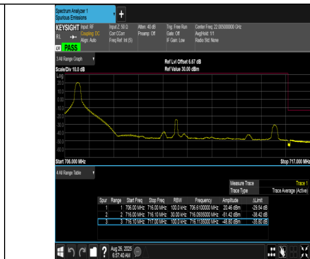
Band12-10MHz-16QAM-23130-1RB#0-PASS
