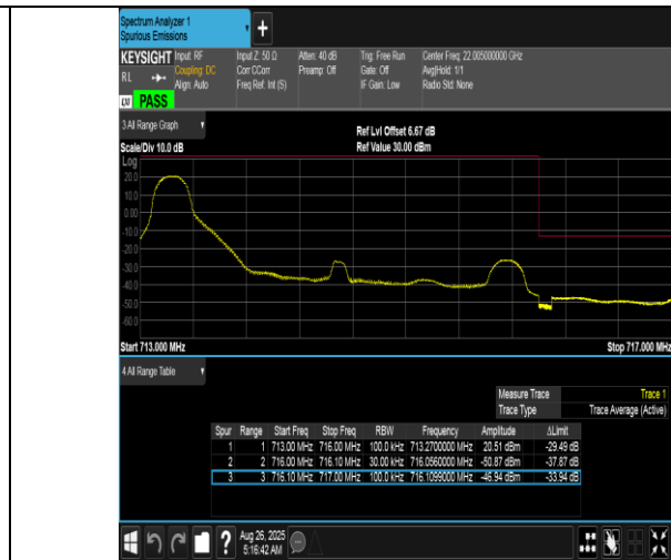
Band12-3MHz-16QAM-23165-1RB#0-PASS
