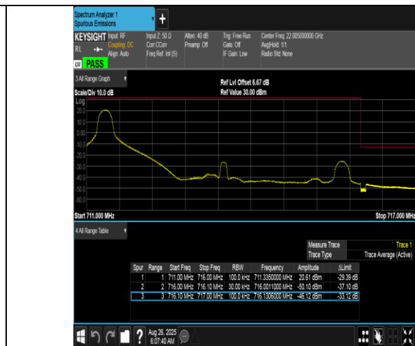
Band12-5MHz-16QAM-23155-1RB#0-PASS
