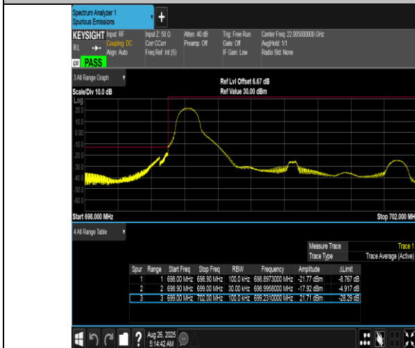
Band12-3MHz-QPSK-23025-1RB#0-PASS
