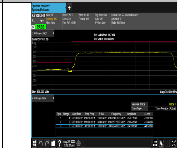
Band12-3MHz-16QAM-23025-15RB#0-PASS
