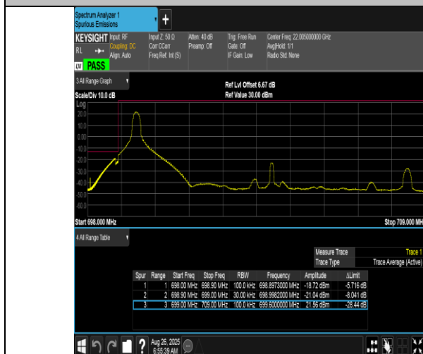
Band12-10MHz-QPSK-23060-1RB#0-PASS
