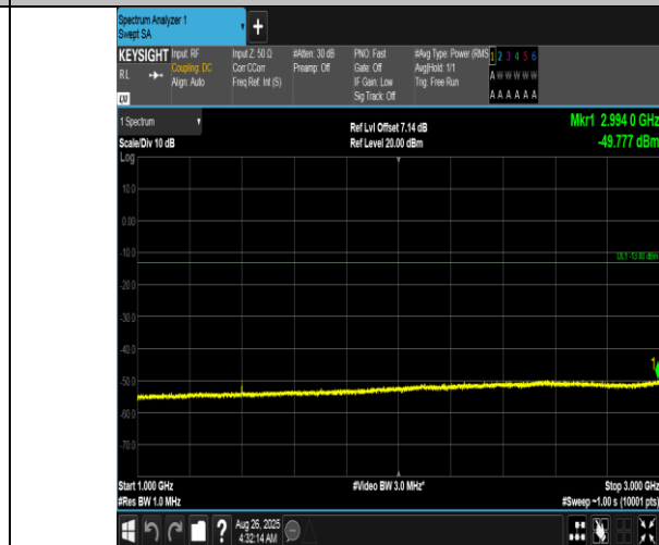
Band12-1.4MHz-QPSK-23017-6RB#0-1000~3000-PASS
