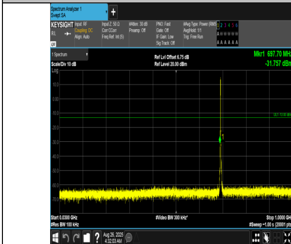
Band12-1.4MHz-QPSK-23017-6RB#0-30~1000-PASS
