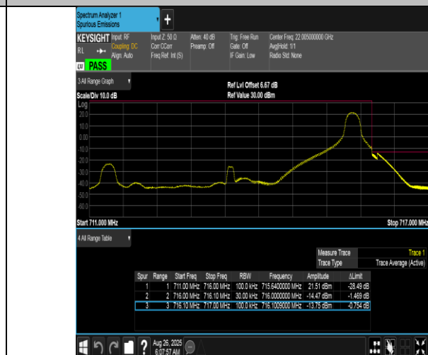
Band12-5MHz-QPSK-23155-1RB#24-PASS
