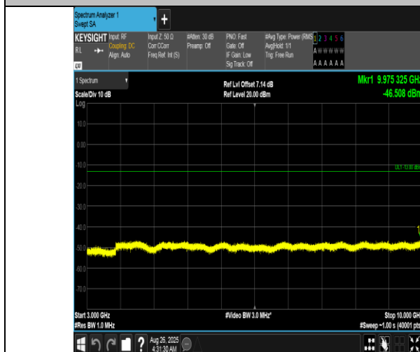
Band12-1.4MHz-16QAM-23017-1RB#5-3000~10000-PASS
