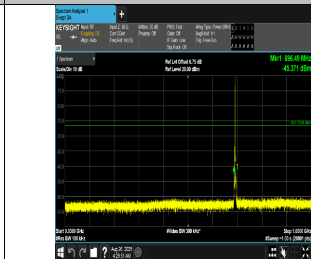
Band12-1.4MHz-QPSK-23017-1RB#5-30~1000-PASS
