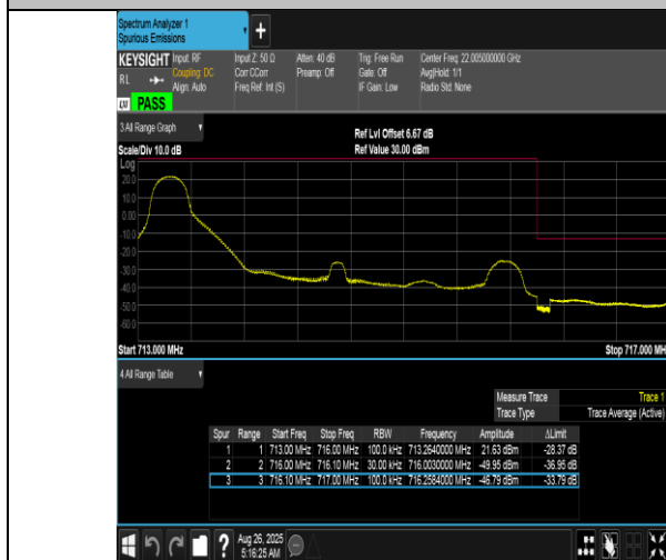
Band12-3MHz-QPSK-23165-1RB#0-PASS
