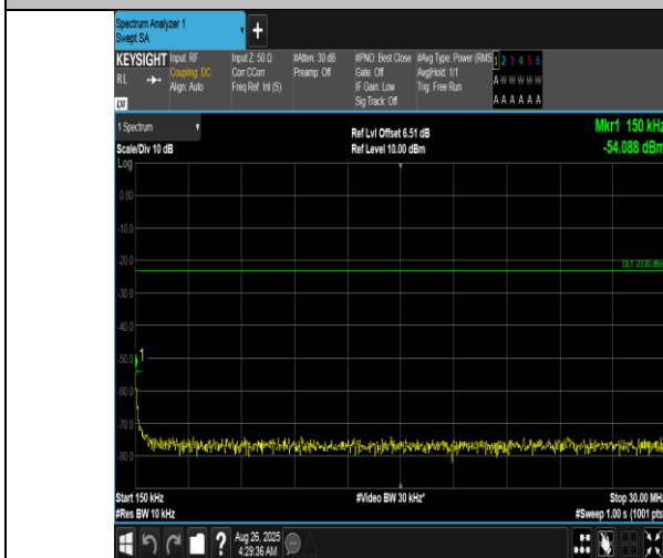
Band12-1.4MHz-QPSK-23017-1RB#5-0.15~30-PASS
