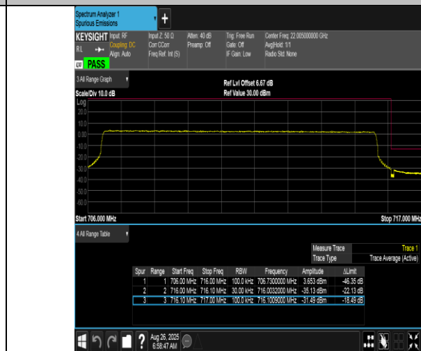
Band12-10MHz-16QAM-23130-50RB#0-PASS
