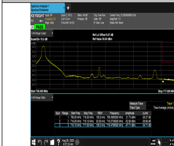
Band12-10MHz-QPSK-23130-1RB#0-PASS
