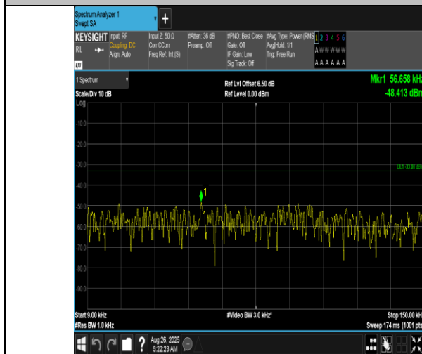
Band12-3MHz-QPSK-23025-15RB#0-0.009~0.15-PASS
