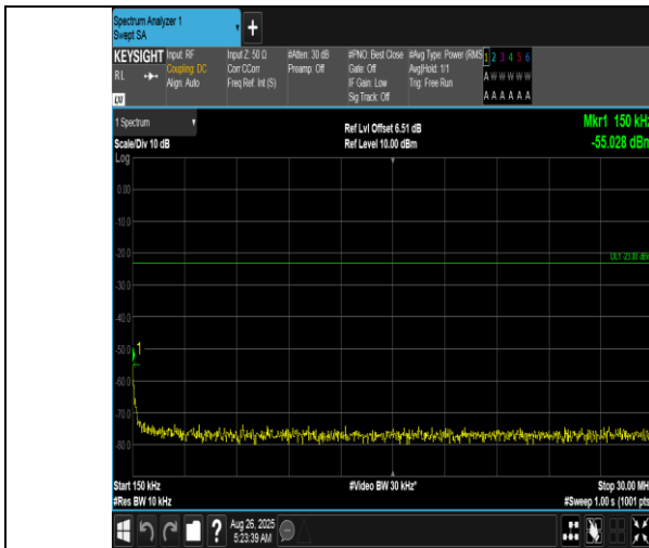
Band12-3MHz-16QAM-23025-15RB#0-0.15~30-PASS
