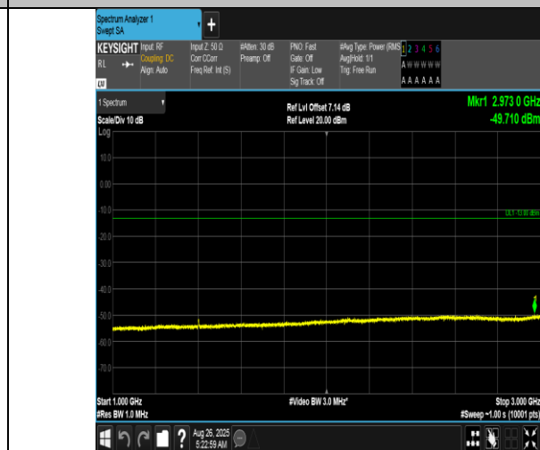
Band12-3MHz-QPSK-23025-15RB#0-1000~3000-PASS
