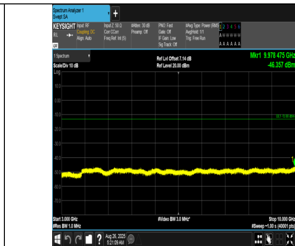
Band12-3MHz-QPSK-23025-1RB#14-3000~10000-PASS
