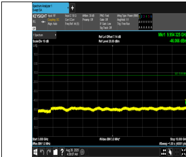
Band12-1.4MHz-QPSK-23095-6RB#0-3000~10000-PASS
