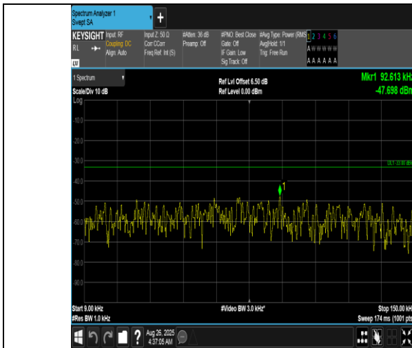
Band12-1.4MHz-16QAM-23095-1RB#5-0.009~0.15-PASS
