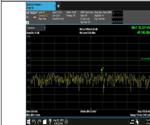
Band12-1.4MHz-QPSK-23173-1RB#0-0.009~0.15-PASS
