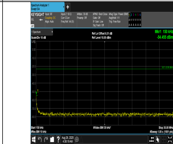
Band12-1.4MHz-QPSK-23095-6RB#0-0.15~30-PASS
