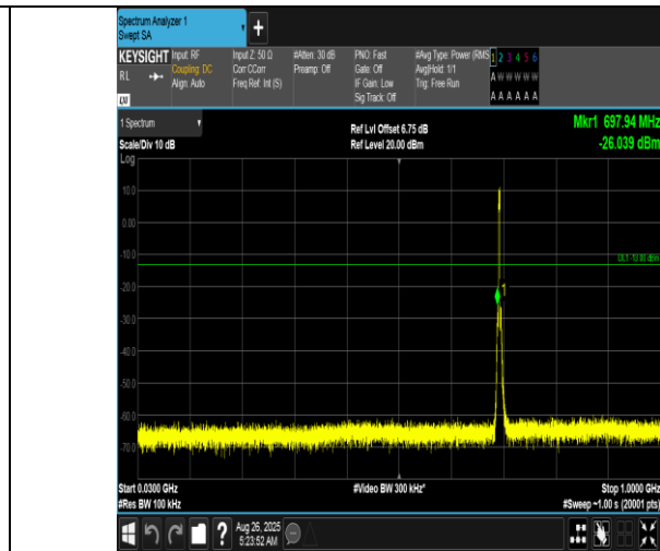
Band12-3MHz-16QAM-23025-15RB#0-30~1000-PASS
