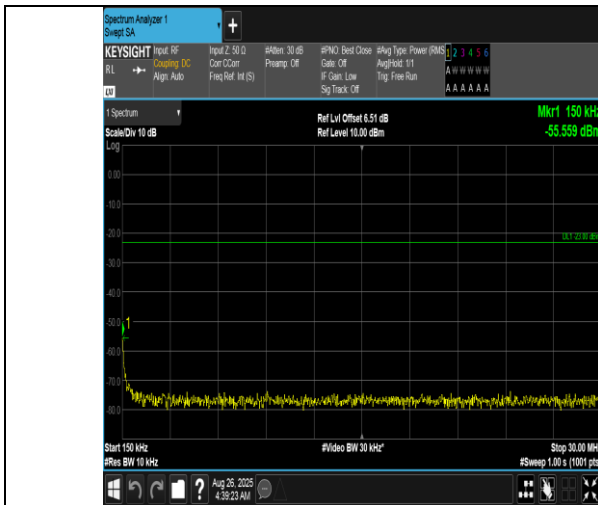
Band12-1.4MHz-16QAM-23095-6RB#0-0.15~30-PASS
