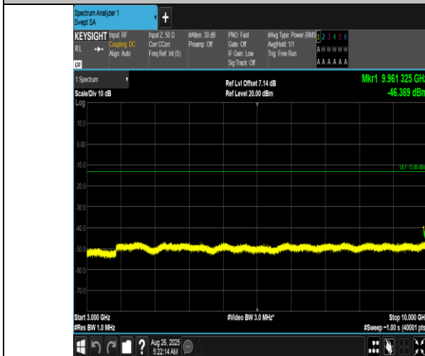
Band12-3MHz-16QAM-23025-1RB#14-3000~10000-PASS
