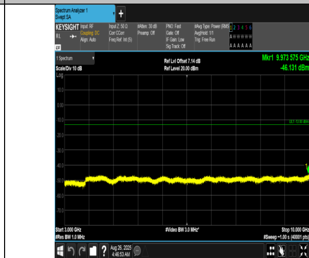
Band12-1.4MHz-16QAM-23173-6RB#0-3000~10000-PASS
