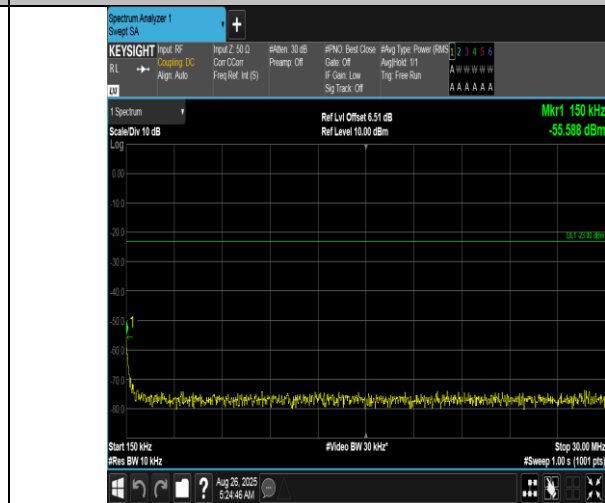
Band12-3MHz-QPSK-23095-1RB#0-0.15~30-PASS
