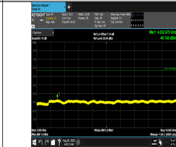
Band12-1.4MHz-16QAM-23095-6RB#0-3000~10000-PASS
