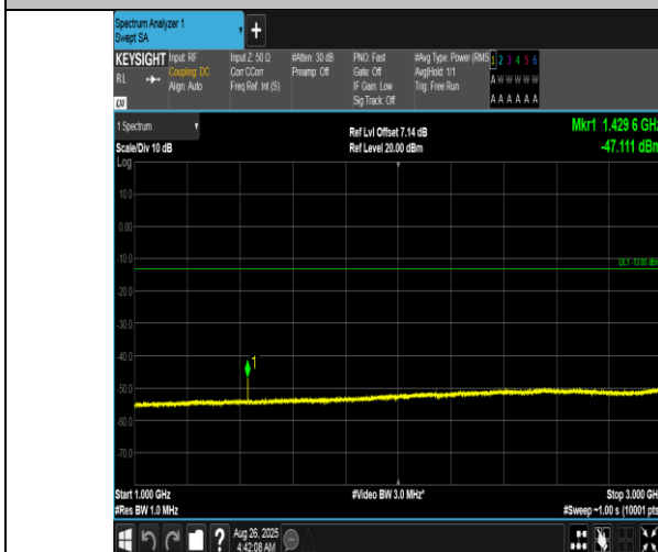
Band12-1.4MHz-16QAM-23173-1RB#0-1000~3000-PASS
