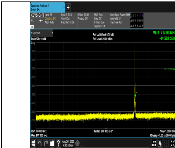
Band12-1.4MHz-QPSK-23173-1RB#0-30~1000-PASS
