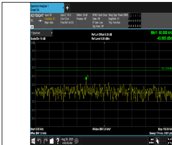
Band12-1.4MHz-16QAM-23173-1RB#5-0.009~0.15-PASS
