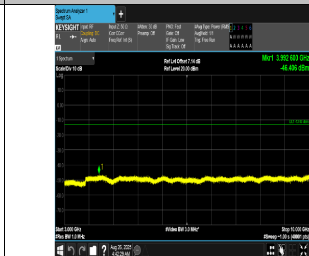
Band12-1.4MHz-16QAM-23173-1RB#0-3000~10000-PASS
