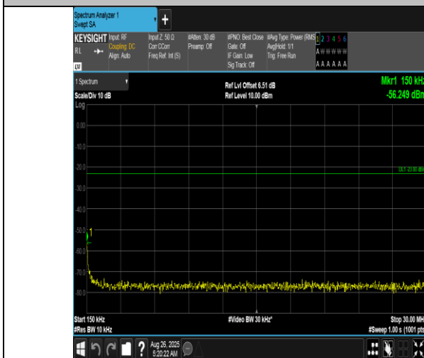
Band12-3MHz-QPSK-23025-1RB#14-0.15~30-PASS
