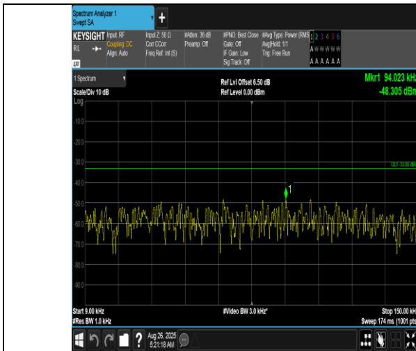
Band12-3MHz-16QAM-23025-1RB#14-0.009~0.15-PASS
