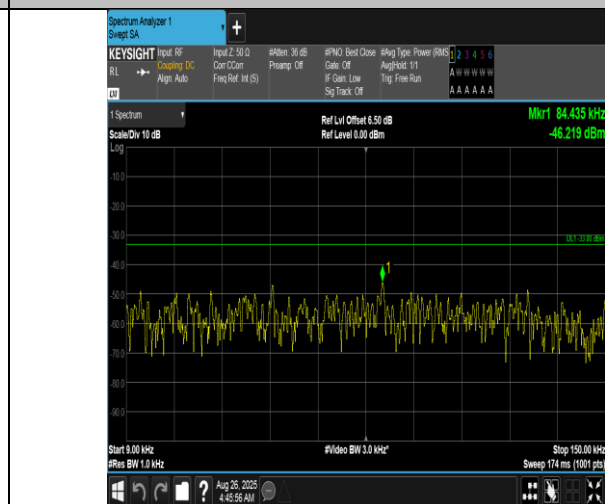
Band12-1.4MHz-16QAM-23173-6RB#0-0.009~0.15-PASS
