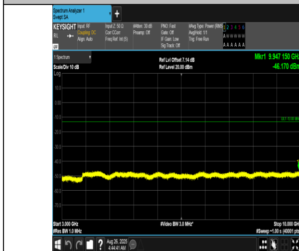
Band12-1.4MHz-16QAM-23173-1RB#5-3000~10000-PASS
