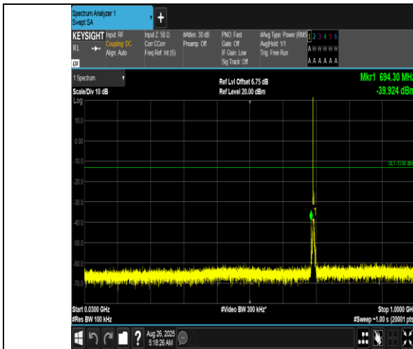
Band12-3MHz-QPSK-23025-1RB#0-30~1000-PASS
