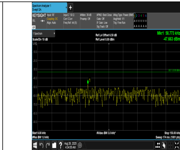
Band12-1.4MHz-16QAM-23095-1RB#0-0.009~0.15-PASS
