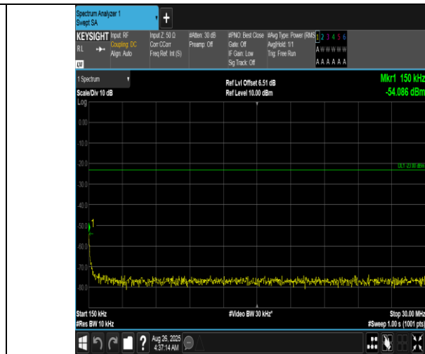
Band12-1.4MHz-16QAM-23095-1RB#5-0.15~30-PASS
