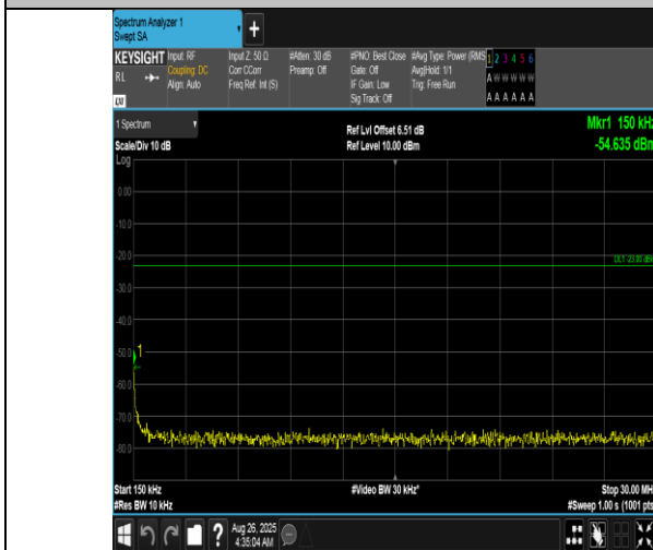
Band12-1.4MHz-16QAM-23095-1RB#0-0.15~30-PASS
