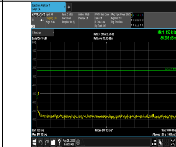
Band12-1.4MHz-QPSK-23173-6RB#0-0.15~30-PASS
