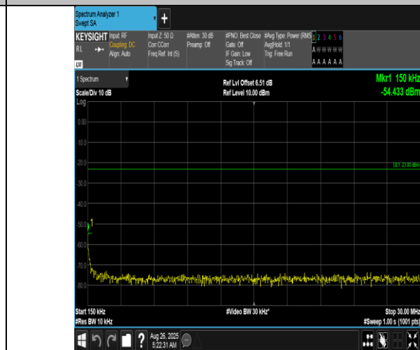
Band12-3MHz-QPSK-23025-15RB#0-0.15~30-PASS
