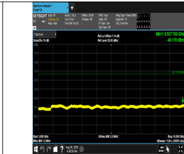
Band12-1.4MHz-QPSK-23095-1RB#5-3000~10000-PASS
