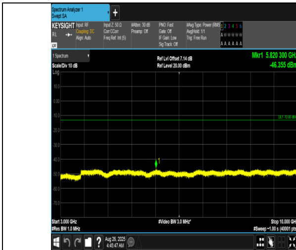
Band12-1.4MHz-QPSK-23173-6RB#0-3000~10000-PASS
