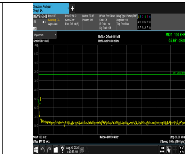
Band12-1.4MHz-16QAM-23173-1RB#5-0.15~30-PASS
