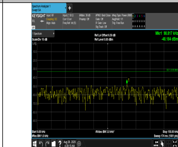
Band12-1.4MHz-16QAM-23095-6RB#0-0.009~0.15-PASS
