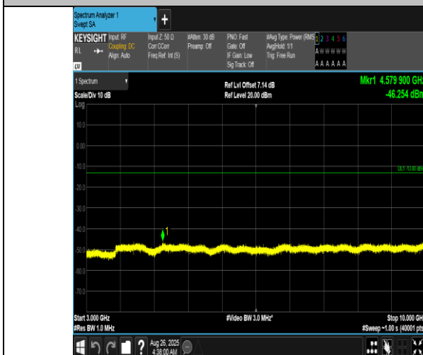
Band12-1.4MHz-16QAM-23095-1RB#5-3000~10000-PASS
