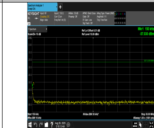
Band12-3MHz-QPSK-23025-1RB#0-0.15~30-PASS
