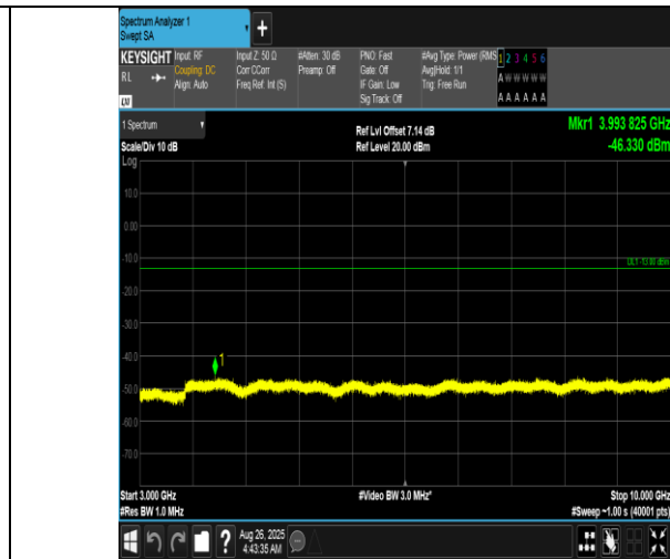
Band12-1.4MHz-QPSK-23173-1RB#5-3000~10000-PASS
