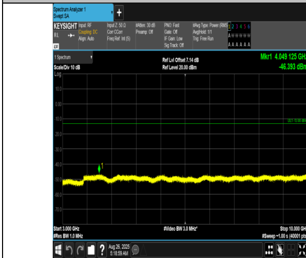
Band12-3MHz-QPSK-23025-1RB#0-3000~10000-PASS
