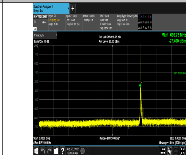
Band12-3MHz-QPSK-23025-1RB#14-30~1000-PASS
