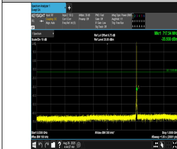
Band12-1.4MHz-16QAM-23173-1RB#5-30~1000-PASS
