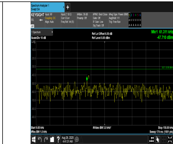
Band12-1.4MHz-16QAM-23173-1RB#0-0.009~0.15-PASS
