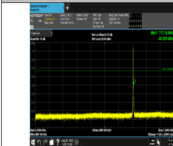
Band12-1.4MHz-QPSK-23173-6RB#0-30~1000-PASS
