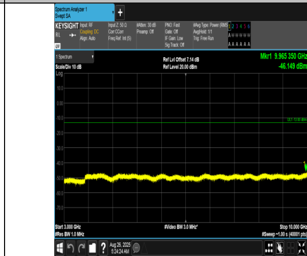
Band12-3MHz-16QAM-23025-15RB#0-3000~10000-PASS
