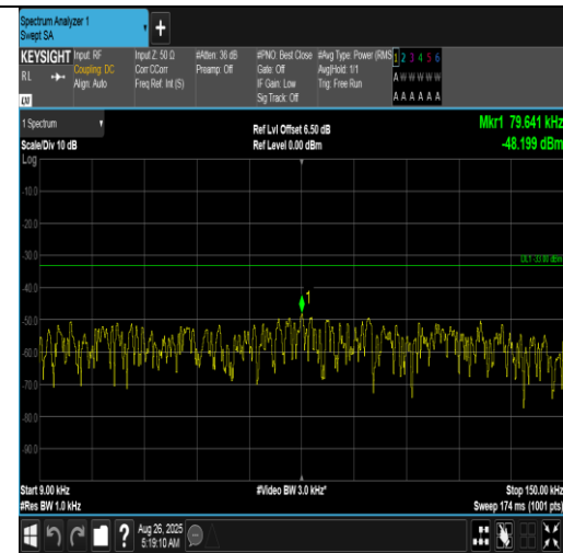
Band12-3MHz-16QAM-23025-1RB#0-0.009~0.15-PASS
