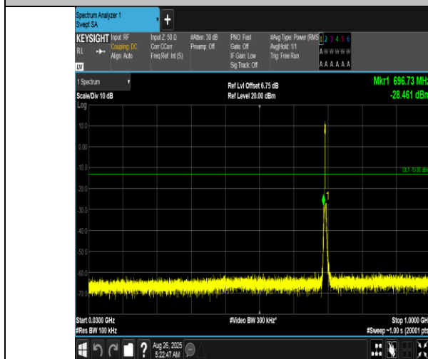
Band12-3MHz-QPSK-23025-15RB#0-30~1000-PASS
