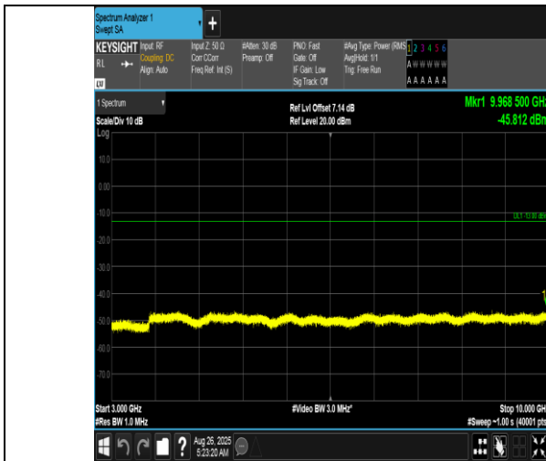
Band12-3MHz-QPSK-23025-15RB#0-3000~10000-PASS
