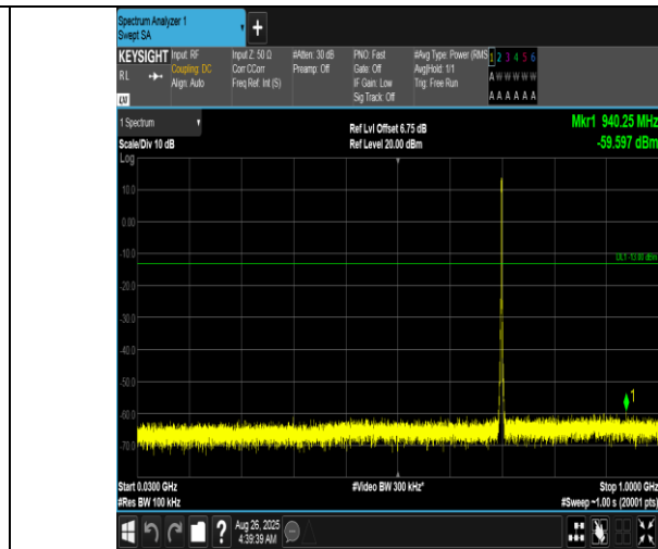
Band12-1.4MHz-16QAM-23095-6RB#0-30~1000-PASS
