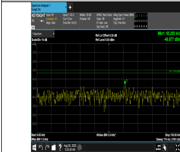
Band12-3MHz-QPSK-23095-1RB#0-0.009~0.15-PASS
