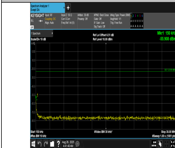
Band12-1.4MHz-16QAM-23173-1RB#0-0.15~30-PASS
