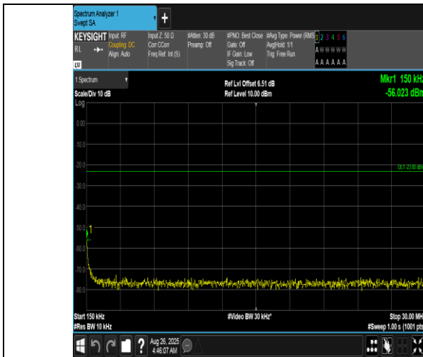
Band12-1.4MHz-16QAM-23173-6RB#0-0.15~30-PASS
