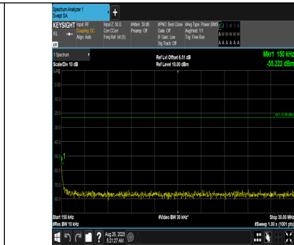
Band12-3MHz-16QAM-23025-1RB#14-0.15~30-PASS
