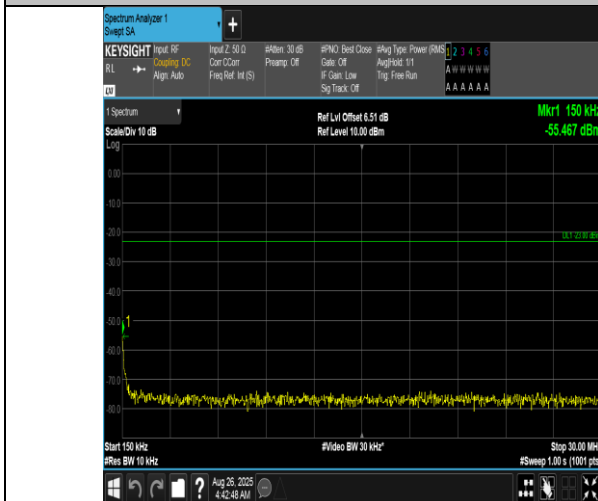
Band12-1.4MHz-QPSK-23173-1RB#5-0.15~30-PASS
