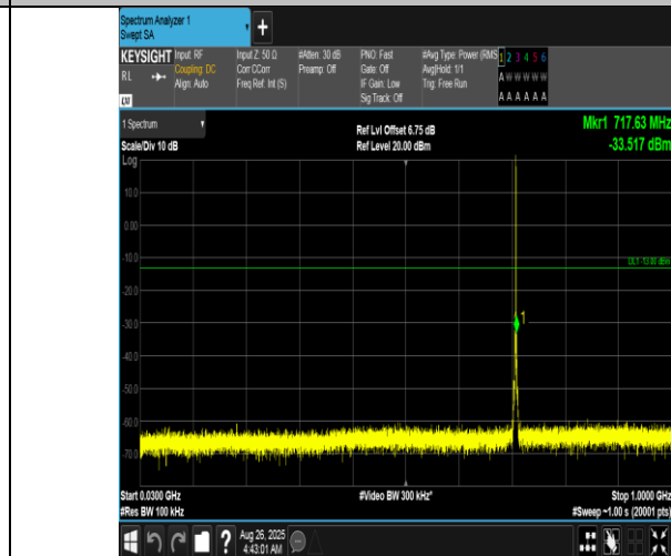
Band12-1.4MHz-QPSK-23173-1RB#5-30~1000-PASS
