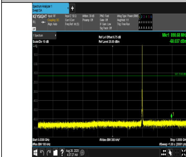
Band12-1.4MHz-16QAM-23095-1RB#5-30~1000-PASS
