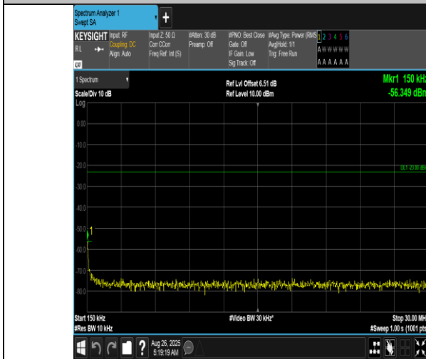
Band12-3MHz-16QAM-23025-1RB#0-0.15~30-PASS
