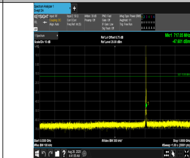
Band12-1.4MHz-16QAM-23173-1RB#0-30~1000-PASS
