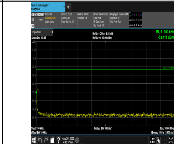
Band12-1.4MHz-QPSK-23173-1RB#0-0.15~30-PASS
