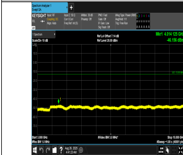
Band12-1.4MHz-QPSK-23173-1RB#0-3000~10000-PASS
