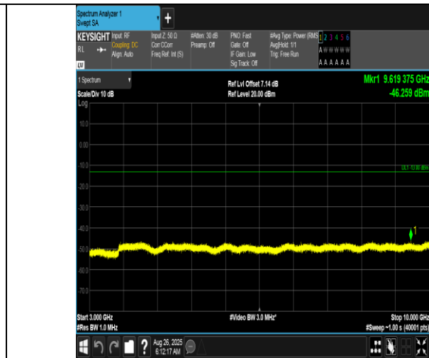
Band12-5MHz-QPSK-23035-1RB#24-3000~10000-PASS
