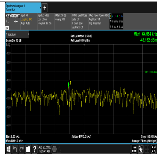
Band12-3MHz-16QAM-23095-1RB#0-0.009~0.15-PASS
