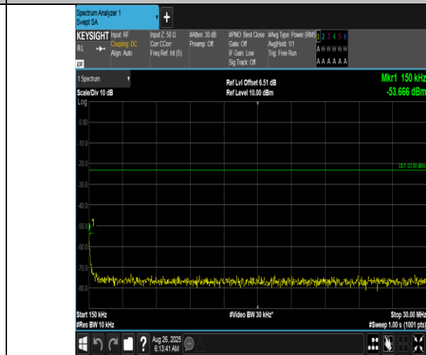
Band12-5MHz-QPSK-23035-25RB#0-0.15~30-PASS
