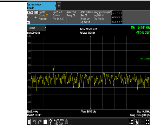
Band12-3MHz-16QAM-23095-15RB#0-0.009~0.15-PASS
