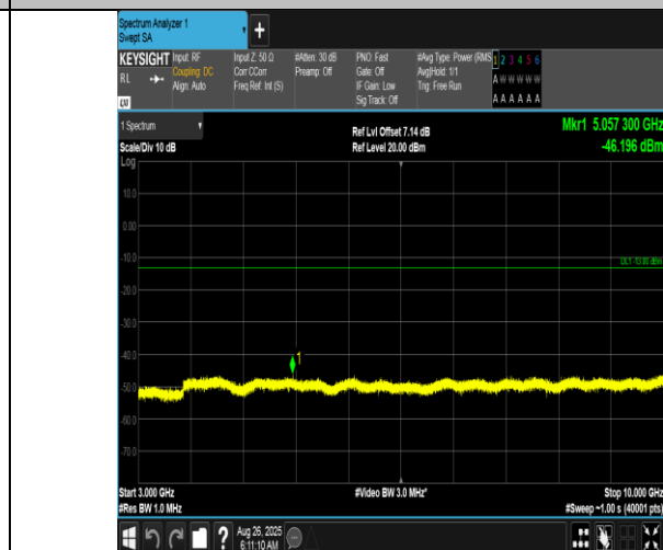
Band12-5MHz-16QAM-23035-1RB#0-3000~10000-PASS
