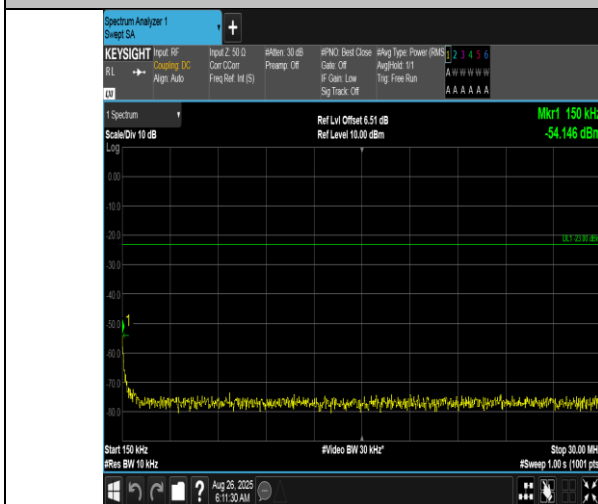
Band12-5MHz-QPSK-23035-1RB#24-0.15~30-PASS
