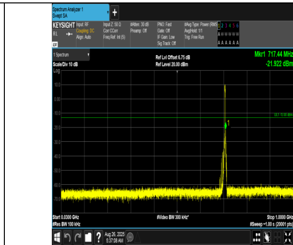
Band12-3MHz-16QAM-23165-15RB#0-30~1000-PASS
