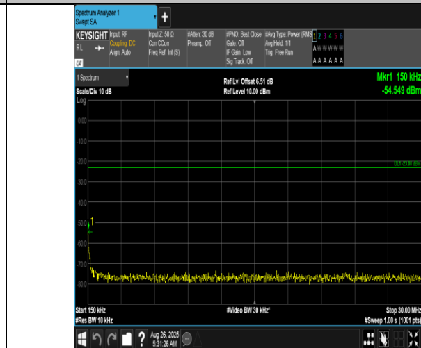
Band12-3MHz-QPSK-23165-1RB#0-0.15~30-PASS
