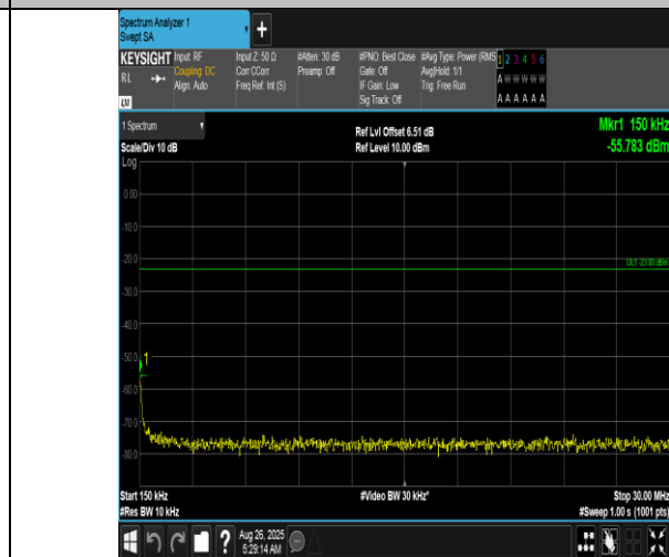
Band12-3MHz-QPSK-23095-15RB#0-0.15~30-PASS
