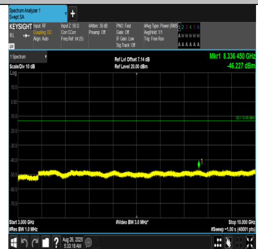
Band12-3MHz-16QAM-23165-1RB#0-3000~10000-PASS
