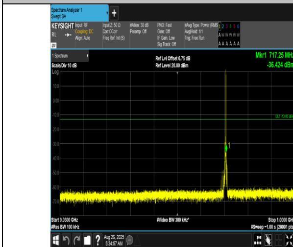
Band12-3MHz-16QAM-23165-1RB#14-30~1000-PASS
