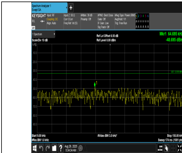
Band12-3MHz-16QAM-23165-1RB#14-0.009~0.15-PASS
