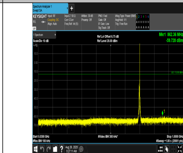
Band12-3MHz-QPSK-23095-1RB#14-30~1000-PASS
