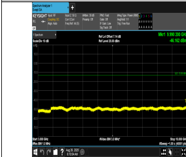
Band12-5MHz-QPSK-23035-1RB#0-3000~10000-PASS
