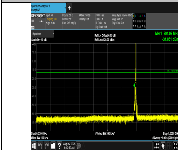
Band12-5MHz-16QAM-23035-1RB#24-30~1000-PASS
