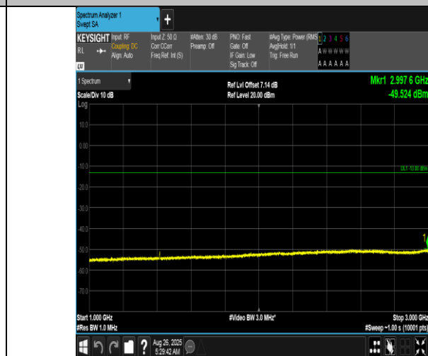
Band12-3MHz-QPSK-23095-15RB#0-1000~3000-PASS
