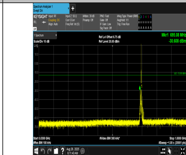
Band12-5MHz-QPSK-23035-1RB#24-30~1000-PASS
