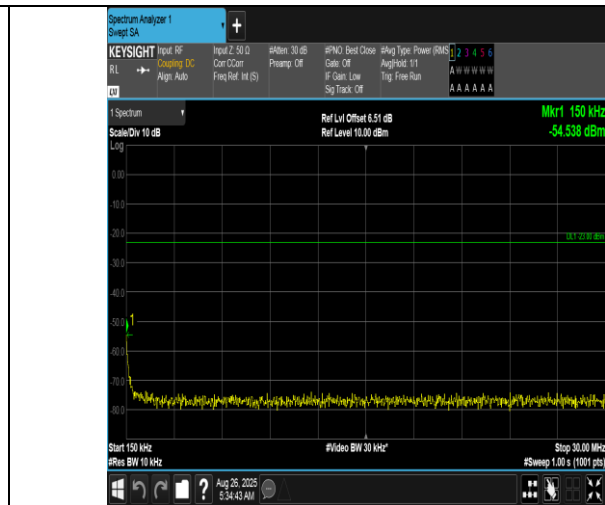
Band12-3MHz-16QAM-23165-1RB#14-0.15~30-PASS
