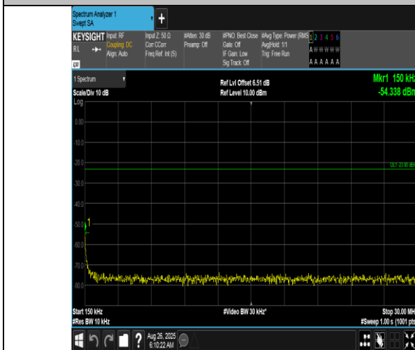
Band12-5MHz-16QAM-23035-1RB#0-0.15~30-PASS
