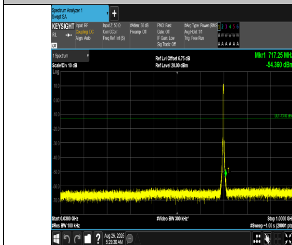
Band12-3MHz-QPSK-23095-15RB#0-30~1000-PASS
