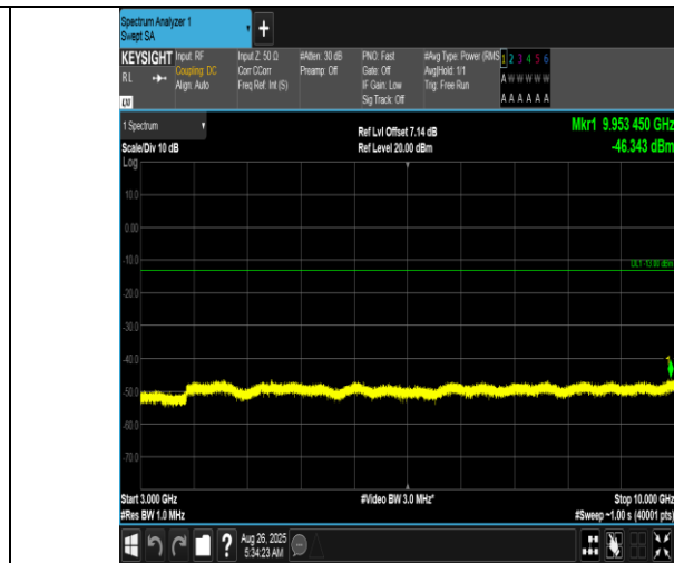
Band12-3MHz-QPSK-23165-1RB#14-3000~10000-PASS
