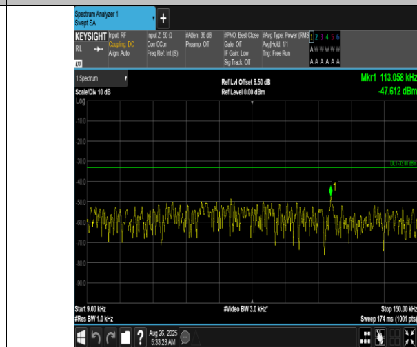
Band12-3MHz-QPSK-23165-1RB#14-0.009~0.15-PASS
