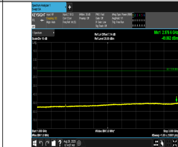
Band12-5MHz-QPSK-23035-25RB#0-1000~3000-PASS
