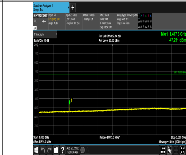
Band12-3MHz-16QAM-23095-1RB#14-1000~3000-PASS
