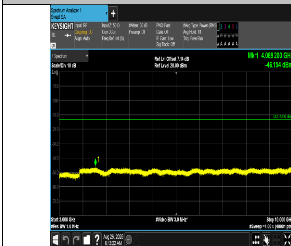
Band12-5MHz-16QAM-23035-1RB#24-3000~10000-PASS
