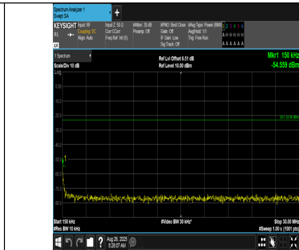
Band12-3MHz-16QAM-23095-1RB#14-0.15~30-PASS
