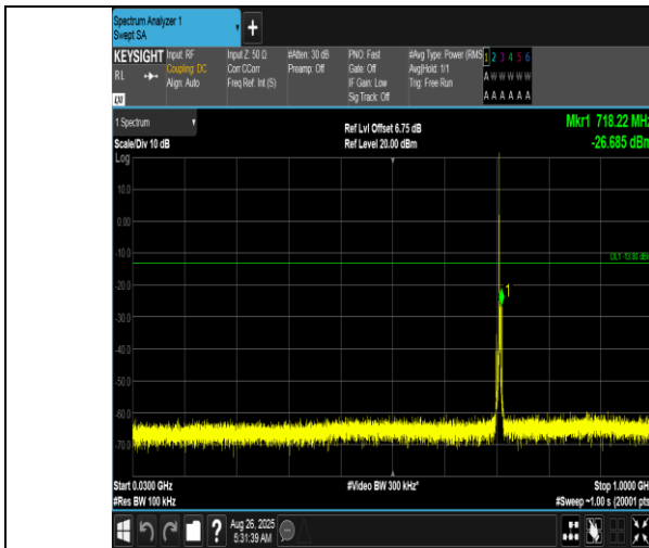
Band12-3MHz-QPSK-23165-1RB#0-30~1000-PASS
