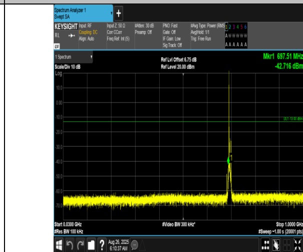
Band12-5MHz-16QAM-23035-1RB#0-30~1000-PASS
