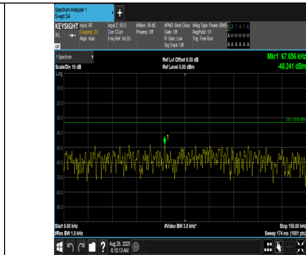
Band12-5MHz-16QAM-23035-1RB#0-0.009~0.15-PASS
