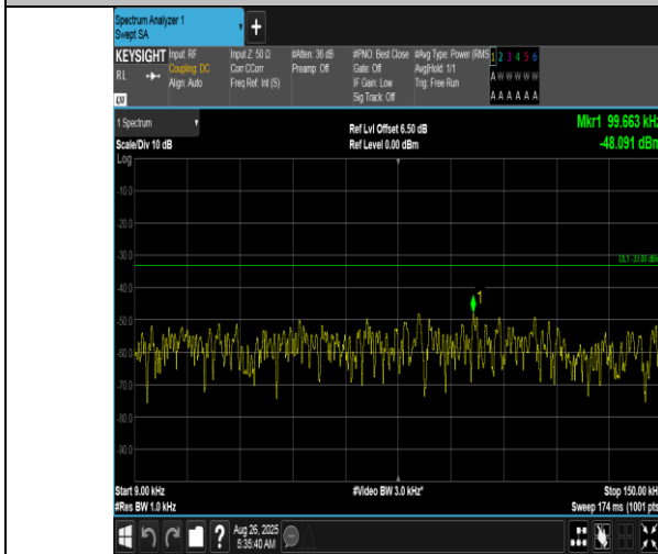
Band12-3MHz-QPSK-23165-15RB#0-0.009~0.15-PASS
