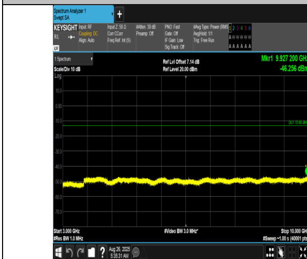
Band12-3MHz-16QAM-23165-1RB#14-3000~10000-PASS
