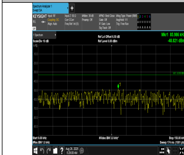
Band12-3MHz-QPSK-23095-15RB#0-0.009~0.15-PASS
