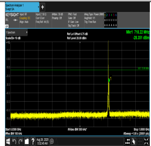
Band12-3MHz-16QAM-23165-1RB#0-30~1000-PASS
