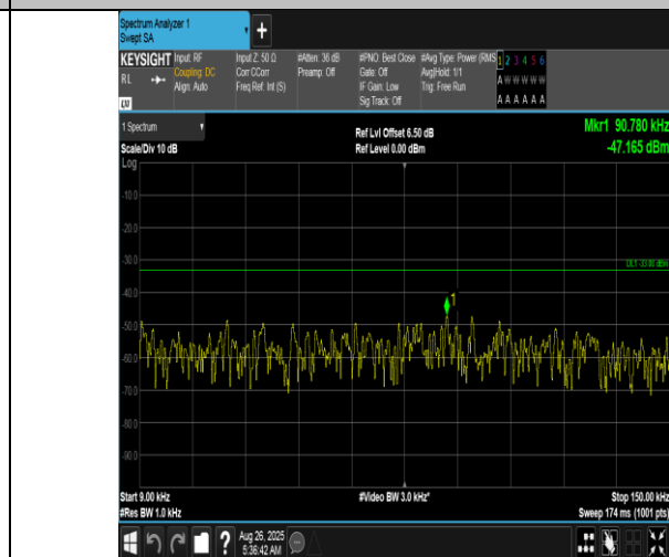
Band12-3MHz-16QAM-23165-15RB#0-0.009~0.15-PASS
