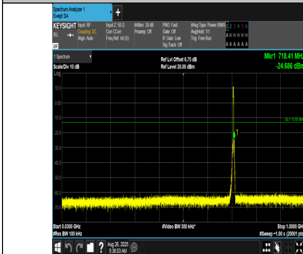
Band12-3MHz-QPSK-23165-15RB#0-30~1000-PASS
