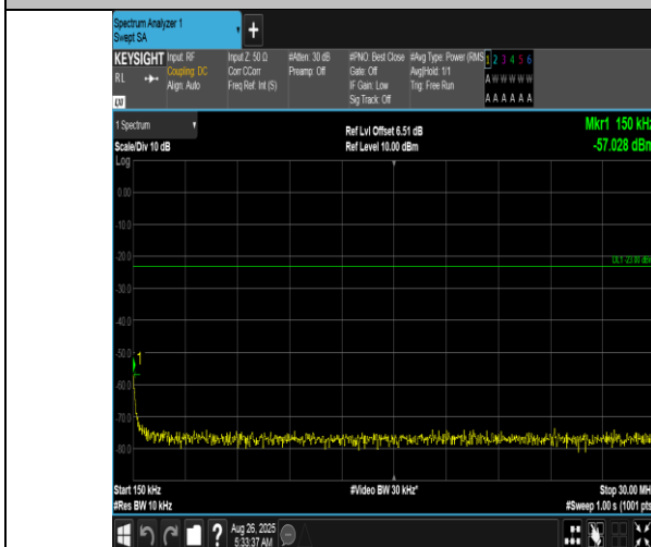
Band12-3MHz-QPSK-23165-1RB#14-0.15~30-PASS
