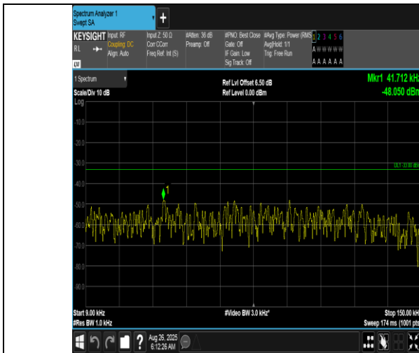
Band12-5MHz-16QAM-23035-1RB#24-0.009~0.15-PASS
