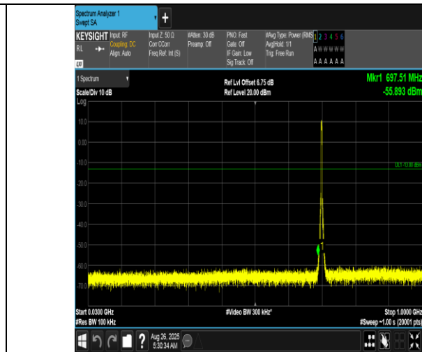
Band12-3MHz-16QAM-23095-15RB#0-30~1000-PASS
