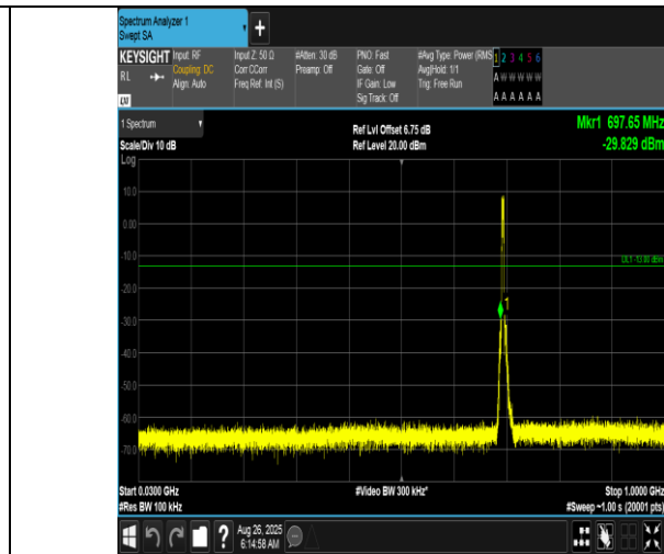
Band12-5MHz-16QAM-23035-25RB#0-30~1000-PASS
