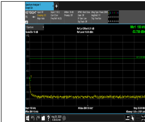
Band12-3MHz-16QAM-23165-15RB#0-0.15~30-PASS
