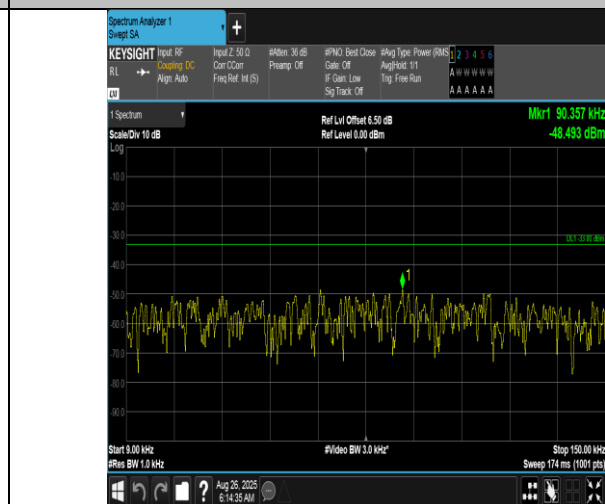
Band12-5MHz-16QAM-23035-25RB#0-0.009~0.15-PASS
