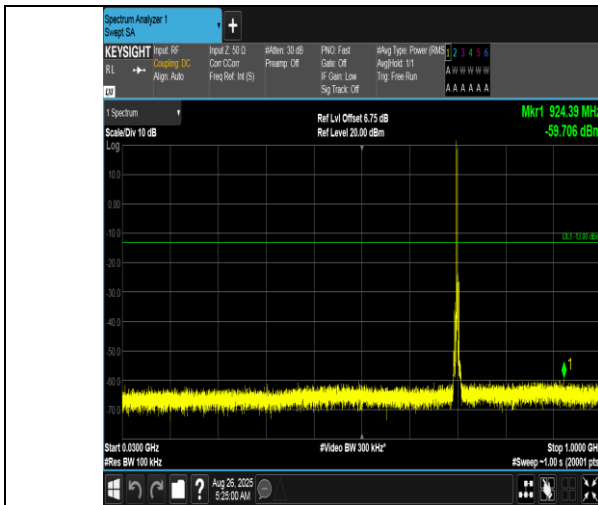
Band12-3MHz-QPSK-23095-1RB#0-30~1000-PASS
