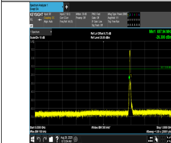
Band12-5MHz-QPSK-23035-25RB#0-30~1000-PASS
