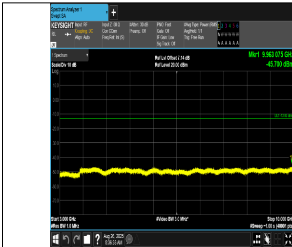
Band12-3MHz-QPSK-23165-15RB#0-3000~10000-PASS
