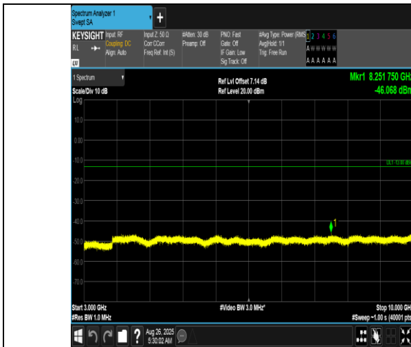
Band12-3MHz-QPSK-23095-15RB#0-3000~10000-PASS
