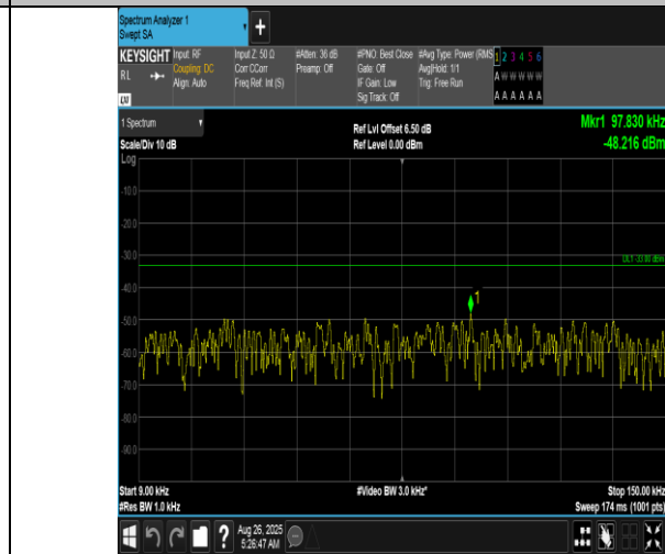
Band12-3MHz-QPSK-23095-1RB#14-0.009~0.15-PASS
