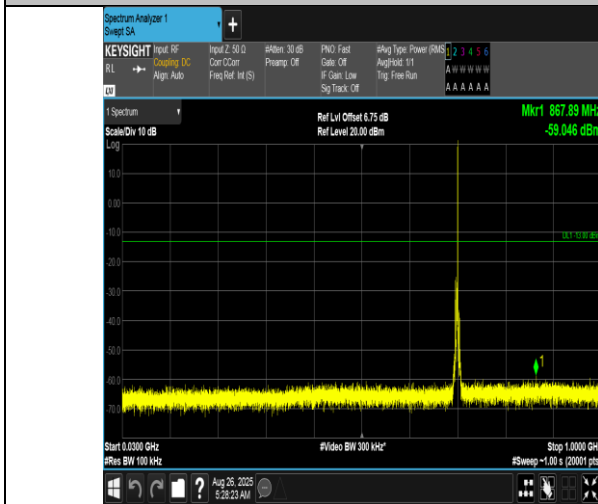
Band12-3MHz-16QAM-23095-1RB#14-30~1000-PASS
