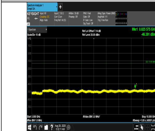
Band12-3MHz-QPSK-23165-1RB#0-3000~10000-PASS
