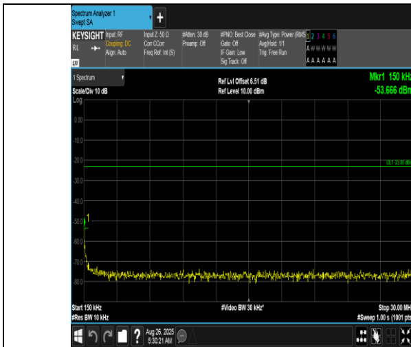
Band12-3MHz-16QAM-23095-15RB#0-0.15~30-PASS
