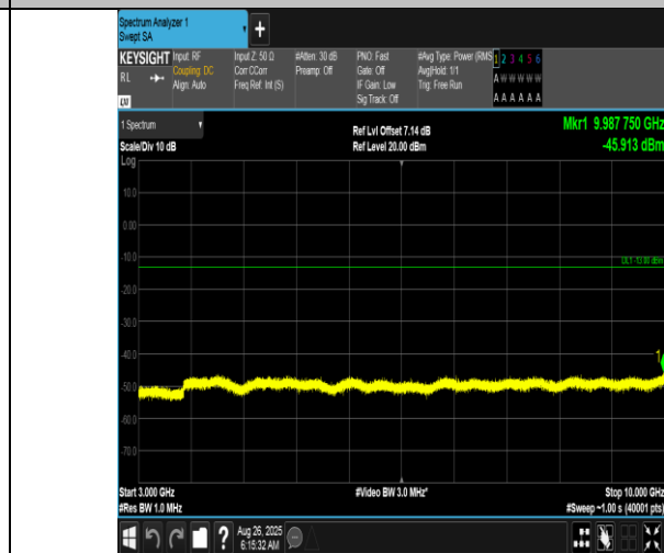
Band12-5MHz-16QAM-23035-25RB#0-3000~10000-PASS
