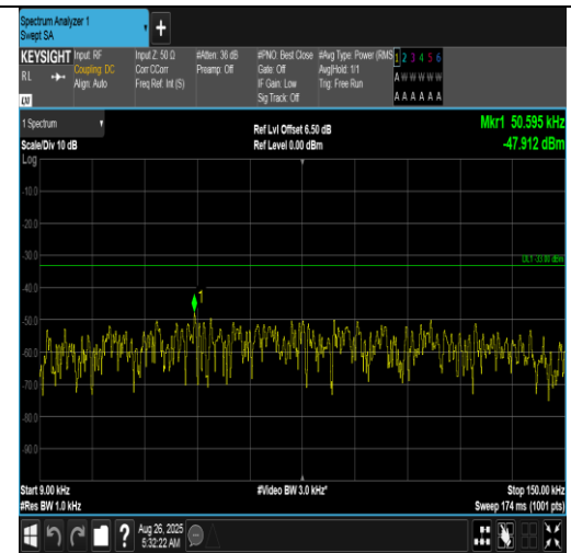
Band12-3MHz-16QAM-23165-1RB#0-0.009~0.15-PASS
