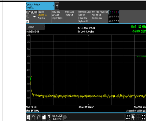
Band12-3MHz-QPSK-23165-15RB#0-0.15~30-PASS
