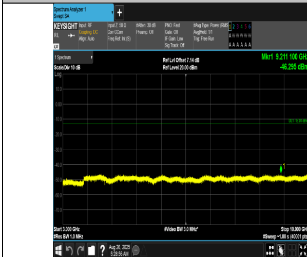
Band12-3MHz-16QAM-23095-1RB#14-3000~10000-PASS
