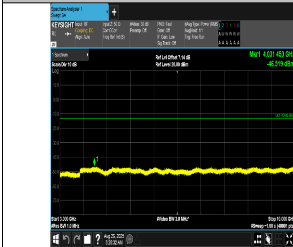
Band12-3MHz-QPSK-23095-1RB#0-3000~10000-PASS
