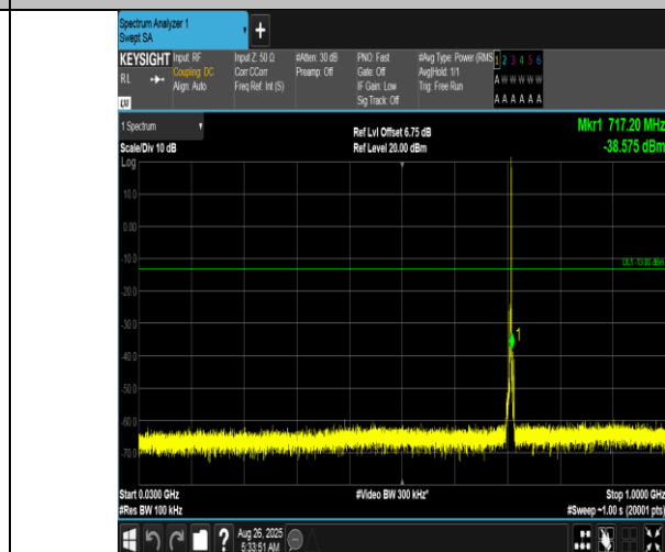
Band12-3MHz-QPSK-23165-1RB#14-30~1000-PASS
