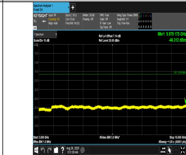
Band12-3MHz-16QAM-23095-15RB#0-3000~10000-PASS
