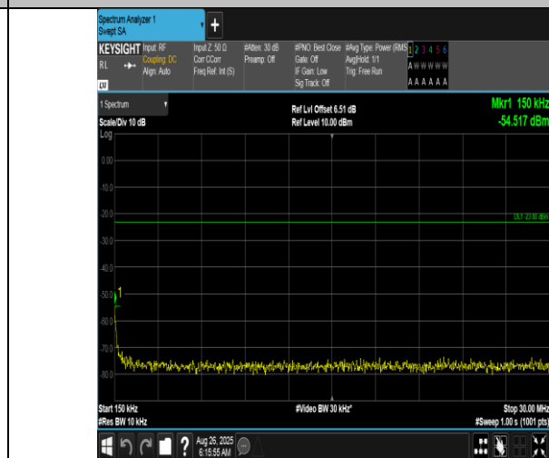
Band12-5MHz-QPSK-23095-1RB#0-0.15~30-PASS
