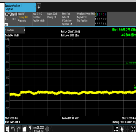
Band12-3MHz-16QAM-23095-1RB#0-3000~10000-PASS
