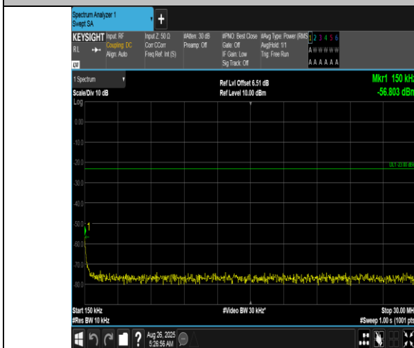
Band12-3MHz-QPSK-23095-1RB#14-0.15~30-PASS
