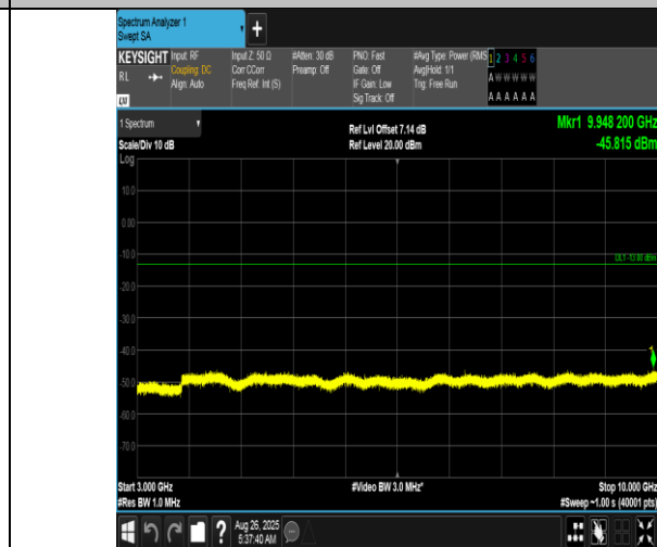
Band12-3MHz-16QAM-23165-15RB#0-3000~10000-PASS
