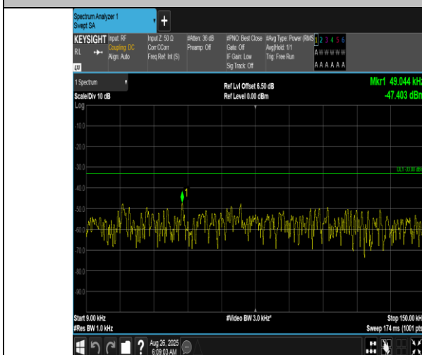
Band12-5MHz-QPSK-23035-1RB#0-0.009~0.15-PASS
