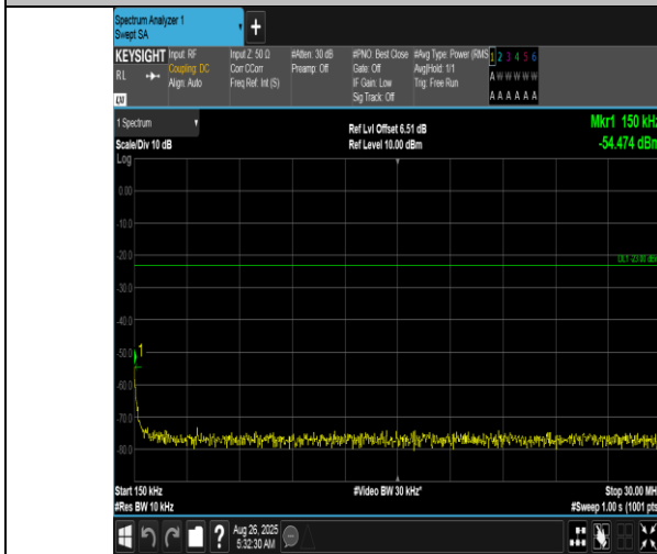
Band12-3MHz-16QAM-23165-1RB#0-0.15~30-PASS
