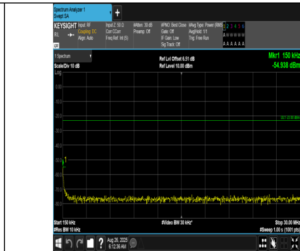
Band12-5MHz-16QAM-23035-1RB#24-0.15~30-PASS
