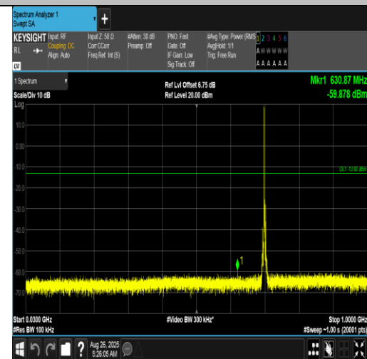
Band12-3MHz-16QAM-23095-1RB#0-30~1000-PASS
