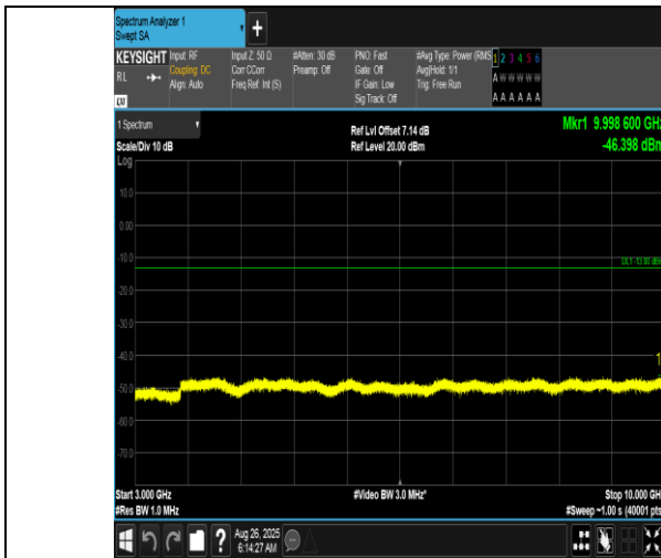
Band12-5MHz-QPSK-23035-25RB#0-3000~10000-PASS
