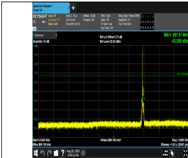
Band12-5MHz-QPSK-23035-1RB#0-30~1000-PASS
