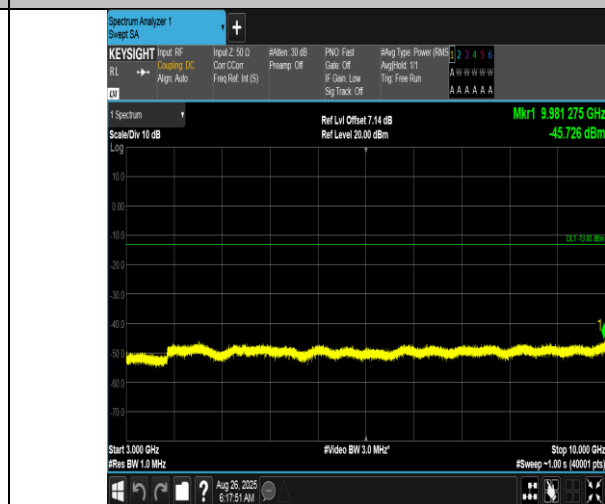
Band12-5MHz-16QAM-23095-1RB#0-3000~10000-PASS
