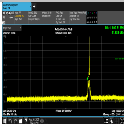
Band12-10MHz-16QAM-23060-1RB#49-30~1000-PASS
