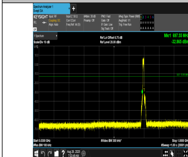
Band12-10MHz-QPSK-23060-50RB#0-30~1000-PASS
