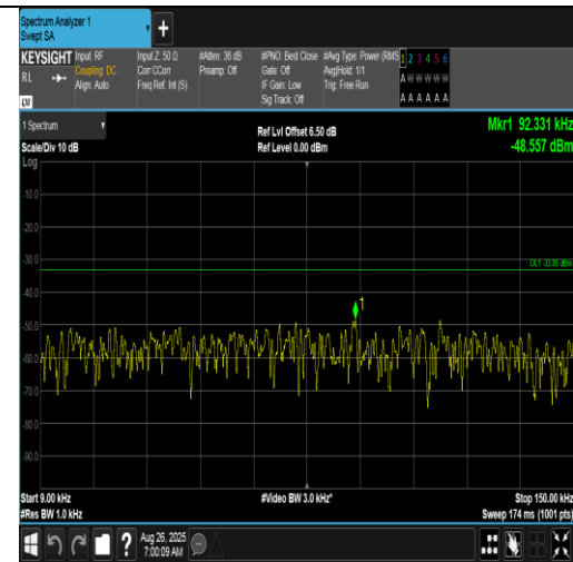
Band12-10MHz-16QAM-23060-1RB#0-0.009~0.15-PASS
