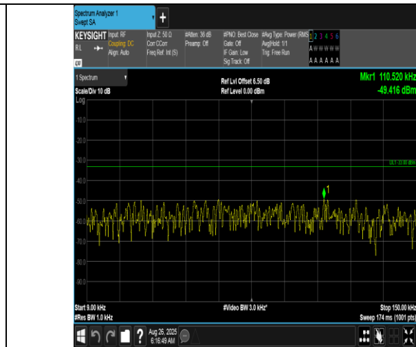
Band12-5MHz-16QAM-23095-1RB#0-0.009~0.15-PASS
