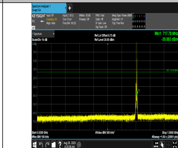
Band12-5MHz-QPSK-23155-1RB#24-30~1000-PASS
