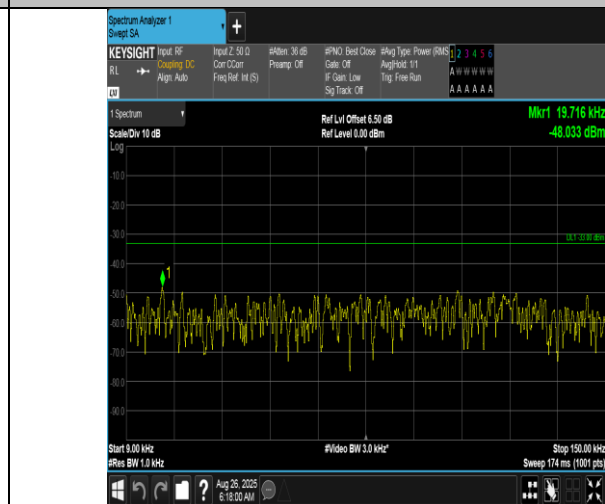
Band12-5MHz-QPSK-23095-1RB#24-0.009~0.15-PASS
