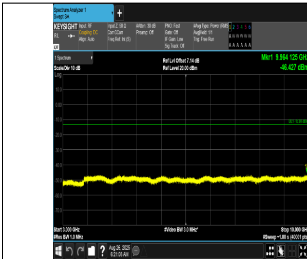
Band12-5MHz-QPSK-23095-25RB#0-3000~10000-PASS
