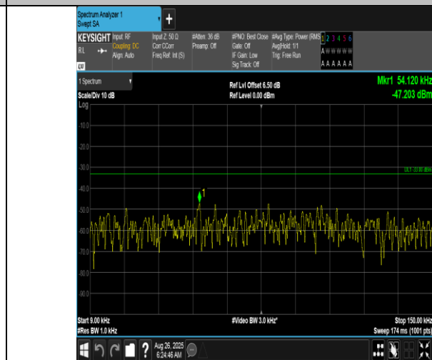
Band12-5MHz-QPSK-23155-1RB#24-0.009~0.15-PASS
