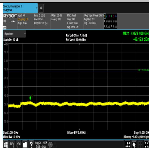
Band12-10MHz-16QAM-23060-1RB#49-3000~10000-PASS
