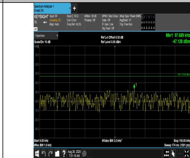
Band12-10MHz-QPSK-23060-1RB#49-0.009~0.15-PASS
