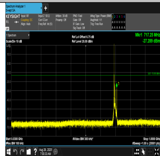
Band12-10MHz-16QAM-23060-1RB#0-30~1000-PASS
