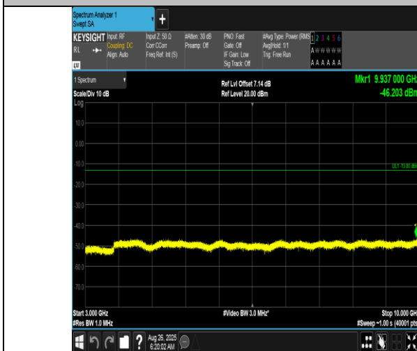
Band12-5MHz-16QAM-23095-1RB#24-3000~10000-PASS
