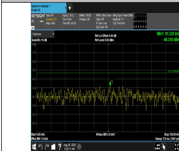
Band12-5MHz-QPSK-23095-25RB#0-0.009~0.15-PASS
