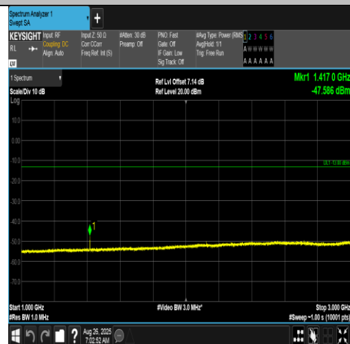
Band12-10MHz-16QAM-23060-1RB#49-1000~3000-PASS
