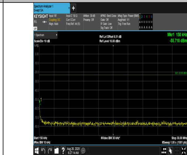
Band12-5MHz-QPSK-23155-25RB#0-0.15~30-PASS
