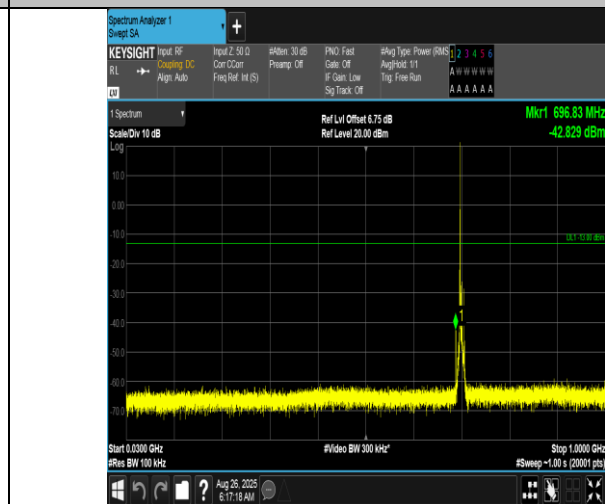
Band12-5MHz-16QAM-23095-1RB#0-30~1000-PASS
