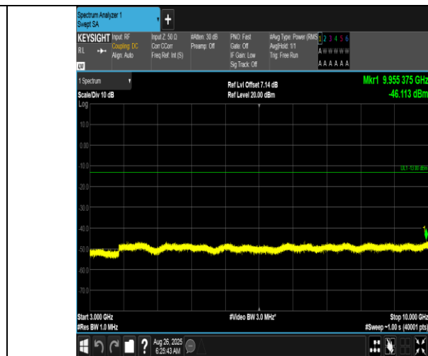
Band12-5MHz-QPSK-23155-1RB#24-3000~10000-PASS
