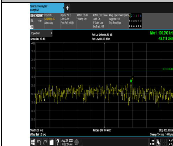
Band12-5MHz-QPSK-23155-1RB#0-0.009~0.15-PASS
