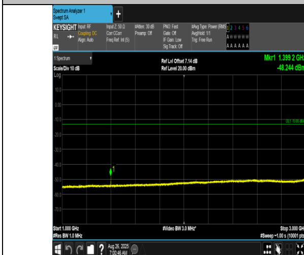
Band12-10MHz-16QAM-23060-1RB#0-1000~3000-PASS
