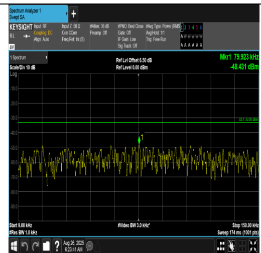
Band12-5MHz-16QAM-23155-1RB#0-0.009~0.15-PASS
