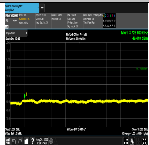
Band12-5MHz-16QAM-23155-1RB#0-3000~10000-PASS
