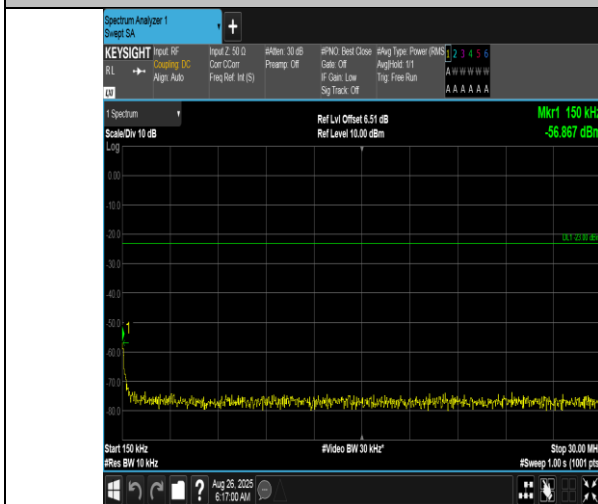
Band12-5MHz-16QAM-23095-1RB#0-0.15~30-PASS
