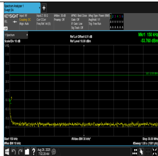
Band12-10MHz-16QAM-23060-1RB#49-0.15~30-PASS
