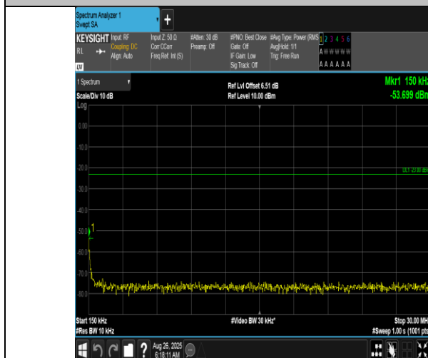
Band12-5MHz-QPSK-23095-1RB#24-0.15~30-PASS
