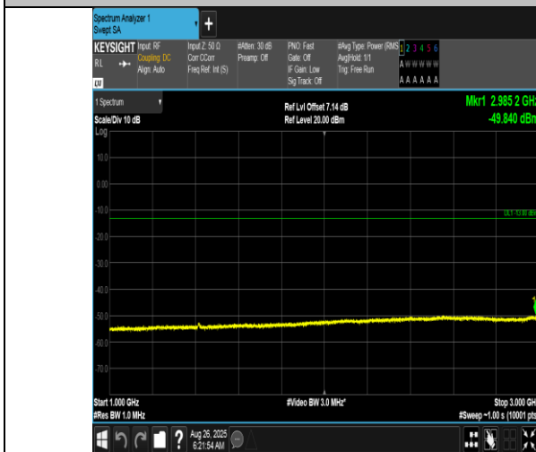
Band12-5MHz-16QAM-23095-25RB#0-1000~3000-PASS
