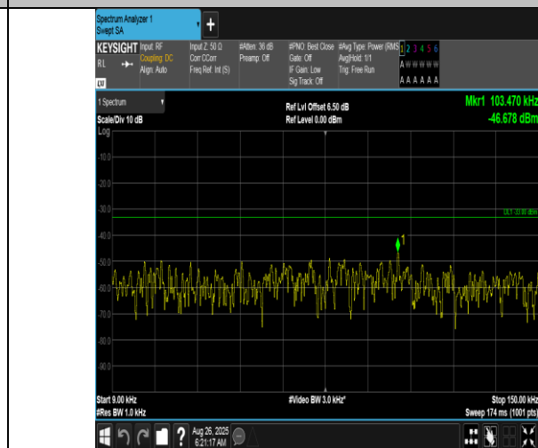
Band12-5MHz-16QAM-23095-25RB#0-0.009~0.15-PASS
