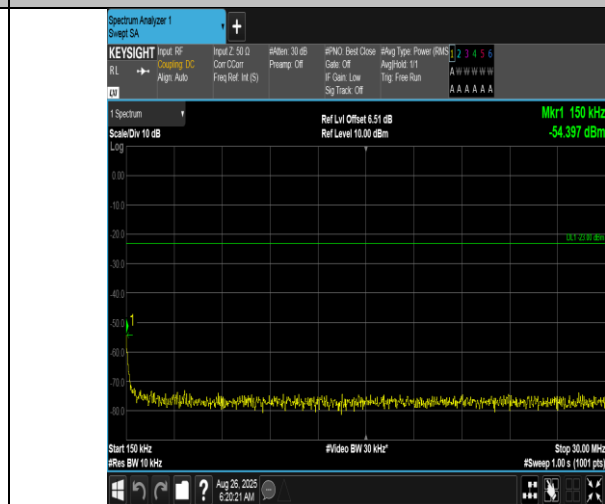
Band12-5MHz-QPSK-23095-25RB#0-0.15~30-PASS
