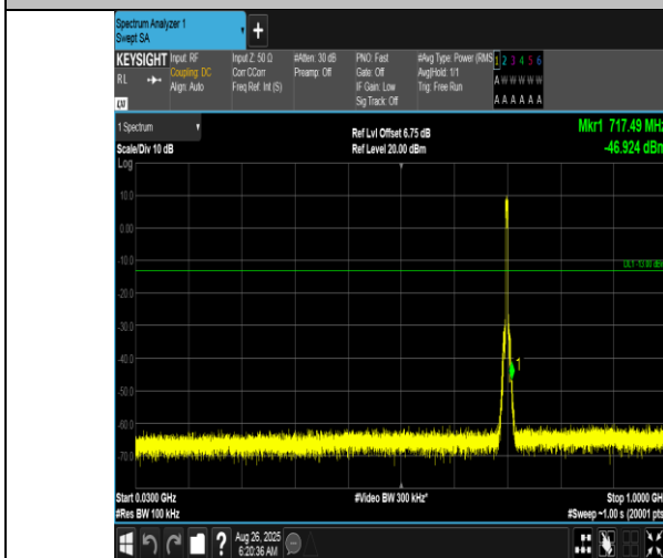
Band12-5MHz-QPSK-23095-25RB#0-30~1000-PASS
