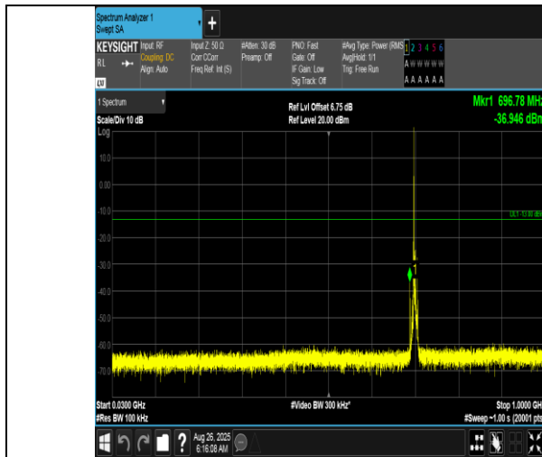
Band12-5MHz-QPSK-23095-1RB#0-30~1000-PASS
