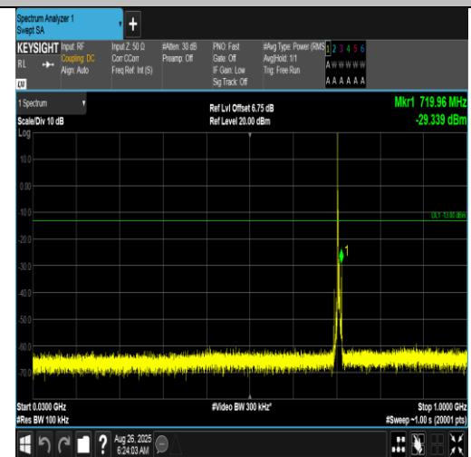
Band12-5MHz-16QAM-23155-1RB#0-30~1000-PASS
