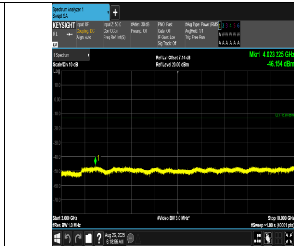
Band12-5MHz-QPSK-23095-1RB#24-3000~10000-PASS
