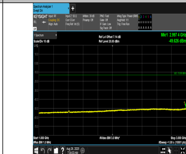
Band12-10MHz-QPSK-23060-50RB#0-1000~3000-PASS
