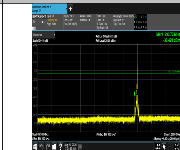
Band12-10MHz-QPSK-23060-1RB#49-30~1000-PASS
