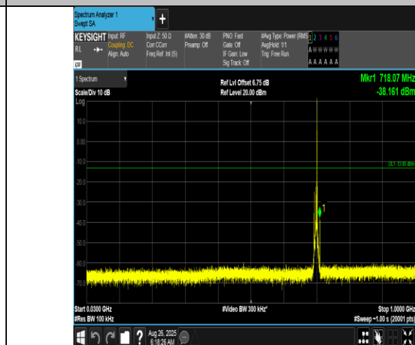
Band12-5MHz-QPSK-23095-1RB#24-30~1000-PASS
