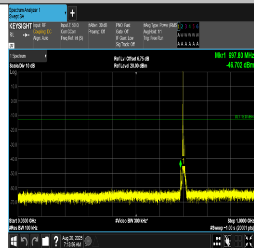
Band12-10MHz-16QAM-23130-1RB#0-30~1000-PASS
