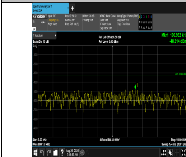
Band12-10MHz-QPSK-23130-50RB#0-0.009~0.15-PASS
