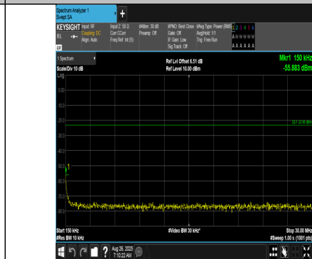
Band12-10MHz-QPSK-23095-50RB#0-0.15~30-PASS
