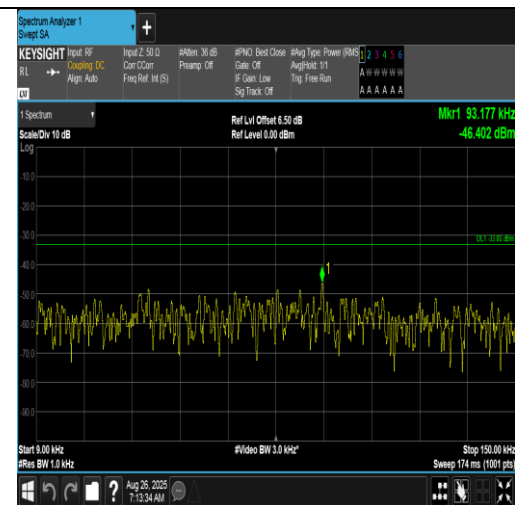
Band12-10MHz-16QAM-23130-1RB#0-0.009~0.15-PASS
