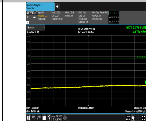
Band12-10MHz-QPSK-23095-50RB#0-1000~3000-PASS
