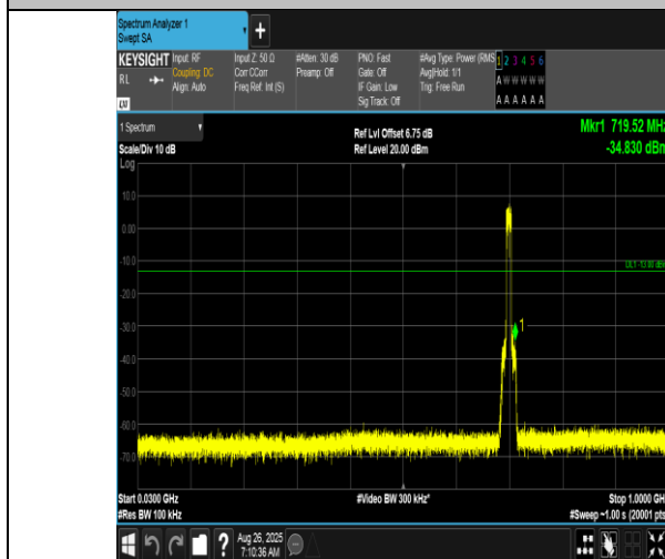
Band12-10MHz-QPSK-23095-50RB#0-30~1000-PASS
