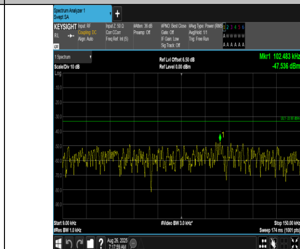
Band12-10MHz-16QAM-23130-50RB#0-0.009~0.15-PASS
