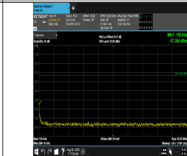
Band12-10MHz-QPSK-23130-50RB#0-0.15~30-PASS
