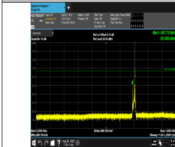
Band12-10MHz-16QAM-23130-1RB#49-30~1000-PASS
