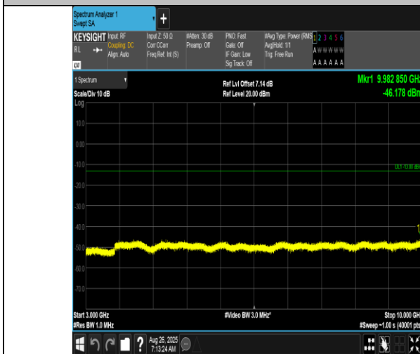
Band12-10MHz-QPSK-23130-1RB#0-3000~10000-PASS
