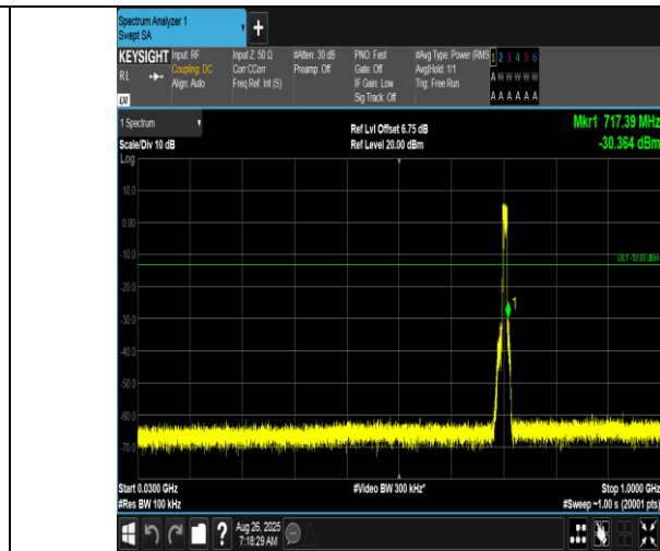
Band12-10MHz-16QAM-23130-50RB#0-30~1000-PASS
