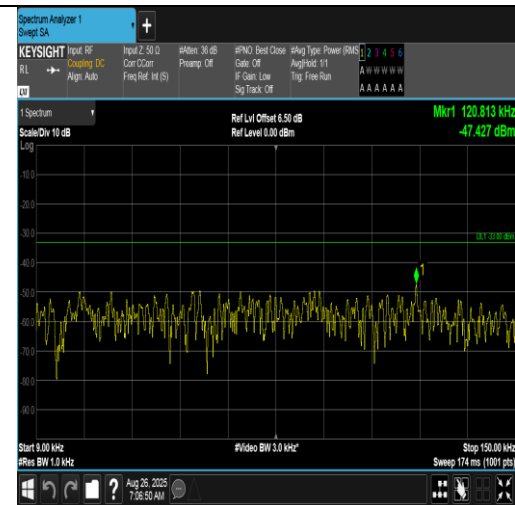
Band12-10MHz-16QAM-23095-1RB#0-0.009~0.15-PASS
