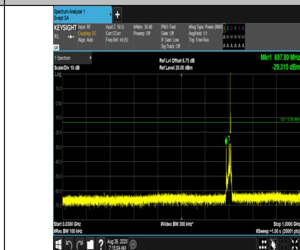
Band12-10MHz-QPSK-23130-1RB#49-30~1000-PASS
