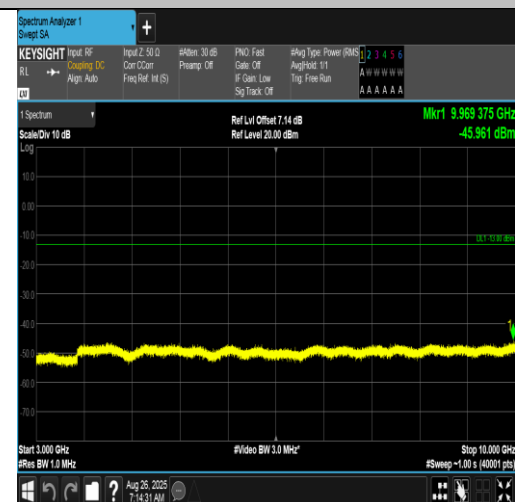
Band12-10MHz-16QAM-23130-1RB#0-3000~10000-PASS
