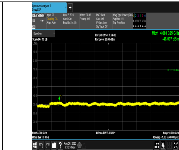
Band12-10MHz-QPSK-23130-1RB#49-3000~10000-PASS
