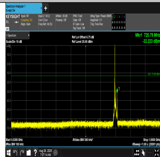
Band12-10MHz-16QAM-23095-1RB#0-30~1000-PASS
