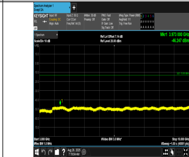
Band12-10MHz-16QAM-23130-50RB#0-3000~10000-PASS
