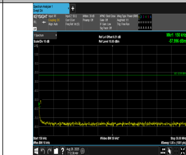
Band12-10MHz-QPSK-23130-1RB#0-0.15~30-PASS
