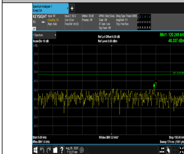
Band12-10MHz-QPSK-23130-1RB#0-0.009~0.15-PASS
