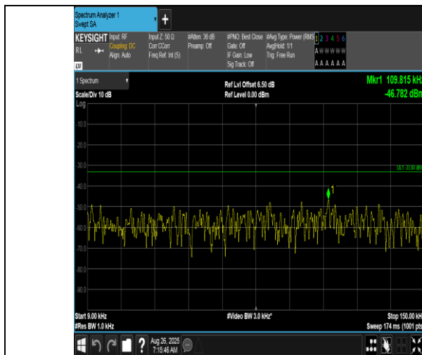
Band12-10MHz-16QAM-23130-1RB#49-0.009~0.15-PASS
