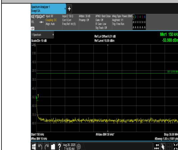
Band12-10MHz-QPSK-23130-1RB#49-0.15~30-PASS
