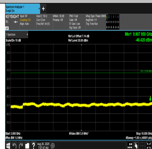
Band12-10MHz-16QAM-23095-1RB#0-3000~10000-PASS
