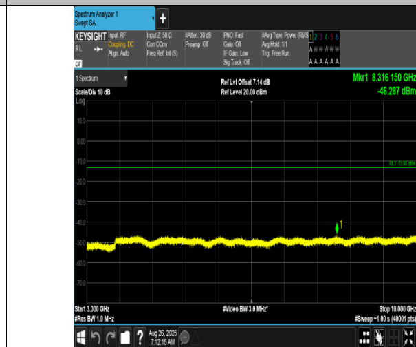
Band12-10MHz-16QAM-23095-50RB#0-3000~10000-PASS
