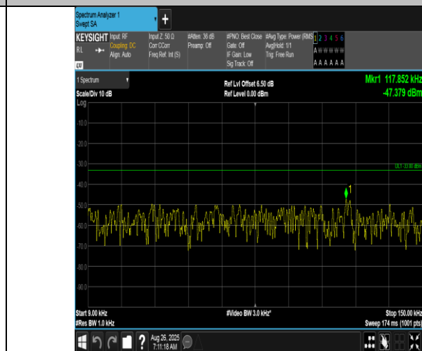
Band12-10MHz-16QAM-23095-50RB#0-0.009~0.15-PASS
