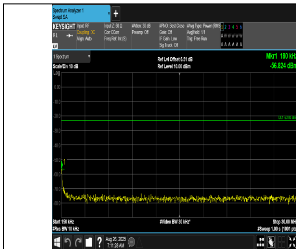
Band12-10MHz-16QAM-23095-50RB#0-0.15~30-PASS
