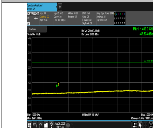
Band12-10MHz-16QAM-23130-1RB#0-1000~3000-PASS
