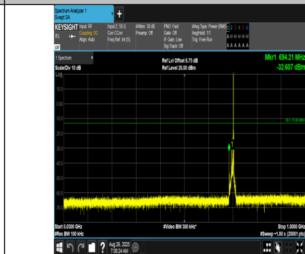
Band12-10MHz-QPSK-23095-1RB#49-30~1000-PASS
