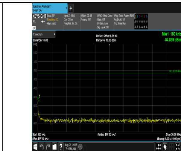
Band12-10MHz-16QAM-23130-1RB#49-0.15~30-PASS
