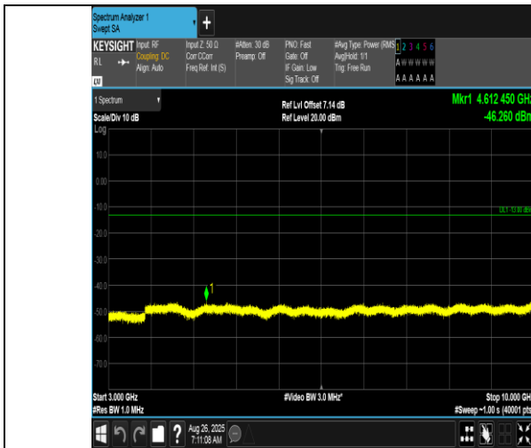
Band12-10MHz-QPSK-23095-50RB#0-3000~10000-PASS
