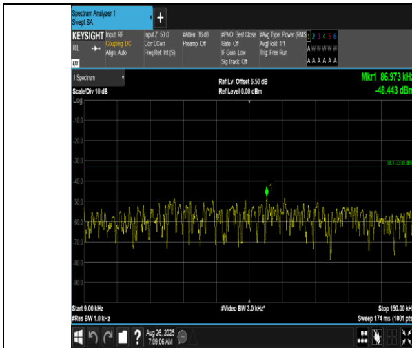
Band12-10MHz-16QAM-23095-1RB#49-0.009~0.15-PASS
