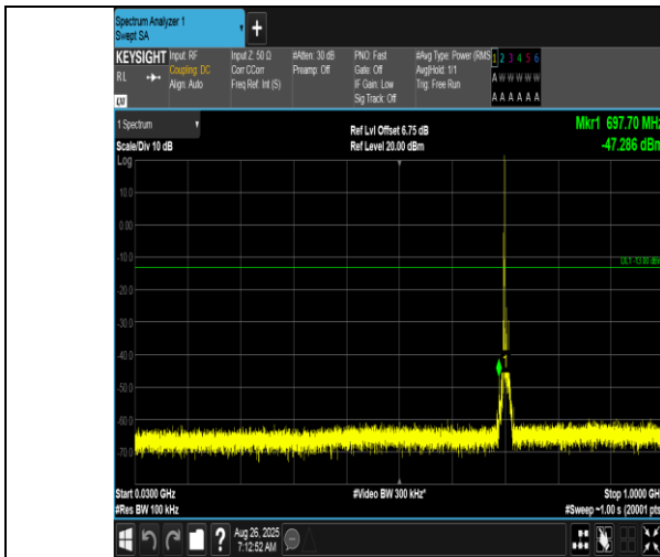
Band12-10MHz-QPSK-23130-1RB#0-30~1000-PASS
