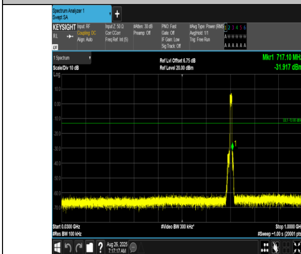
Band12-10MHz-QPSK-23130-50RB#0-30~1000-PASS
