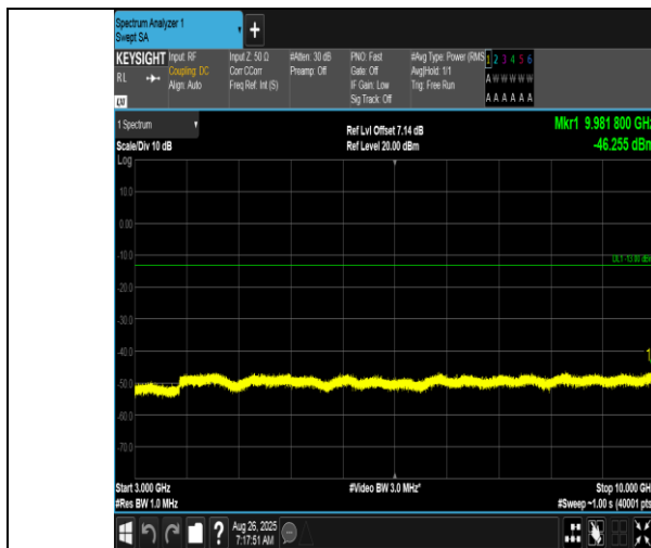
Band12-10MHz-QPSK-23130-50RB#0-3000~10000-PASS
