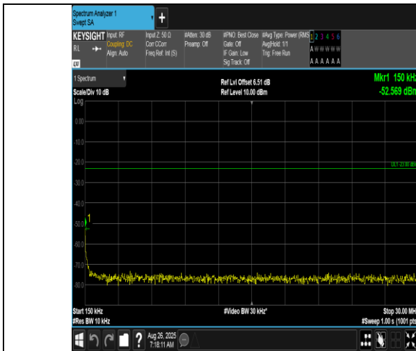
Band12-10MHz-16QAM-23130-50RB#0-0.15~30-PASS
