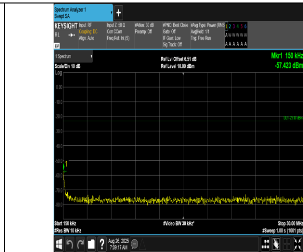
Band12-10MHz-16QAM-23095-1RB#49-0.15~30-PASS
