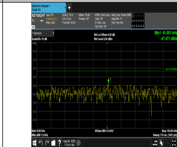
Band12-10MHz-QPSK-23130-1RB#49-0.009~0.15-PASS
