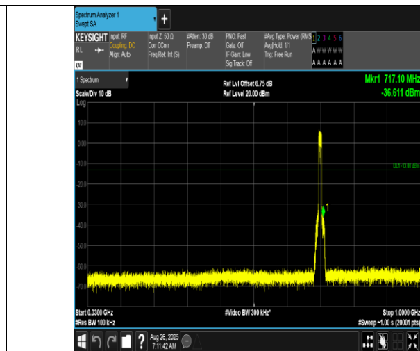
Band12-10MHz-16QAM-23095-50RB#0-30~1000-PASS
