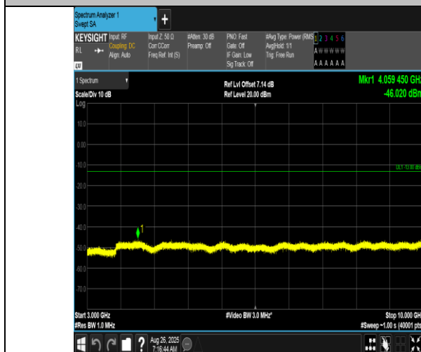
Band12-10MHz-16QAM-23130-1RB#49-3000~10000-PASS
