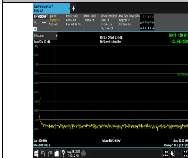
Band12-10MHz-16QAM-23130-1RB#0-0.15~30-PASS
