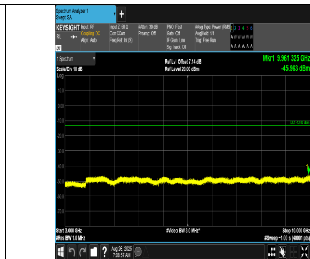
Band12-10MHz-QPSK-23095-1RB#49-3000~10000-PASS
