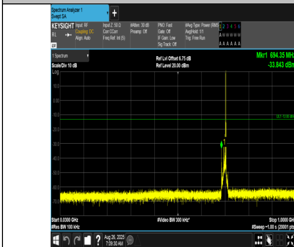
Band12-10MHz-16QAM-23095-1RB#49-30~1000-PASS
