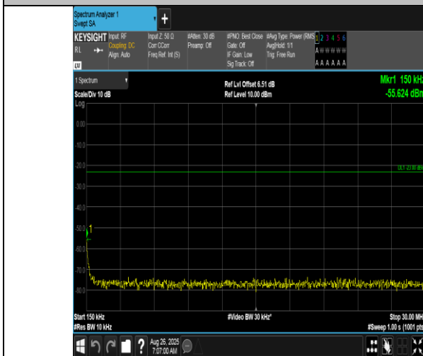
Band12-10MHz-16QAM-23095-1RB#0-0.15~30-PASS
