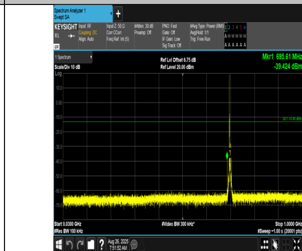
Band17-5MHz-16QAM-23755-1RB#0-30~1000-PASS
