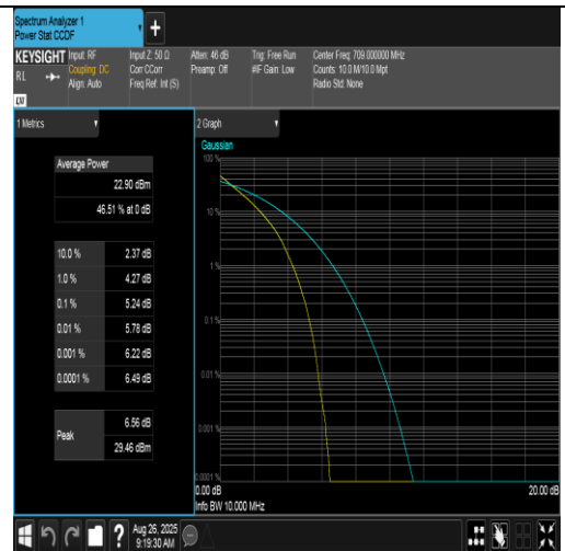
Band17-10MHz-QPSK-23780-50RB#0-PASS
