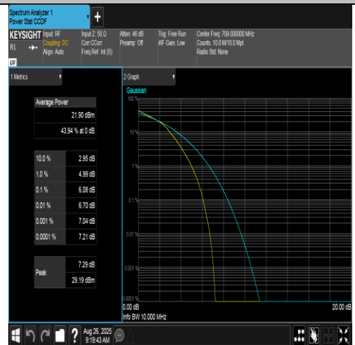
Band17-10MHz-16QAM-23780-50RB#0-PASS
