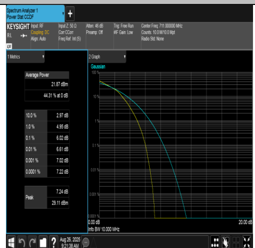
Band17-10MHz-16QAM-23800-50RB#0-PASS
