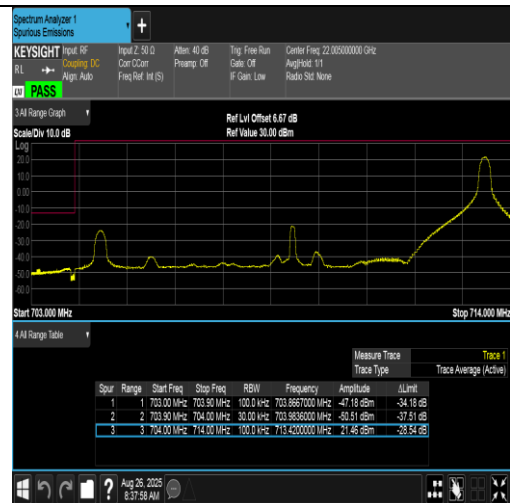
Band17-10MHz-QPSK-23780-1RB#49-PASS
