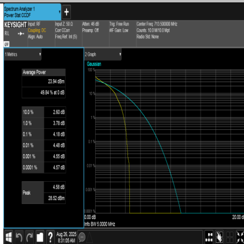
Band17-5MHz-QPSK-23825-1RB#0-PASS
