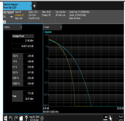
Band17-5MHz-16QAM-23825-25RB#0-PASS
