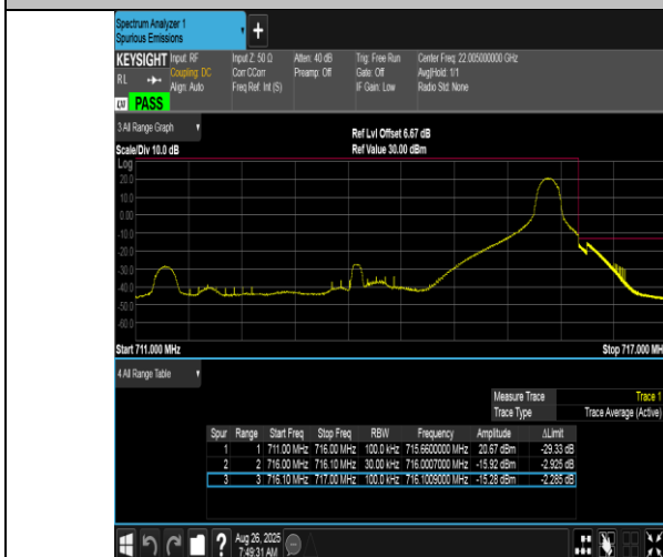
Band17-5MHz-16QAM-23825-1RB#24-PASS
