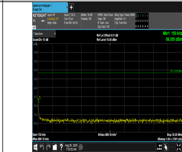
Band17-5MHz-16QAM-23755-1RB#24-0.15~30-PASS
