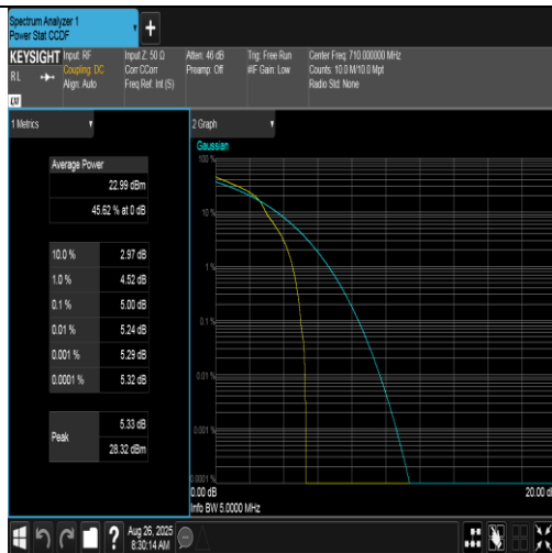
Band17-5MHz-16QAM-23790-1RB#0-PASS
