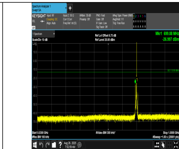
Band17-5MHz-QPSK-23755-1RB#24-30~1000-PASS
