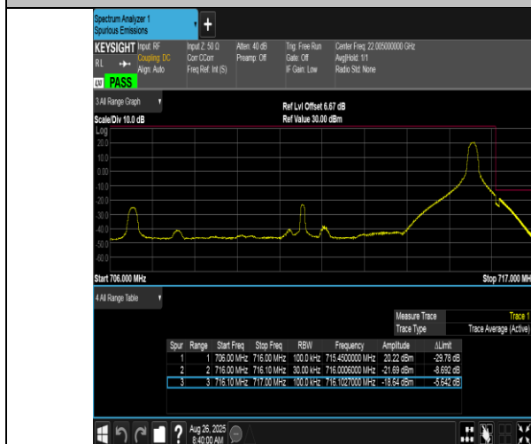
Band17-10MHz-16QAM-23800-1RB#49-PASS
