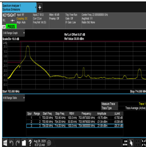
Band17-10MHz-QPSK-23780-1RB#0-PASS
