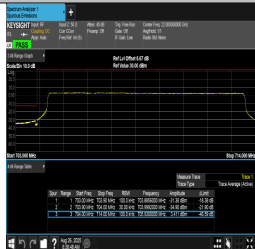
Band17-10MHz-16QAM-23780-50RB#0-PASS
