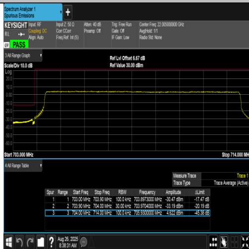
Band17-10MHz-QPSK-23780-50RB#0-PASS
