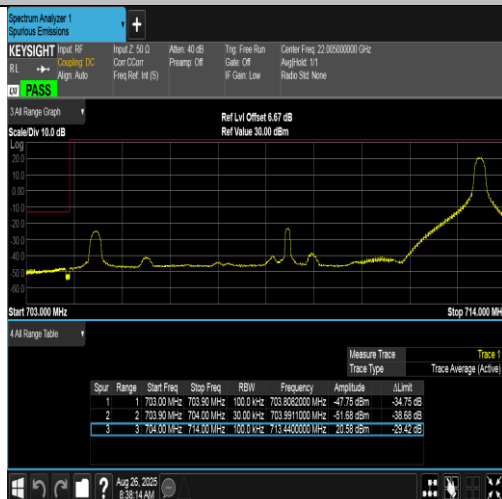
Band17-10MHz-16QAM-23780-1RB#49-PASS
