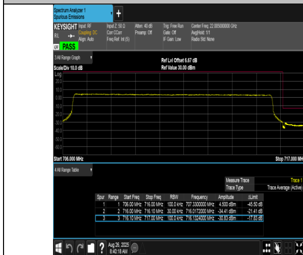
Band17-10MHz-QPSK-23800-50RB#0-PASS
