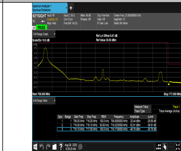
Band17-10MHz-16QAM-23800-1RB#0-PASS
