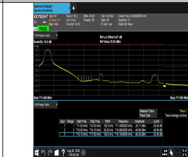
Band17-5MHz-16QAM-23825-1RB#0-PASS
