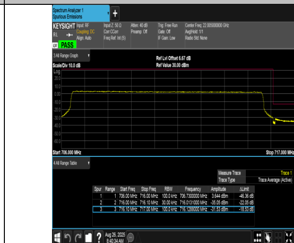
Band17-10MHz-16QAM-23800-50RB#0-PASS
