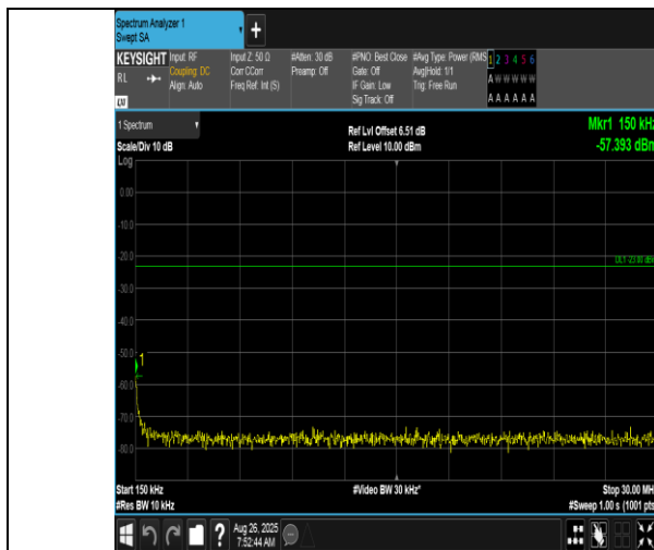
Band17-5MHz-QPSK-23755-1RB#24-0.15~30-PASS
