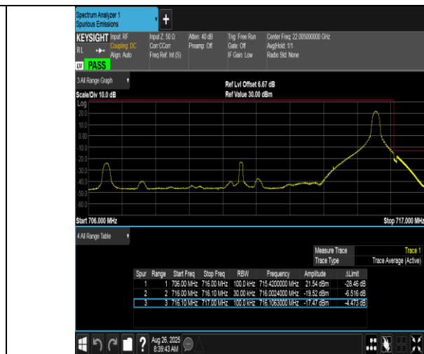
Band17-10MHz-QPSK-23800-1RB#49-PASS
