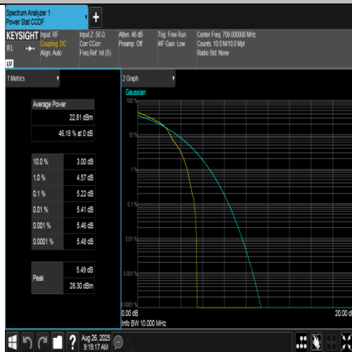
Band17-10MHz-16QAM-23780-1RB#0-PASS
