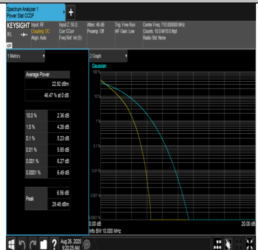
Band17-10MHz-QPSK-23790-50RB#0-PASS
