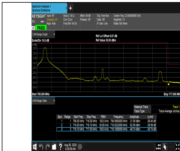
Band17-10MHz-QPSK-23800-1RB#0-PASS
