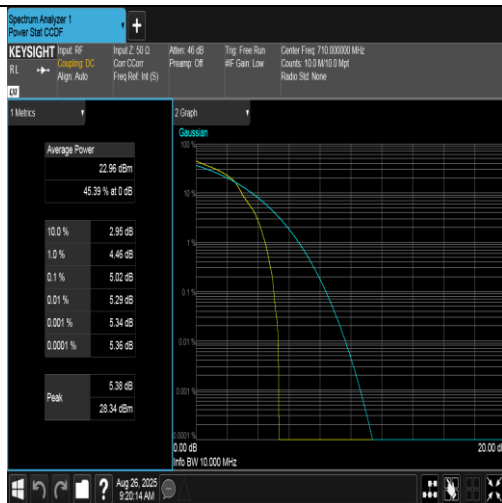
Band17-10MHz-16QAM-23790-1RB#0-PASS
