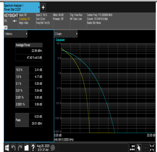
Band17-5MHz-QPSK-23825-25RB#0-PASS
