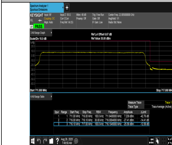
Band17-5MHz-QPSK-23825-25RB#0-PASS
