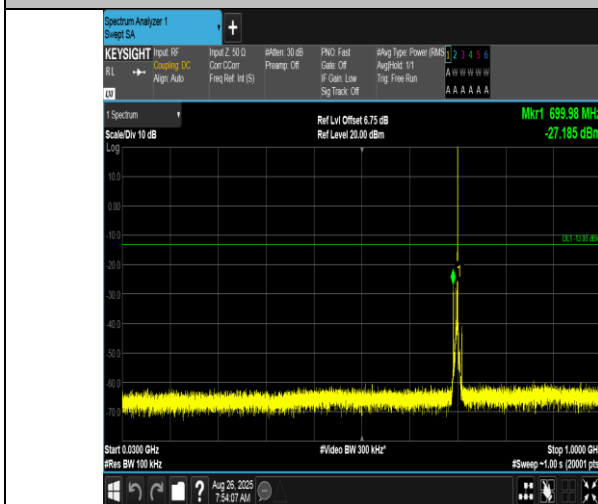
Band17-5MHz-16QAM-23755-1RB#24-30~1000-PASS
