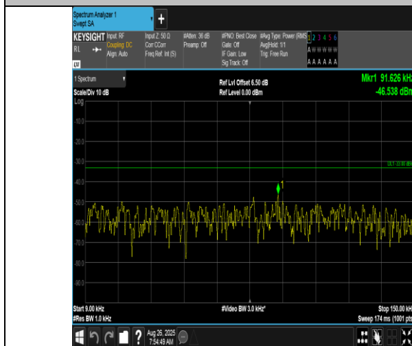
Band17-5MHz-QPSK-23755-25RB#0-0.009~0.15-PASS
