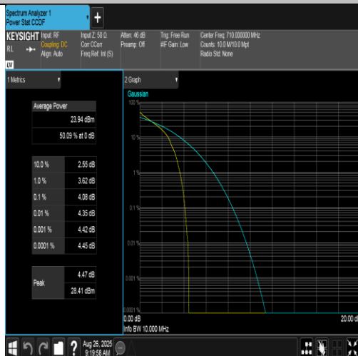
Band17-10MHz-QPSK-23790-1RB#0-PASS
