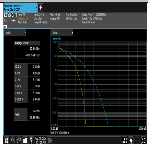
Band17-10MHz-QPSK-23800-50RB#0-PASS
