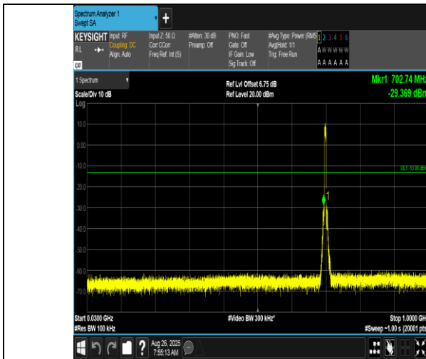
Band17-5MHz-QPSK-23755-25RB#0-30~1000-PASS
