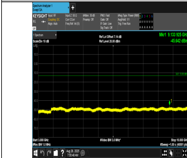
Band17-5MHz-QPSK-23755-25RB#0-3000~10000-PASS
