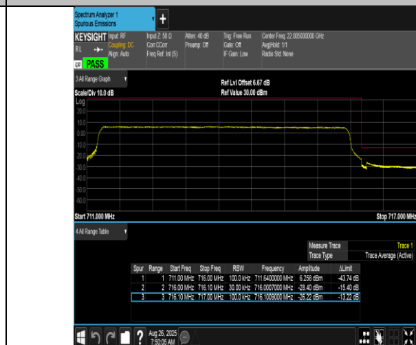
Band17-5MHz-16QAM-23825-25RB#0-PASS
