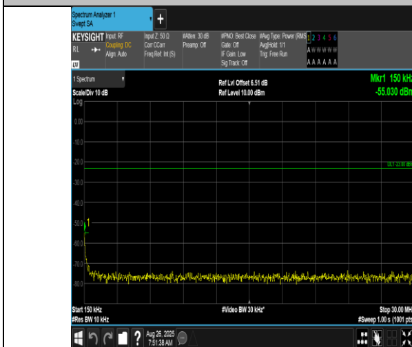
Band17-5MHz-16QAM-23755-1RB#0-0.15~30-PASS
