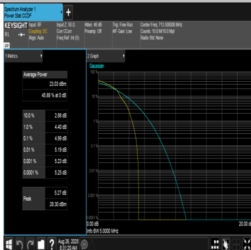
Band17-5MHz-16QAM-23825-1RB#0-PASS
