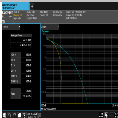
Band17-10MHz-QPSK-23800-1RB#0-PASS
