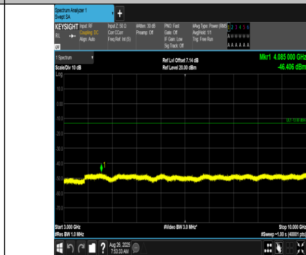
Band17-5MHz-QPSK-23755-1RB#24-3000~10000-PASS
