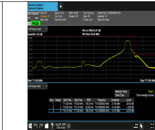
Band17-5MHz-QPSK-23825-1RB#24-PASS
