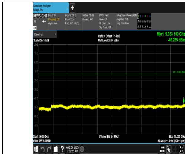
Band17-5MHz-16QAM-23755-1RB#0-3000~10000-PASS
