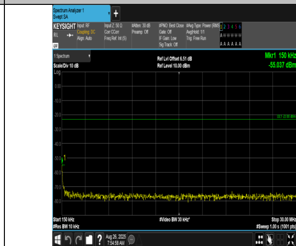
Band17-5MHz-QPSK-23755-25RB#0-0.15~30-PASS
