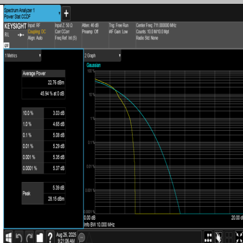
Band17-10MHz-16QAM-23800-1RB#0-PASS
