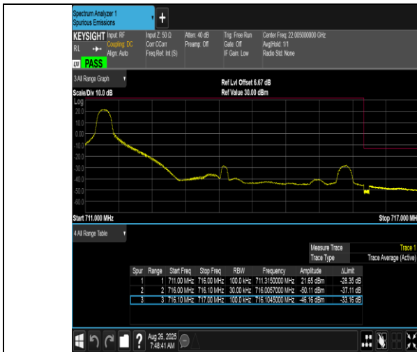
Band17-5MHz-QPSK-23825-1RB#0-PASS
