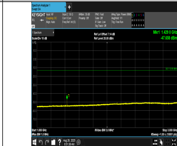
Band17-10MHz-16QAM-23790-1RB#49-1000~3000-PASS
