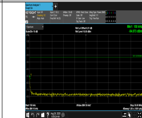
Band17-10MHz-QPSK-23800-50RB#0-0.15~30-PASS
