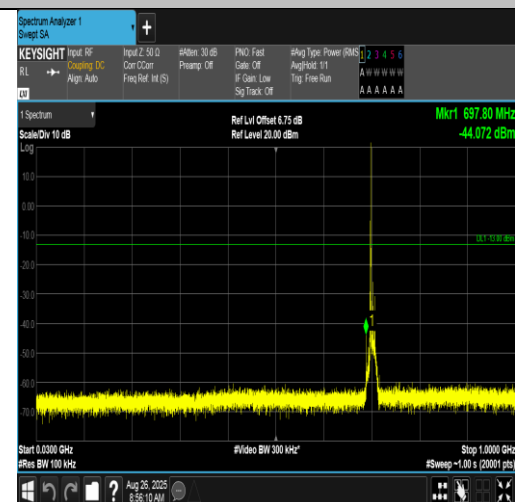
Band17-10MHz-16QAM-23800-1RB#0-30~1000-PASS
