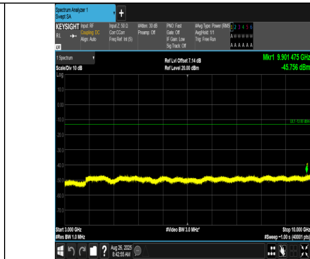
Band17-10MHz-16QAM-23780-1RB#0-3000~10000-PASS
