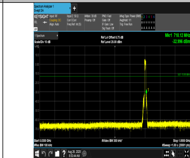
Band17-10MHz-16QAM-23790-50RB#0-30~1000-PASS
