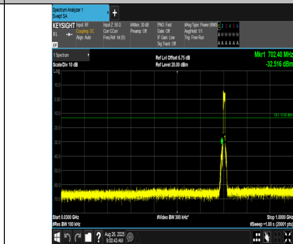
Band17-10MHz-16QAM-23800-50RB#0-30~1000-PASS
