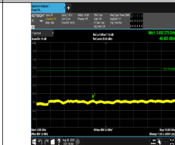
Band17-10MHz-16QAM-23800-50RB#0-3000~10000-PASS
