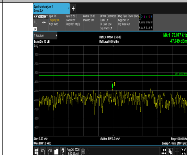
Band17-10MHz-QPSK-23790-1RB#49-0.009~0.15-PASS
