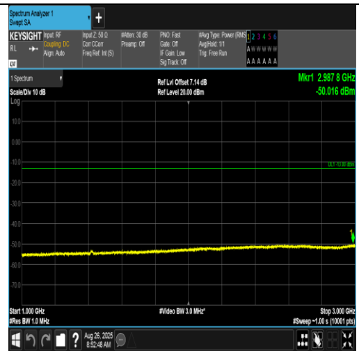
Band17-10MHz-QPSK-23790-50RB#0-1000~3000-PASS
