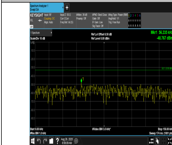
Band17-10MHz-16QAM-23800-1RB#49-0.009~0.15-PASS
