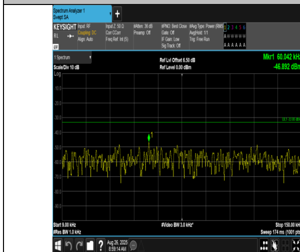
Band17-10MHz-QPSK-23800-50RB#0-0.009~0.15-PASS
