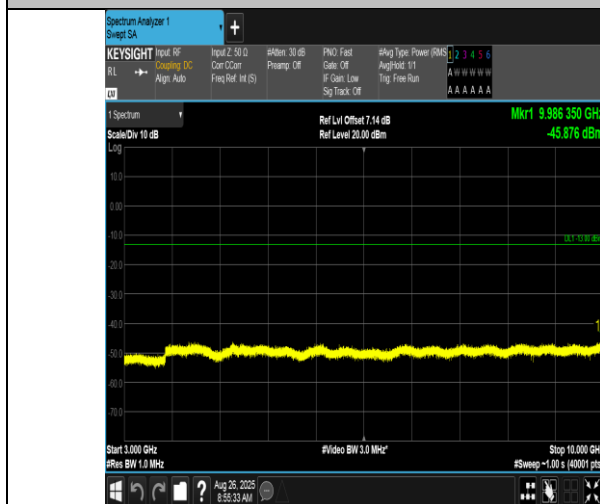
Band17-10MHz-QPSK-23800-1RB#0-3000~10000-PASS
