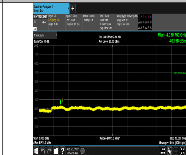
Band17-10MHz-16QAM-23790-50RB#0-3000~10000-PASS
