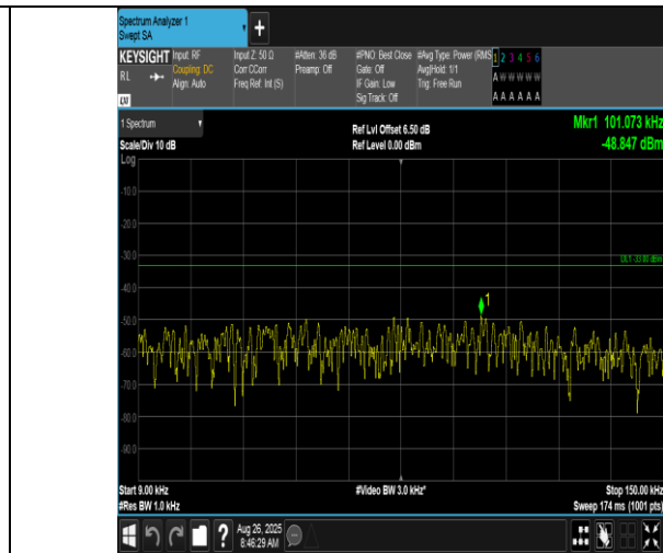
Band17-10MHz-16QAM-23780-50RB#0-0.009~0.15-PASS
