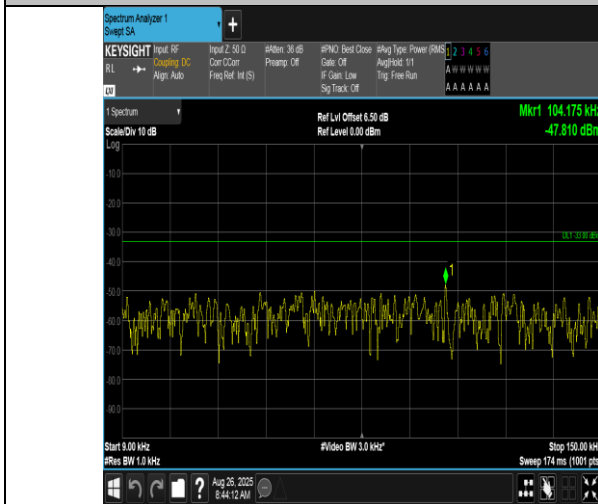
Band17-10MHz-16QAM-23780-1RB#49-0.009~0.15-PASS
