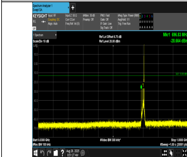
Band17-10MHz-16QAM-23790-1RB#49-30~1000-PASS
