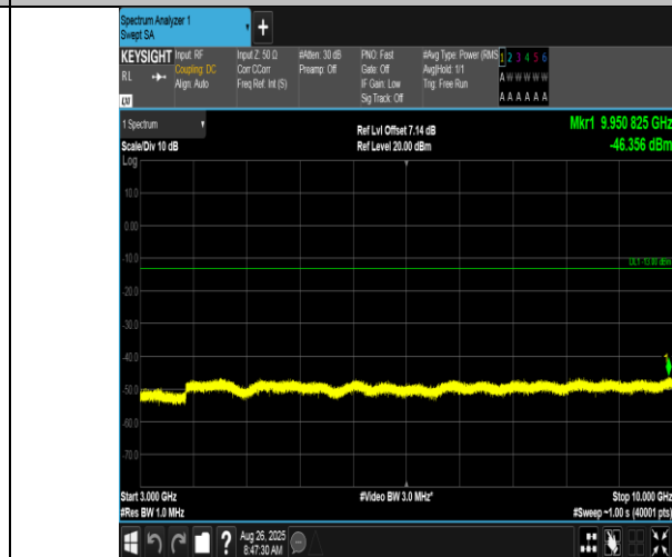
Band17-10MHz-16QAM-23780-50RB#0-3000~10000-PASS
