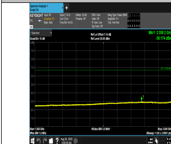
Band17-10MHz-16QAM-23800-50RB#0-1000~3000-PASS
