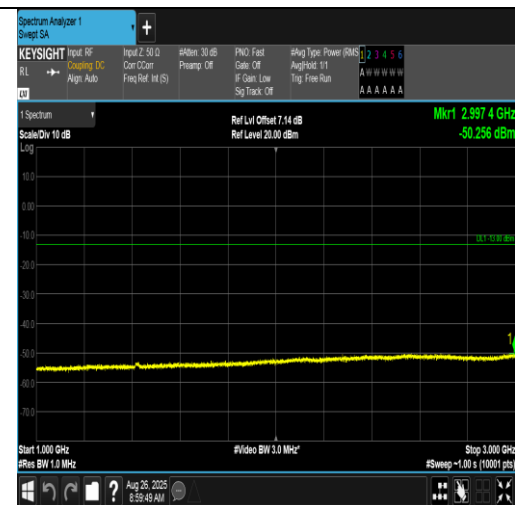
Band17-10MHz-QPSK-23800-50RB#0-1000~3000-PASS
