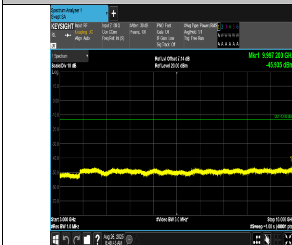
Band17-10MHz-QPSK-23790-1RB#0-3000~10000-PASS
