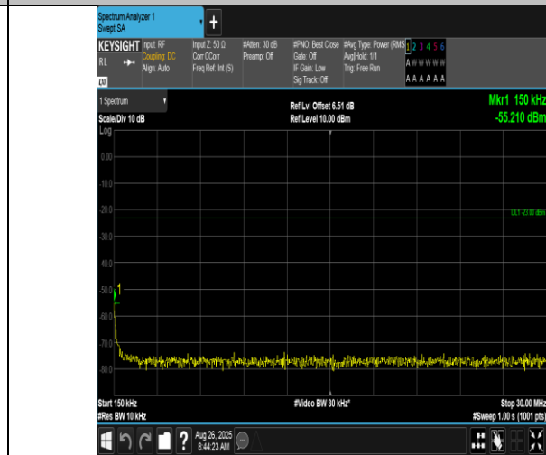
Band17-10MHz-16QAM-23780-1RB#49-0.15~30-PASS
