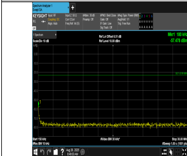
Band17-10MHz-16QAM-23790-1RB#0-0.15~30-PASS
