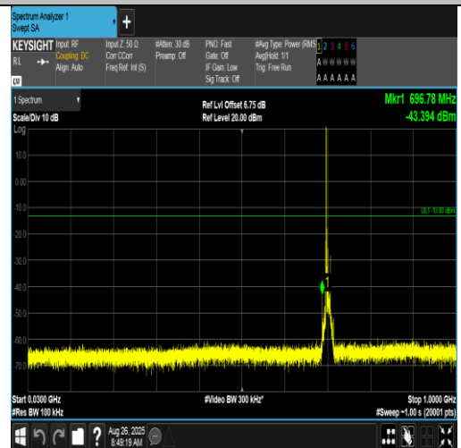
Band17-10MHz-16QAM-23790-1RB#0-30~1000-PASS
