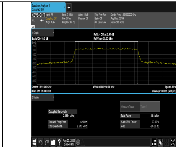
Band2-3MHz-16QAM-18615-15RB#0-PASS
