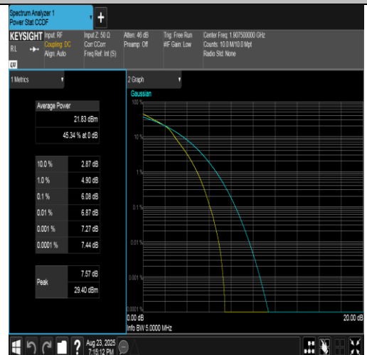
Band2-5MHz-16QAM-19175-25RB#0-PASS
