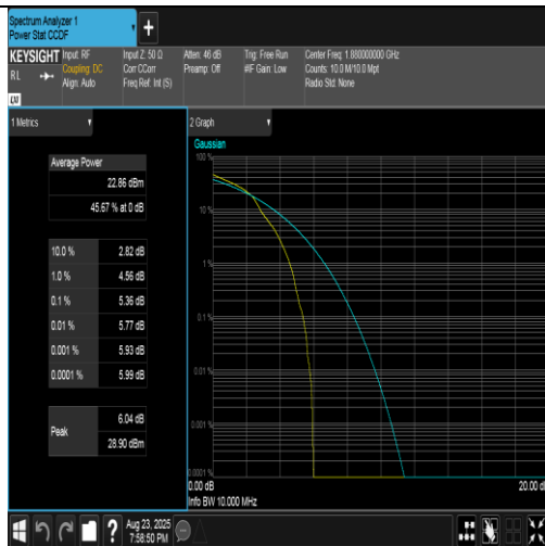
Band2-10MHz-16QAM-18900-1RB#0-PASS
