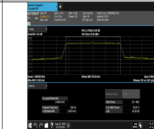
Band2-3MHz-16QAM-18900-15RB#0-PASS
