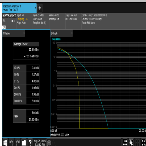
Band2-15MHz-16QAM-19125-1RB#0-PASS
