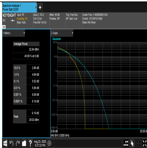
Band2-3MHz-16QAM-18900-1RB#0-PASS
