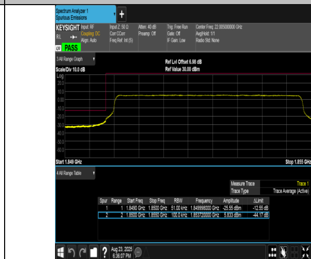
Band2-5MHz-16QAM-18625-25RB#0-PASS
