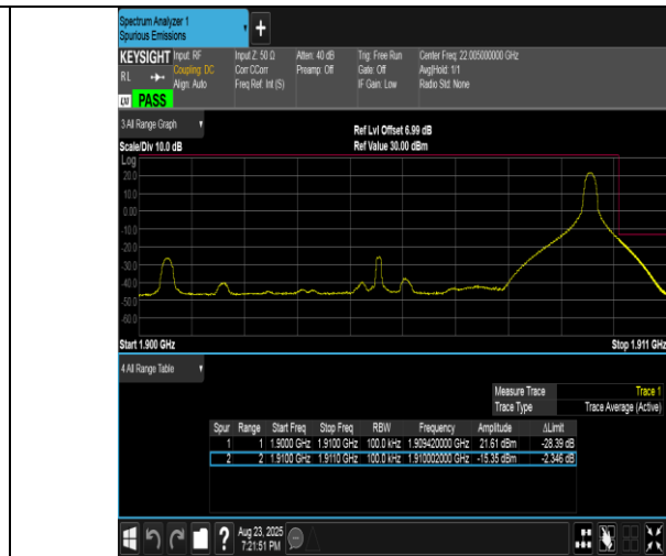
Band2-10MHz-QPSK-19150-1RB#49-PASS
