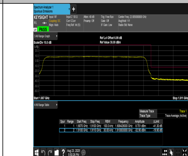
Band2-3MHz-16QAM-19185-15RB#0-PASS
