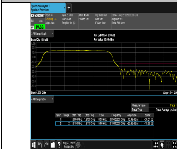
Band2-1.4MHz-QPSK-19193-6RB#0-PASS
