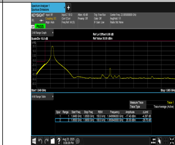
Band2-15MHz-16QAM-18675-1RB#0-PASS
