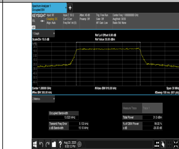
Band2-15MHz-16QAM-18900-75RB#0-PASS
