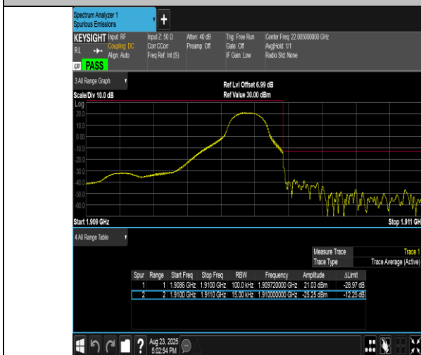
Band2-1.4MHz-16QAM-19193-1RB#5-PASS
