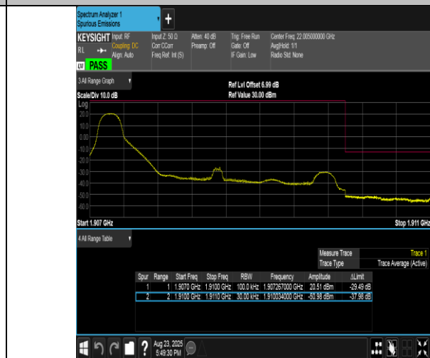
Band2-3MHz-16QAM-19185-1RB#0-PASS
