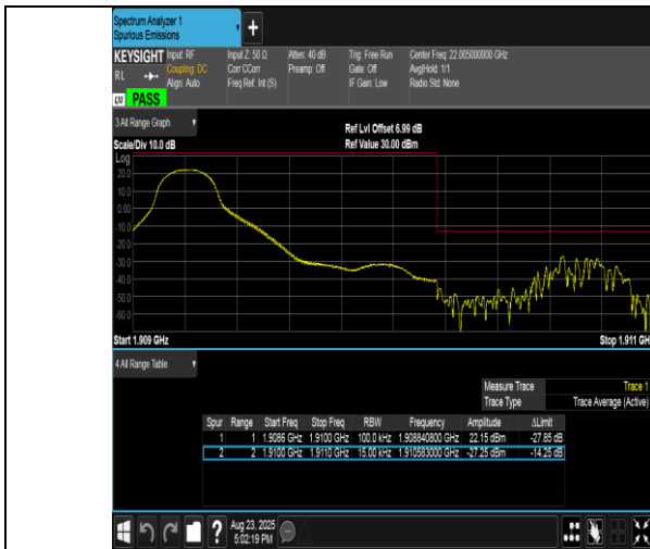
Band2-1.4MHz-QPSK-19193-1RB#0-PASS
