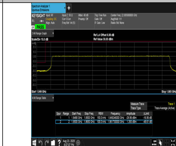
Band2-15MHz-16QAM-18675-75RB#0-PASS
