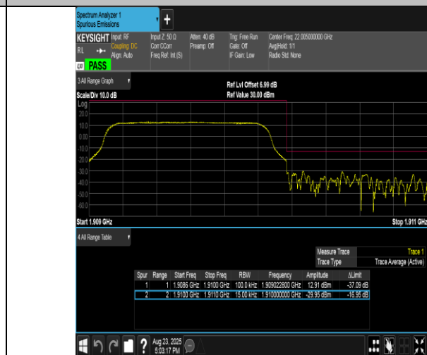
Band2-1.4MHz-16QAM-19193-6RB#0-PASS
