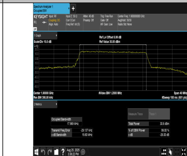
Band2-20MHz-16QAM-19100-100RB#0-PASS
