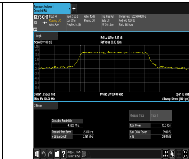
Band2-5MHz-16QAM-18625-25RB#0-PASS
