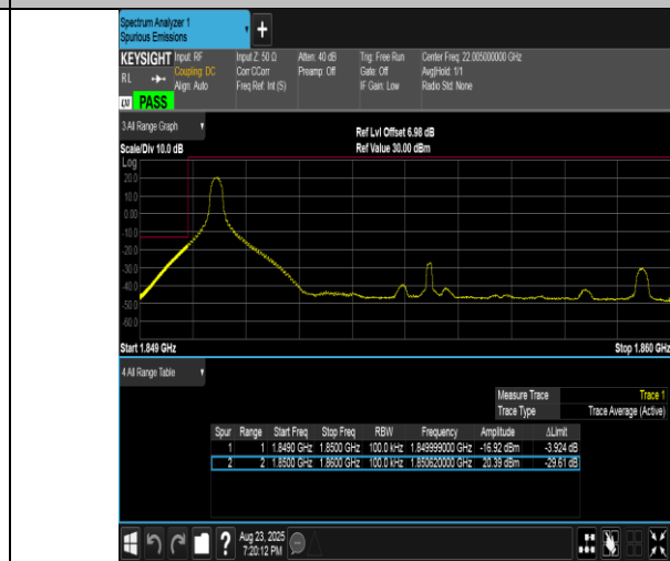
Band2-10MHz-16QAM-18650-1RB#0-PASS
