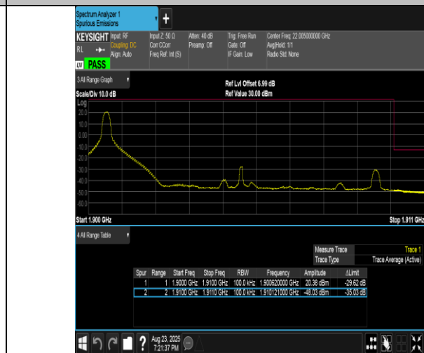
Band2-10MHz-16QAM-19150-1RB#0-PASS
