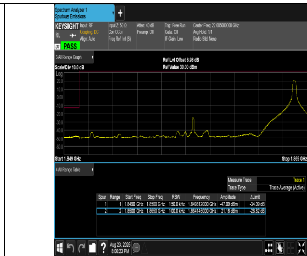
Band2-15MHz-QPSK-18675-1RB#74-PASS
