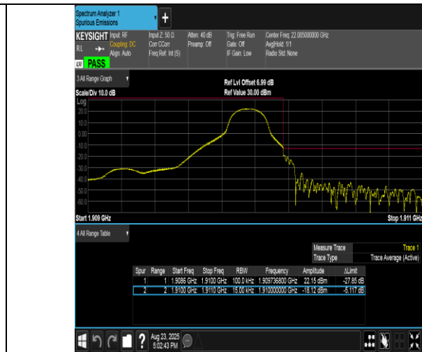
Band2-1.4MHz-QPSK-19193-1RB#5-PASS
