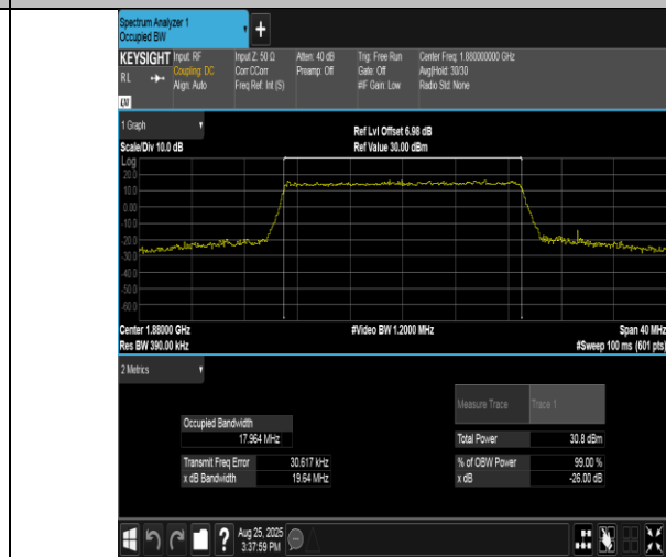
Band2-20MHz-16QAM-18900-100RB#0-PASS
