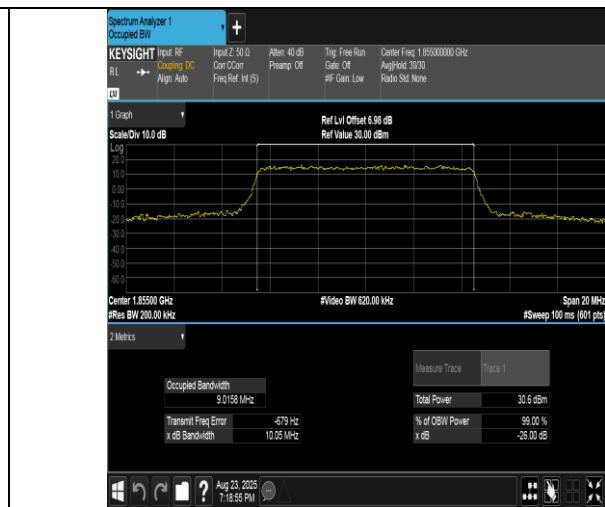
Band2-10MHz-16QAM-18650-50RB#0-PASS
