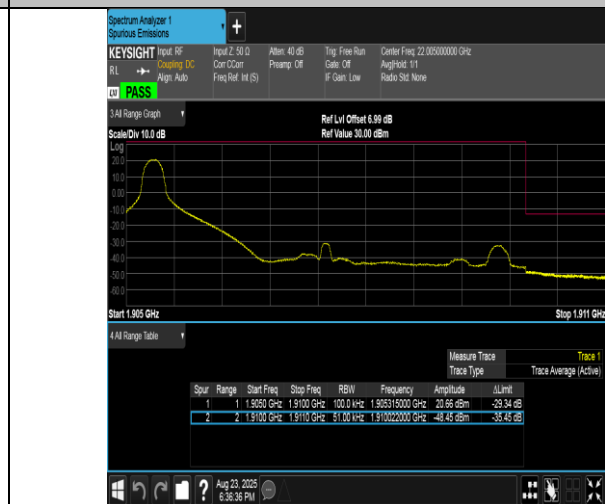
Band2-5MHz-16QAM-19175-1RB#0-PASS
