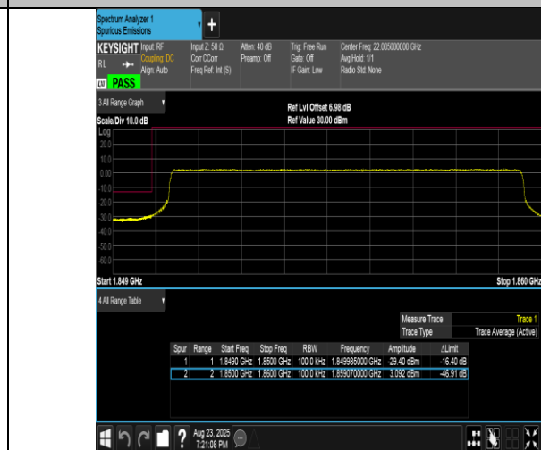
Band2-10MHz-16QAM-18650-50RB#0-PASS
