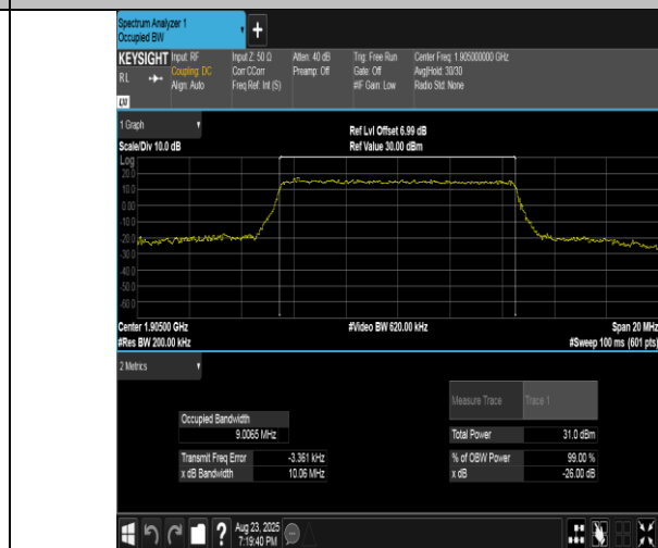
Band2-10MHz-16QAM-19150-50RB#0-PASS
