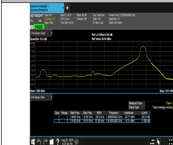
Band2-5MHz-16QAM-19175-1RB#24-PASS
