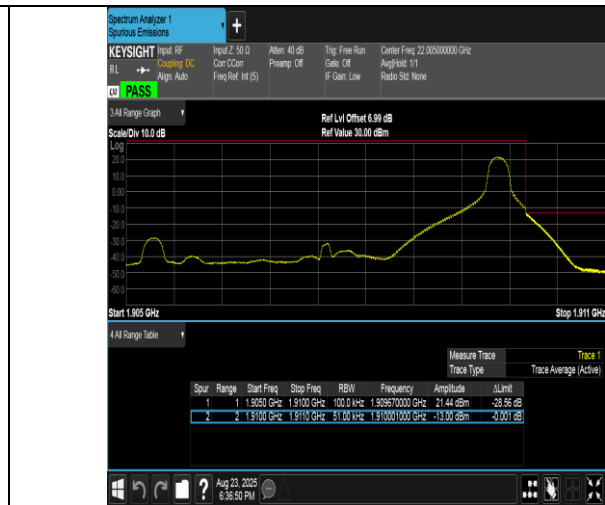
Band2-5MHz-QPSK-19175-1RB#24-PASS
