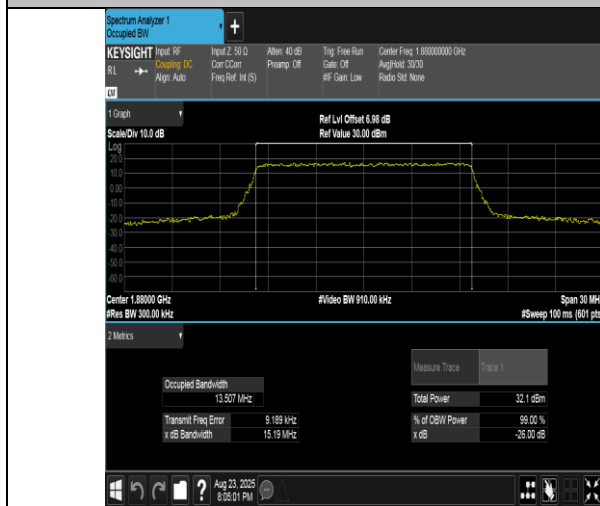
Band2-15MHz-QPSK-18900-75RB#0-PASS
