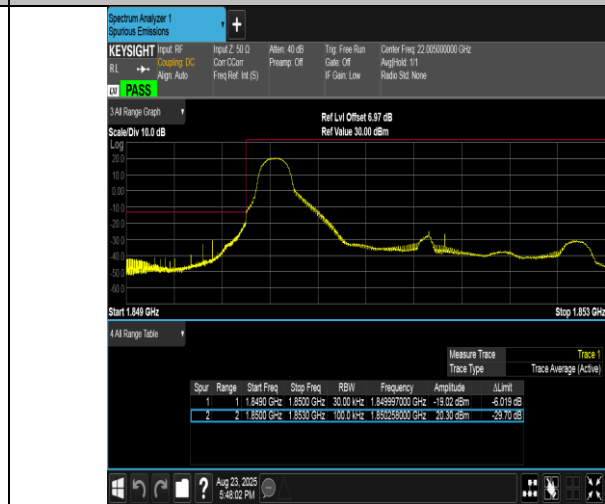
Band2-3MHz-16QAM-18615-1RB#0-PASS
