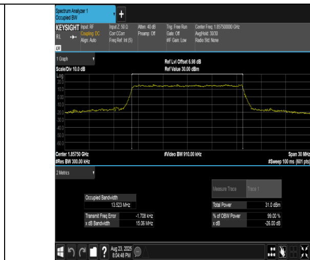
Band2-15MHz-16QAM-18675-75RB#0-PASS
