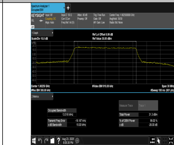
Band2-15MHz-16QAM-19125-75RB#0-PASS
