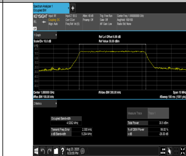
Band2-5MHz-16QAM-18900-25RB#0-PASS
