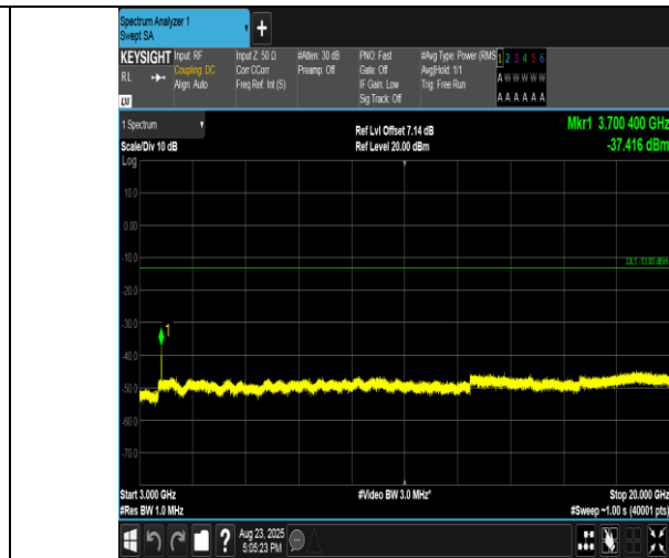
Band2-1.4MHz-16QAM-18607-1RB#0-3000~20000-PASS
