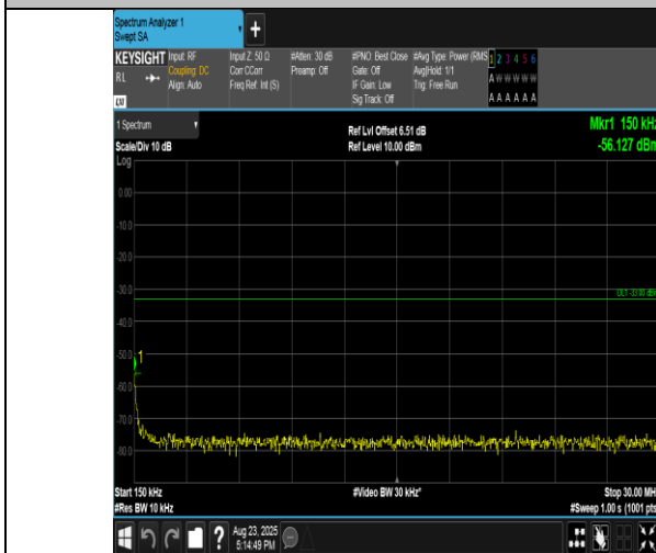
Band2-1.4MHz-16QAM-18900-6RB#0-0.15~30-PASS
