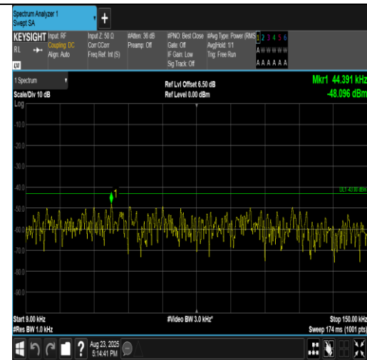
Band2-1.4MHz-16QAM-18900-6RB#0-0.009~0.15-PASS
