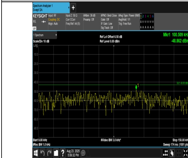
Band2-1.4MHz-16QAM-18607-1RB#5-0.009~0.15-PASS
