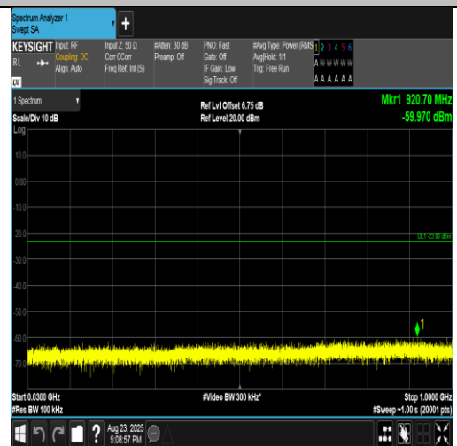
Band2-1.4MHz-16QAM-18607-6RB#0-30~1000-PASS
