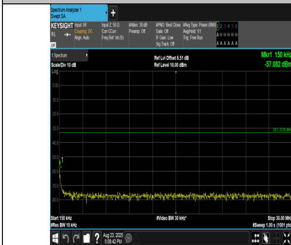
Band2-1.4MHz-16QAM-18607-6RB#0-0.15~30-PASS
