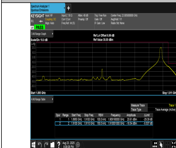
Band2-15MHz-16QAM-19125-1RB#74-PASS
