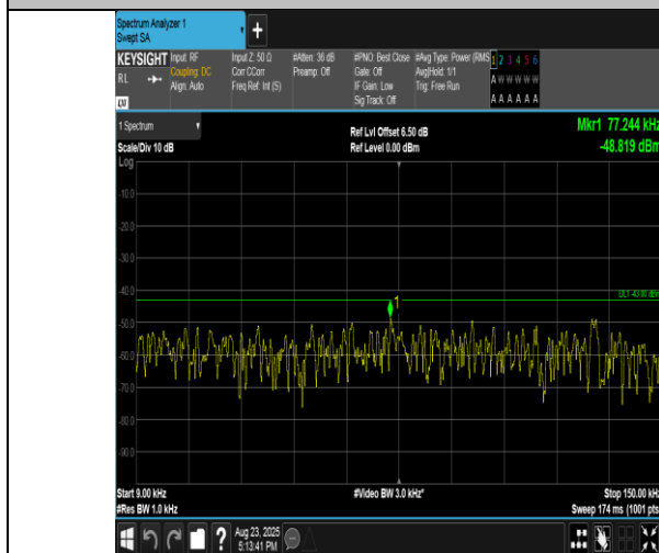
Band2-1.4MHz-QPSK-18900-6RB#0-0.009~0.15-PASS
