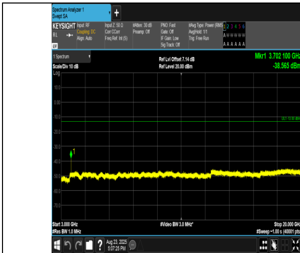
Band2-1.4MHz-16QAM-18607-1RB#5-3000~20000-PASS
