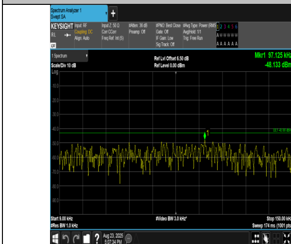
Band2-1.4MHz-QPSK-18607-6RB#0-0.009~0.15-PASS
