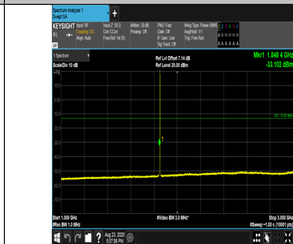
Band2-1.4MHz-16QAM-18607-1RB#5-1000~3000-PASS
