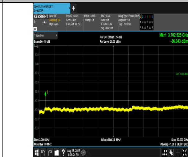
Band2-1.4MHz-QPSK-18607-1RB#5-3000~20000-PASS
