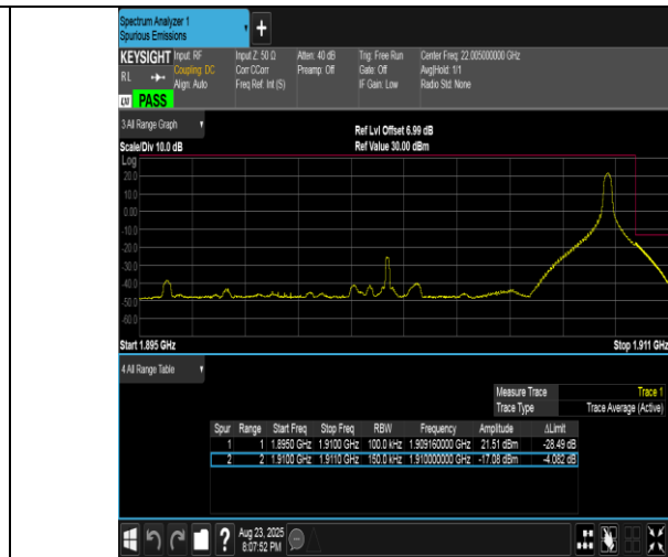
Band2-15MHz-QPSK-19125-1RB#74-PASS
