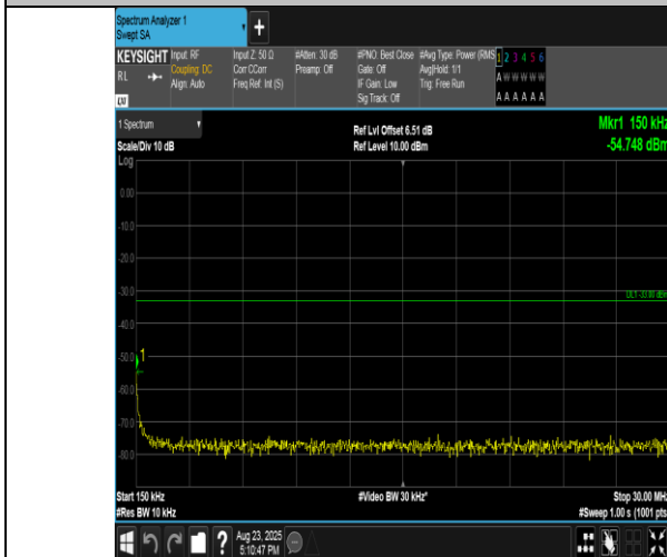
Band2-1.4MHz-16QAM-18900-1RB#0-0.15~30-PASS
