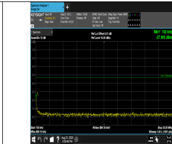
Band2-1.4MHz-QPSK-18900-1RB#0-0.15~30-PASS
