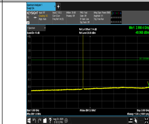
Band2-1.4MHz-QPSK-18900-1RB#0-1000~3000-PASS
