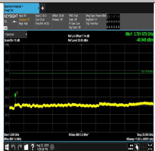
Band2-1.4MHz-16QAM-18607-6RB#0-3000~20000-PASS
