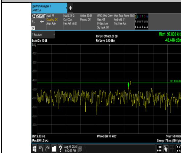
Band2-1.4MHz-16QAM-18900-1RB#5-0.009~0.15-PASS
