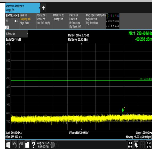
Band2-1.4MHz-16QAM-18900-6RB#0-30~1000-PASS
