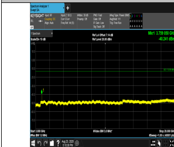
Band2-1.4MHz-QPSK-18900-1RB#0-3000~20000-PASS
