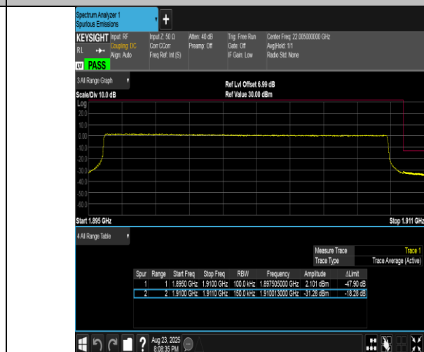
Band2-15MHz-16QAM-19125-75RB#0-PASS
