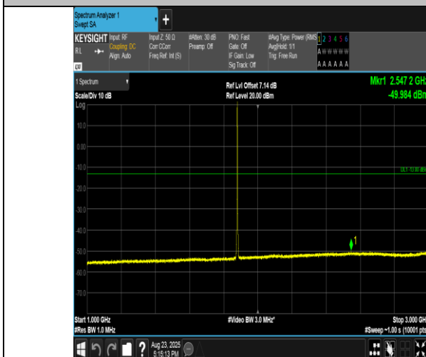
Band2-1.4MHz-16QAM-18900-6RB#0-1000~3000-PASS
