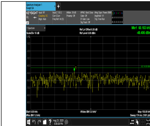
Band2-1.4MHz-QPSK-18900-1RB#0-0.009~0.15-PASS
