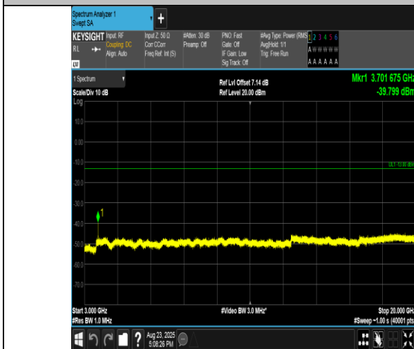
Band2-1.4MHz-QPSK-18607-6RB#0-3000~20000-PASS
