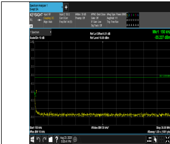
Band2-1.4MHz-QPSK-18607-1RB#5-0.15~30-PASS
