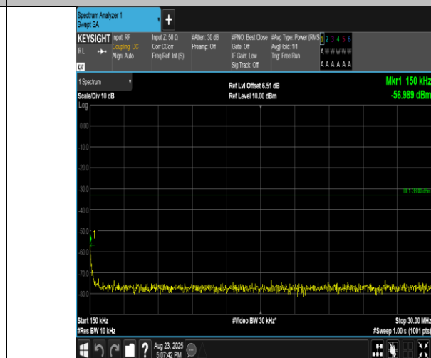
Band2-1.4MHz-QPSK-18607-6RB#0-0.15~30-PASS
