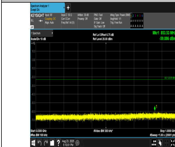
Band2-1.4MHz-QPSK-18900-1RB#0-30~1000-PASS
