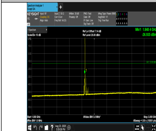
Band2-1.4MHz-16QAM-18607-6RB#0-1000~3000-PASS
