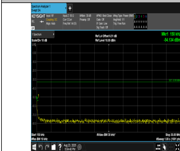
Band2-1.4MHz-16QAM-18607-1RB#0-0.15~30-PASS
