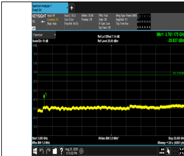
Band2-1.4MHz-16QAM-18900-1RB#5-3000~20000-PASS
