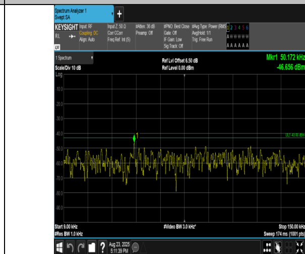
Band2-1.4MHz-QPSK-18900-1RB#5-0.009~0.15-PASS
