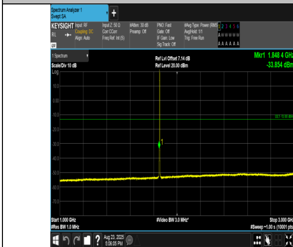
Band2-1.4MHz-QPSK-18607-1RB#5-1000~3000-PASS
