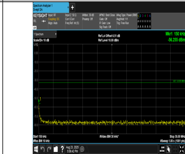
Band2-1.4MHz-16QAM-18607-1RB#5-0.15~30-PASS
