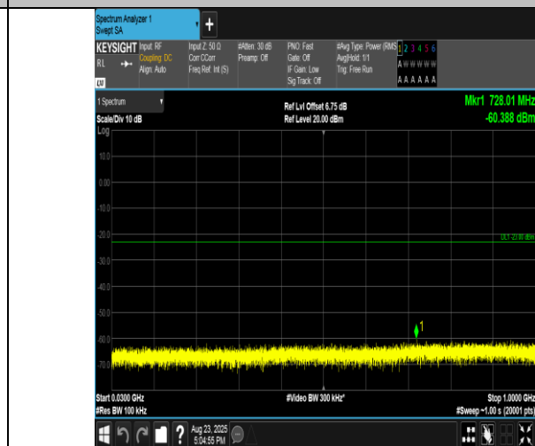
Band2-1.4MHz-16QAM-18607-1RB#0-30~1000-PASS
