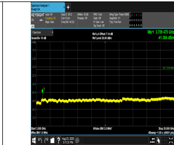
Band2-1.4MHz-16QAM-18900-1RB#0-3000~20000-PASS
