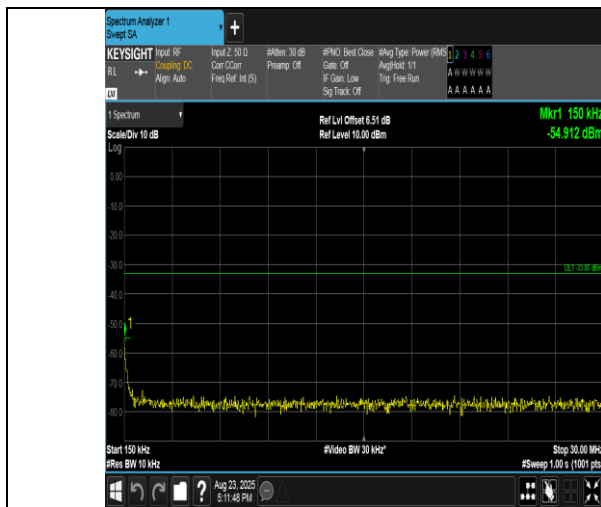
Band2-1.4MHz-QPSK-18900-1RB#5-0.15~30-PASS
