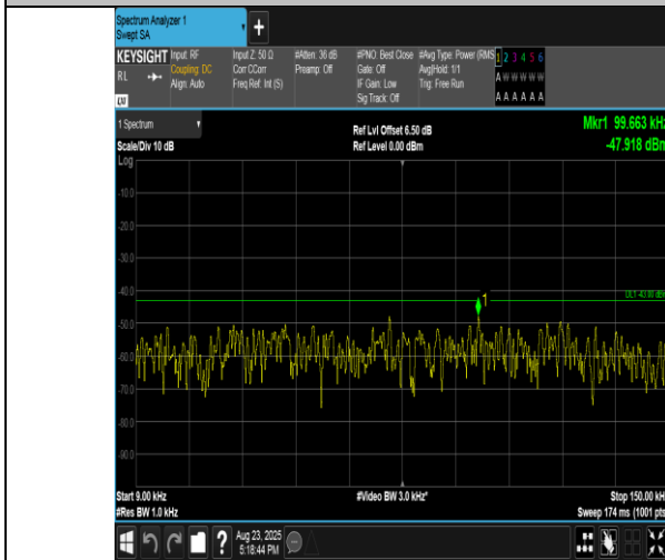
Band2-1.4MHz-16QAM-19193-1RB#5-0.009~0.15-PASS
