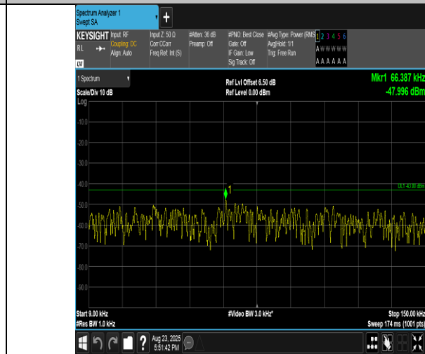
Band2-3MHz-16QAM-18615-1RB#0-0.009~0.15-PASS
