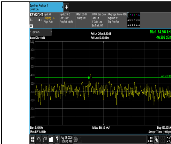
Band2-3MHz-QPSK-18615-1RB#0-0.009~0.15-PASS
