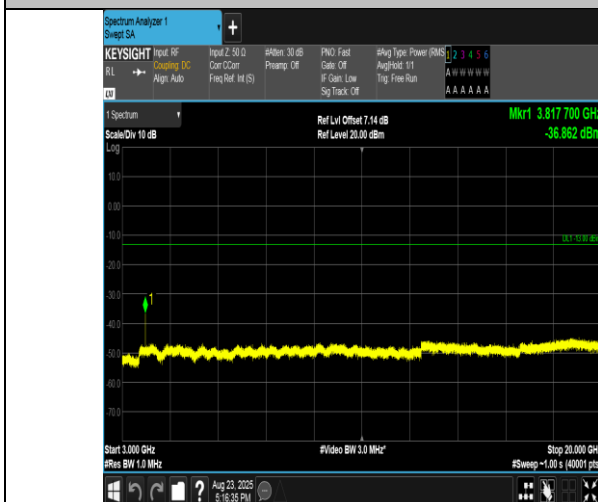
Band2-1.4MHz-QPSK-19193-1RB#0-3000~20000-PASS
