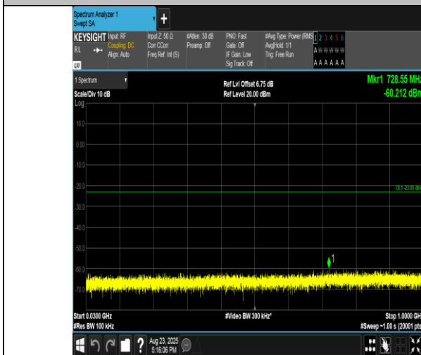
Band2-1.4MHz-QPSK-19193-1RB#0-30~1000-PASS
