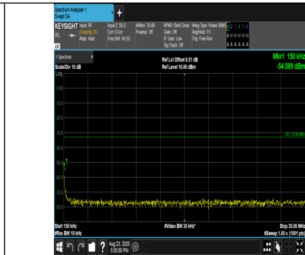
Band2-3MHz-QPSK-18615-1RB#0-0.15~30-PASS
