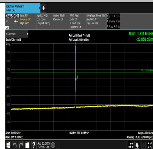
Band2-1.4MHz-16QAM-19193-1RB#5-1000~3000-PASS
