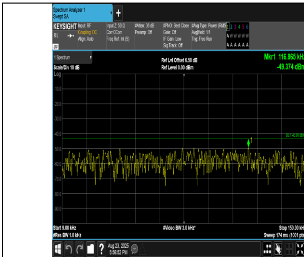
Band2-3MHz-QPSK-18900-1RB#0-0.009~0.15-PASS
