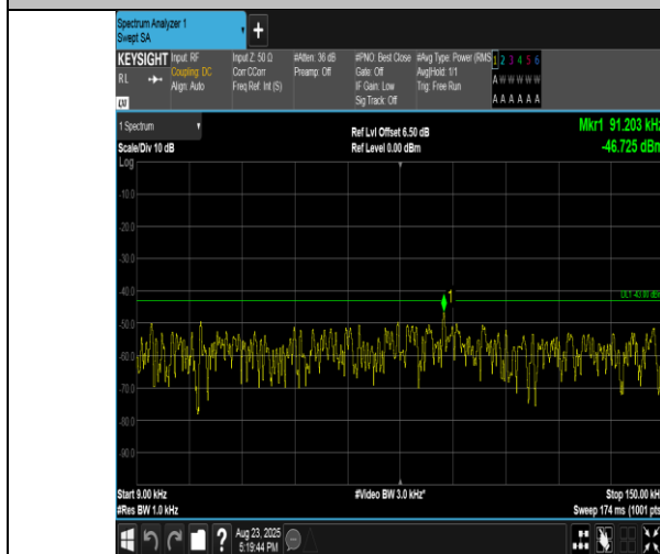
Band2-1.4MHz-QPSK-19193-6RB#0-0.009~0.15-PASS
