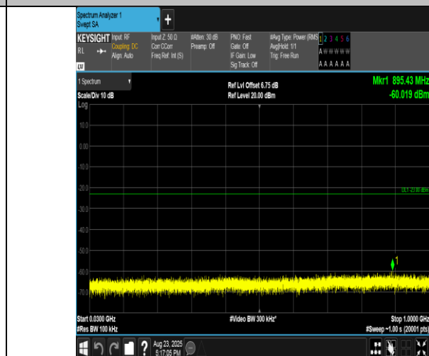
Band2-1.4MHz-16QAM-19193-1RB#0-30~1000-PASS
