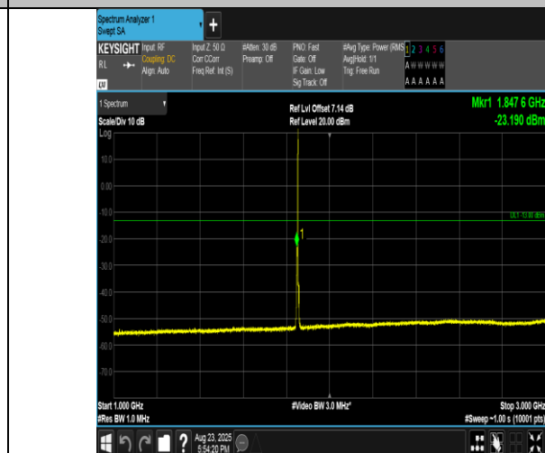
Band2-3MHz-16QAM-18615-1RB#14-1000~3000-PASS
