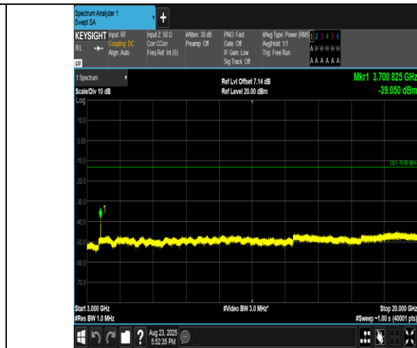
Band2-3MHz-16QAM-18615-1RB#0-3000~20000-PASS
