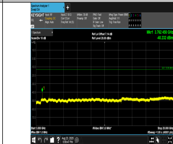
Band2-3MHz-QPSK-18900-1RB#14-3000~20000-PASS
