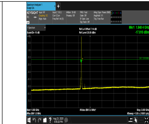
Band2-3MHz-QPSK-18615-15RB#0-1000~3000-PASS
