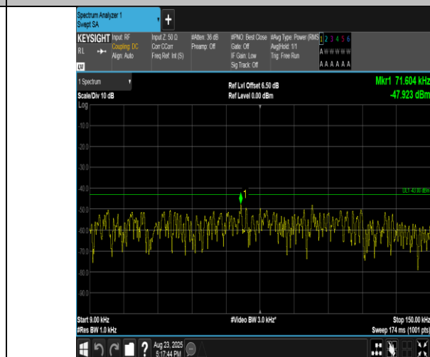
Band2-1.4MHz-QPSK-19193-1RB#5-0.009~0.15-PASS
