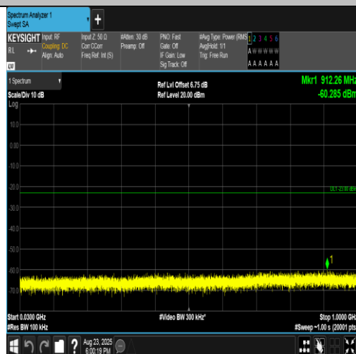
Band2-3MHz-16QAM-18900-1RB#14-30~1000-PASS
