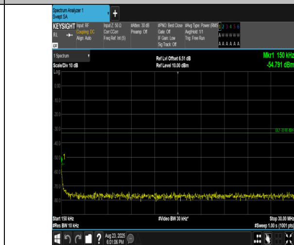
Band2-3MHz-QPSK-18900-15RB#0-0.15~30-PASS
