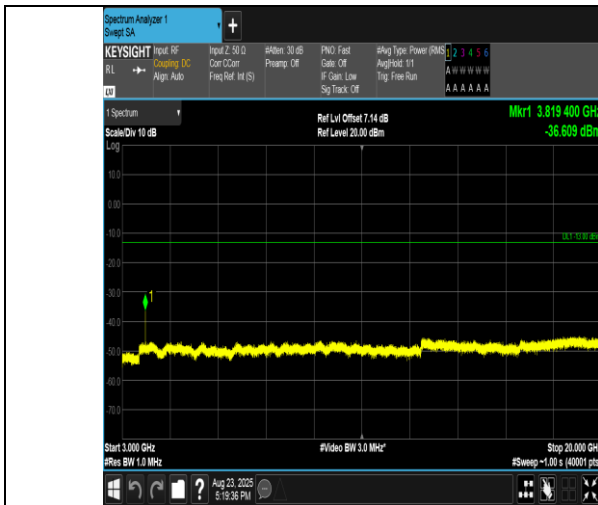
Band2-1.4MHz-16QAM-19193-1RB#5-3000~20000-PASS
