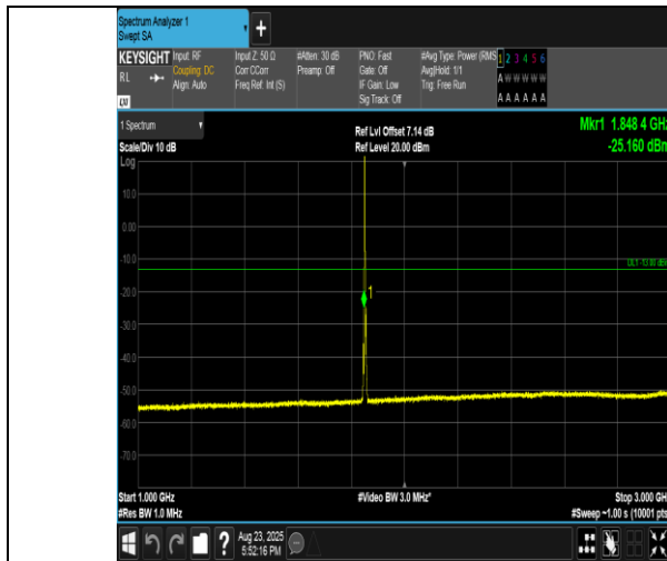
Band2-3MHz-16QAM-18615-1RB#0-1000~3000-PASS
