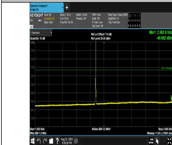
Band2-3MHz-QPSK-18900-1RB#14-1000~3000-PASS
