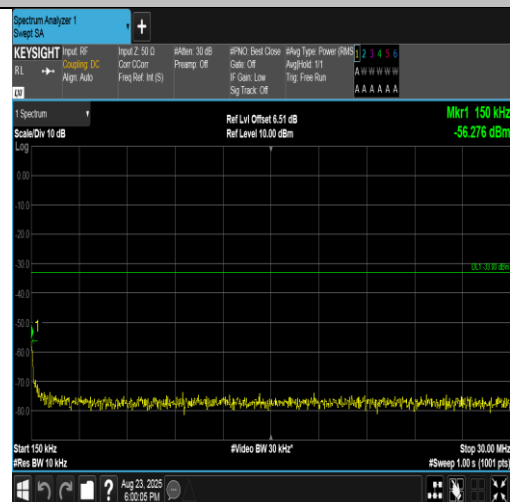
Band2-3MHz-16QAM-18900-1RB#14-0.15~30-PASS
