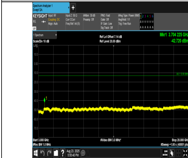
Band2-3MHz-QPSK-18615-15RB#0-3000~20000-PASS
