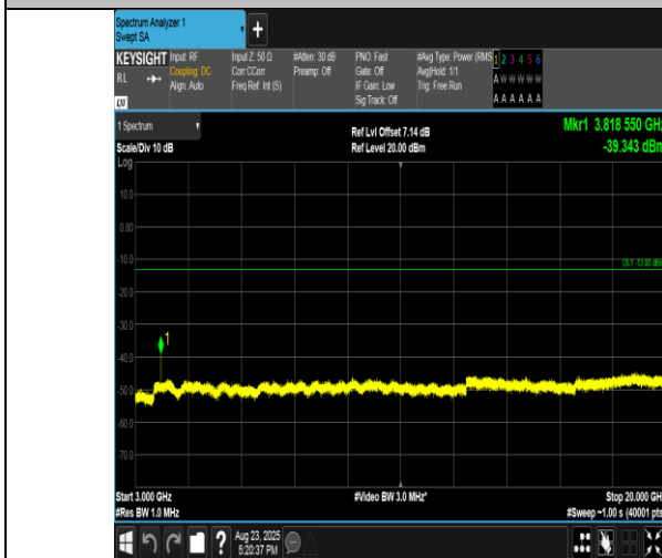
Band2-1.4MHz-QPSK-19193-6RB#0-3000~20000-PASS
