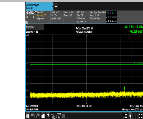
Band2-3MHz-16QAM-18615-1RB#0-30~1000-PASS
