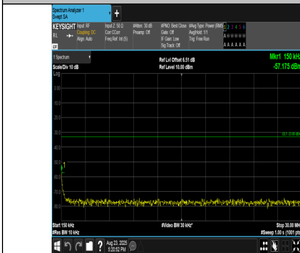
Band2-1.4MHz-16QAM-19193-6RB#0-0.15~30-PASS
