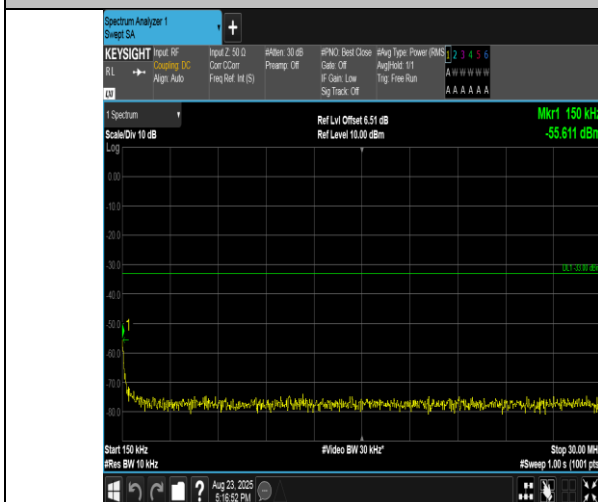
Band2-1.4MHz-16QAM-19193-1RB#0-0.15~30-PASS
