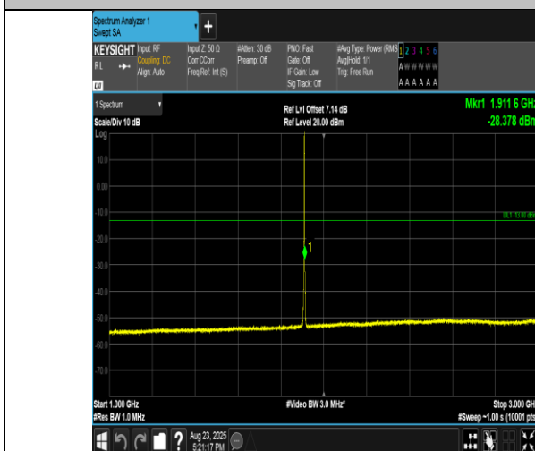
Band2-1.4MHz-16QAM-19193-6RB#0-1000~3000-PASS
