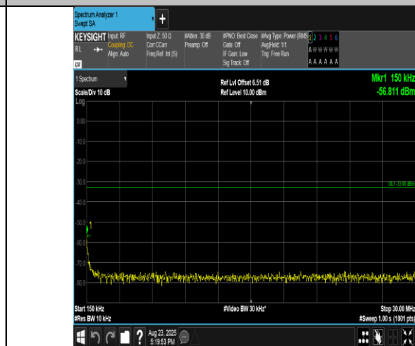
Band2-1.4MHz-QPSK-19193-6RB#0-0.15~30-PASS
