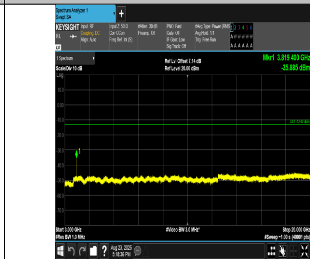
Band2-1.4MHz-QPSK-19193-1RB#5-3000~20000-PASS
