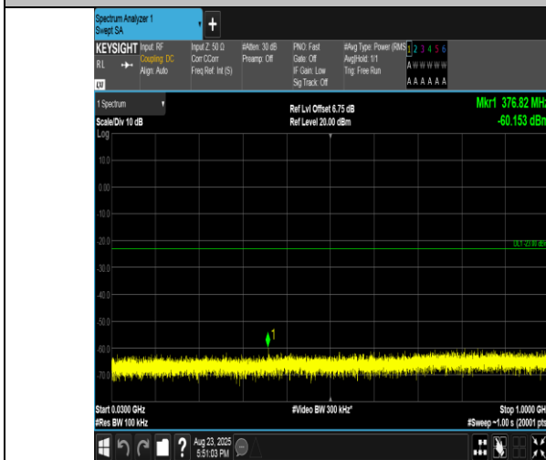
Band2-3MHz-QPSK-18615-1RB#0-30~1000-PASS
