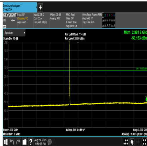
Band2-3MHz-16QAM-18900-1RB#0-1000~3000-PASS
