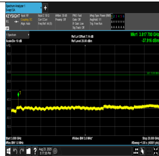
Band2-1.4MHz-16QAM-19193-1RB#0-3000~20000-PASS
