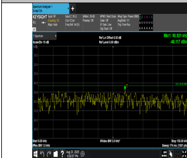
Band2-3MHz-QPSK-18900-15RB#0-0.009~0.15-PASS
