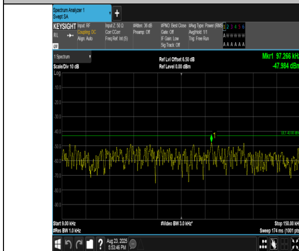
Band2-3MHz-16QAM-18615-1RB#14-0.009~0.15-PASS
