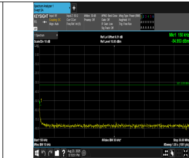
Band2-1.4MHz-QPSK-19193-1RB#0-0.15~30-PASS
