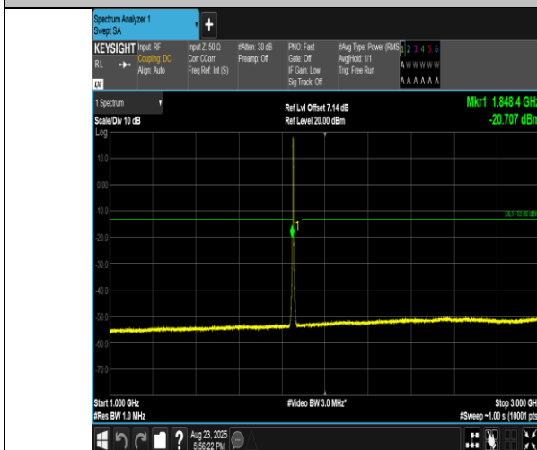
Band2-3MHz-16QAM-18615-15RB#0-1000~3000-PASS
