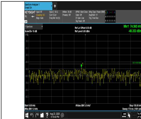
Band2-1.4MHz-QPSK-19193-1RB#0-0.009~0.15-PASS
