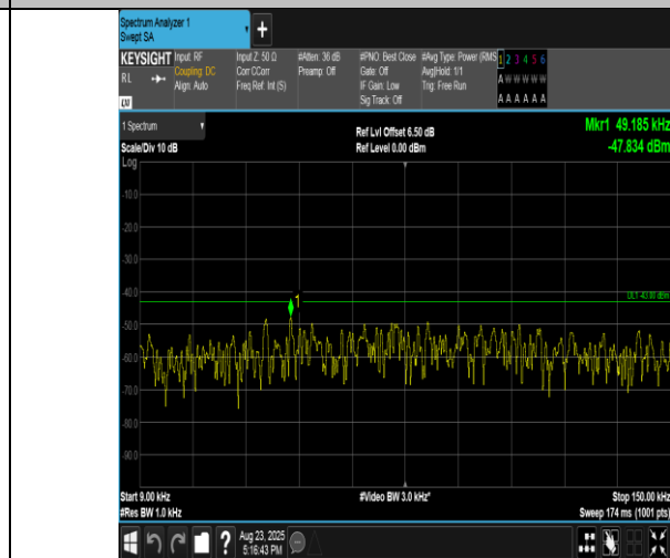
Band2-1.4MHz-16QAM-19193-1RB#0-0.009~0.15-PASS
