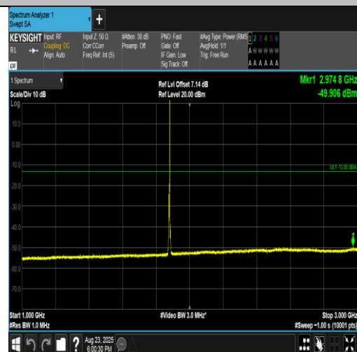
Band2-3MHz-16QAM-18900-1RB#14-1000~3000-PASS
