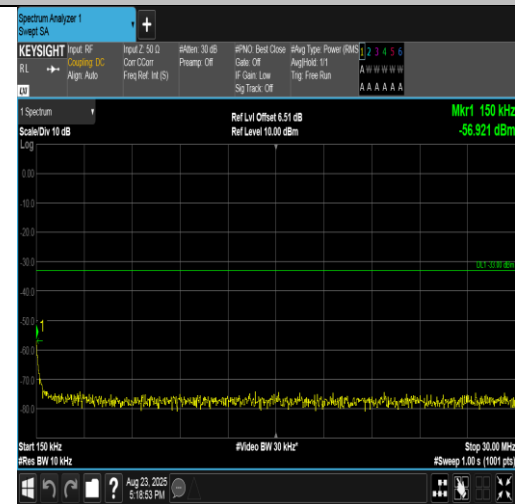
Band2-1.4MHz-16QAM-19193-1RB#5-0.15~30-PASS
