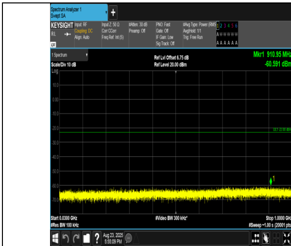
Band2-3MHz-QPSK-18615-15RB#0-30~1000-PASS
