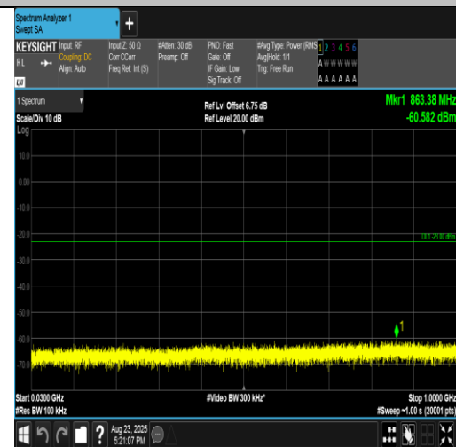
Band2-1.4MHz-16QAM-19193-6RB#0-30~1000-PASS
