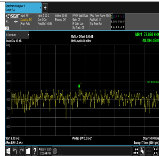
Band2-1.4MHz-16QAM-19193-6RB#0-0.009~0.15-PASS
