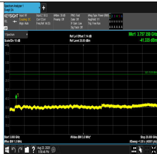
Band2-3MHz-16QAM-18900-1RB#0-3000~20000-PASS
