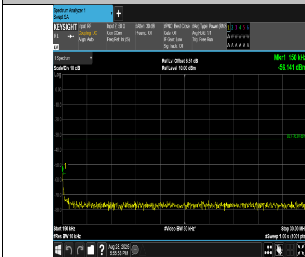
Band2-3MHz-16QAM-18615-15RB#0-0.15~30-PASS
