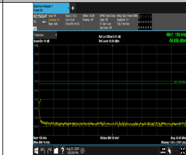
Band2-3MHz-16QAM-18615-1RB#14-0.15~30-PASS
