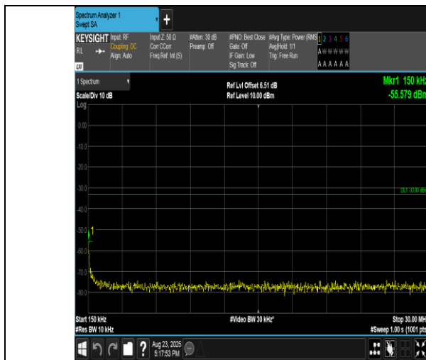
Band2-1.4MHz-QPSK-19193-1RB#5-0.15~30-PASS
