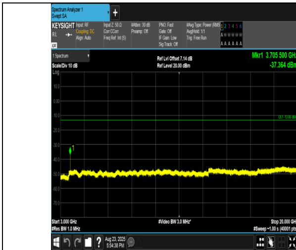
Band2-3MHz-16QAM-18615-1RB#14-3000~20000-PASS
