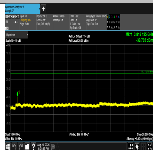
Band2-1.4MHz-16QAM-19193-6RB#0-3000~20000-PASS
