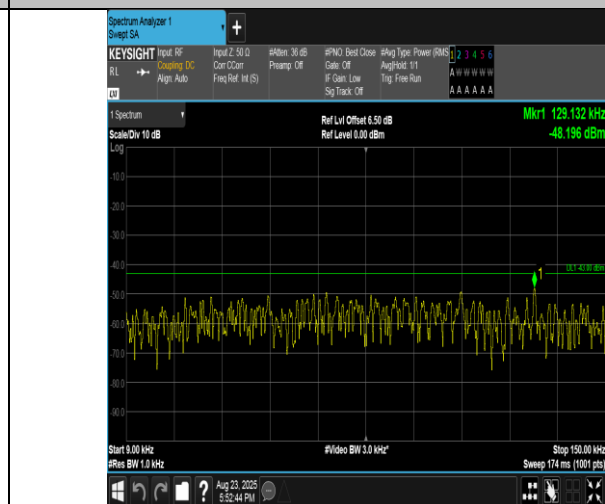
Band2-3MHz-QPSK-18615-1RB#14-0.009~0.15-PASS
