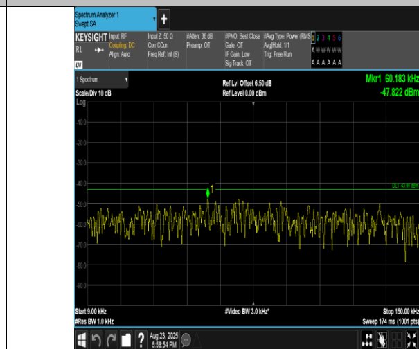
Band2-3MHz-QPSK-18900-1RB#14-0.009~0.15-PASS
