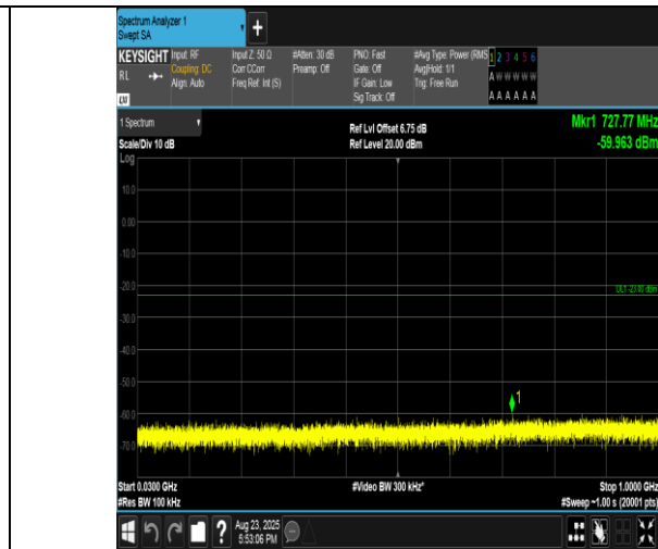
Band2-3MHz-QPSK-18615-1RB#14-30~1000-PASS
