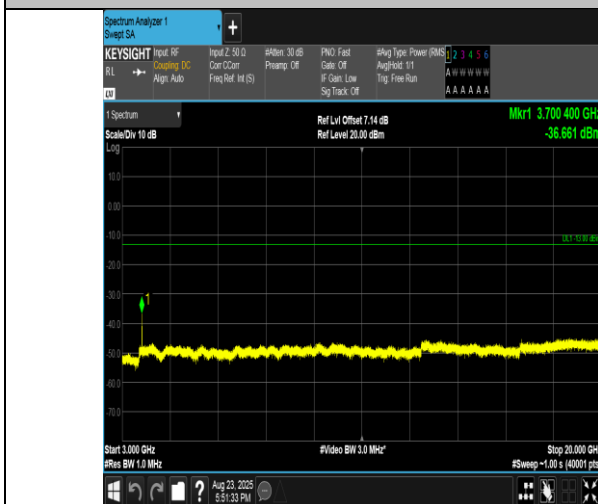
Band2-3MHz-QPSK-18615-1RB#0-3000~20000-PASS
