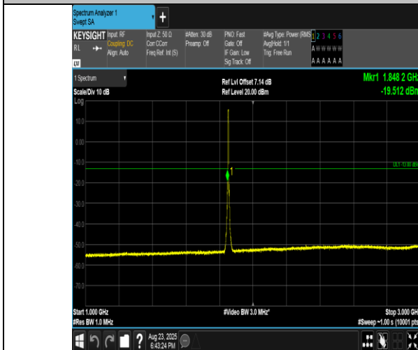
Band2-5MHz-16QAM-18625-25RB#0-1000~3000-PASS
