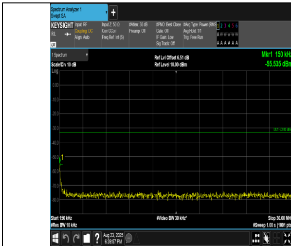
Band2-5MHz-QPSK-18625-1RB#24-0.15~30-PASS
