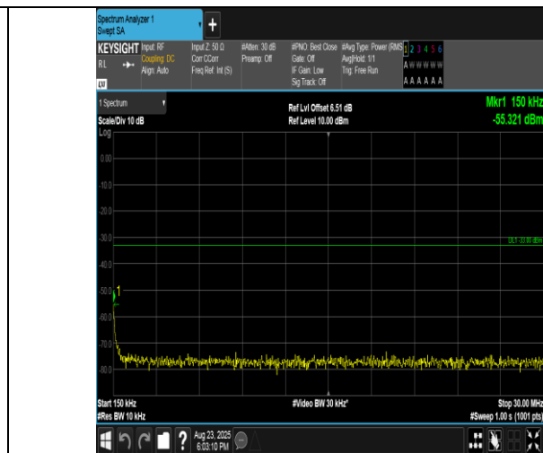
Band2-3MHz-QPSK-19185-1RB#0-0.15~30-PASS
