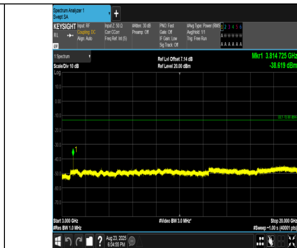
Band2-3MHz-16QAM-19185-1RB#0-3000~20000-PASS
