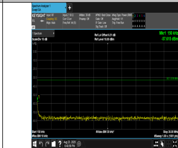
Band2-5MHz-16QAM-18625-1RB#24-0.15~30-PASS
