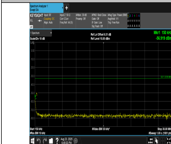
Band2-5MHz-16QAM-18900-1RB#0-0.15~30-PASS
