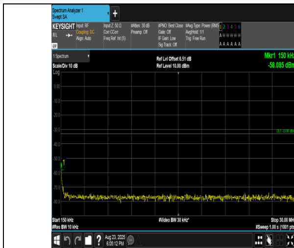
Band2-3MHz-QPSK-19185-1RB#14-0.15~30-PASS
