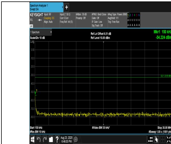
Band2-5MHz-QPSK-18900-1RB#24-0.15~30-PASS
