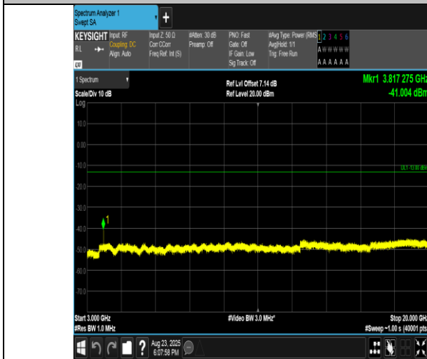
Band2-3MHz-QPSK-19185-15RB#0-3000~20000-PASS
