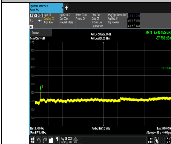
Band2-5MHz-QPSK-18625-1RB#0-3000~20000-PASS
