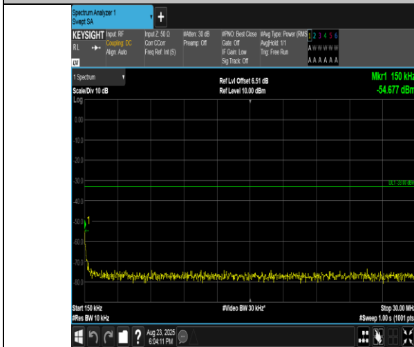
Band2-3MHz-16QAM-19185-1RB#0-0.15~30-PASS
