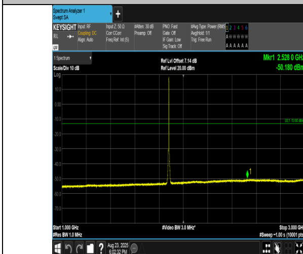
Band2-3MHz-16QAM-18900-15RB#0-1000~3000-PASS
