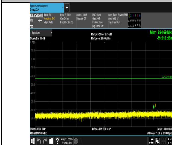
Band2-5MHz-QPSK-18625-1RB#0-30~1000-PASS
