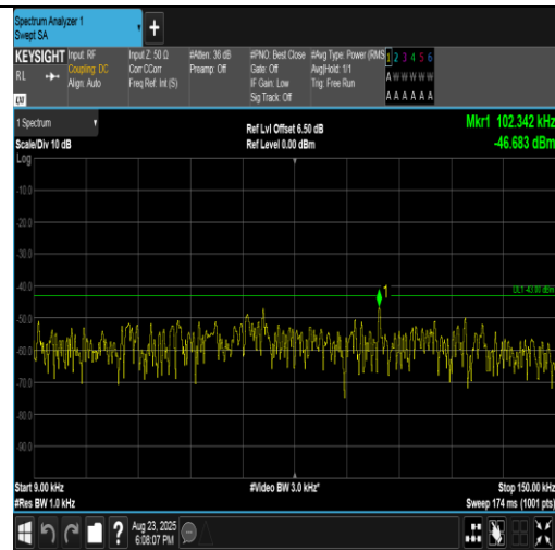
Band2-3MHz-16QAM-19185-15RB#0-0.009~0.15-PASS
