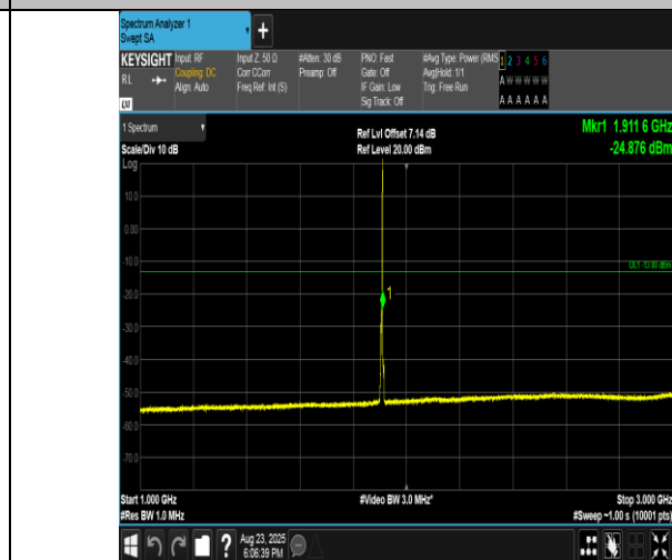
Band2-3MHz-16QAM-19185-1RB#14-1000~3000-PASS
