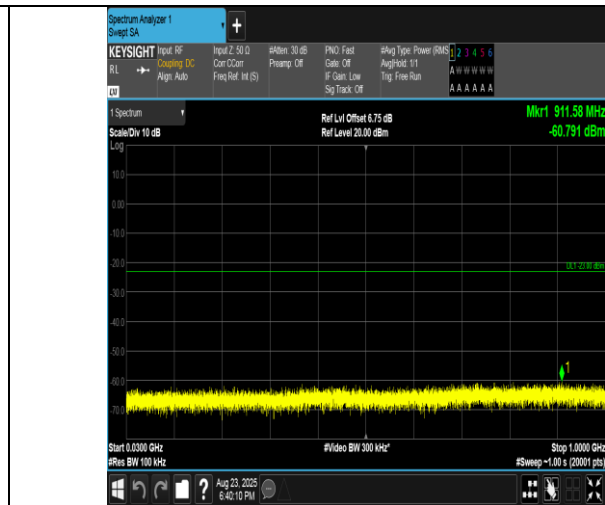
Band2-5MHz-QPSK-18625-1RB#24-30~1000-PASS
