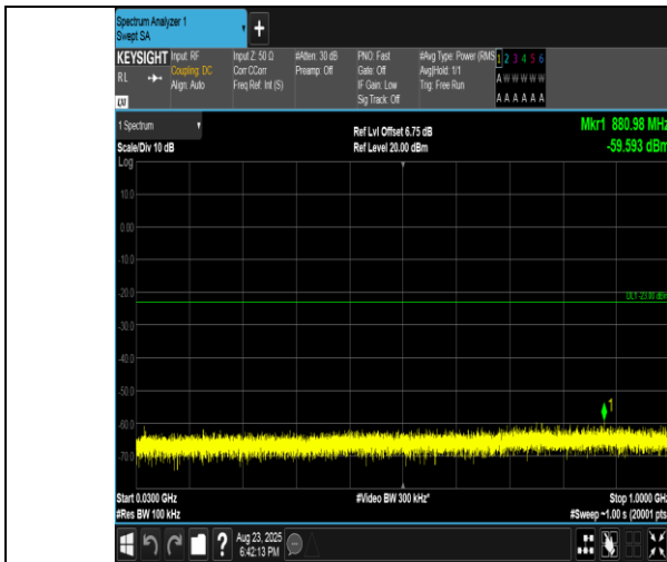
Band2-5MHz-QPSK-18625-25RB#0-30~1000-PASS
