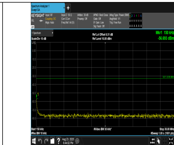
Band2-5MHz-QPSK-18900-1RB#0-0.15~30-PASS
