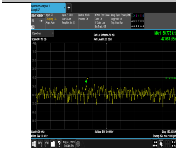
Band2-3MHz-16QAM-19185-1RB#14-0.009~0.15-PASS
