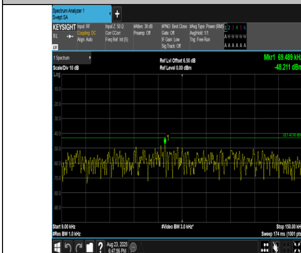
Band2-5MHz-QPSK-18900-25RB#0-0.009~0.15-PASS
