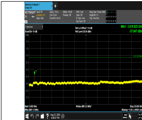
Band2-3MHz-16QAM-19185-1RB#14-3000~20000-PASS
