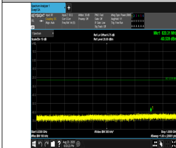
Band2-3MHz-QPSK-19185-1RB#0-30~1000-PASS
