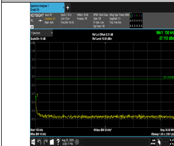
Band2-3MHz-16QAM-19185-15RB#0-0.15~30-PASS
