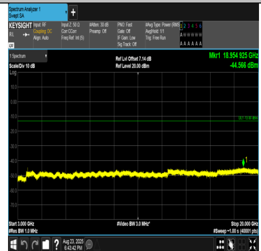
Band2-5MHz-16QAM-18625-25RB#0-3000~20000-PASS
