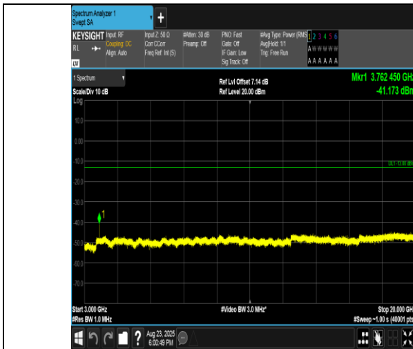
Band2-3MHz-16QAM-18900-1RB#14-3000~20000-PASS
