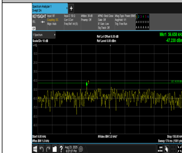
Band2-3MHz-QPSK-19185-15RB#0-0.009~0.15-PASS
