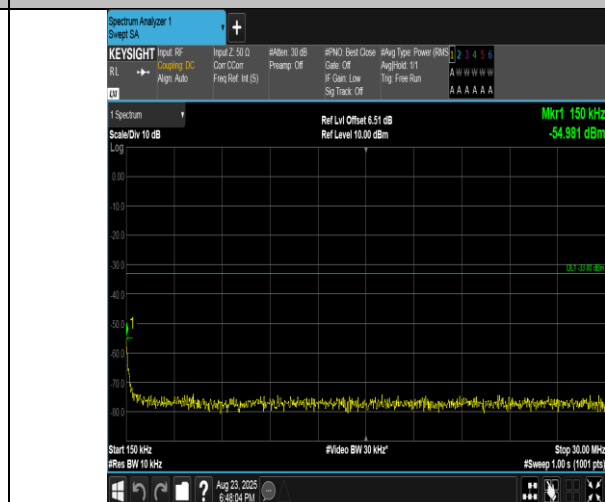
Band2-5MHz-QPSK-18900-25RB#0-0.15~30-PASS
