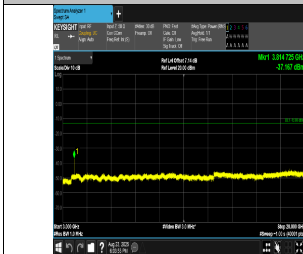
Band2-3MHz-QPSK-19185-1RB#0-3000~20000-PASS
