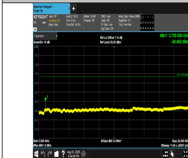
Band2-5MHz-QPSK-18900-1RB#0-3000~20000-PASS
