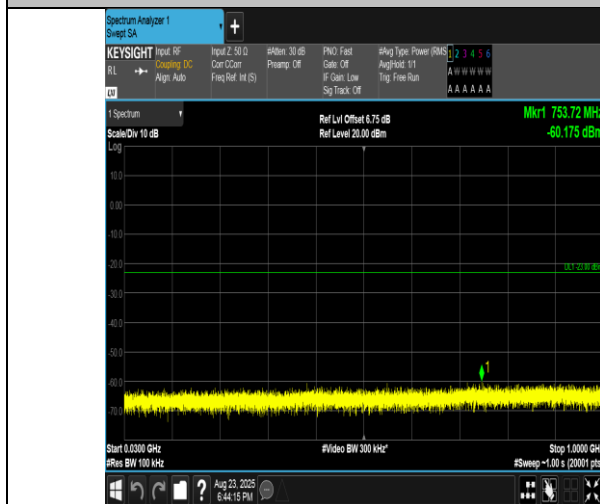
Band2-5MHz-QPSK-18900-1RB#0-30~1000-PASS
