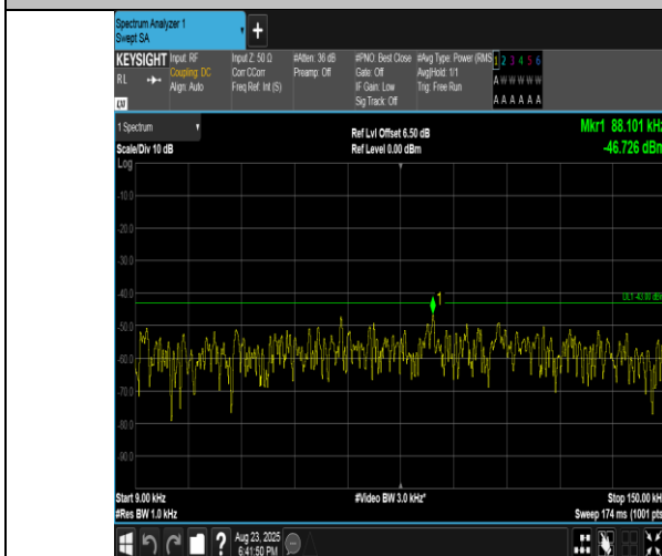
Band2-5MHz-QPSK-18625-25RB#0-0.009~0.15-PASS
