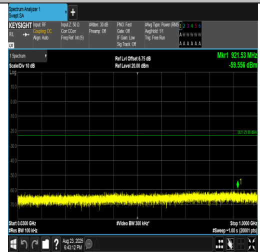
Band2-5MHz-16QAM-18625-25RB#0-30~1000-PASS
