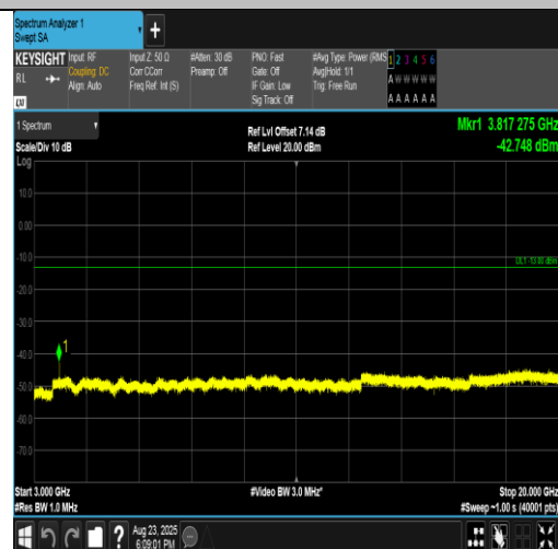
Band2-3MHz-16QAM-19185-15RB#0-3000~20000-PASS
