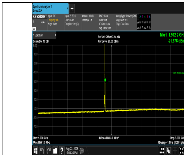
Band2-3MHz-16QAM-19185-1RB#0-1000~3000-PASS
