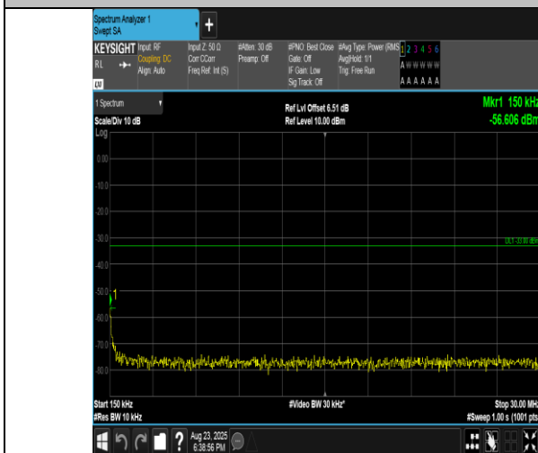
Band2-5MHz-16QAM-18625-1RB#0-0.15~30-PASS
