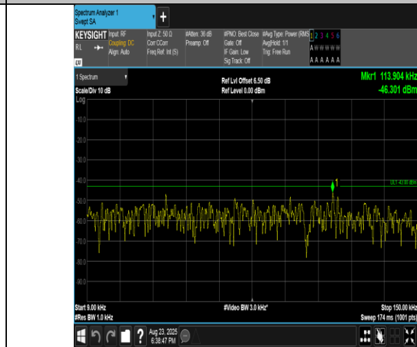
Band2-5MHz-16QAM-18625-1RB#0-0.009~0.15-PASS
