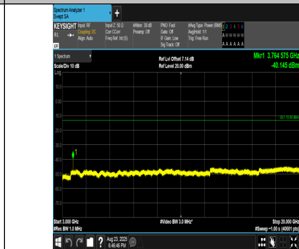
Band2-5MHz-QPSK-18900-1RB#24-3000~20000-PASS
