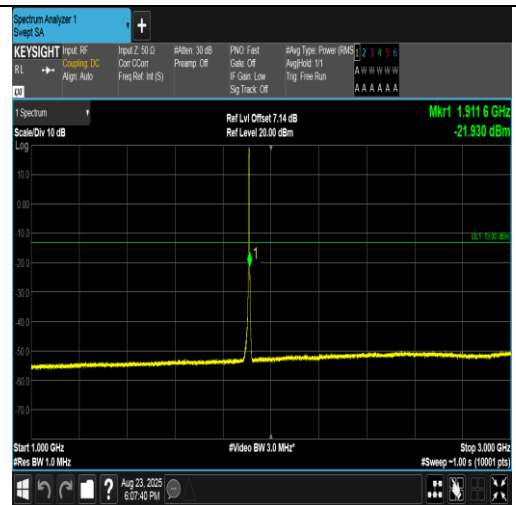
Band2-3MHz-QPSK-19185-15RB#0-1000~3000-PASS
