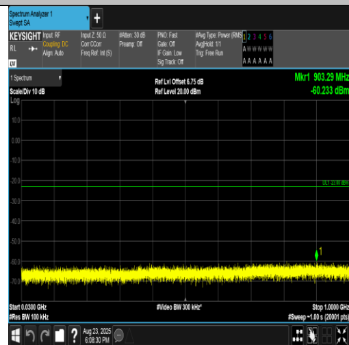
Band2-3MHz-16QAM-19185-15RB#0-30~1000-PASS
