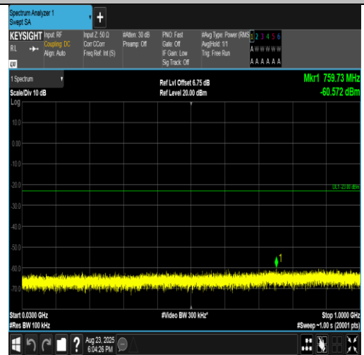
Band2-3MHz-16QAM-19185-1RB#0-30~1000-PASS
