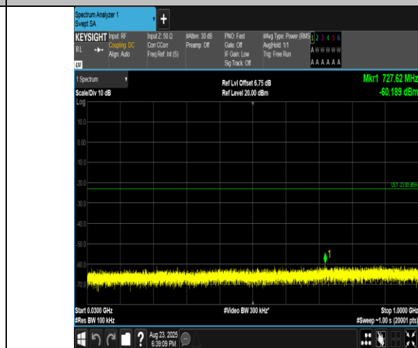
Band2-5MHz-16QAM-18625-1RB#0-30~1000-PASS
