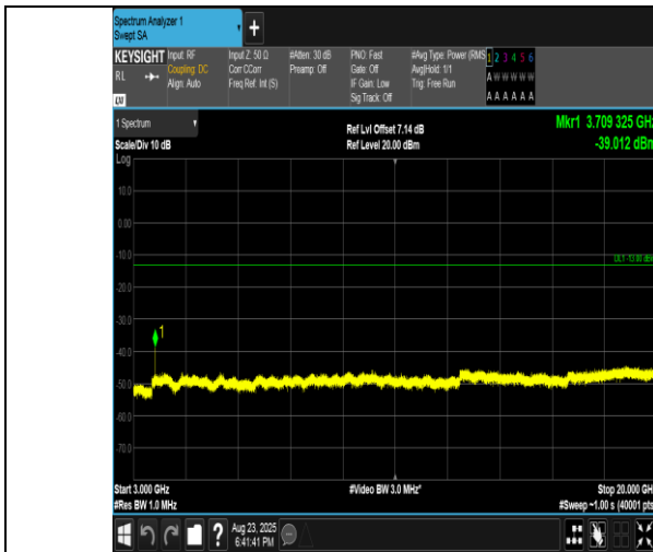
Band2-5MHz-16QAM-18625-1RB#24-3000~20000-PASS
