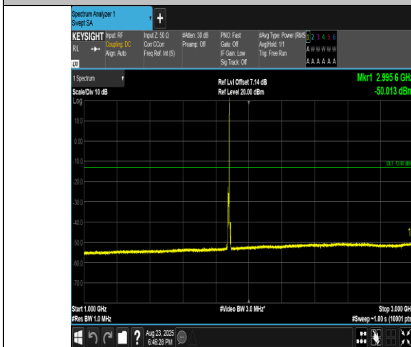
Band2-5MHz-QPSK-18900-1RB#24-1000~3000-PASS
