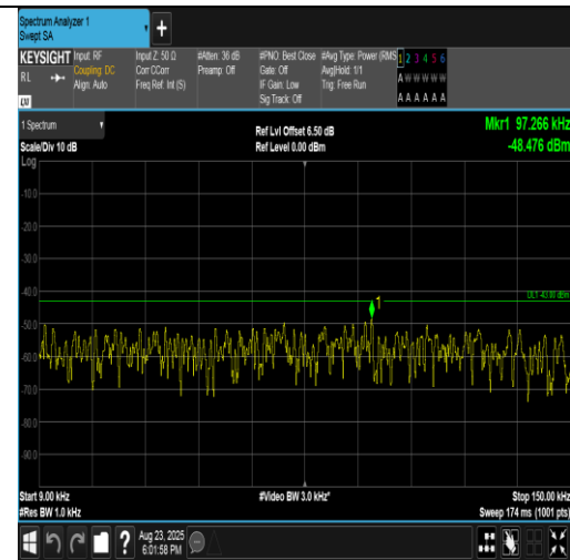
Band2-3MHz-16QAM-18900-15RB#0-0.009~0.15-PASS
