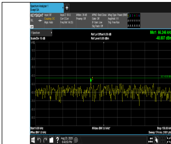
Band2-5MHz-QPSK-18900-1RB#0-0.009~0.15-PASS
