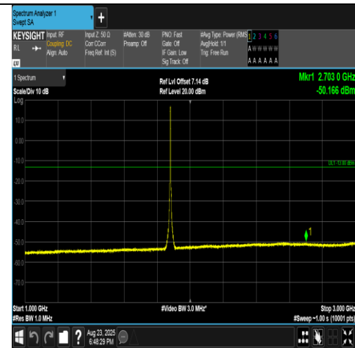
Band2-5MHz-QPSK-18900-25RB#0-1000~3000-PASS
