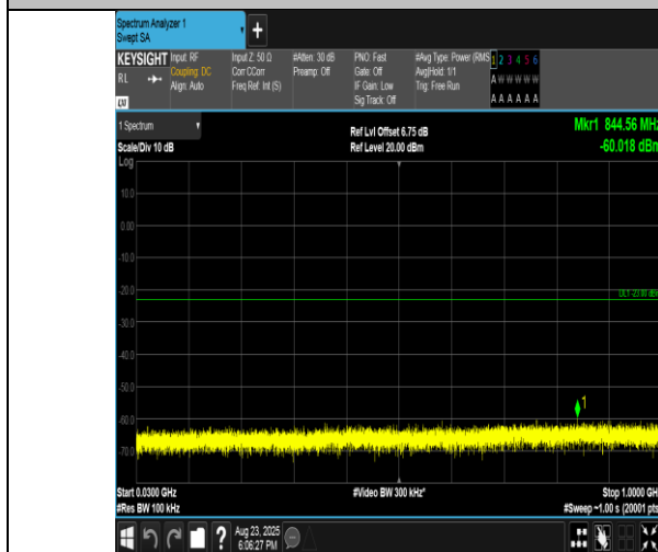
Band2-3MHz-16QAM-19185-1RB#14-30~1000-PASS
