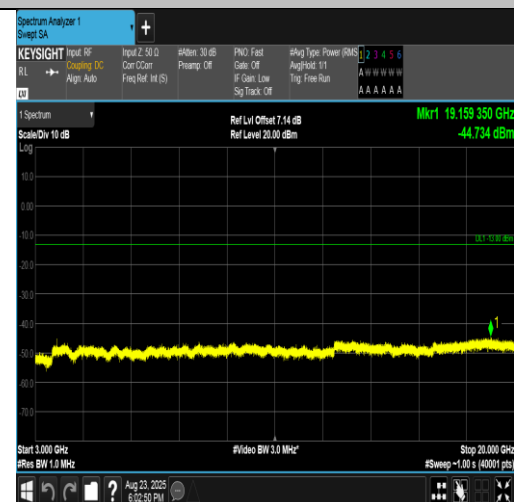
Band2-3MHz-16QAM-18900-15RB#0-3000~20000-PASS
