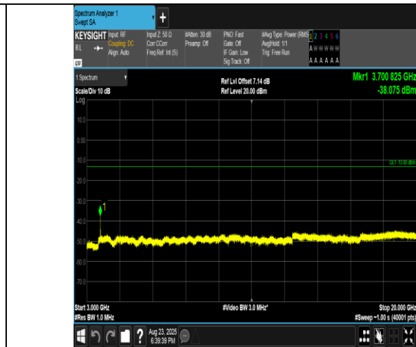
Band2-5MHz-16QAM-18625-1RB#0-3000~20000-PASS
