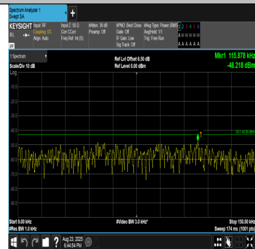
Band2-5MHz-16QAM-18900-1RB#0-0.009~0.15-PASS
