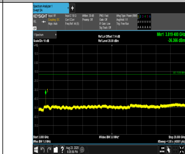
Band2-3MHz-QPSK-19185-1RB#14-3000~20000-PASS
