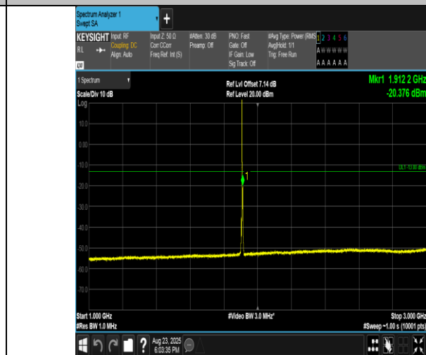
Band2-3MHz-QPSK-19185-1RB#0-1000~3000-PASS
