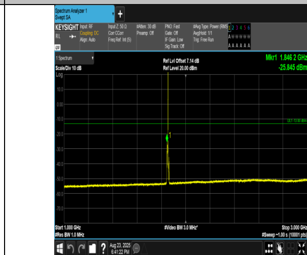
Band2-5MHz-16QAM-18625-1RB#24-1000~3000-PASS
