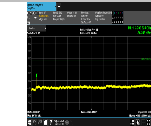
Band2-5MHz-QPSK-18625-1RB#24-3000~20000-PASS
