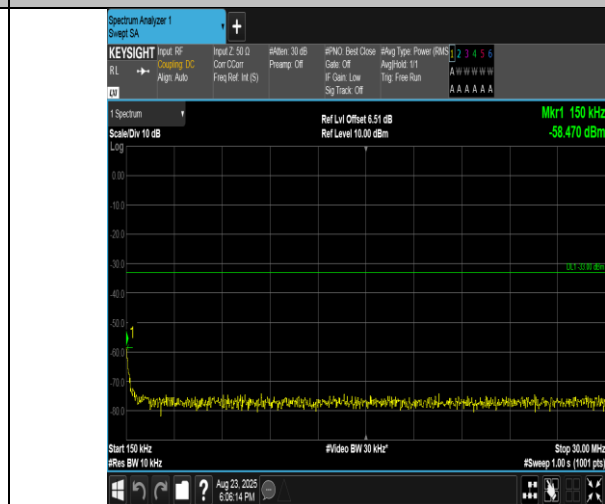
Band2-3MHz-16QAM-19185-1RB#14-0.15~30-PASS
