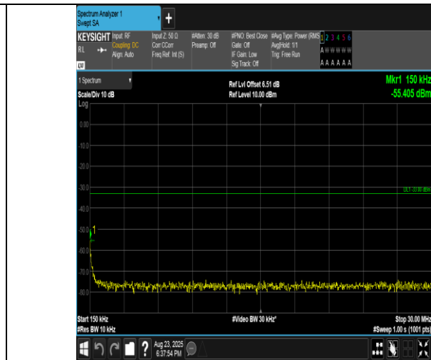
Band2-5MHz-QPSK-18625-1RB#0-0.15~30-PASS
