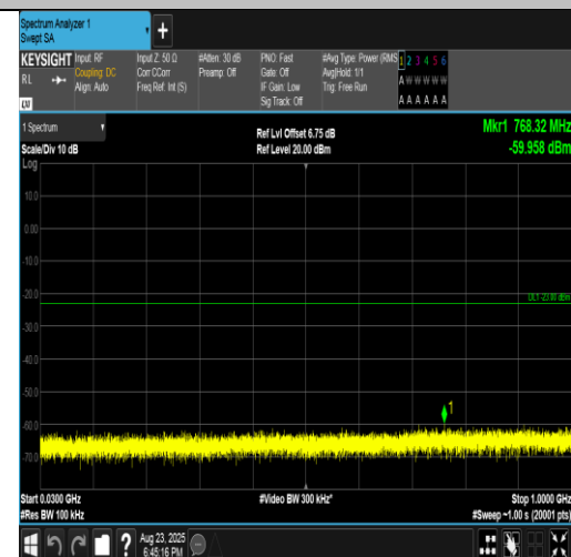
Band2-5MHz-16QAM-18900-1RB#0-30~1000-PASS
