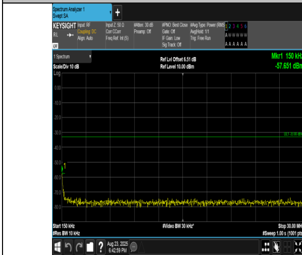
Band2-5MHz-16QAM-18625-25RB#0-0.15~30-PASS
