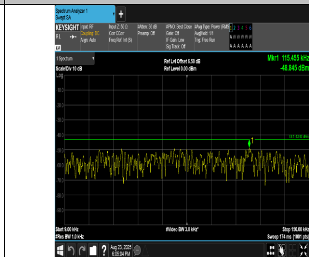
Band2-3MHz-QPSK-19185-1RB#14-0.009~0.15-PASS
