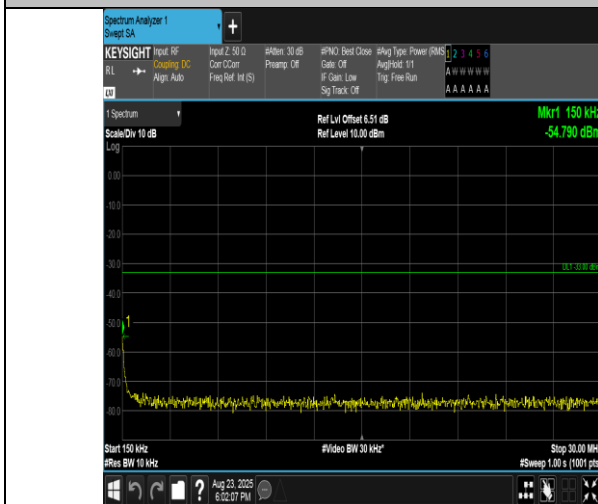
Band2-3MHz-16QAM-18900-15RB#0-0.15~30-PASS
