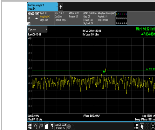
Band2-5MHz-16QAM-18625-1RB#24-0.009~0.15-PASS
