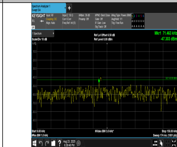
Band2-5MHz-QPSK-18625-1RB#24-0.009~0.15-PASS
