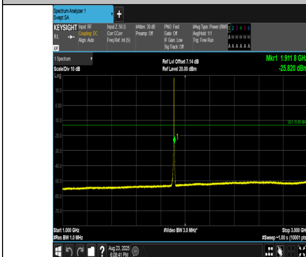
Band2-3MHz-16QAM-19185-15RB#0-1000~3000-PASS
