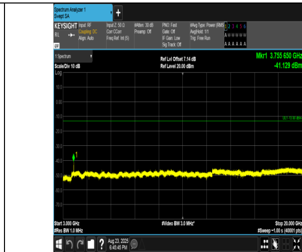
Band2-5MHz-16QAM-18900-1RB#0-3000~20000-PASS
