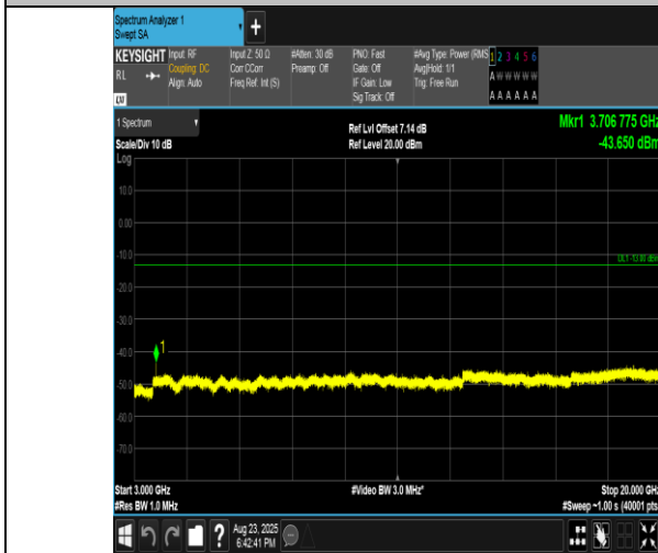
Band2-5MHz-QPSK-18625-25RB#0-3000~20000-PASS
