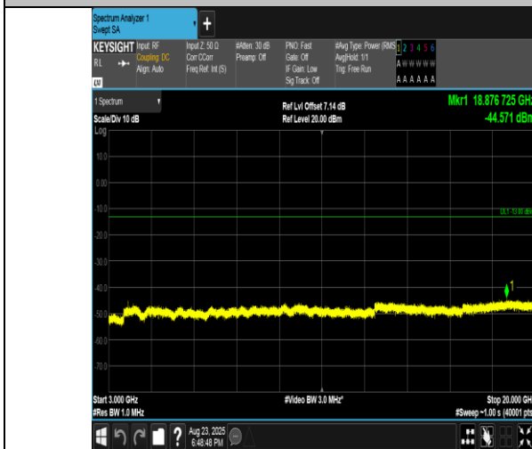
Band2-5MHz-QPSK-18900-25RB#0-3000~20000-PASS
