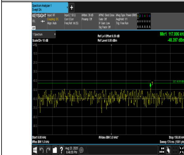
Band2-5MHz-16QAM-18900-1RB#24-0.009~0.15-PASS
