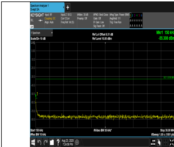
Band2-10MHz-QPSK-18650-1RB#49-0.15~30-PASS
