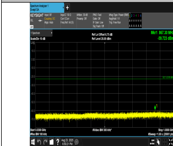
Band2-5MHz-QPSK-19175-1RB#0-30~1000-PASS
