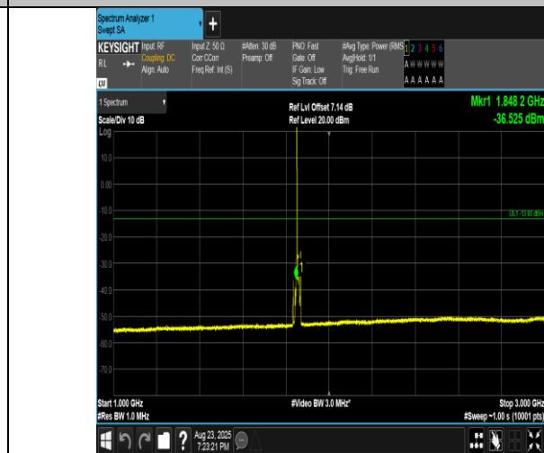
Band2-10MHz-QPSK-18650-1RB#0-1000~3000-PASS
