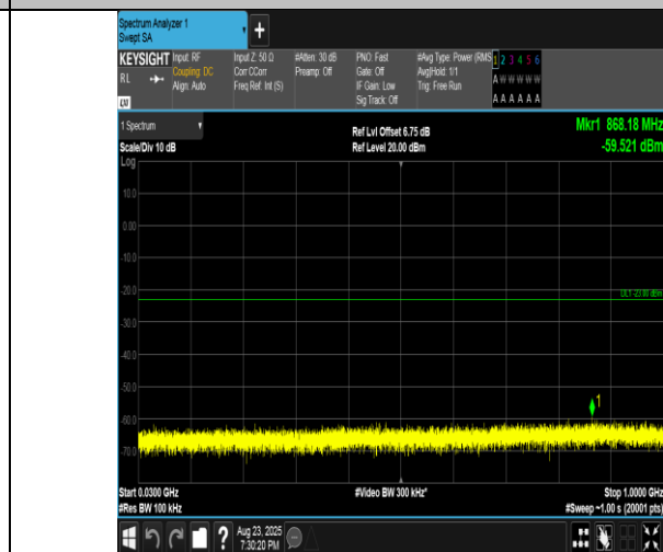
Band2-10MHz-16QAM-18900-1RB#0-30~1000-PASS
