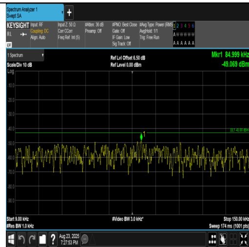
Band2-10MHz-16QAM-18650-50RB#0-0.009~0.15-PASS
