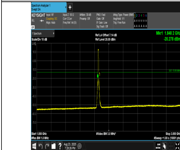
Band2-10MHz-16QAM-18650-50RB#0-1000~3000-PASS
