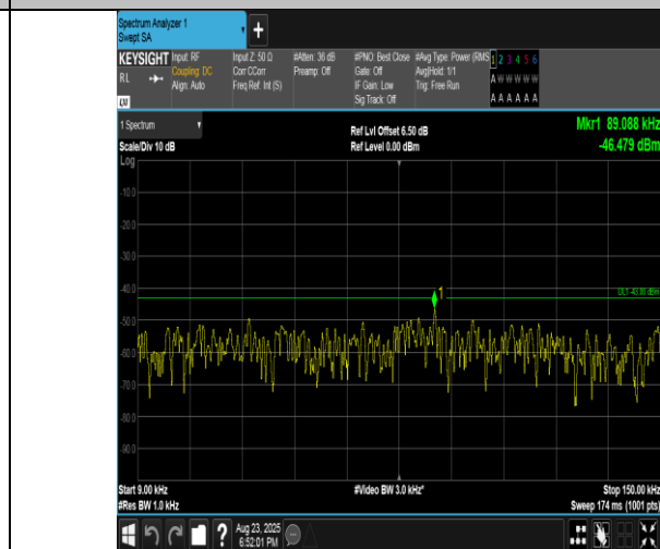
Band2-5MHz-QPSK-19175-1RB#24-0.009~0.15-PASS
