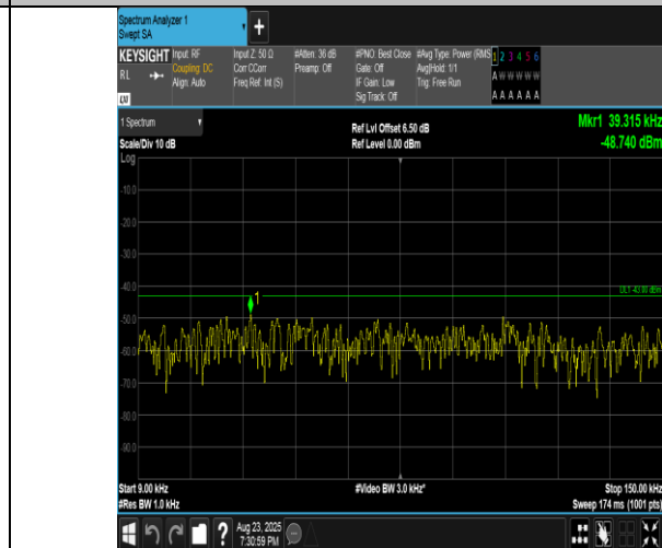
Band2-10MHz-QPSK-18900-1RB#49-0.009~0.15-PASS
