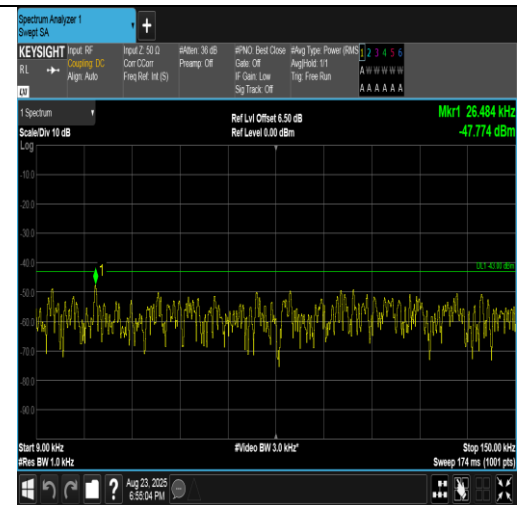
Band2-5MHz-16QAM-19175-25RB#0-0.009~0.15-PASS
