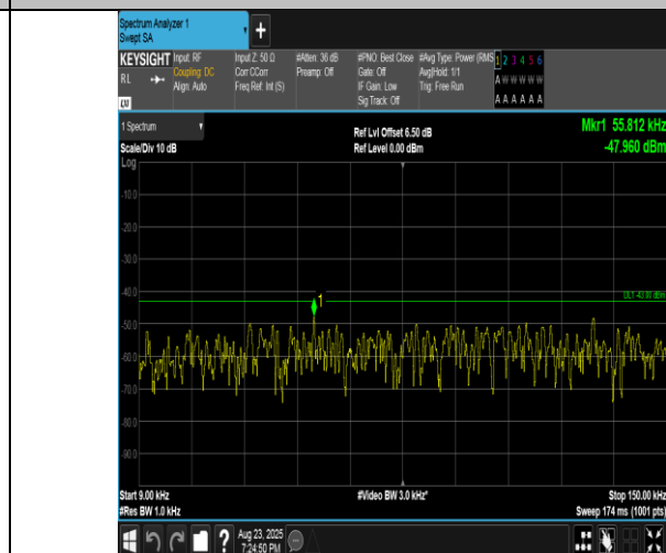
Band2-10MHz-QPSK-18650-1RB#49-0.009~0.15-PASS
