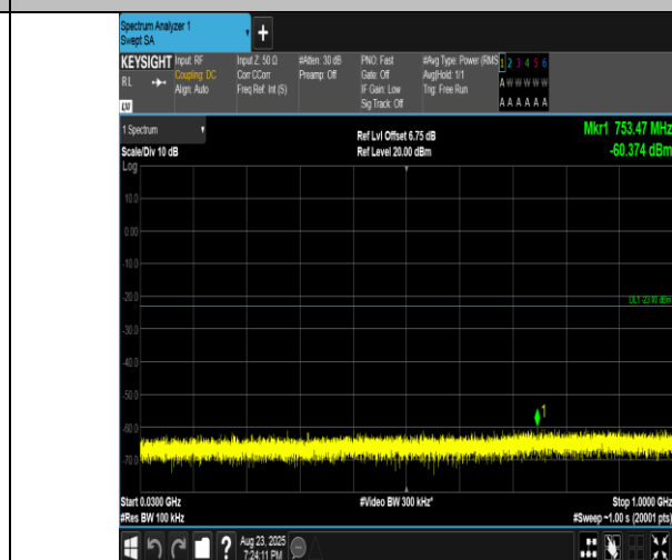
Band2-10MHz-16QAM-18650-1RB#0-30~1000-PASS
