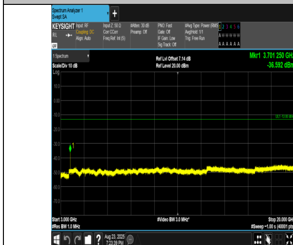
Band2-10MHz-QPSK-18650-1RB#0-3000~20000-PASS
