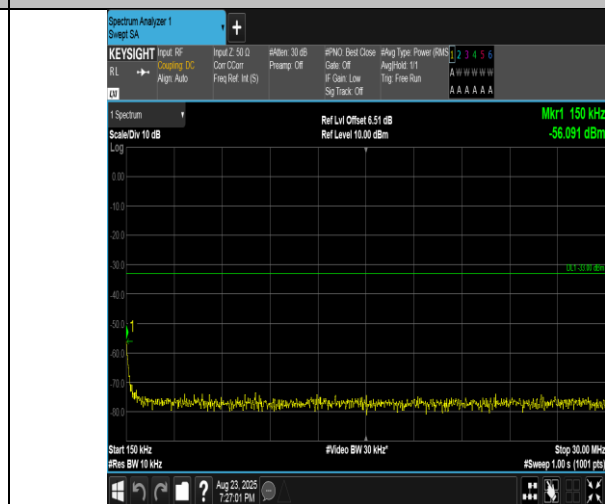
Band2-10MHz-QPSK-18650-50RB#0-0.15~30-PASS
