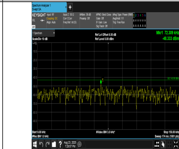
Band2-10MHz-16QAM-18900-1RB#0-0.009~0.15-PASS
