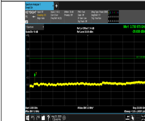
Band2-10MHz-QPSK-18900-1RB#0-3000~20000-PASS
