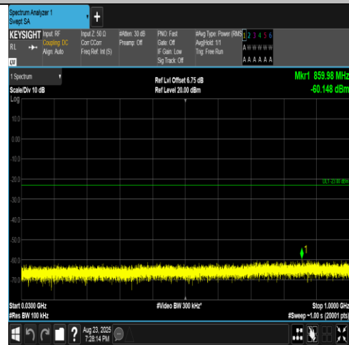
Band2-10MHz-16QAM-18650-50RB#0-30~1000-PASS
