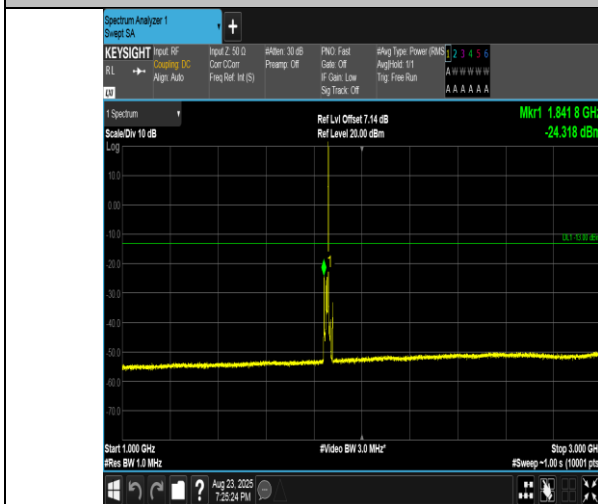
Band2-10MHz-QPSK-18650-1RB#49-1000~3000-PASS
