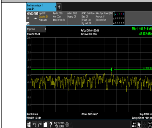
Band2-10MHz-QPSK-18650-50RB#0-0.009~0.15-PASS
