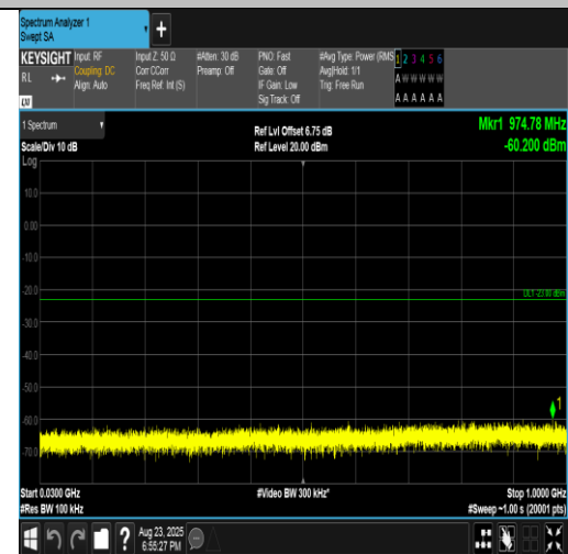
Band2-5MHz-16QAM-19175-25RB#0-30~1000-PASS
