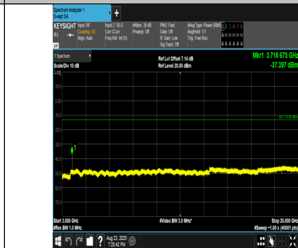
Band2-10MHz-QPSK-18650-1RB#49-3000~20000-PASS
