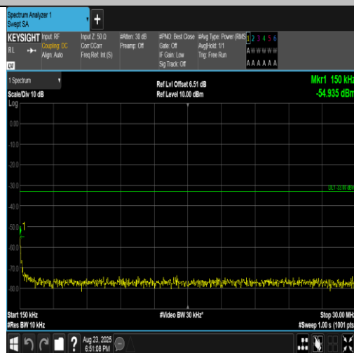
Band2-5MHz-16QAM-19175-1RB#0-0.15~30-PASS
