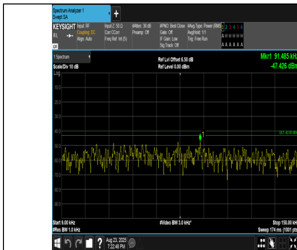
Band2-10MHz-QPSK-18650-1RB#0-0.009~0.15-PASS
