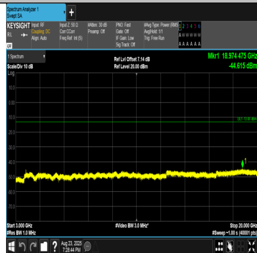
Band2-10MHz-16QAM-18650-50RB#0-3000~20000-PASS
