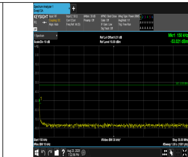
Band2-10MHz-QPSK-18650-1RB#0-0.15~30-PASS
