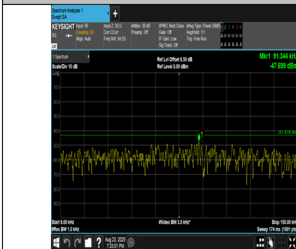
Band2-10MHz-QPSK-18900-50RB#0-0.009~0.15-PASS
