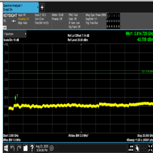
Band2-5MHz-QPSK-19175-25RB#0-3000~20000-PASS
