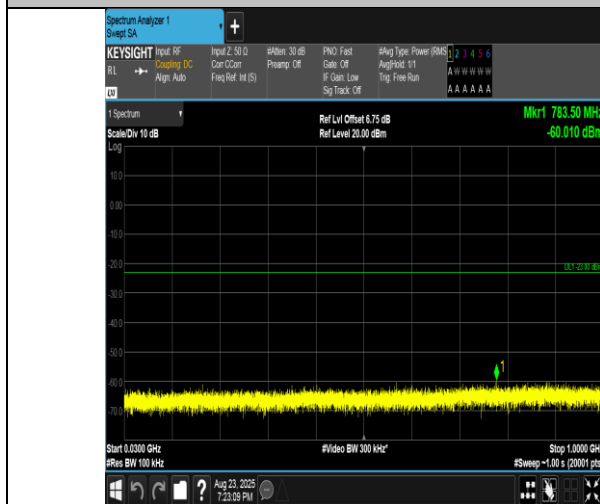
Band2-10MHz-QPSK-18650-1RB#0-30~1000-PASS
