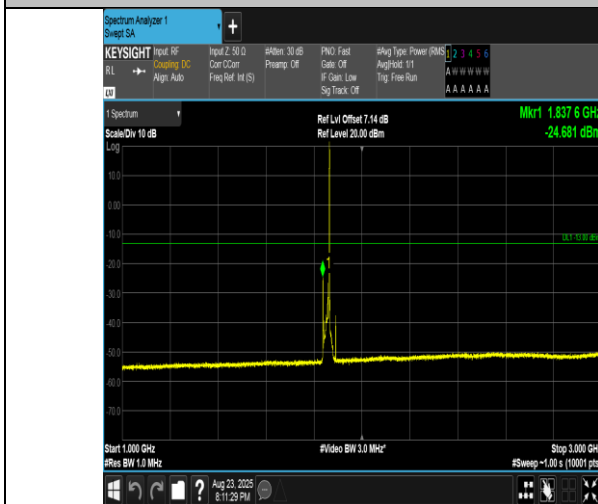
Band2-15MHz-QPSK-18675-1RB#74-1000~3000-PASS
