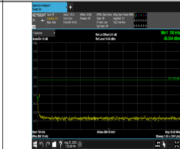
Band2-10MHz-16QAM-18900-1RB#49-0.15~30-PASS
