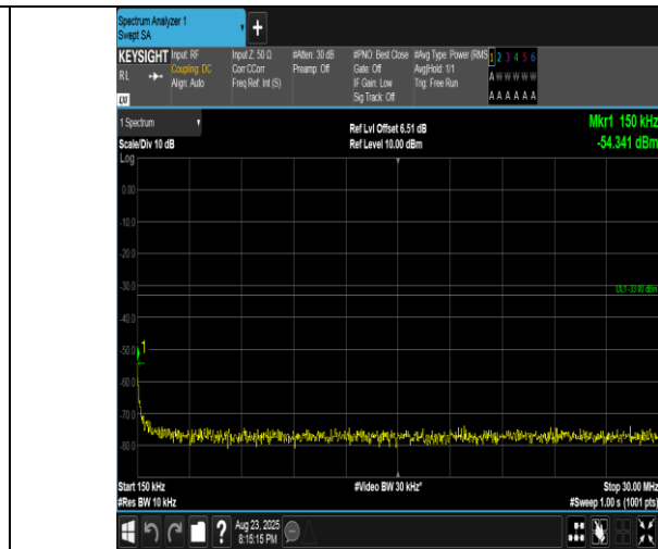
Band2-15MHz-QPSK-18900-1RB#0-0.15~30-PASS
