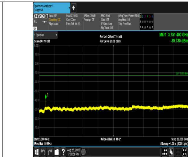
Band2-10MHz-16QAM-18900-1RB#0-3000~20000-PASS
