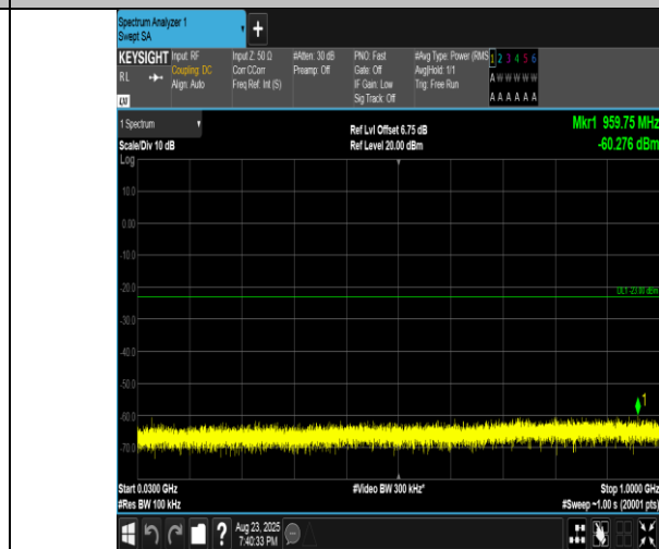
Band2-10MHz-16QAM-19150-50RB#0-30~1000-PASS
