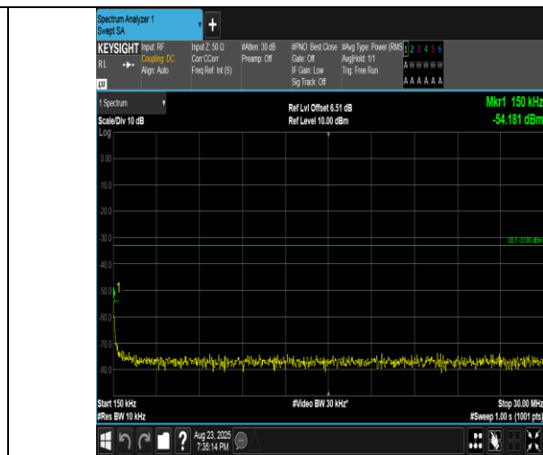
Band2-10MHz-QPSK-19150-1RB#0-0.15~30-PASS
