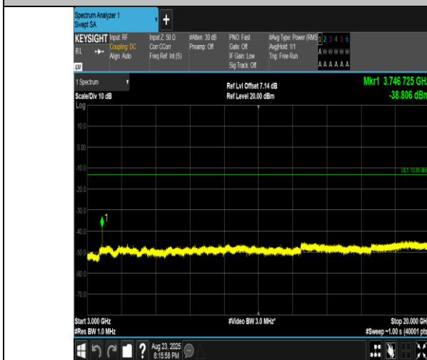
Band2-15MHz-QPSK-18900-1RB#0-3000~20000-PASS
