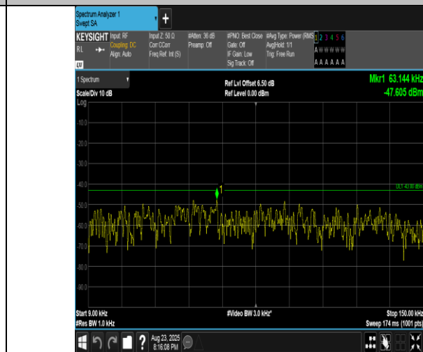
Band2-15MHz-16QAM-18900-1RB#0-0.009~0.15-PASS
