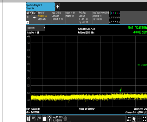
Band2-15MHz-16QAM-18900-1RB#0-30~1000-PASS
