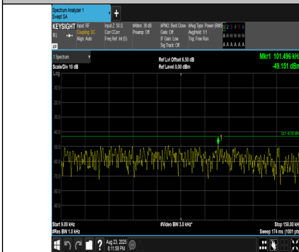
Band2-15MHz-16QAM-18675-1RB#74-0.009~0.15-PASS
