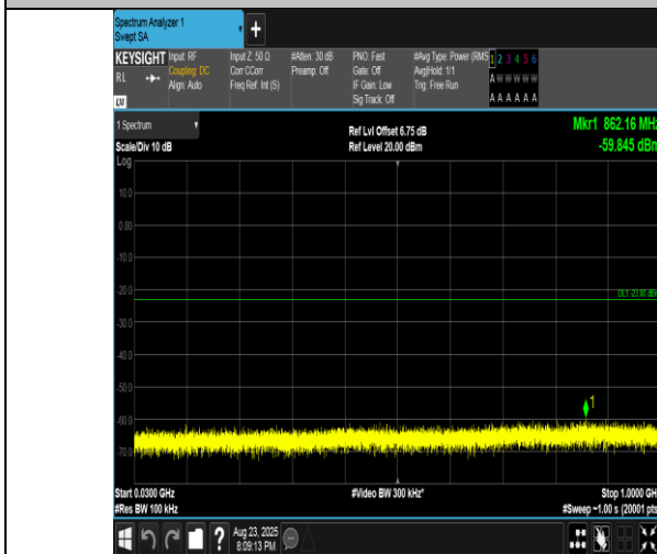
Band2-15MHz-QPSK-18675-1RB#0-30~1000-PASS
