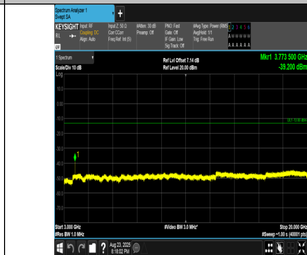
Band2-15MHz-QPSK-18900-1RB#74-3000~20000-PASS
