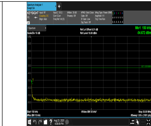
Band2-15MHz-QPSK-18675-1RB#0-0.15~30-PASS
