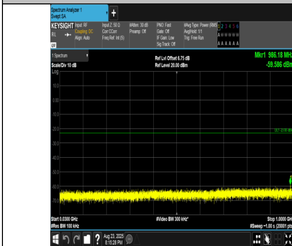
Band2-15MHz-QPSK-18900-1RB#0-30~1000-PASS
