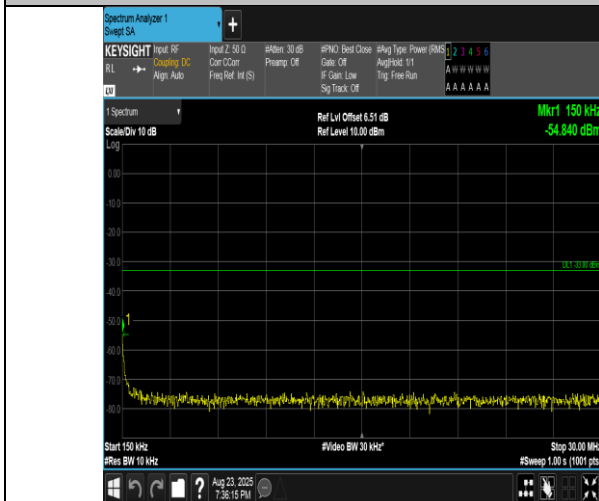
Band2-10MHz-16QAM-19150-1RB#0-0.15~30-PASS
