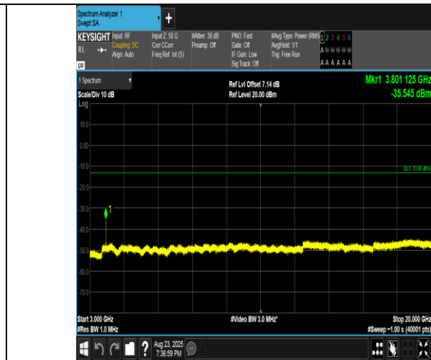
Band2-10MHz-16QAM-19150-1RB#0-3000~20000-PASS
