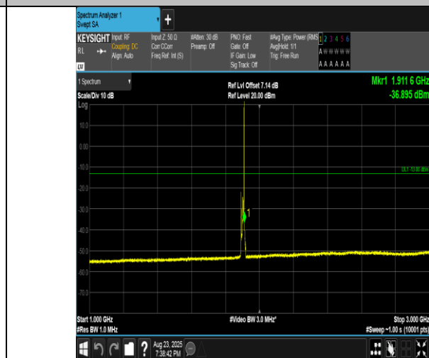
Band2-10MHz-16QAM-19150-1RB#49-1000~3000-PASS
