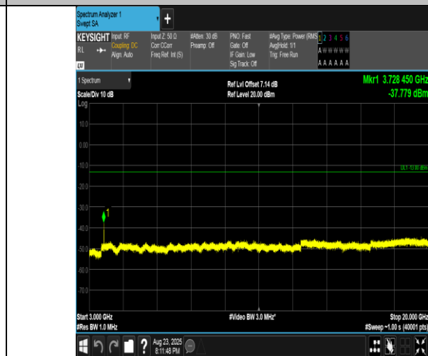
Band2-15MHz-QPSK-18675-1RB#74-3000~20000-PASS
