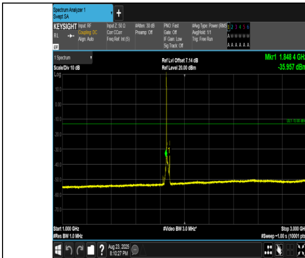
Band2-15MHz-16QAM-18675-1RB#0-1000~3000-PASS
