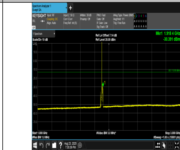
Band2-10MHz-QPSK-19150-1RB#0-1000~3000-PASS
