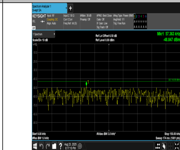
Band2-15MHz-QPSK-18900-1RB#74-0.009~0.15-PASS
