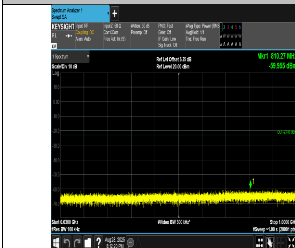
Band2-15MHz-16QAM-18675-1RB#74-30~1000-PASS
