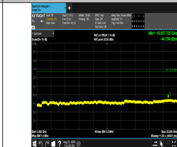
Band2-10MHz-16QAM-19150-50RB#0-3000~20000-PASS
