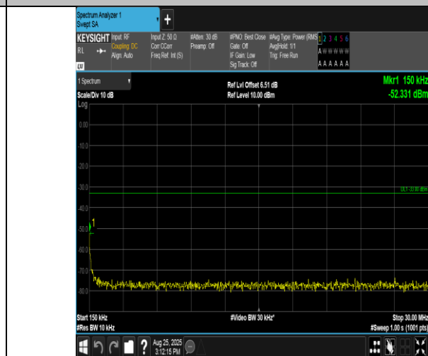
Band2-15MHz-QPSK-18900-75RB#0-0.15~30-PASS
