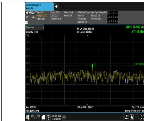
Band2-10MHz-QPSK-19150-1RB#0-0.009~0.15-PASS
