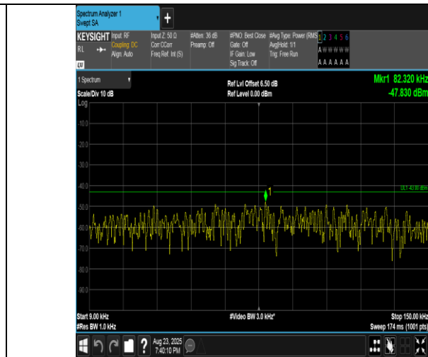
Band2-10MHz-16QAM-19150-50RB#0-0.009~0.15-PASS
