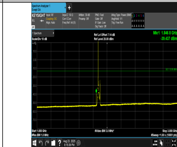
Band2-15MHz-QPSK-18900-1RB#0-1000~3000-PASS
