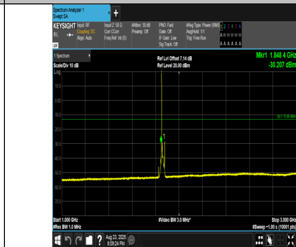
Band2-15MHz-QPSK-18675-1RB#0-1000~3000-PASS
