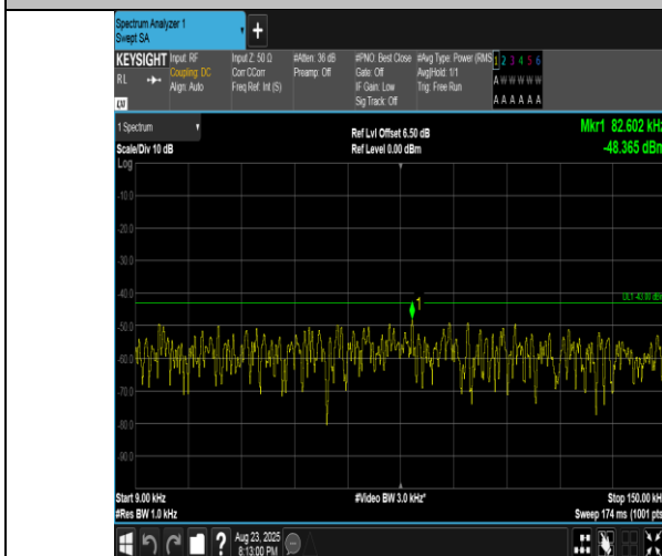
Band2-15MHz-QPSK-18675-75RB#0-0.009~0.15-PASS
