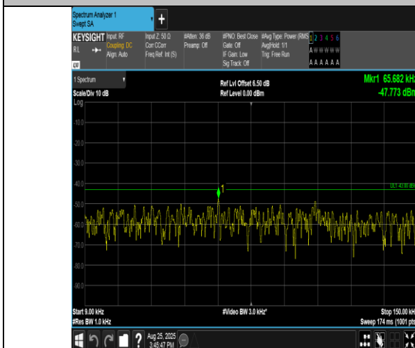
Band2-20MHz-QPSK-18700-100RB#0-0.009~0.15-PASS
