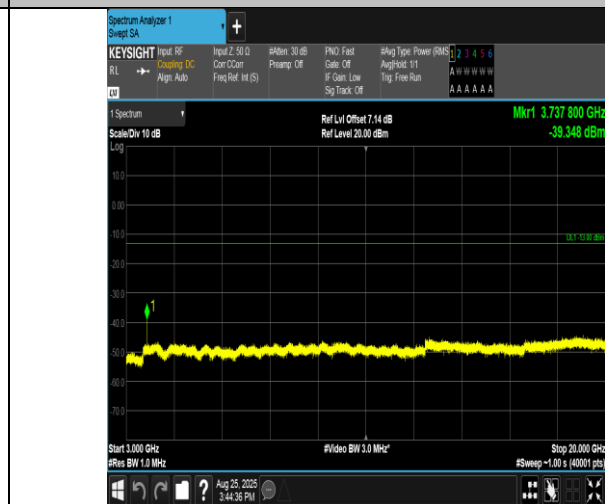
Band2-20MHz-QPSK-18700-1RB#99-3000~20000-PASS
