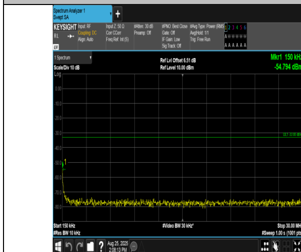
Band2-15MHz-16QAM-19125-1RB#0-0.15~30-PASS
