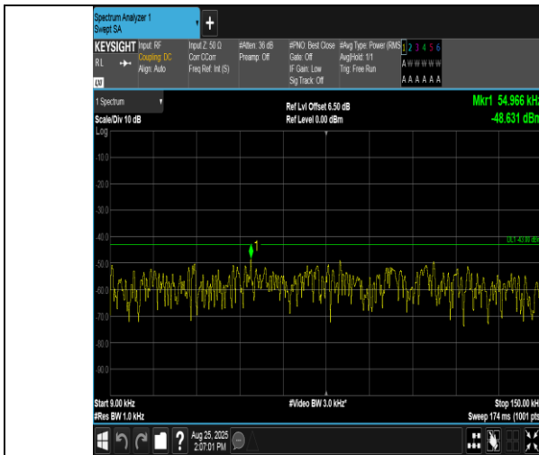
Band2-15MHz-QPSK-19125-1RB#0-0.009~0.15-PASS
