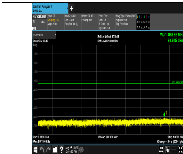
Band2-15MHz-QPSK-19125-75RB#0-30~1000-PASS
