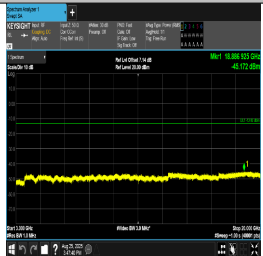
Band2-20MHz-16QAM-18700-100RB#0-3000~20000-PASS
