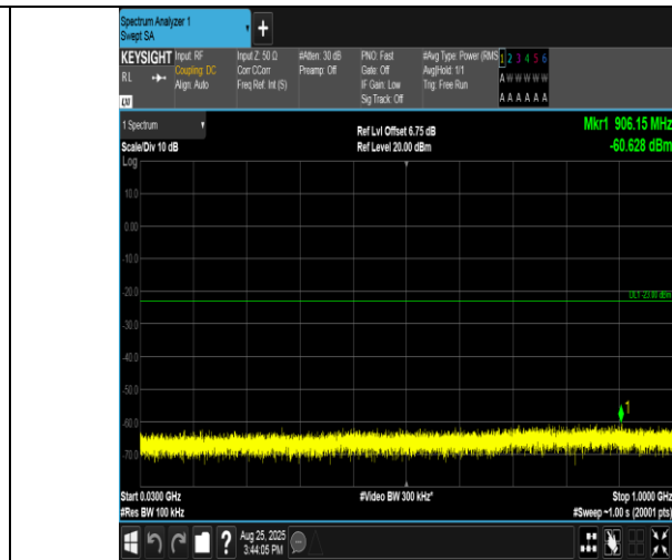
Band2-20MHz-QPSK-18700-1RB#99-30~1000-PASS
