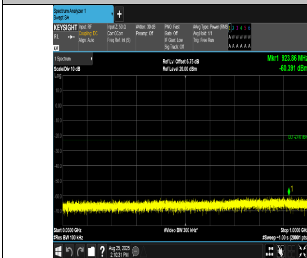
Band2-15MHz-16QAM-19125-1RB#74-30~1000-PASS
