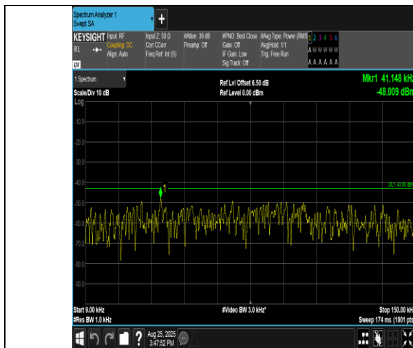
Band2-20MHz-QPSK-18900-1RB#0-0.009~0.15-PASS
