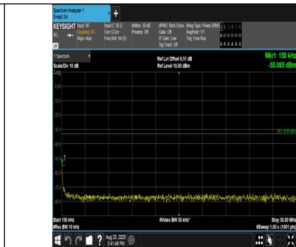
Band2-20MHz-QPSK-18700-1RB#0-0.15~30-PASS
