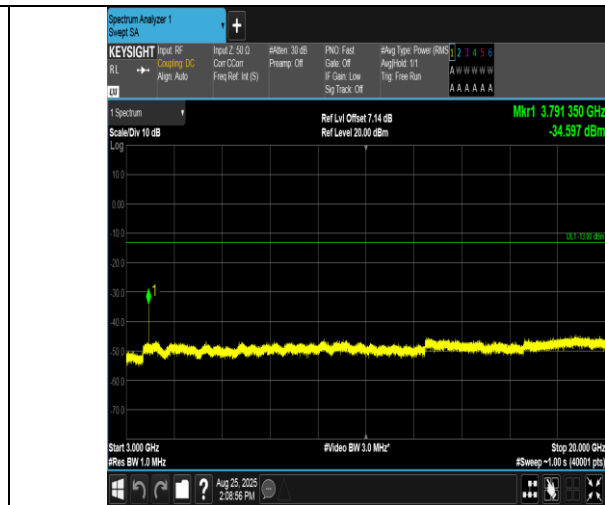
Band2-15MHz-16QAM-19125-1RB#0-3000~20000-PASS
