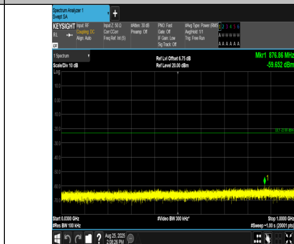
Band2-15MHz-16QAM-19125-1RB#0-30~1000-PASS
