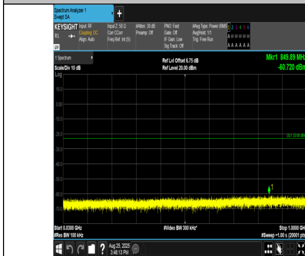
Band2-20MHz-QPSK-18900-1RB#0-30~1000-PASS
