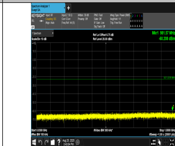
Band2-20MHz-16QAM-18700-1RB#0-30~1000-PASS
