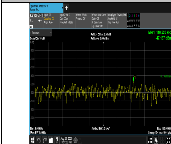
Band2-20MHz-QPSK-18900-100RB#0-0.009~0.15-PASS
