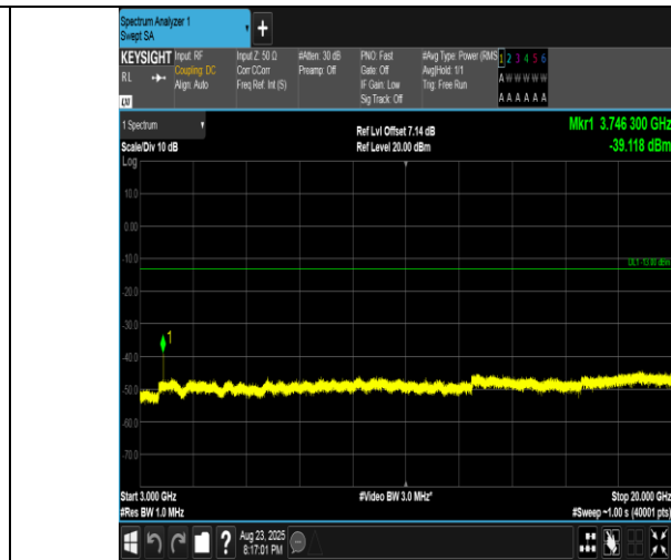
Band2-15MHz-16QAM-18900-1RB#0-3000~20000-PASS
