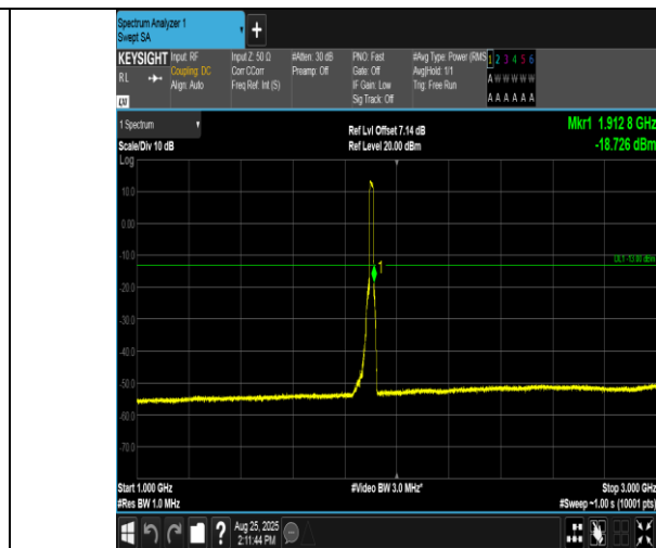
Band2-15MHz-QPSK-19125-75RB#0-1000~3000-PASS
