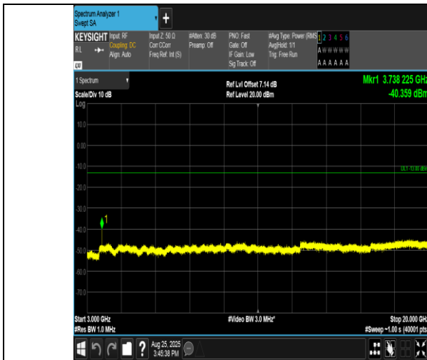
Band2-20MHz-16QAM-18700-1RB#99-3000~20000-PASS
