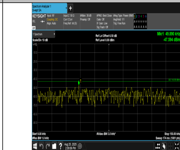
Band2-15MHz-QPSK-19125-1RB#74-0.009~0.15-PASS
