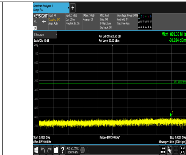
Band2-20MHz-QPSK-18900-1RB#99-30~1000-PASS
