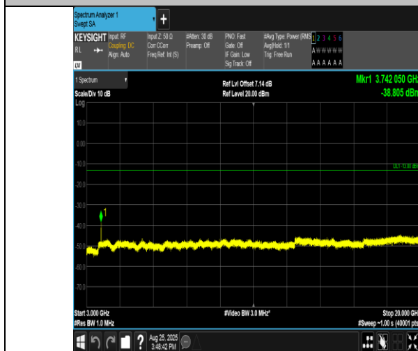
Band2-20MHz-QPSK-18900-1RB#0-3000~20000-PASS
