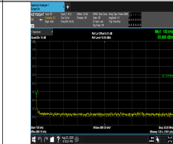
Band2-15MHz-16QAM-18900-1RB#74-0.15~30-PASS
