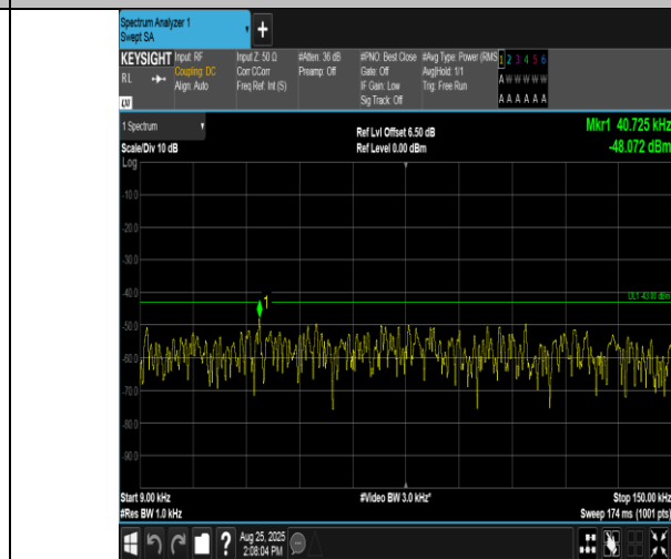
Band2-15MHz-16QAM-19125-1RB#0-0.009~0.15-PASS
