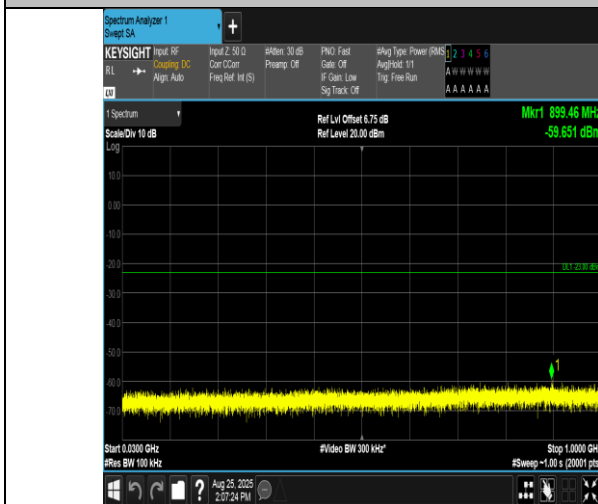
Band2-15MHz-QPSK-19125-1RB#0-30~1000-PASS
