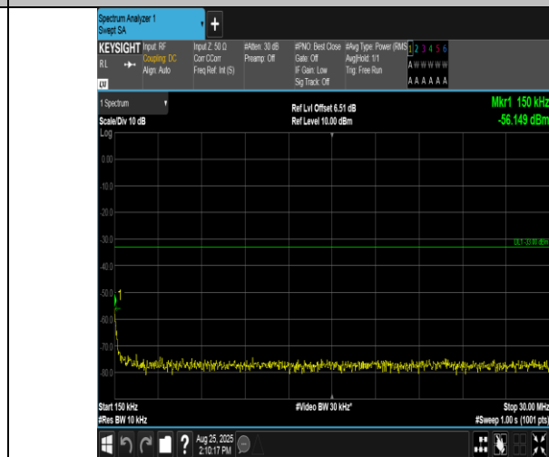
Band2-15MHz-16QAM-19125-1RB#74-0.15~30-PASS
