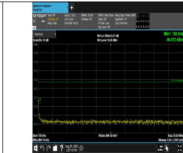
Band2-15MHz-QPSK-19125-1RB#0-0.15~30-PASS
