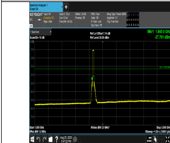
Band2-20MHz-16QAM-18700-100RB#0-1000~3000-PASS
