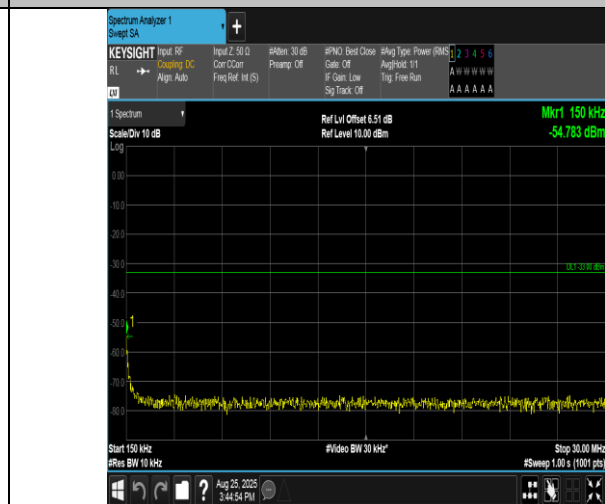
Band2-20MHz-16QAM-18700-1RB#99-0.15~30-PASS
