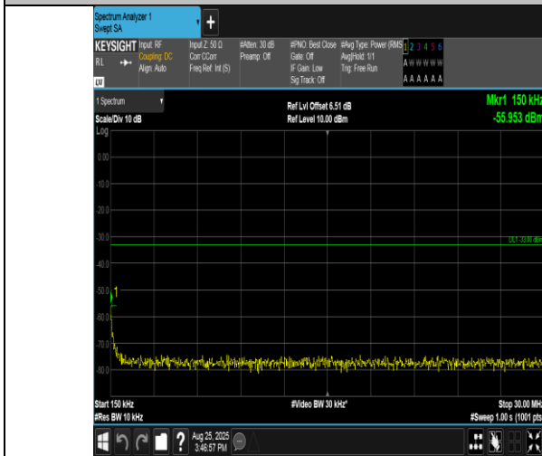
Band2-20MHz-16QAM-18700-100RB#0-0.15~30-PASS
