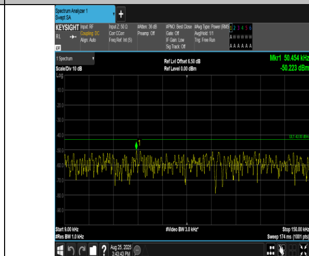
Band2-20MHz-QPSK-18700-1RB#99-0.009~0.15-PASS
