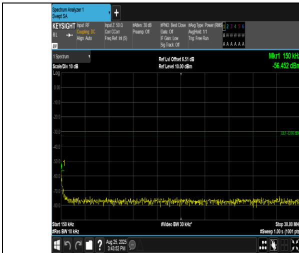
Band2-20MHz-QPSK-18700-1RB#99-0.15~30-PASS
