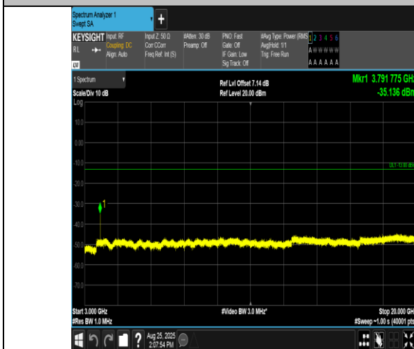
Band2-15MHz-QPSK-19125-1RB#0-3000~20000-PASS
