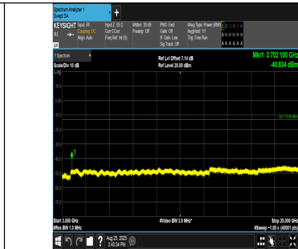
Band2-20MHz-16QAM-18700-1RB#0-3000~20000-PASS
