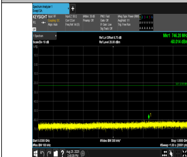
Band2-20MHz-16QAM-18700-1RB#99-30~1000-PASS
