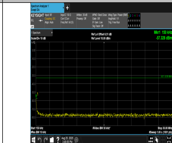
Band2-20MHz-QPSK-18700-100RB#0-0.15~30-PASS
