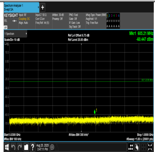
Band2-20MHz-16QAM-18700-100RB#0-30~1000-PASS
