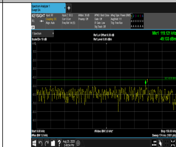
Band2-20MHz-QPSK-18900-1RB#99-0.009~0.15-PASS
