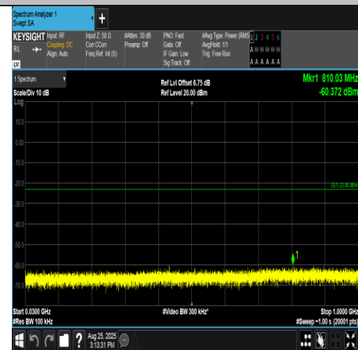
Band2-15MHz-16QAM-18900-75RB#0-30~1000-PASS
