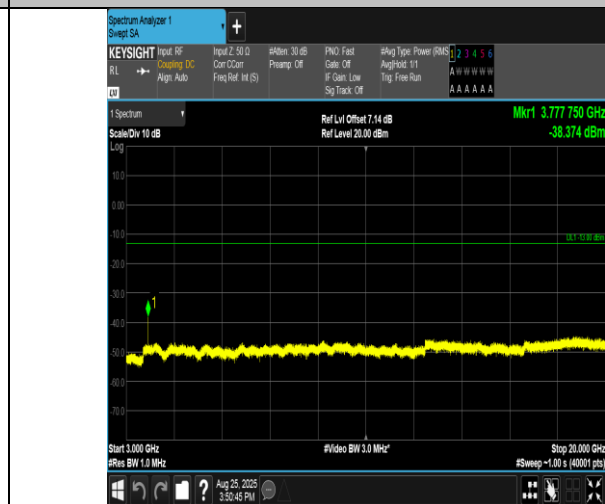
Band2-20MHz-QPSK-18900-1RB#99-3000~20000-PASS
