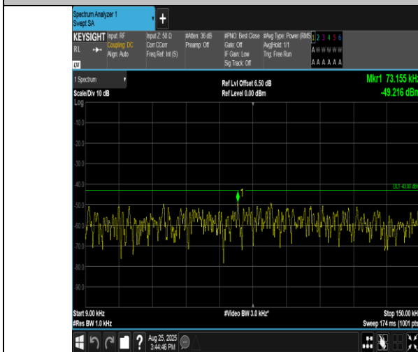
Band2-20MHz-16QAM-18700-1RB#99-0.009~0.15-PASS
