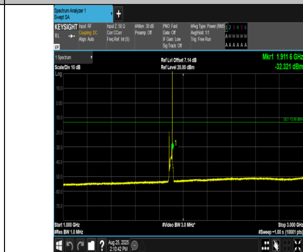
Band2-15MHz-16QAM-19125-1RB#74-1000~3000-PASS
