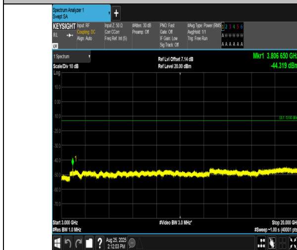
Band2-15MHz-QPSK-19125-75RB#0-3000~20000-PASS
