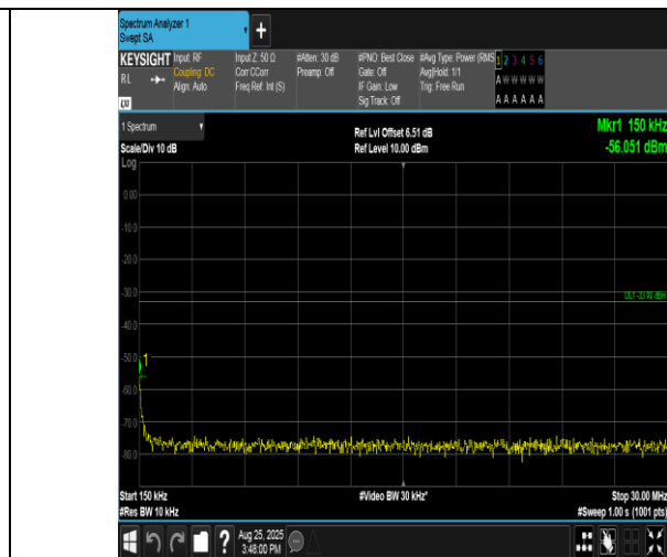
Band2-20MHz-QPSK-18900-1RB#0-0.15~30-PASS
