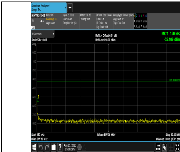
Band2-20MHz-QPSK-18900-1RB#99-0.15~30-PASS
