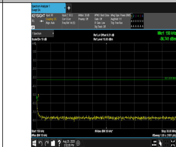
Band2-20MHz-QPSK-18900-100RB#0-0.15~30-PASS
