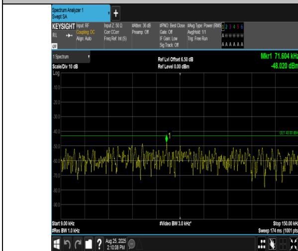
Band2-15MHz-16QAM-19125-1RB#74-0.009~0.15-PASS
