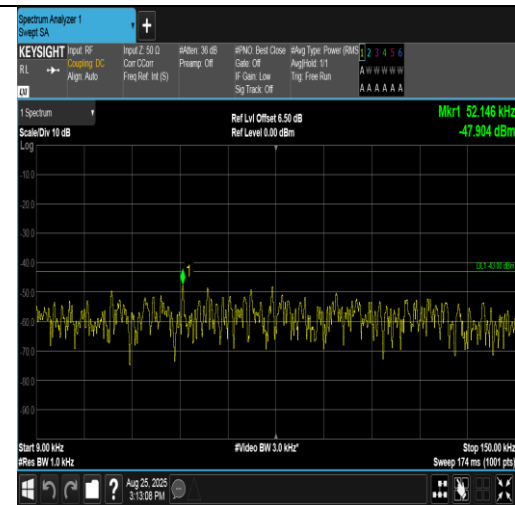
Band2-15MHz-16QAM-18900-75RB#0-0.009~0.15-PASS
