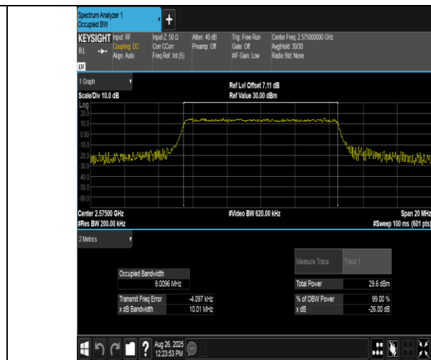
Band38-10MHz-16QAM-37800-50RB#0-PASS
