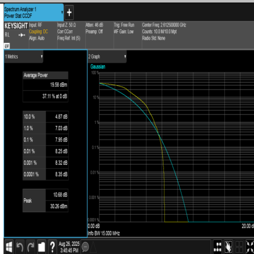
Band38-15MHz-QPSK-38175-1RB#0-PASS
