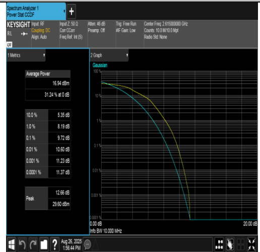
Band38-10MHz-16QAM-38200-50RB#0-PASS
