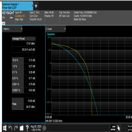
Band38-10MHz-16QAM-38200-1RB#0-PASS
