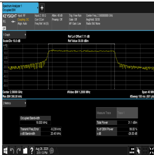
Band38-20MHz-QPSK-37850-100RB#0-PASS
