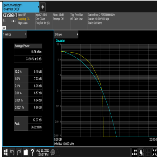
Band38-10MHz-QPSK-38000-1RB#0-PASS
