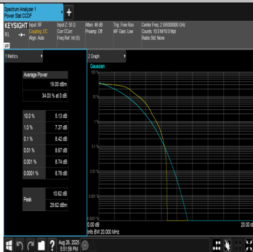
Band38-20MHz-QPSK-38000-1RB#0-PASS
