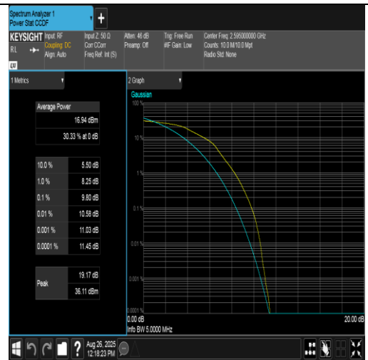
Band38-5MHz-16QAM-38000-25RB#0-PASS
