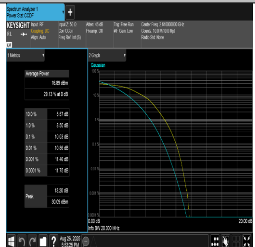
Band38-20MHz-16QAM-38150-100RB#0-PASS
