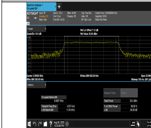
Band38-10MHz-QPSK-38000-50RB#0-PASS
