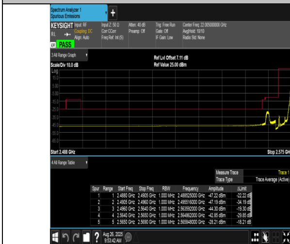
Band38-5MHz-16QAM-37775-1RB#24-PASS
