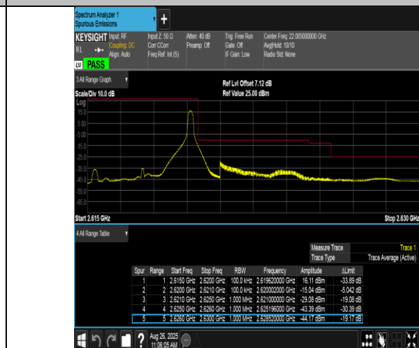
Band38-5MHz-QPSK-38225-1RB#24-PASS
