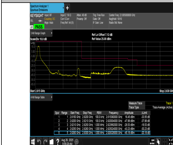
Band38-5MHz-QPSK-38225-1RB#0-PASS
