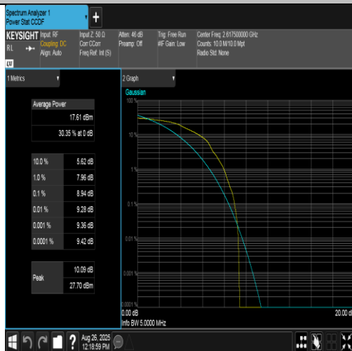
Band38-5MHz-16QAM-38225-1RB#0-PASS
