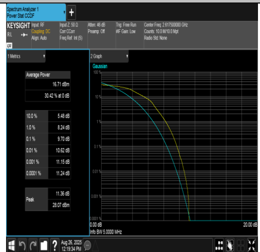
Band38-5MHz-16QAM-38225-25RB#0-PASS
