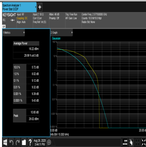
Band38-15MHz-16QAM-37825-1RB#0-PASS
