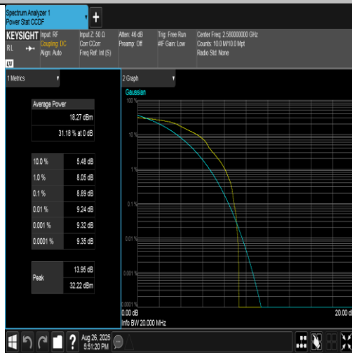
Band38-20MHz-16QAM-37850-1RB#0-PASS
