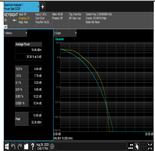
Band38-15MHz-QPSK-38000-75RB#0-PASS
