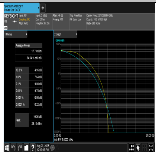
Band38-5MHz-QPSK-38225-25RB#0-PASS
