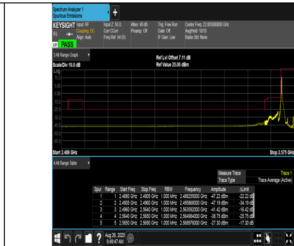
Band38-5MHz-16QAM-37775-1RB#0-PASS
