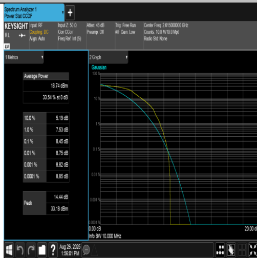
Band38-10MHz-QPSK-38200-1RB#0-PASS
