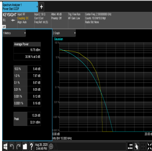
Band38-15MHz-QPSK-38000-1RB#0-PASS
