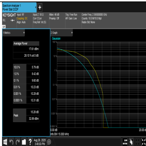
Band38-15MHz-16QAM-38000-1RB#0-PASS
