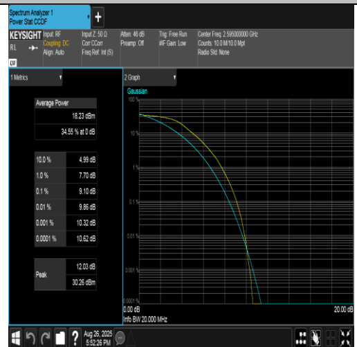
Band38-20MHz-QPSK-38000-100RB#0-PASS
