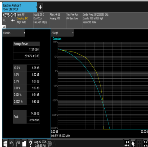
Band38-15MHz-16QAM-38175-1RB#0-PASS
