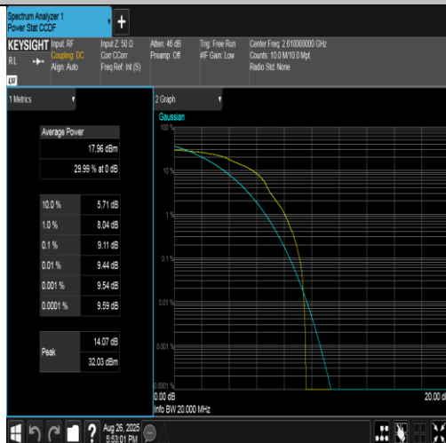
Band38-20MHz-16QAM-38150-1RB#0-PASS
