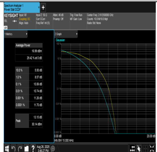
Band38-15MHz-16QAM-38175-75RB#0-PASS
