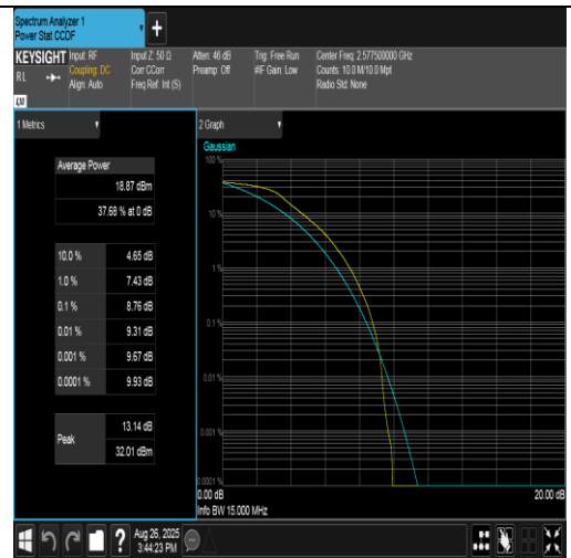
Band38-15MHz-QPSK-37825-75RB#0-PASS
