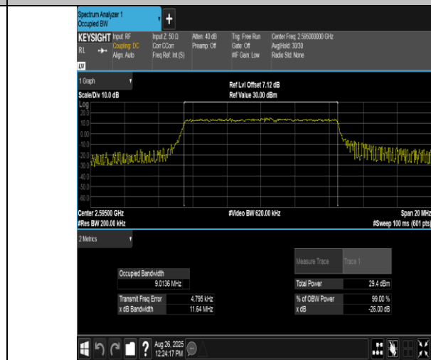
Band38-10MHz-16QAM-38000-50RB#0-PASS
