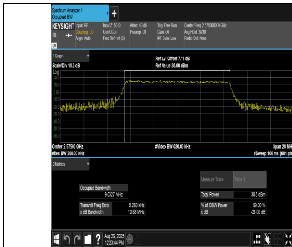
Band38-10MHz-QPSK-37800-50RB#0-PASS
