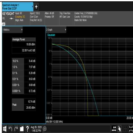
Band38-10MHz-QPSK-37800-1RB#0-PASS
