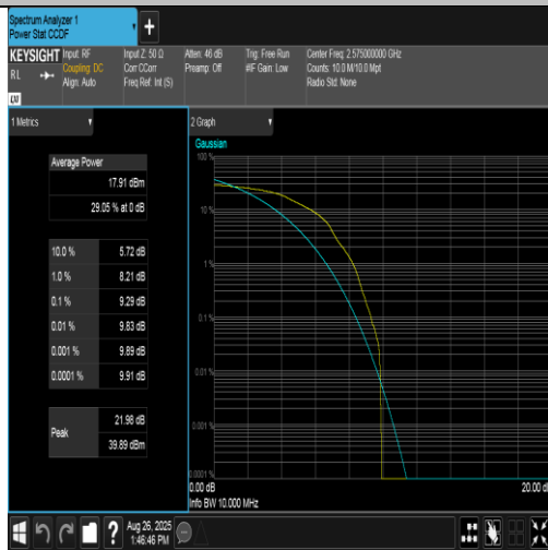
Band38-10MHz-16QAM-37800-1RB#0-PASS
