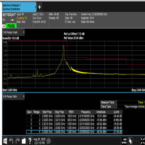
Band38-15MHz-16QAM-38175-1RB#74-PASS
