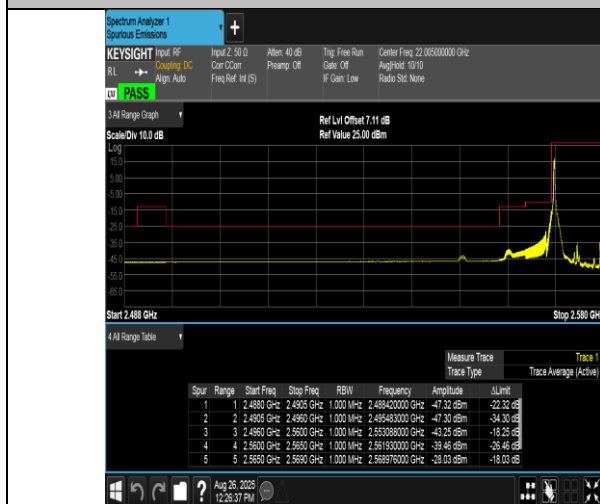
Band38-10MHz-QPSK-37800-1RB#0-PASS
