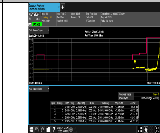
Band38-10MHz-QPSK-37800-1RB#49-PASS
