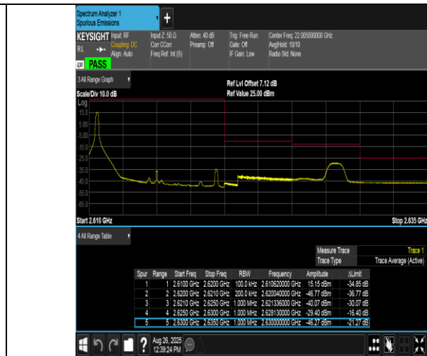
Band38-10MHz-16QAM-38200-1RB#0-PASS
