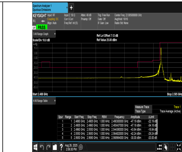
Band38-15MHz-16QAM-37825-1RB#0-PASS
