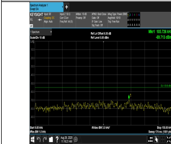
Band38-5MHz-QPSK-37775-1RB#24-0.009~0.15-PASS
