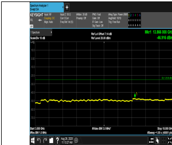
Band38-5MHz-QPSK-37775-1RB#0-3000~18000-PASS
