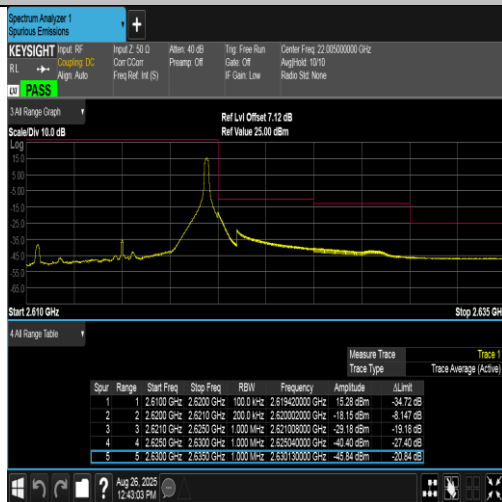
Band38-10MHz-16QAM-38200-1RB#49-PASS
