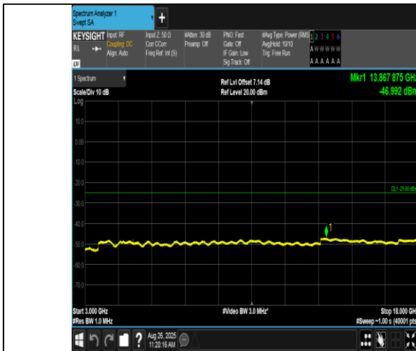
Band38-5MHz-16QAM-37775-1RB#24-3000~18000-PASS
