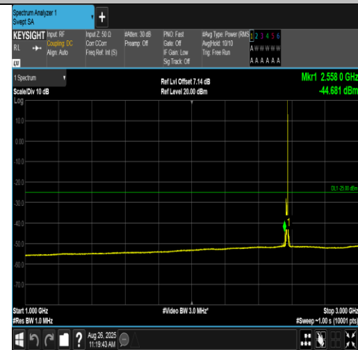
Band38-5MHz-16QAM-37775-1RB#24-1000~3000-PASS
