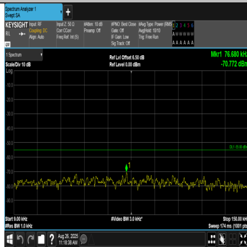
Band38-5MHz-16QAM-37775-1RB#24-0.009~0.15-PASS
