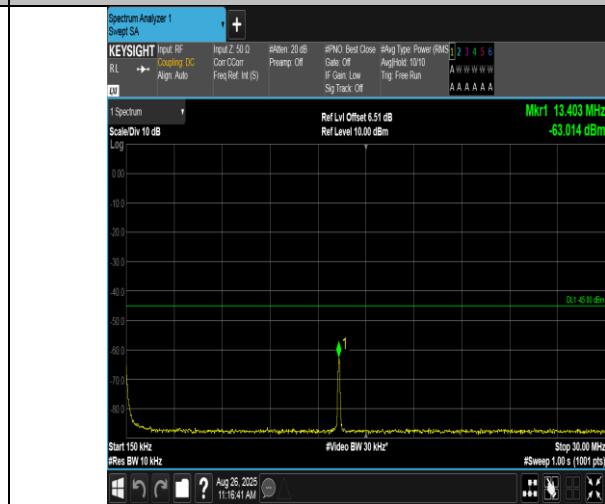
Band38-5MHz-QPSK-37775-1RB#24-0.15~30-PASS
