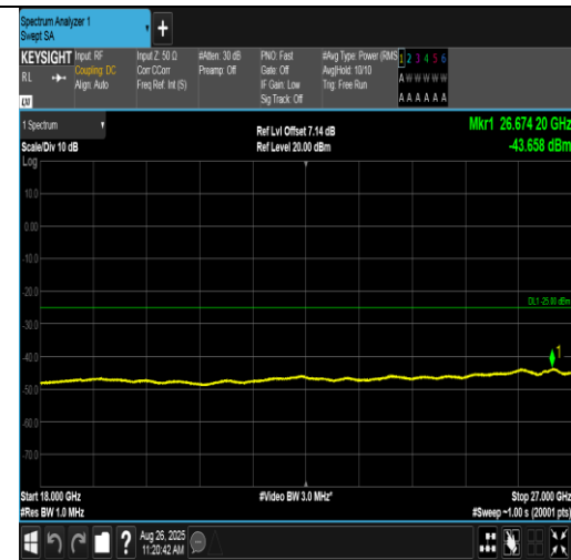
Band38-5MHz-16QAM-37775-1RB#24-18000~27000-PASS
