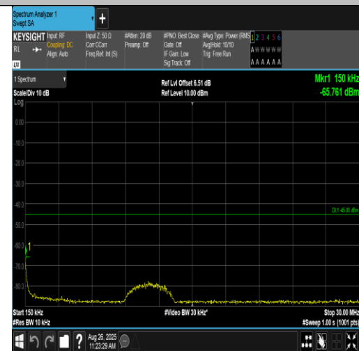
Band38-5MHz-16QAM-37775-25RB#0-0.15~30-PASS
