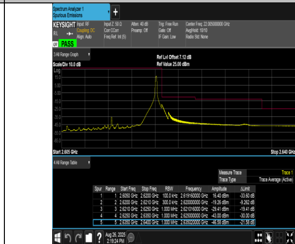
Band38-15MHz-QPSK-38175-1RB#74-PASS
