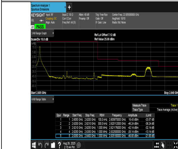
Band38-15MHz-QPSK-38175-1RB#0-PASS
