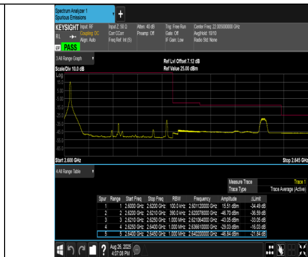
Band38-20MHz-16QAM-38150-1RB#0-PASS
