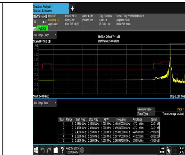
Band38-10MHz-16QAM-37800-1RB#0-PASS
