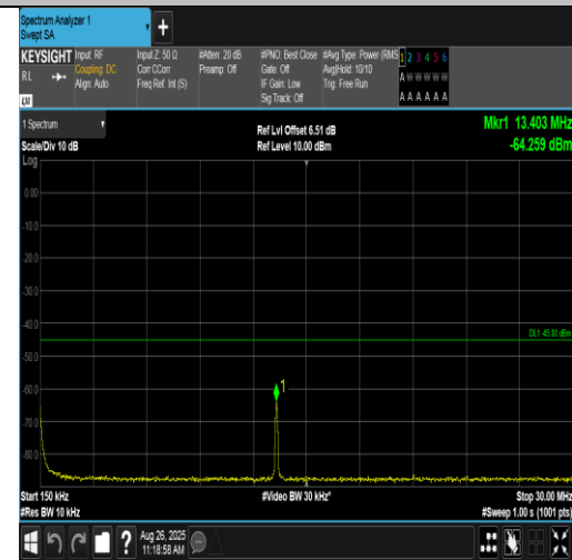
Band38-5MHz-16QAM-37775-1RB#24-0.15~30-PASS
