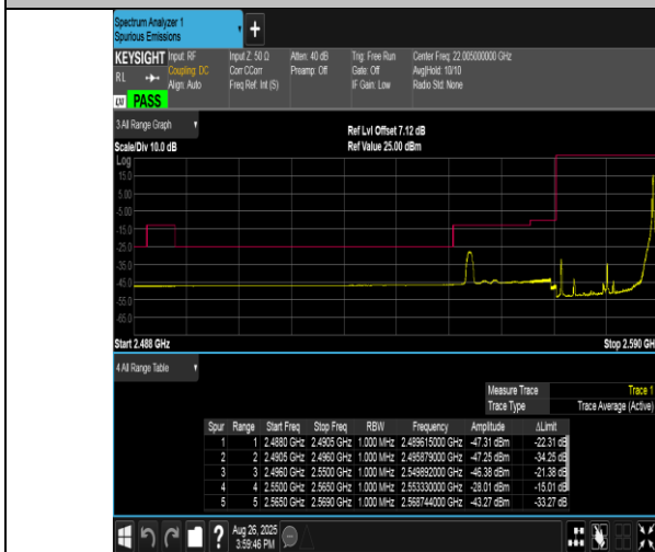
Band38-20MHz-16QAM-37850-1RB#99-PASS
