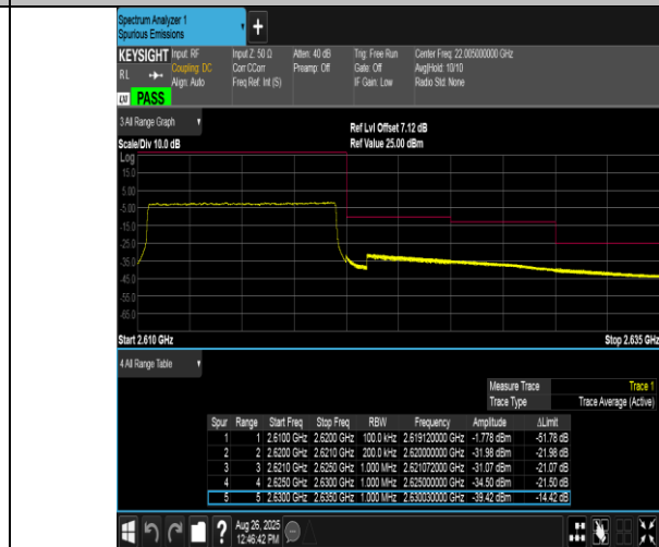
Band38-10MHz-16QAM-38200-50RB#0-PASS
