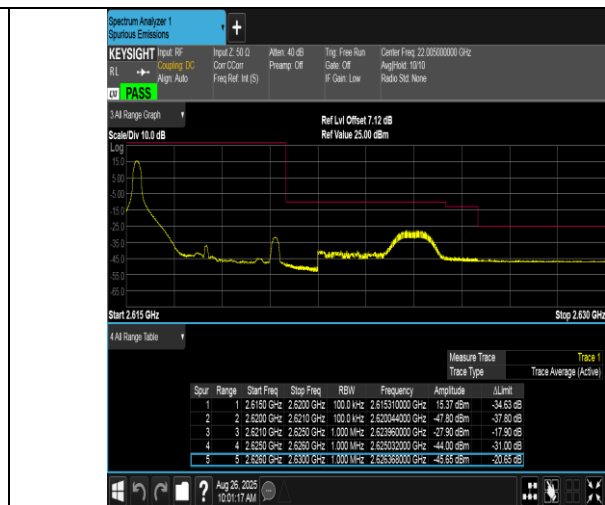
Band38-5MHz-16QAM-38225-1RB#0-PASS
