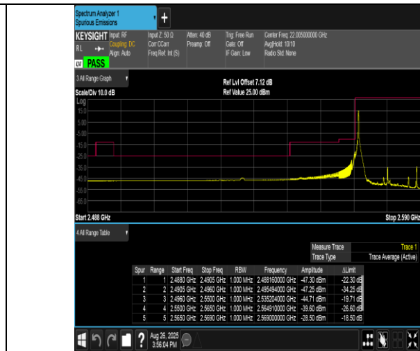
Band38-20MHz-16QAM-37850-1RB#0-PASS
