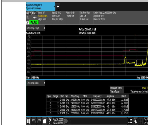
Band38-10MHz-16QAM-37800-1RB#49-PASS
