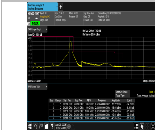
Band38-5MHz-16QAM-38225-1RB#24-PASS
