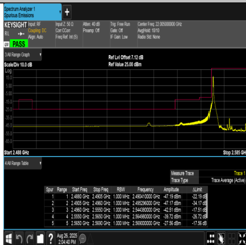
Band38-15MHz-QPSK-37825-1RB#0-PASS
