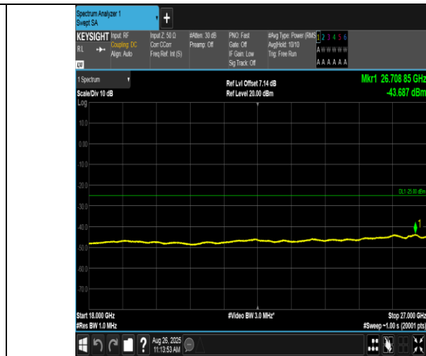
Band38-5MHz-QPSK-37775-1RB#0-18000~27000-PASS
