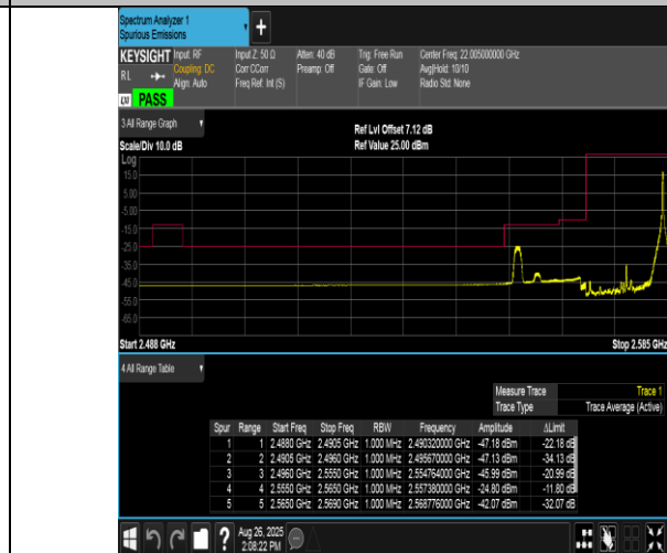
Band38-15MHz-QPSK-37825-1RB#74-PASS
