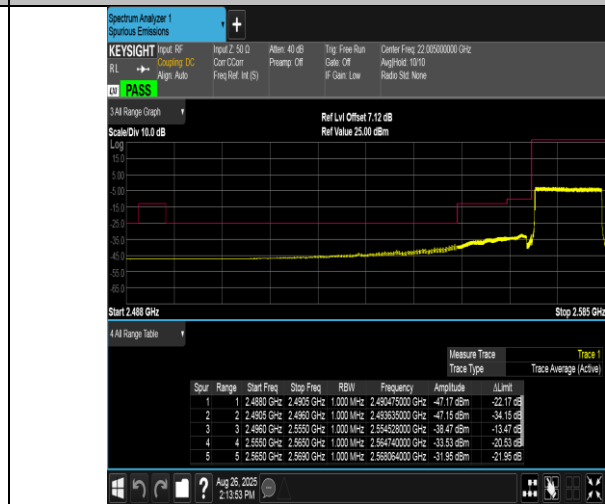
Band38-15MHz-16QAM-37825-75RB#0-PASS
