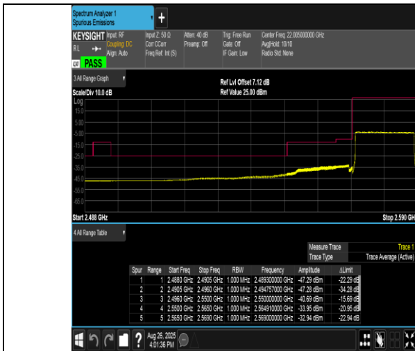
Band38-20MHz-QPSK-37850-100RB#0-PASS
