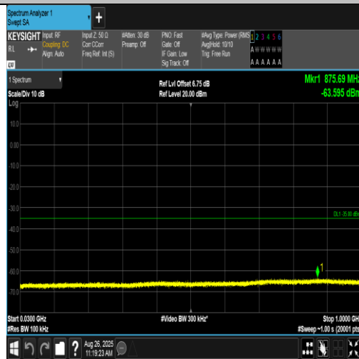
Band38-5MHz-16QAM-37775-1RB#24-30~1000-PASS
