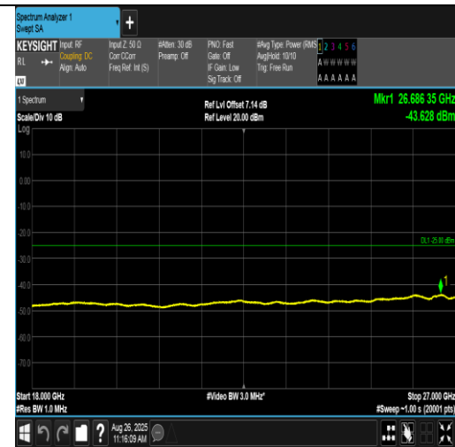
Band38-5MHz-16QAM-37775-1RB#0-18000~27000-PASS
