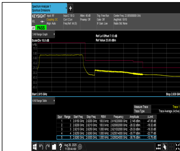
Band38-5MHz-QPSK-38225-25RB#0-PASS
