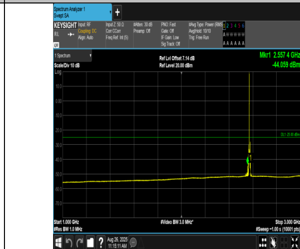
Band38-5MHz-16QAM-37775-1RB#0-1000~3000-PASS
