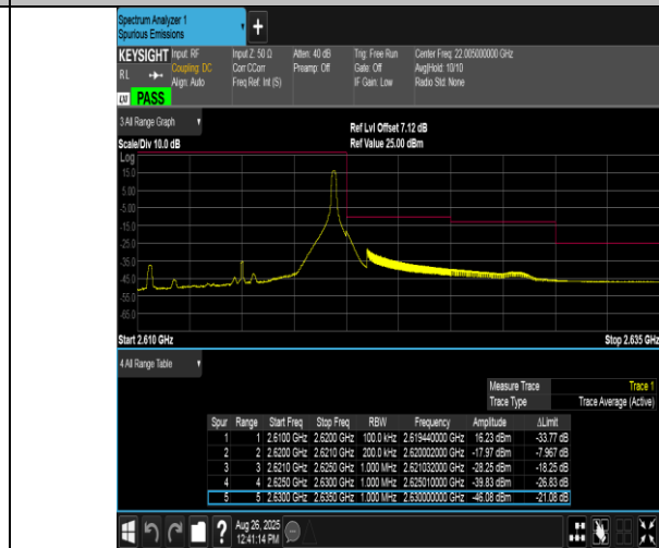
Band38-10MHz-QPSK-38200-1RB#49-PASS
