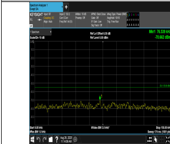
Band38-5MHz-16QAM-37775-1RB#0-0.009~0.15-PASS
