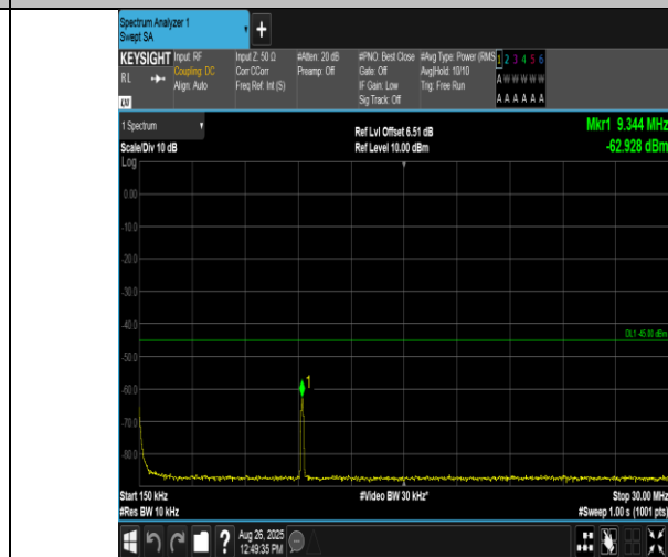
Band38-10MHz-16QAM-37800-1RB#0-0.15~30-PASS
