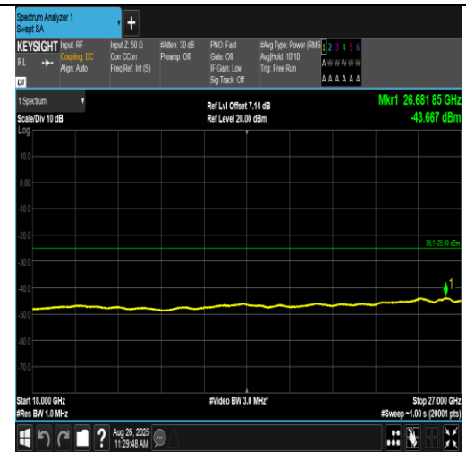
Band38-5MHz-16QAM-38000-1RB#0-18000~27000-PASS
