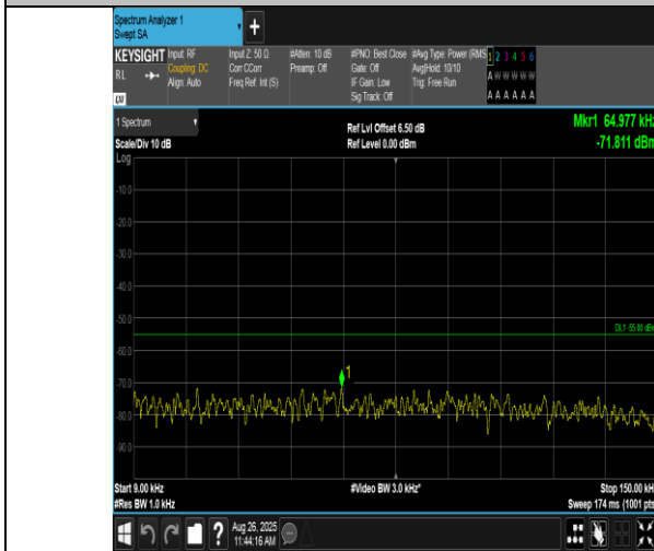
Band38-5MHz-16QAM-38225-1RB#0-0.009~0.15-PASS
