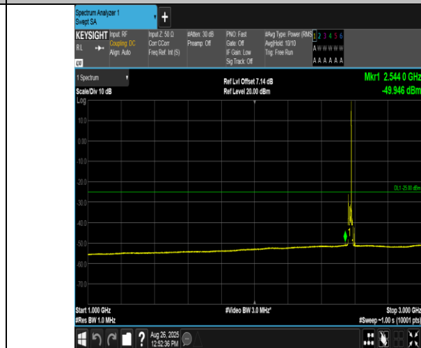
Band38-10MHz-QPSK-37800-1RB#49-1000~3000-PASS
