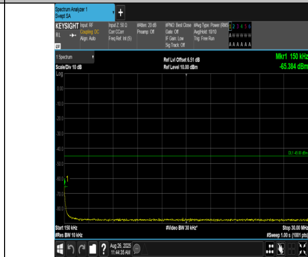
Band38-5MHz-16QAM-38225-1RB#0-0.15~30-PASS
