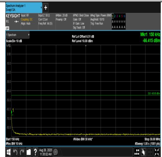
Band38-5MHz-16QAM-38000-1RB#24-0.15~30-PASS
