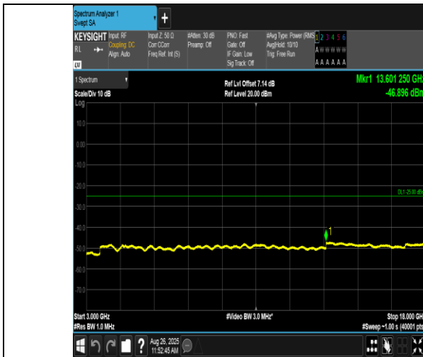
Band38-5MHz-QPSK-38225-25RB#0-3000~18000-PASS
