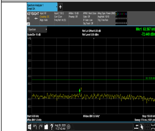
Band38-5MHz-16QAM-38000-1RB#0-0.009~0.15-PASS
