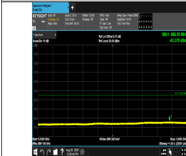
Band38-10MHz-QPSK-37800-50RB#0-30~1000-PASS
