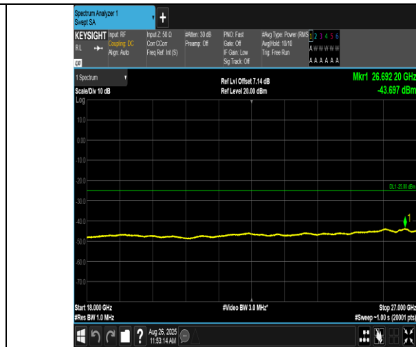
Band38-5MHz-QPSK-38225-25RB#0-18000~27000-PASS
