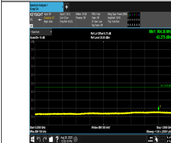
Band38-10MHz-QPSK-37800-1RB#49-30~1000-PASS
