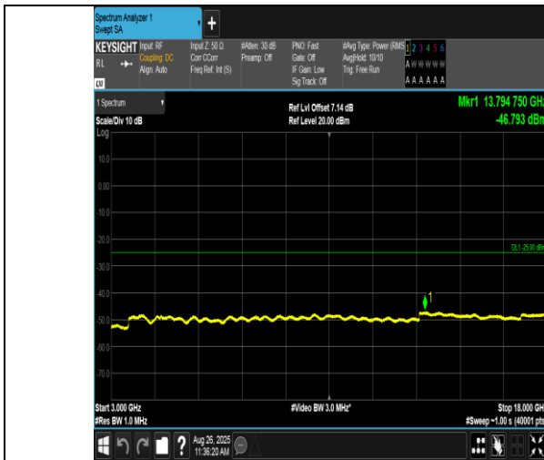
Band38-5MHz-16QAM-38000-1RB#24-3000~18000-PASS
