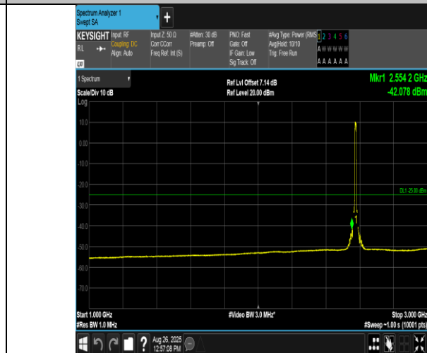
Band38-10MHz-QPSK-37800-50RB#0-1000~3000-PASS
