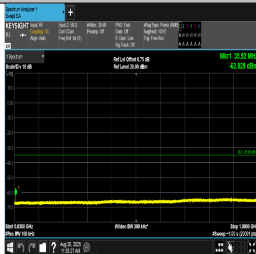
Band38-5MHz-16QAM-38000-1RB#24-30~1000-PASS
