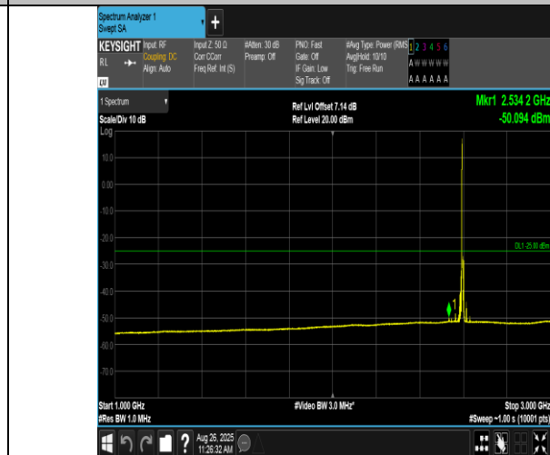
Band38-5MHz-QPSK-38000-1RB#0-1000~3000-PASS
