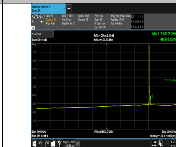
Band38-5MHz-16QAM-38225-1RB#24-1000~3000-PASS
