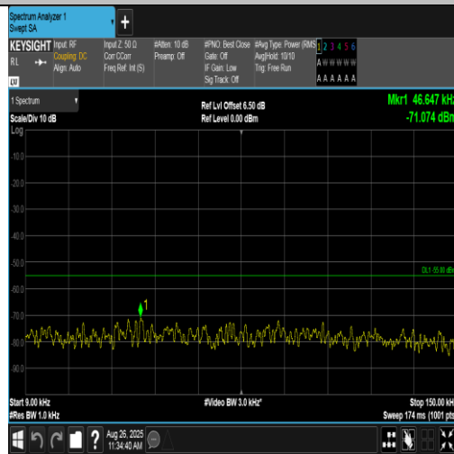
Band38-5MHz-16QAM-38000-1RB#24-0.009~0.15-PASS
