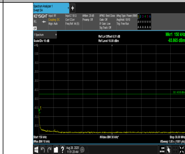
Band38-5MHz-QPSK-38225-25RB#0-0.15~30-PASS
