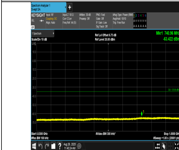
Band38-5MHz-16QAM-38000-25RB#0-30~1000-PASS
