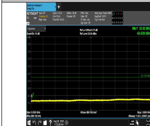
Band38-5MHz-QPSK-38000-1RB#24-30~1000-PASS
