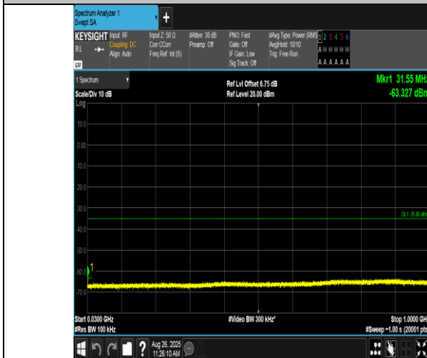
Band38-5MHz-QPSK-38000-1RB#0-30~1000-PASS
