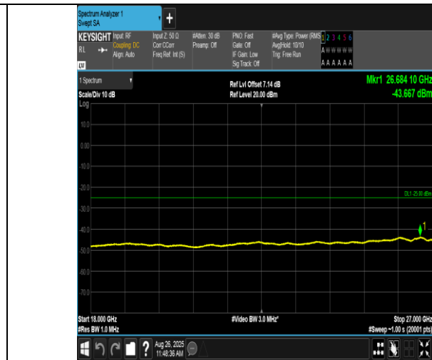
Band38-5MHz-QPSK-38225-1RB#24-18000~27000-PASS
