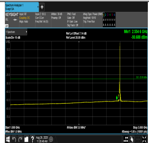
Band38-5MHz-16QAM-38000-1RB#24-1000~3000-PASS
