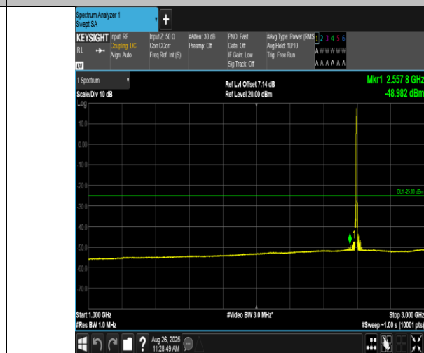
Band38-5MHz-16QAM-38000-1RB#0-1000~3000-PASS
