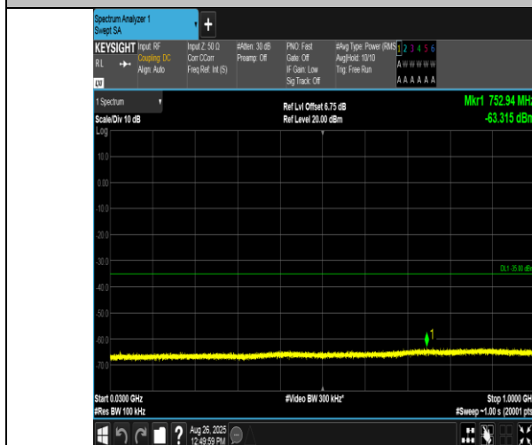
Band38-10MHz-16QAM-37800-1RB#0-30~1000-PASS
