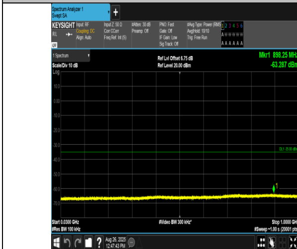
Band38-10MHz-QPSK-37800-1RB#0-30~1000-PASS
