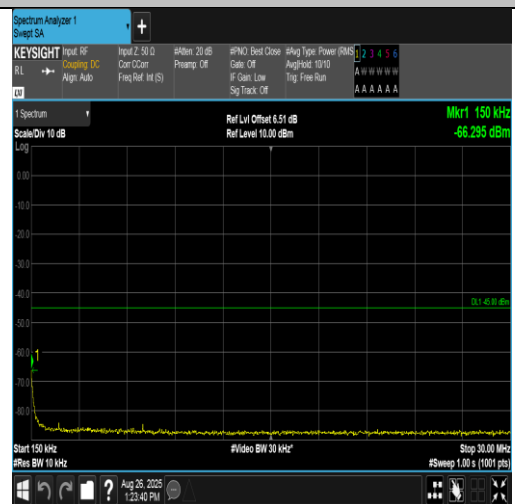
Band38-10MHz-QPSK-38200-50RB#0-0.15~30-PASS
