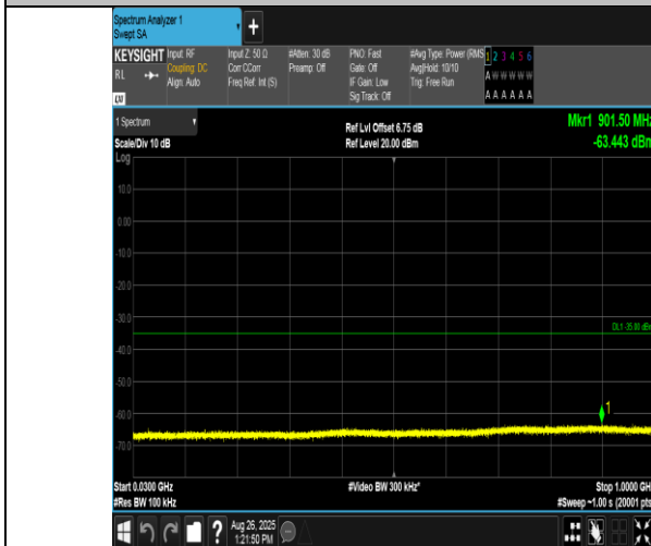
Band38-10MHz-16QAM-38200-1RB#49-30~1000-PASS
