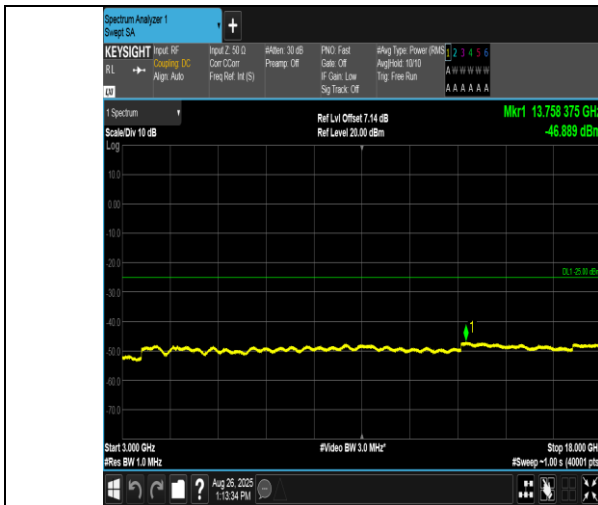
Band38-10MHz-16QAM-38000-50RB#0-3000~18000-PASS
