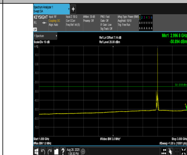
Band38-10MHz-16QAM-38000-1RB#49-1000~3000-PASS
