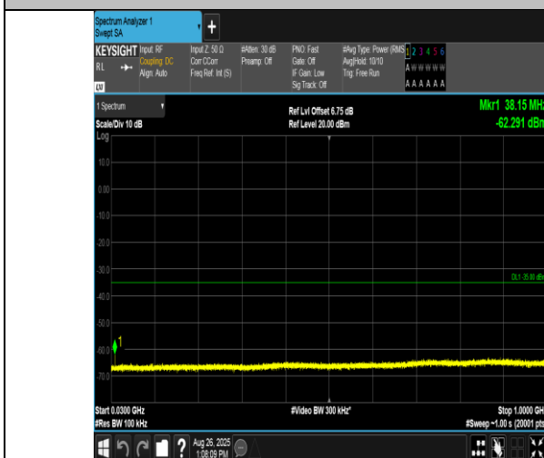
Band38-10MHz-16QAM-38000-1RB#49-30~1000-PASS
