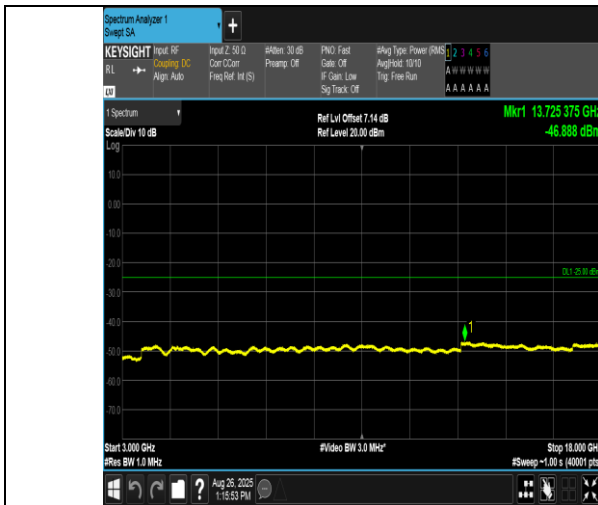
Band38-10MHz-QPSK-38200-1RB#0-3000~18000-PASS
