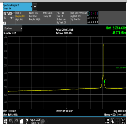
Band38-10MHz-QPSK-38200-50RB#0-1000~3000-PASS
