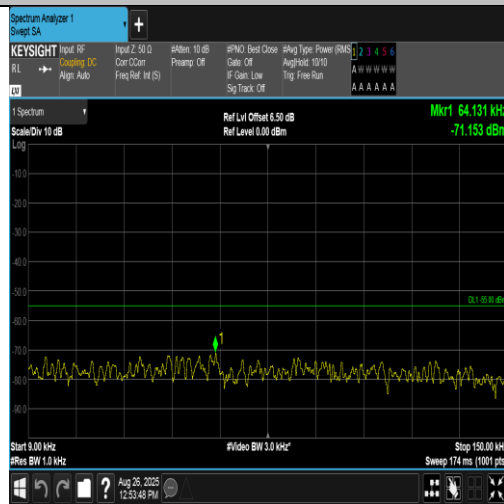
Band38-10MHz-16QAM-37800-1RB#49-0.009~0.15-PASS
