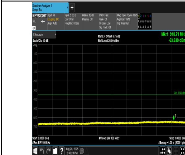
Band38-15MHz-QPSK-37825-1RB#74-30~1000-PASS
