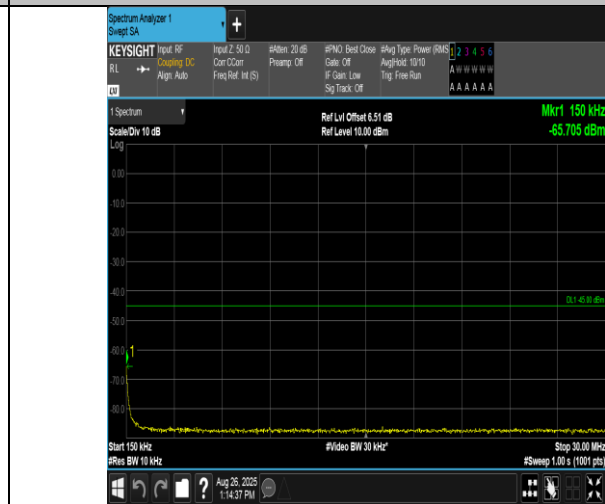
Band38-10MHz-QPSK-38200-1RB#0-0.15~30-PASS
