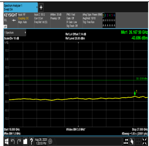
Band38-10MHz-QPSK-38200-1RB#49-18000~27000-PASS
