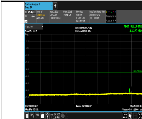
Band38-10MHz-16QAM-38000-50RB#0-30~1000-PASS
