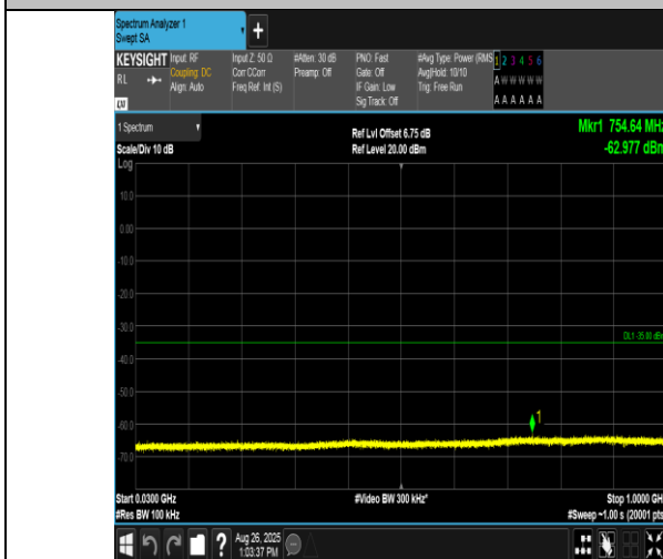
Band38-10MHz-16QAM-38000-1RB#0-30~1000-PASS
