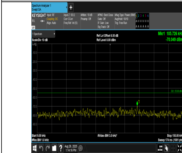
Band38-10MHz-QPSK-38200-1RB#0-0.009~0.15-PASS
