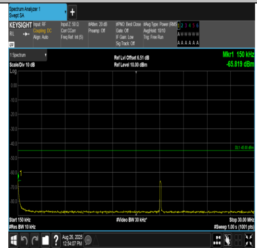
Band38-10MHz-16QAM-37800-1RB#49-0.15~30-PASS
