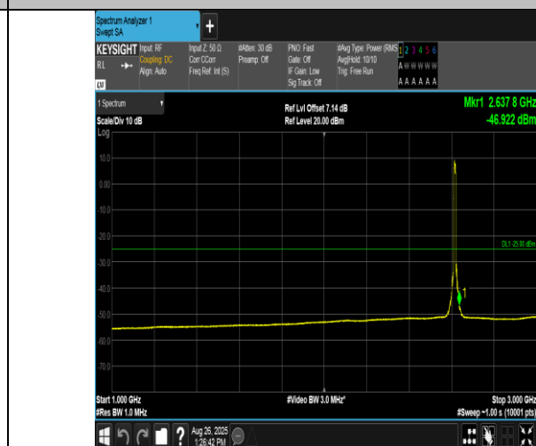
Band38-10MHz-16QAM-38200-50RB#0-1000~3000-PASS
