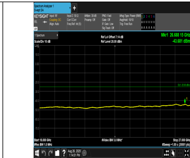
Band38-10MHz-16QAM-38000-50RB#0-18000~27000-PASS
