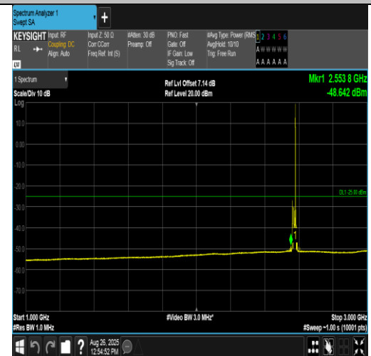
Band38-10MHz-16QAM-37800-1RB#49-1000~3000-PASS
