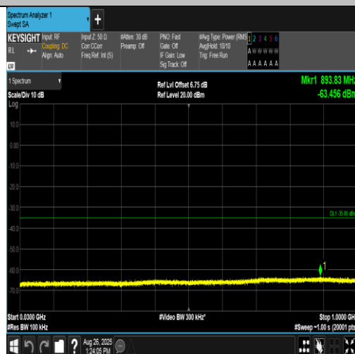
Band38-10MHz-QPSK-38200-50RB#0-30~1000-PASS
