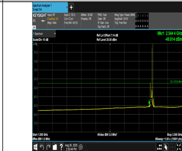
Band38-15MHz-QPSK-37825-1RB#74-1000~3000-PASS
