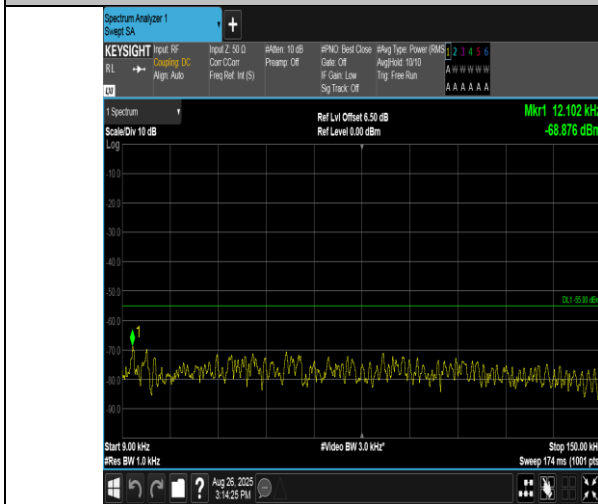
Band38-15MHz-16QAM-38175-1RB#0-0.009~0.15-PASS
