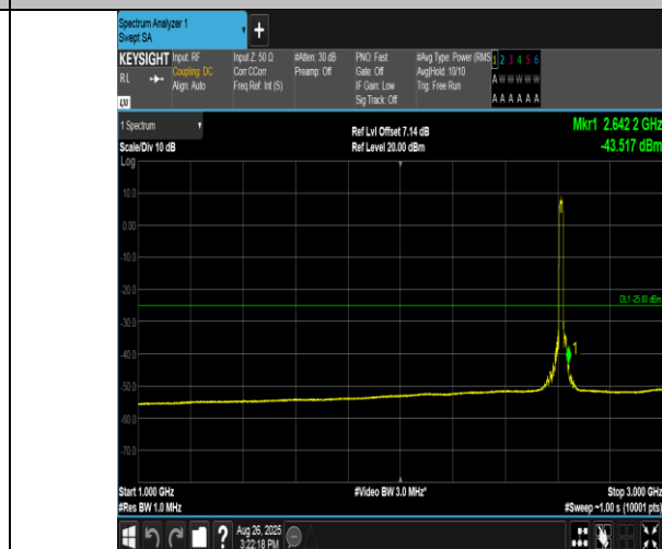
Band38-15MHz-QPSK-38175-75RB#0-1000~3000-PASS
