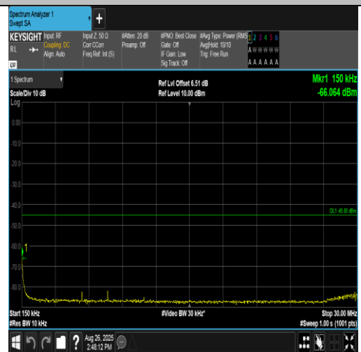
Band38-15MHz-QPSK-38000-75RB#0-0.15~30-PASS
