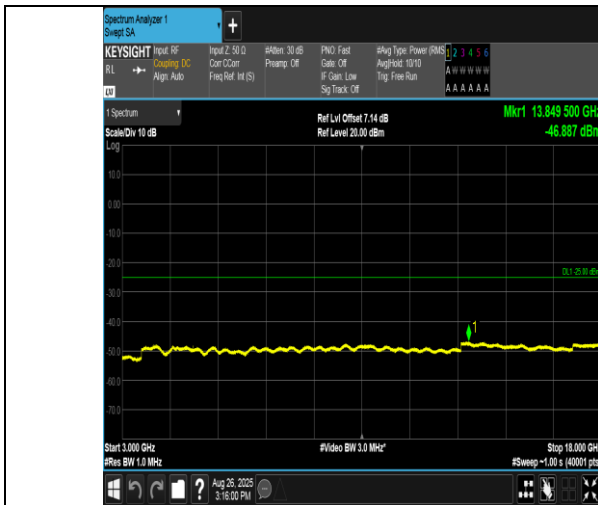
Band38-15MHz-16QAM-38175-1RB#0-3000~18000-PASS
