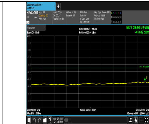
Band38-15MHz-16QAM-38000-1RB#74-18000~27000-PASS
