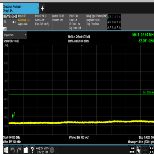
Band38-15MHz-QPSK-38175-1RB#74-30~1000-PASS
