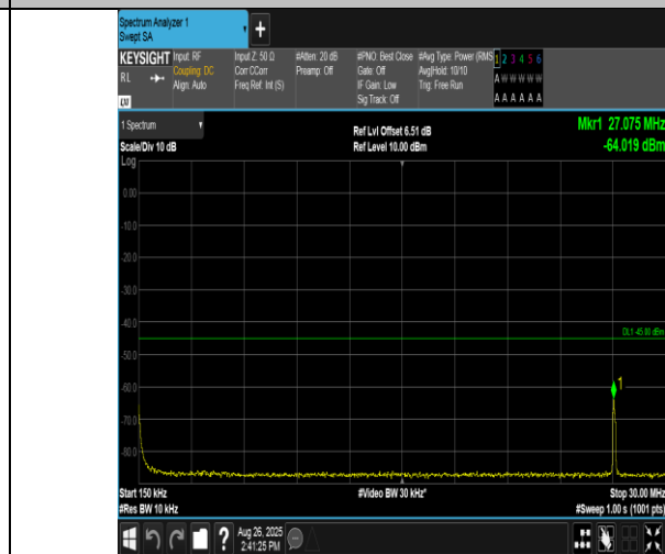
Band38-15MHz-16QAM-38000-1RB#0-0.15~30-PASS
