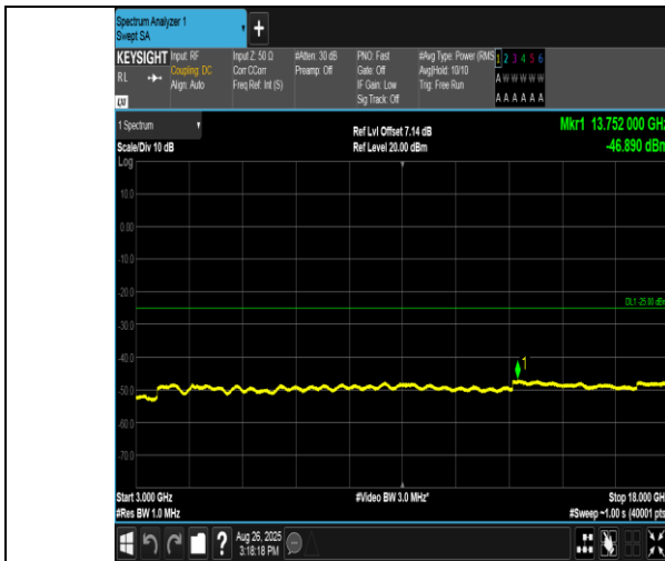
Band38-15MHz-QPSK-38175-1RB#74-3000~18000-PASS
