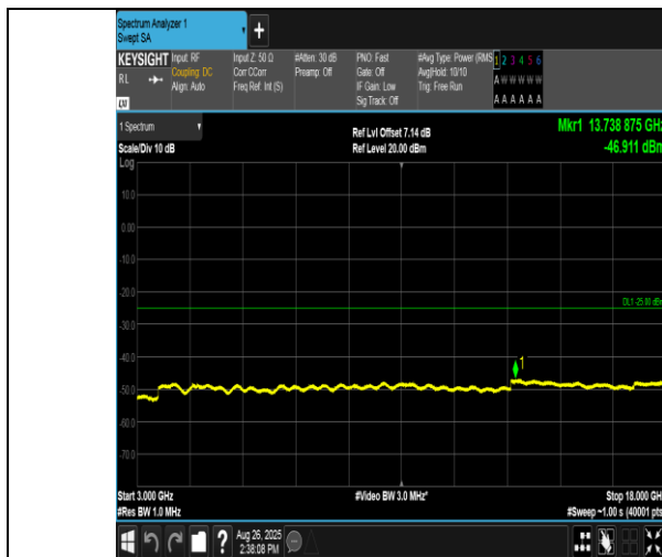
Band38-15MHz-16QAM-37825-75RB#0-3000~18000-PASS
