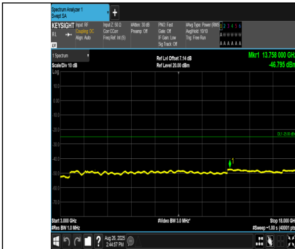
Band38-15MHz-QPSK-38000-1RB#74-3000~18000-PASS
