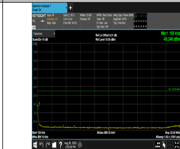
Band38-15MHz-16QAM-38000-75RB#0-0.15~30-PASS
