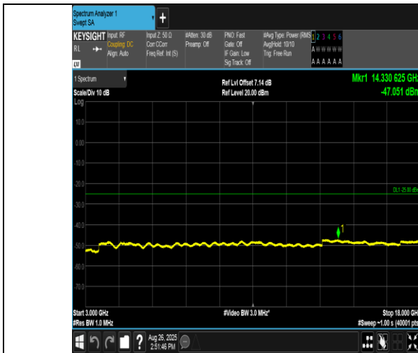
Band38-15MHz-16QAM-38000-75RB#0-3000~18000-PASS
