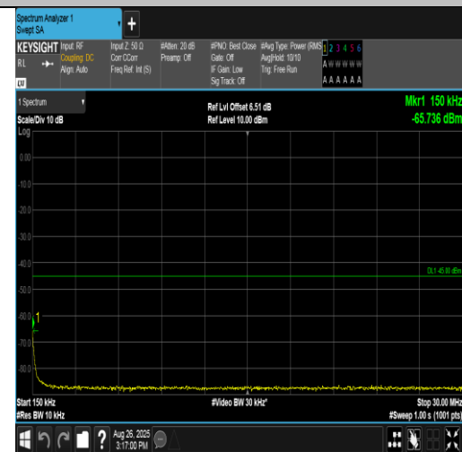
Band38-15MHz-QPSK-38175-1RB#74-0.15~30-PASS
