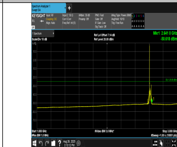
Band38-15MHz-QPSK-38175-1RB#0-1000~3000-PASS
