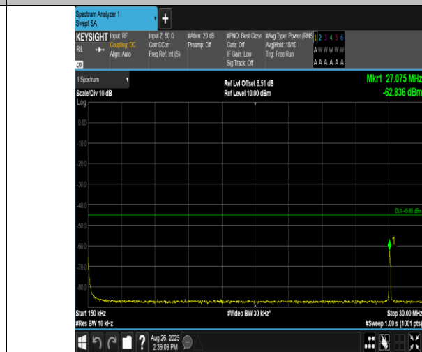
Band38-15MHz-QPSK-38000-1RB#0-0.15~30-PASS
