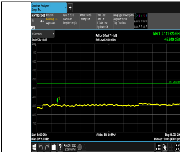
Band38-15MHz-16QAM-37825-1RB#0-3000~18000-PASS
