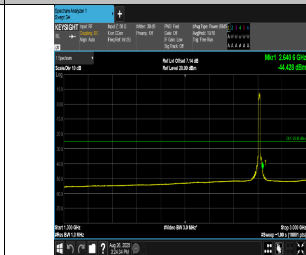
Band38-15MHz-16QAM-38175-75RB#0-1000~3000-PASS
