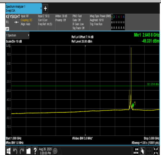
Band38-15MHz-16QAM-38175-1RB#74-1000~3000-PASS
