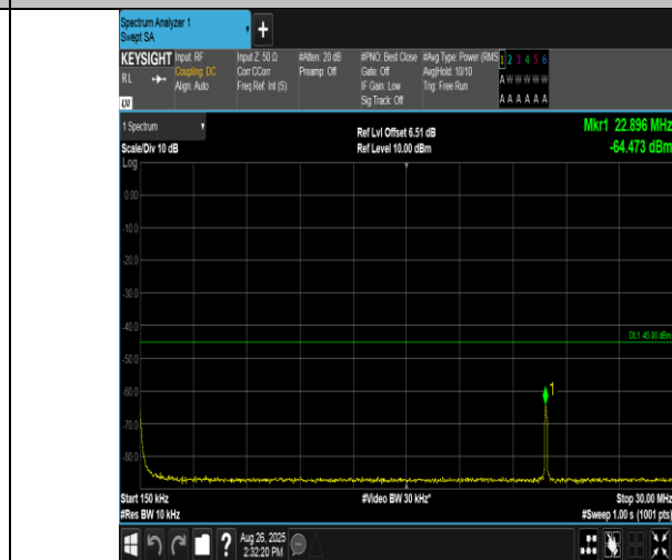
Band38-15MHz-16QAM-37825-1RB#74-0.15~30-PASS
