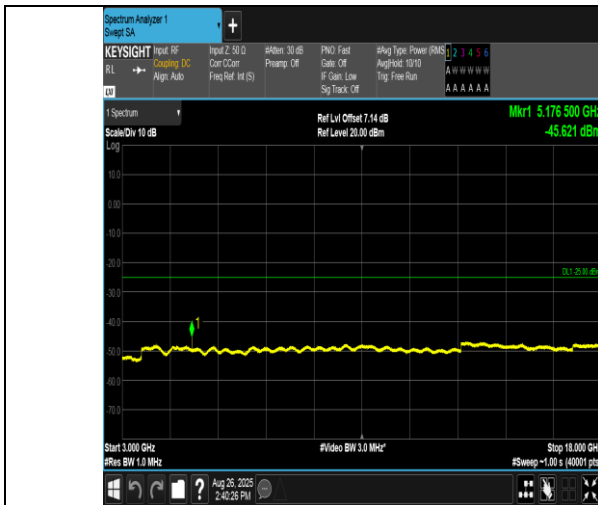
Band38-15MHz-QPSK-38000-1RB#0-3000~18000-PASS
