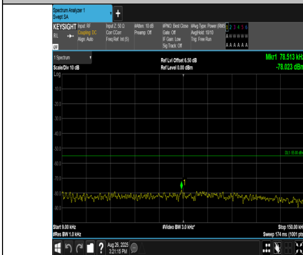
Band38-15MHz-QPSK-38175-75RB#0-0.009~0.15-PASS
