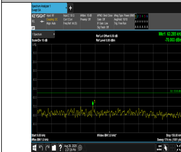
Band38-15MHz-16QAM-37825-1RB#0-0.009~0.15-PASS
