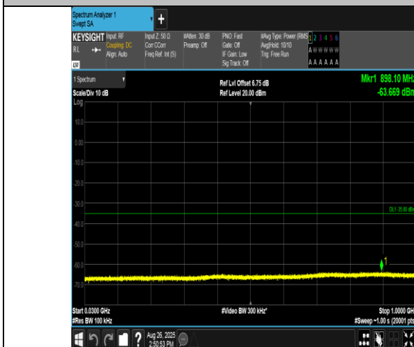
Band38-15MHz-16QAM-38000-75RB#0-30~1000-PASS
