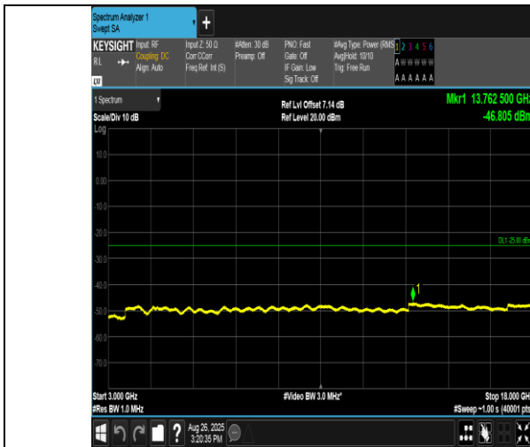
Band38-15MHz-16QAM-38175-1RB#74-3000~18000-PASS
