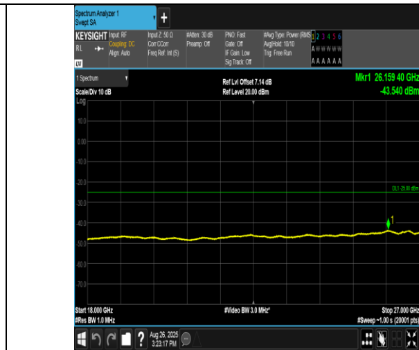
Band38-15MHz-QPSK-38175-75RB#0-18000~27000-PASS
