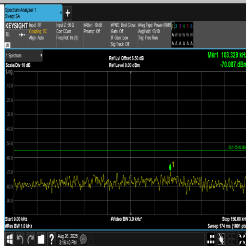
Band38-15MHz-QPSK-38175-1RB#74-0.009~0.15-PASS
