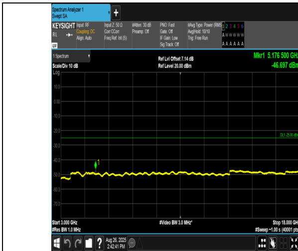
Band38-15MHz-16QAM-38000-1RB#0-3000~18000-PASS
