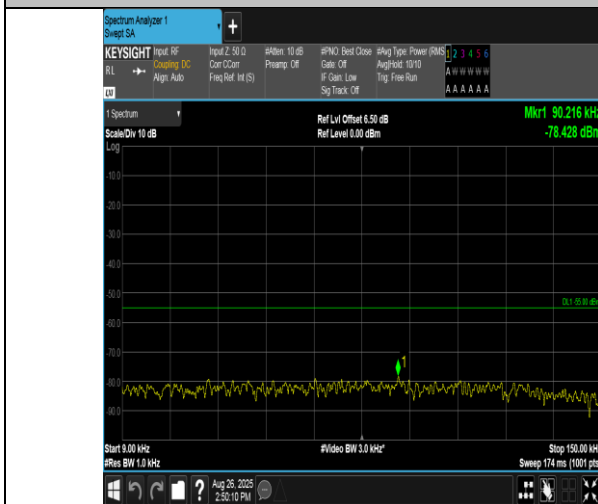
Band38-15MHz-16QAM-38000-75RB#0-0.009~0.15-PASS
