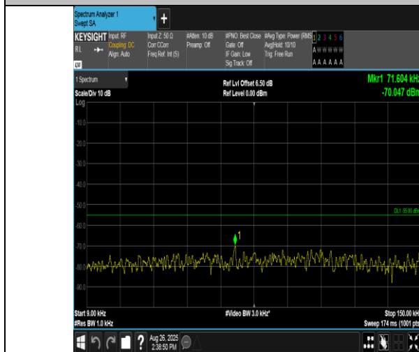
Band38-15MHz-QPSK-38000-1RB#0-0.009~0.15-PASS
