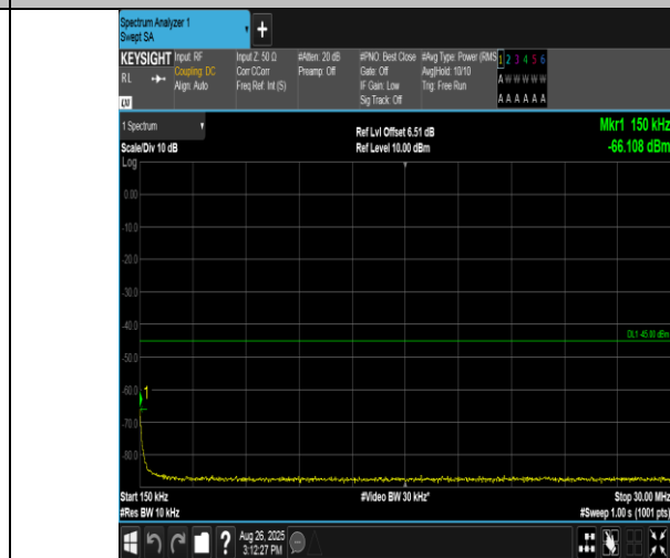
Band38-15MHz-QPSK-38175-1RB#0-0.15~30-PASS
