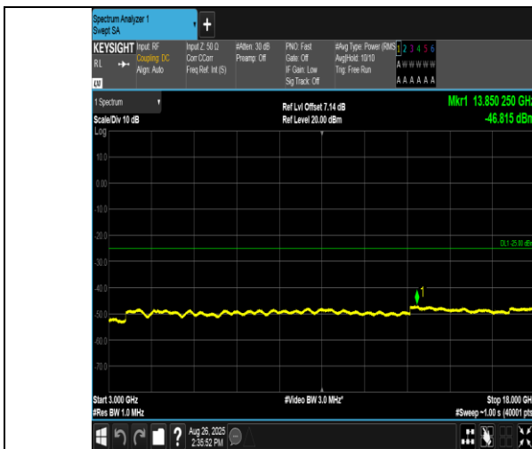
Band38-15MHz-QPSK-37825-75RB#0-3000~18000-PASS
