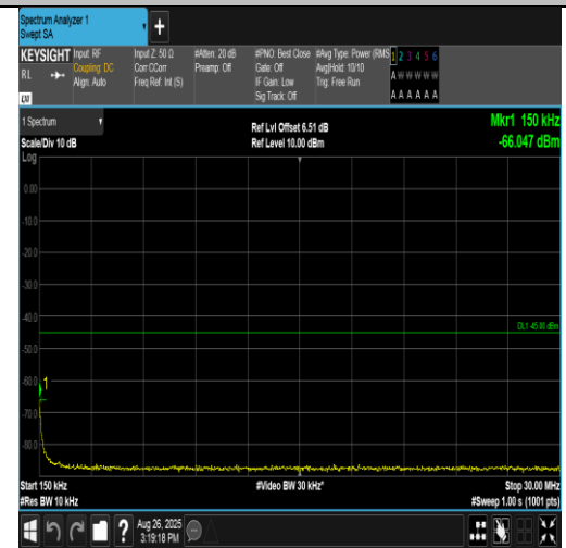
Band38-15MHz-16QAM-38175-1RB#74-0.15~30-PASS
