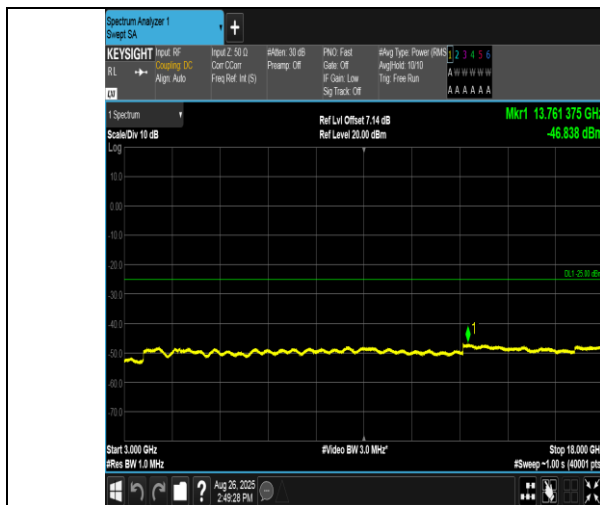
Band38-15MHz-QPSK-38000-75RB#0-3000~18000-PASS
