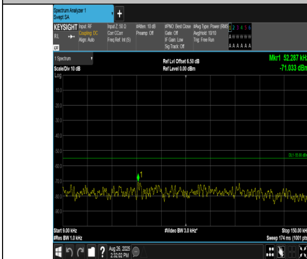
Band38-15MHz-16QAM-37825-1RB#74-0.009~0.15-PASS
