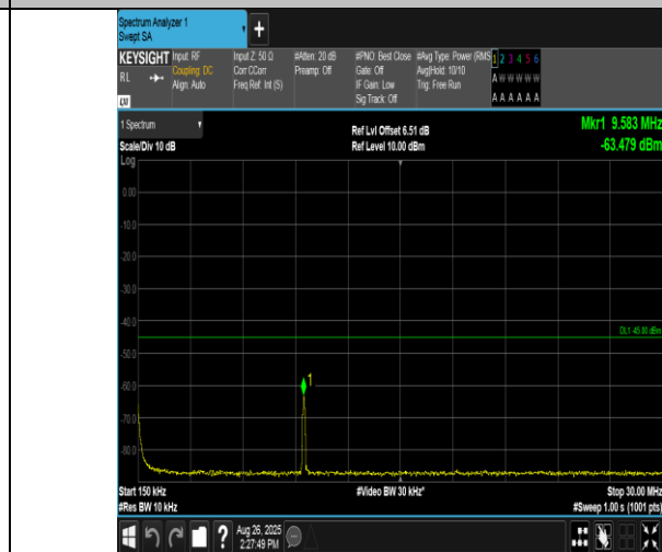
Band38-15MHz-16QAM-37825-1RB#0-0.15~30-PASS
