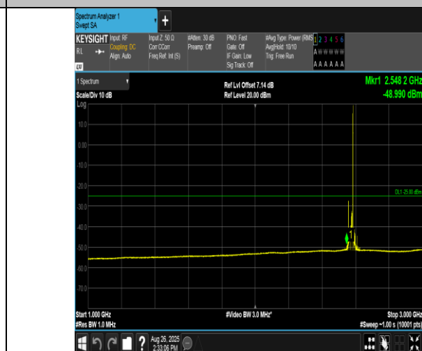
Band38-15MHz-16QAM-37825-1RB#74-1000~3000-PASS
