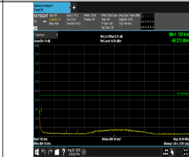
Band38-15MHz-16QAM-37825-75RB#0-0.15~30-PASS
