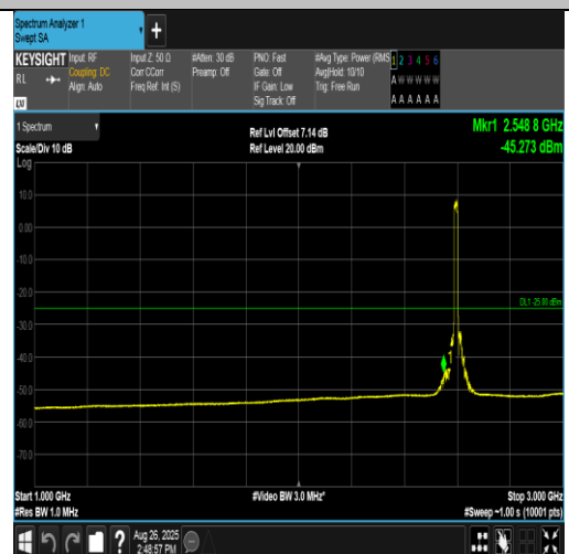
Band38-15MHz-QPSK-38000-75RB#0-1000~3000-PASS
