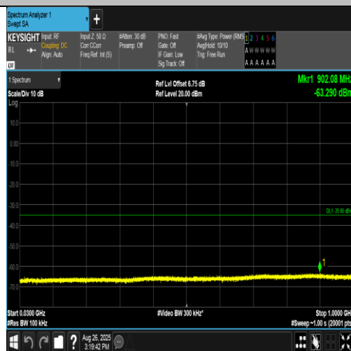
Band38-15MHz-16QAM-38175-1RB#74-30~1000-PASS
