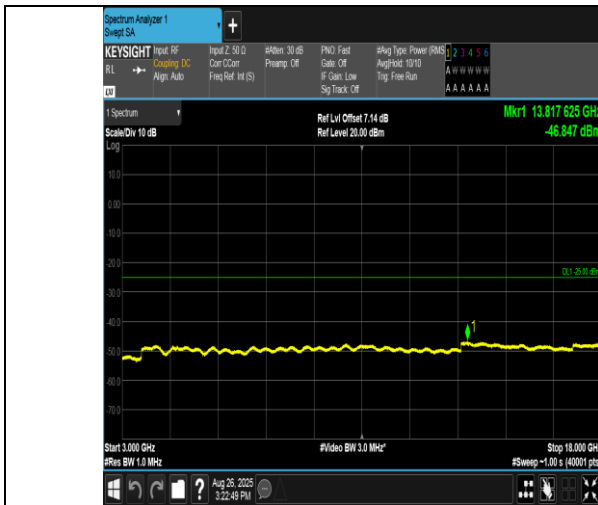
Band38-15MHz-QPSK-38175-75RB#0-3000~18000-PASS
