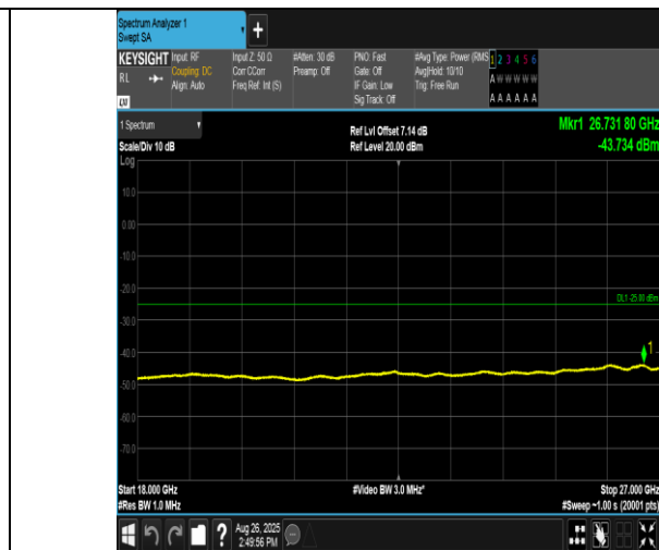
Band38-15MHz-QPSK-38000-75RB#0-18000~27000-PASS
