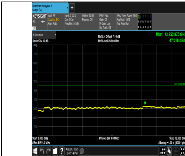
Band38-15MHz-16QAM-38000-1RB#74-3000~18000-PASS
