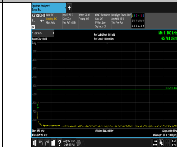
Band38-15MHz-16QAM-38000-1RB#74-0.15~30-PASS
