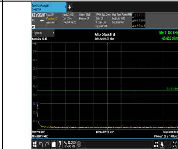
Band38-15MHz-16QAM-38175-1RB#0-0.15~30-PASS
