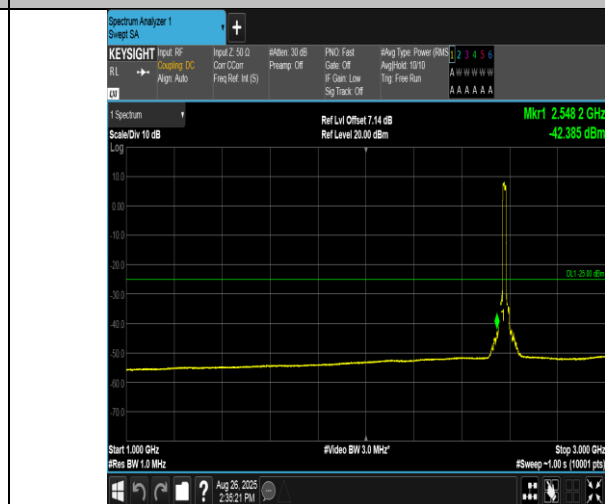
Band38-15MHz-QPSK-37825-75RB#0-1000~3000-PASS
