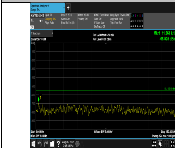
Band38-15MHz-16QAM-38000-1RB#74-0.009~0.15-PASS
