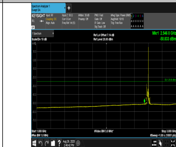
Band38-15MHz-16QAM-38000-1RB#74-1000~3000-PASS
