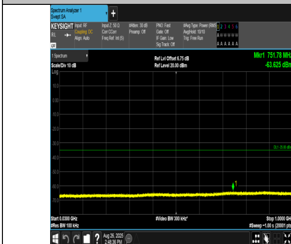
Band38-15MHz-QPSK-38000-75RB#0-30~1000-PASS
