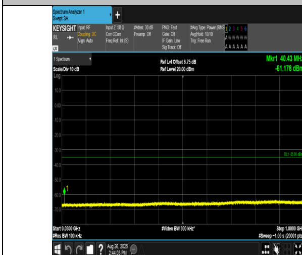
Band38-15MHz-QPSK-38000-1RB#74-30~1000-PASS
