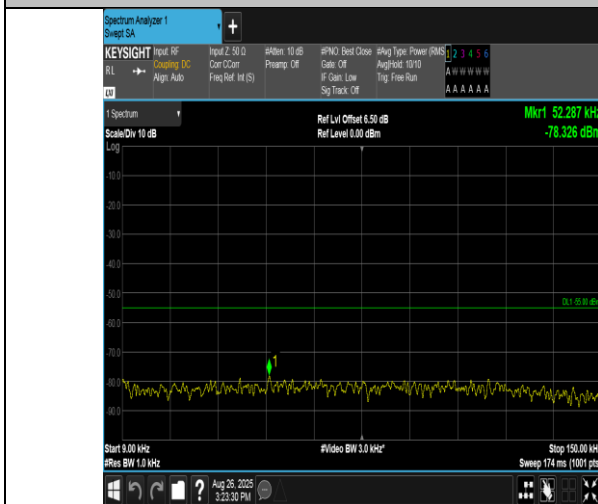
Band38-15MHz-16QAM-38175-75RB#0-0.009~0.15-PASS
