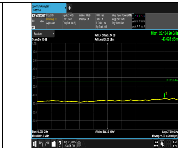
Band38-15MHz-16QAM-37825-75RB#0-18000~27000-PASS
