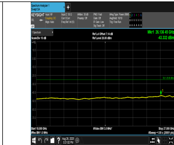
Band38-15MHz-16QAM-38175-1RB#74-18000~27000-PASS
