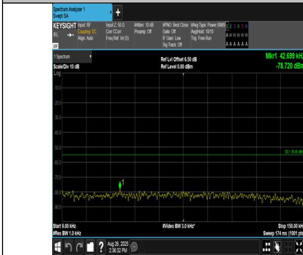
Band38-15MHz-16QAM-37825-75RB#0-0.009~0.15-PASS
