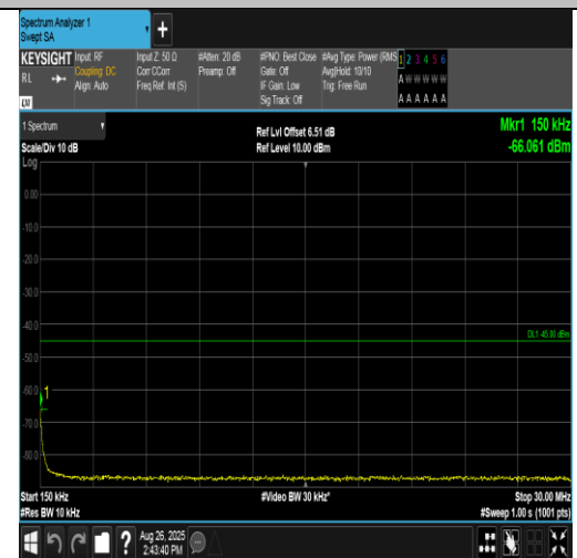
Band38-15MHz-QPSK-38000-1RB#74-0.15~30-PASS
