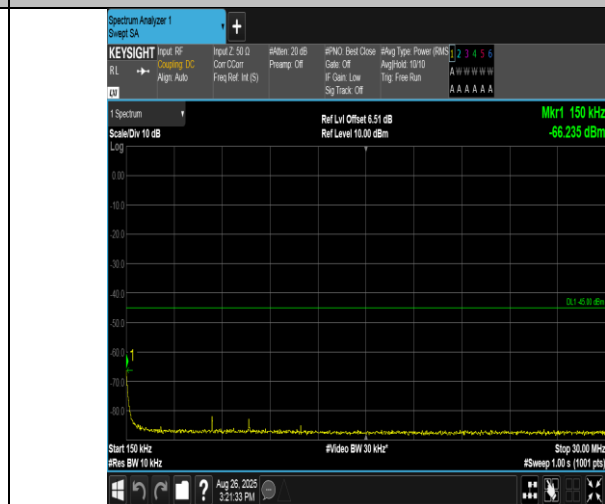
Band38-15MHz-QPSK-38175-75RB#0-0.15~30-PASS
