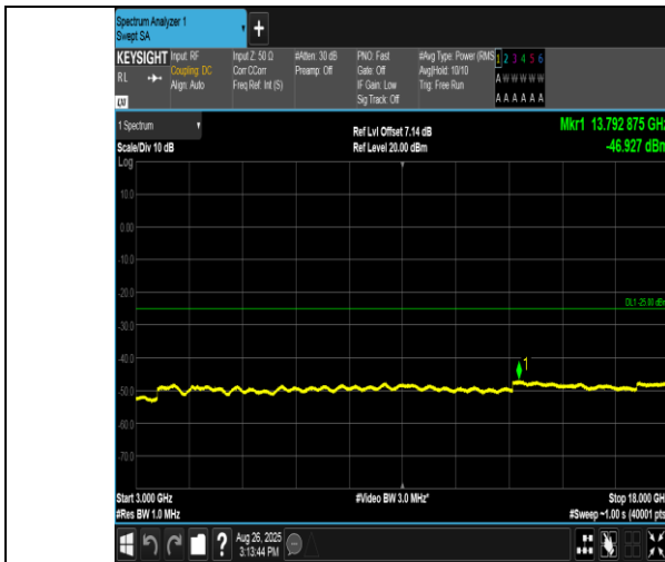
Band38-15MHz-QPSK-38175-1RB#0-3000~18000-PASS
