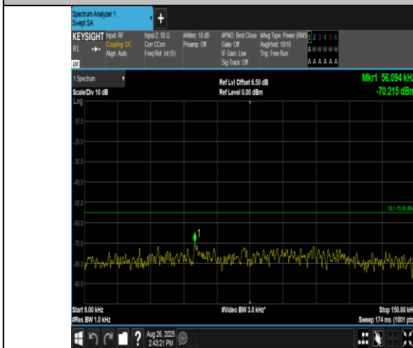
Band38-15MHz-QPSK-38000-1RB#74-0.009~0.15-PASS
