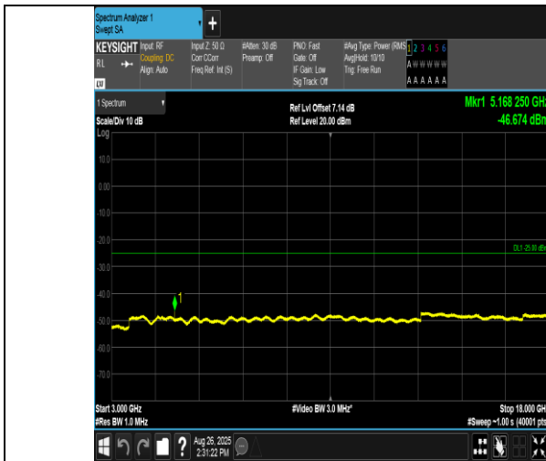
Band38-15MHz-QPSK-37825-1RB#74-3000~18000-PASS
