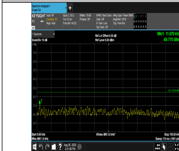
Band38-15MHz-16QAM-38000-1RB#0-0.009~0.15-PASS
