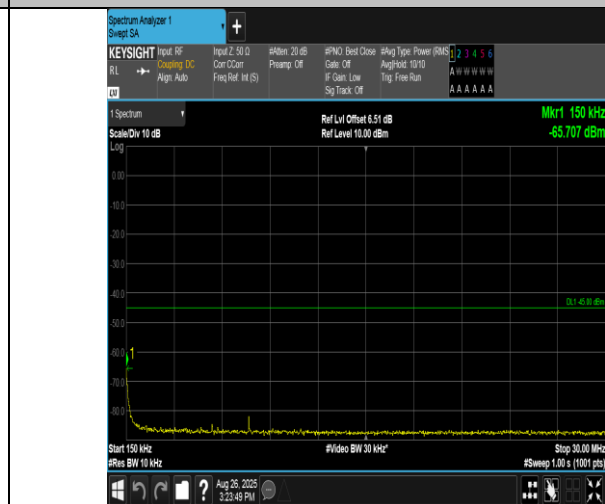
Band38-15MHz-16QAM-38175-75RB#0-0.15~30-PASS
