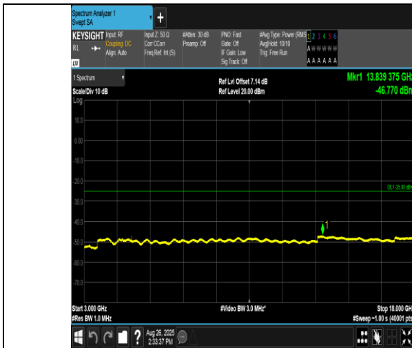
Band38-15MHz-16QAM-37825-1RB#74-3000~18000-PASS
