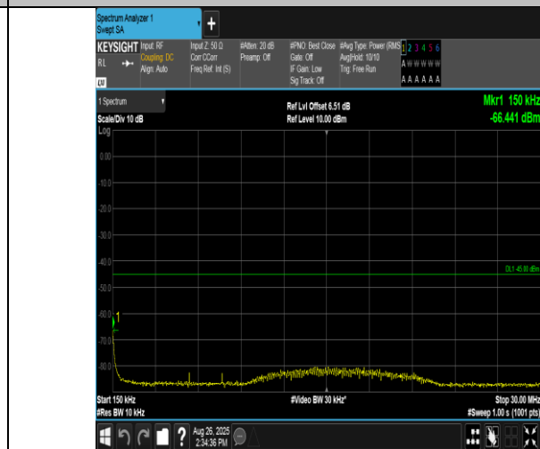
Band38-15MHz-QPSK-37825-75RB#0-0.15~30-PASS
