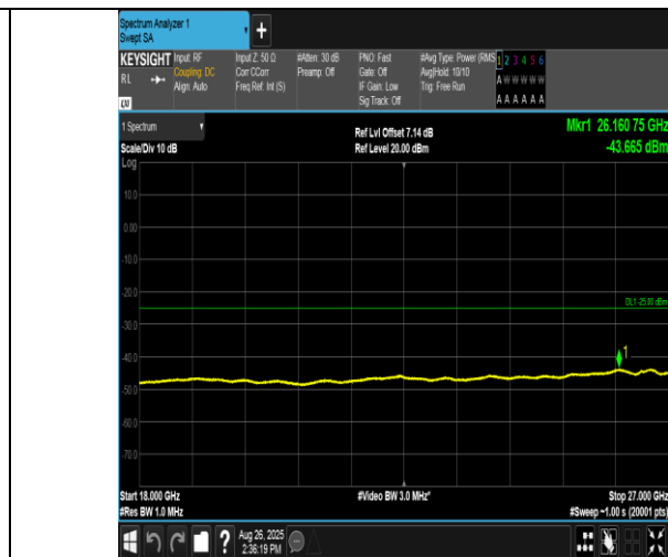
Band38-15MHz-QPSK-37825-75RB#0-18000~27000-PASS
