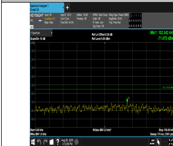
Band38-15MHz-QPSK-38175-1RB#0-0.009~0.15-PASS
