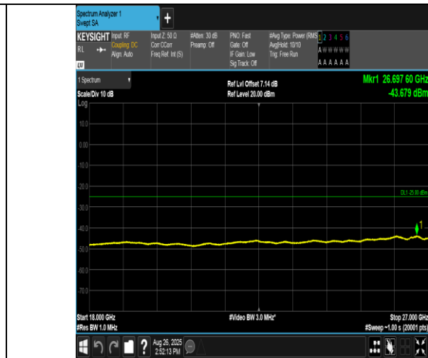
Band38-15MHz-16QAM-38000-75RB#0-18000~27000-PASS
