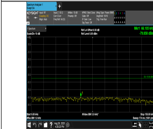
Band38-20MHz-16QAM-37850-100RB#0-0.009~0.15-PASS
