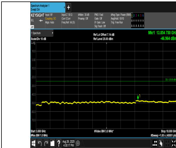
Band38-20MHz-QPSK-38000-1RB#0-3000~18000-PASS
