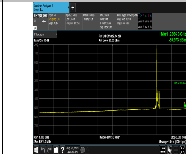
Band38-20MHz-16QAM-38150-1RB#0-1000~3000-PASS
