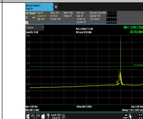
Band38-20MHz-16QAM-38000-1RB#99-1000~3000-PASS
