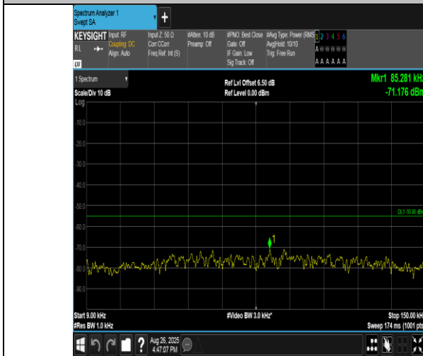
Band38-20MHz-QPSK-38150-1RB#99-0.009~0.15-PASS
