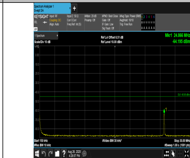
Band38-20MHz-QPSK-38000-1RB#0-0.15~30-PASS
