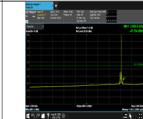
Band38-20MHz-QPSK-38150-1RB#99-1000~3000-PASS
