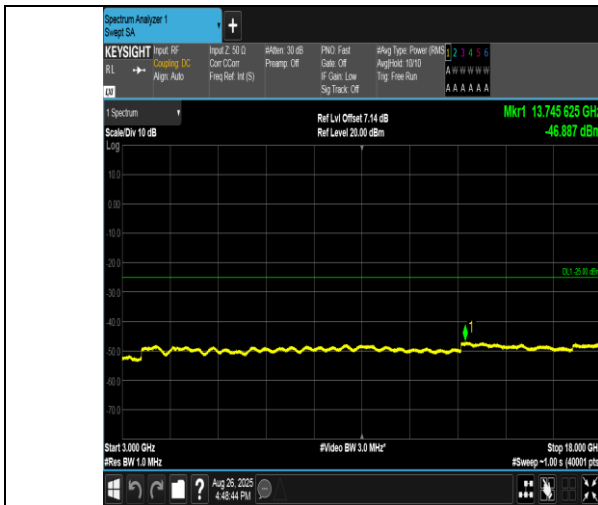
Band38-20MHz-QPSK-38150-1RB#99-3000~18000-PASS
