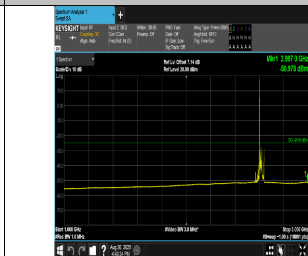
Band38-20MHz-QPSK-38150-1RB#0-1000~3000-PASS
