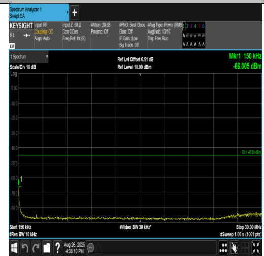
Band38-20MHz-QPSK-38000-100RB#0-0.15~30-PASS
