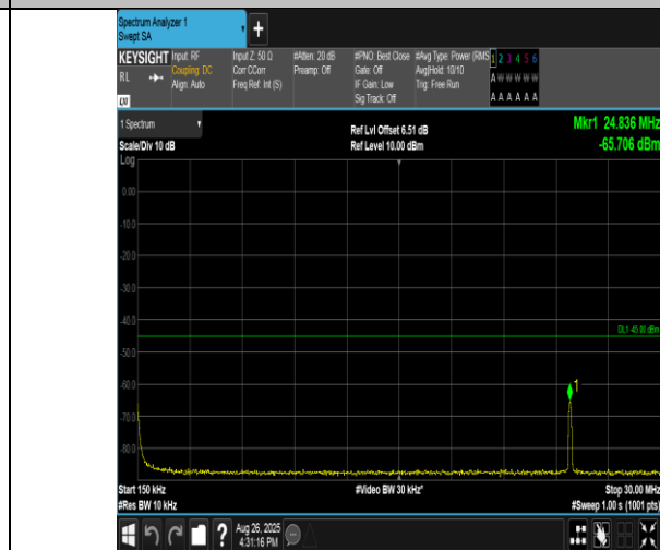
Band38-20MHz-16QAM-38000-1RB#0-0.15~30-PASS
