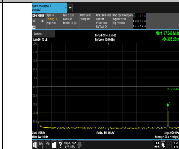
Band38-20MHz-16QAM-37850-1RB#99-0.15~30-PASS
