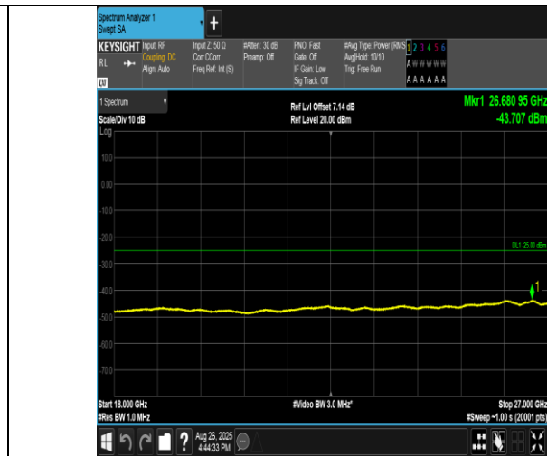
Band38-20MHz-QPSK-38150-1RB#0-18000~27000-PASS
