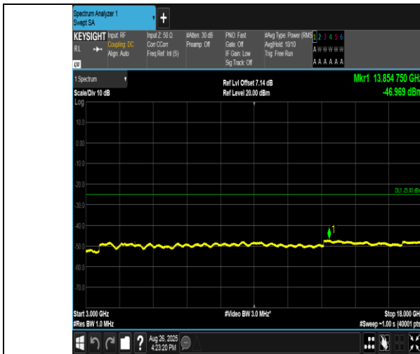
Band38-20MHz-16QAM-37850-1RB#99-3000~18000-PASS
