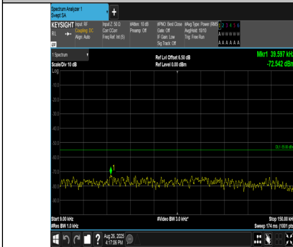
Band38-20MHz-16QAM-37850-1RB#0-0.009~0.15-PASS
