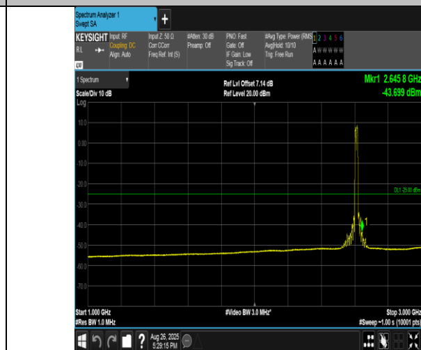
Band38-20MHz-QPSK-38150-100RB#0-1000~3000-PASS
