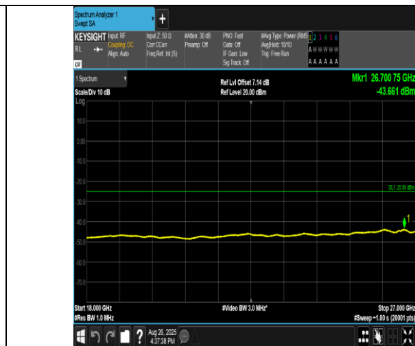
Band38-20MHz-16QAM-38000-1RB#99-18000~27000-PASS
