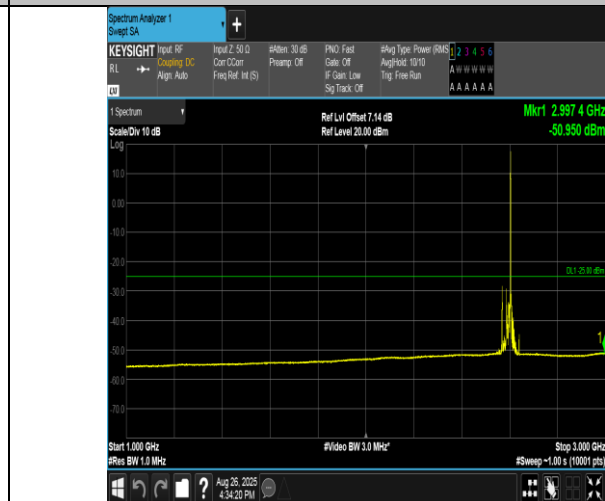
Band38-20MHz-QPSK-38000-1RB#99-1000~3000-PASS
