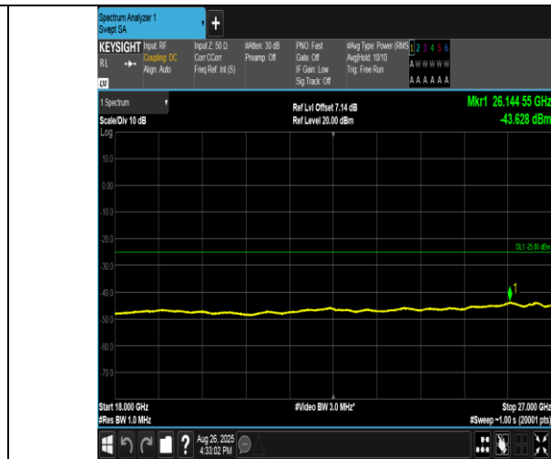
Band38-20MHz-16QAM-38000-1RB#0-18000~27000-PASS
