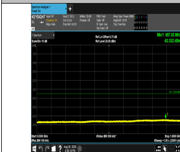
Band38-20MHz-16QAM-38000-1RB#99-30~1000-PASS
