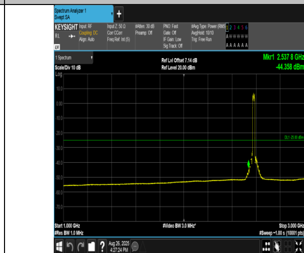
Band38-20MHz-16QAM-37850-100RB#0-1000~3000-PASS
