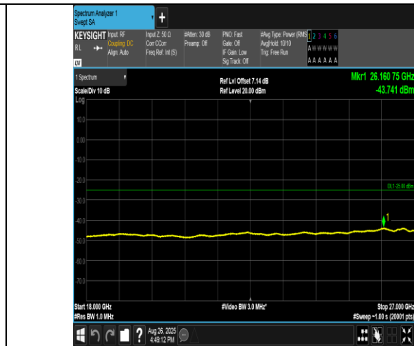
Band38-20MHz-QPSK-38150-1RB#99-18000~27000-PASS
