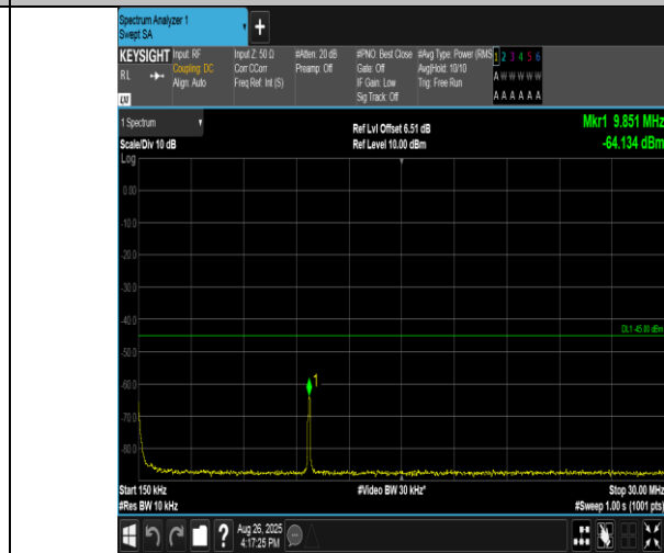
Band38-20MHz-16QAM-37850-1RB#0-0.15~30-PASS
