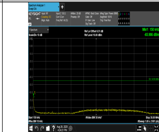
Band38-20MHz-QPSK-37850-100RB#0-0.15~30-PASS
