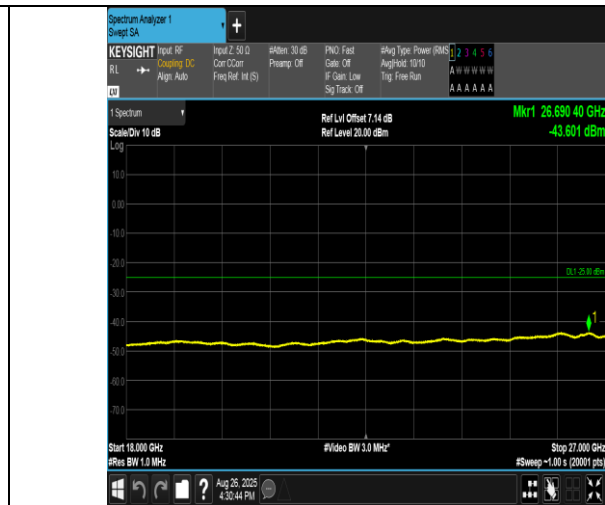
Band38-20MHz-QPSK-38000-1RB#0-18000~27000-PASS
