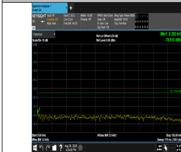
Band38-20MHz-QPSK-37850-100RB#0-0.009~0.15-PASS
