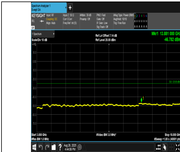
Band38-20MHz-QPSK-38150-1RB#0-3000~18000-PASS
