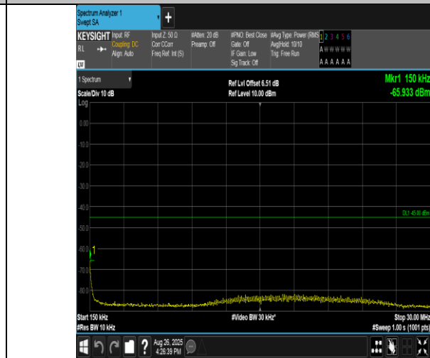
Band38-20MHz-16QAM-37850-100RB#0-0.15~30-PASS
