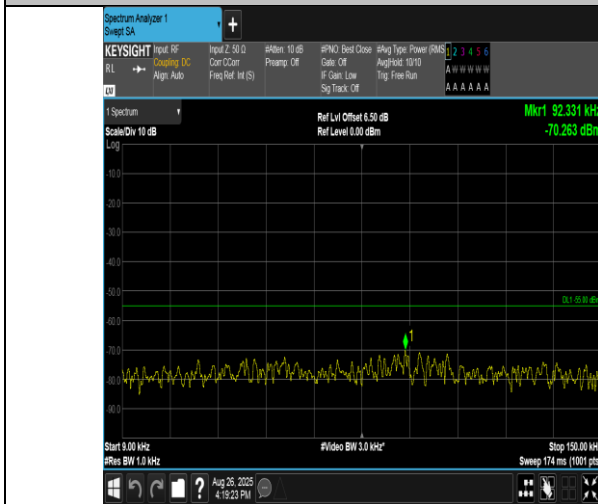
Band38-20MHz-QPSK-37850-1RB#99-0.009~0.15-PASS
