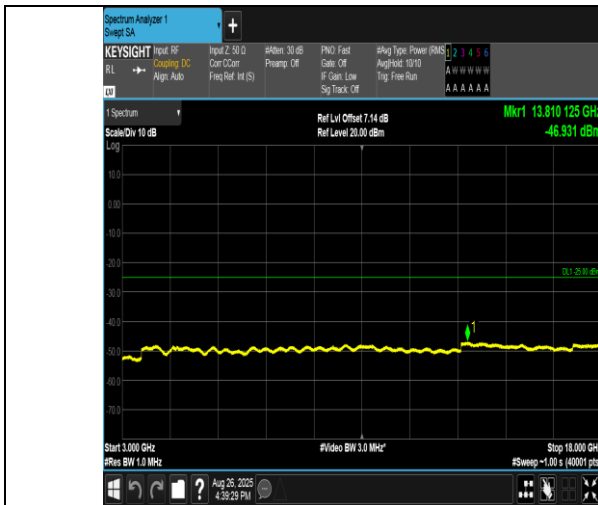
Band38-20MHz-QPSK-38000-100RB#0-3000~18000-PASS
