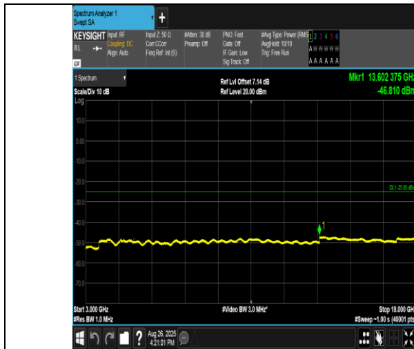
Band38-20MHz-QPSK-37850-1RB#99-3000~18000-PASS
