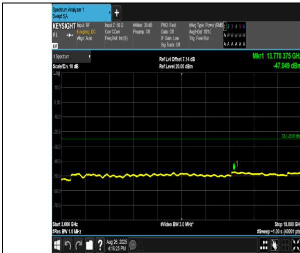
Band38-20MHz-QPSK-37850-1RB#0-3000~18000-PASS
