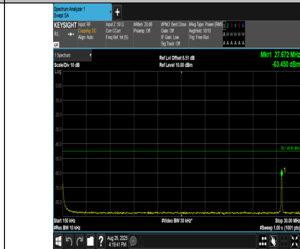
Band38-20MHz-QPSK-37850-1RB#99-0.15~30-PASS
