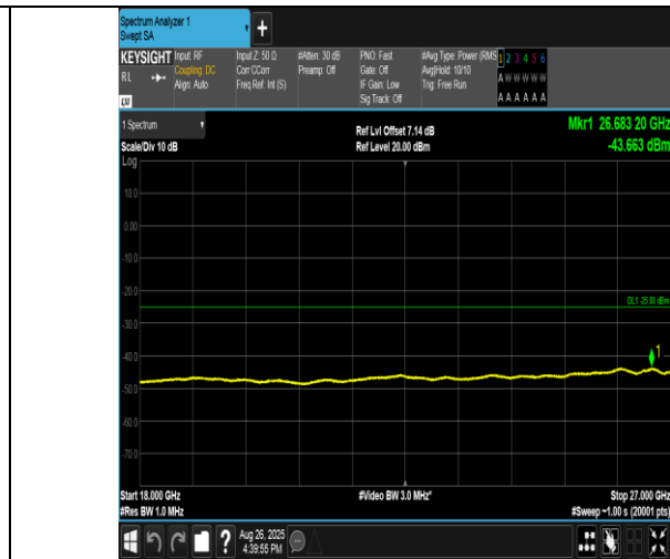
Band38-20MHz-QPSK-38000-100RB#0-18000~27000-PASS
