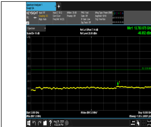
Band38-20MHz-16QAM-38000-1RB#0-3000~18000-PASS
