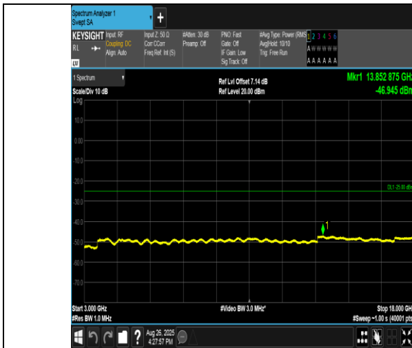
Band38-20MHz-16QAM-37850-100RB#0-3000~18000-PASS
