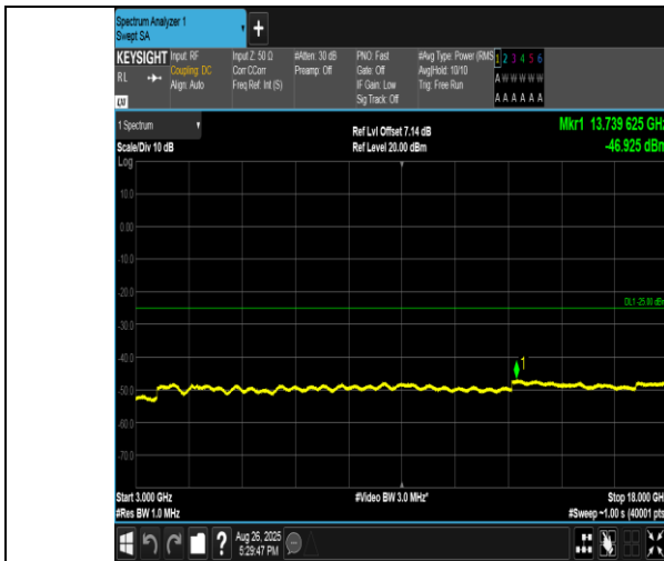
Band38-20MHz-QPSK-38150-100RB#0-3000~18000-PASS
