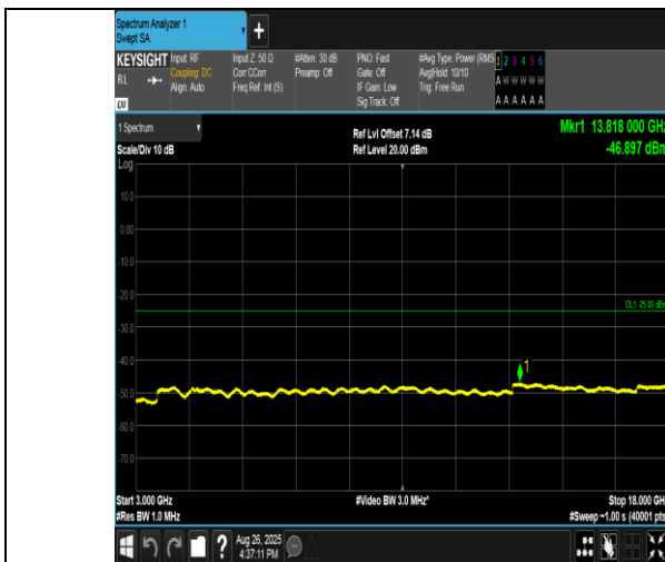
Band38-20MHz-16QAM-38000-1RB#99-3000~18000-PASS
