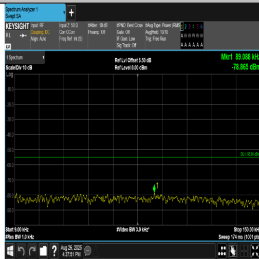
Band38-20MHz-QPSK-38000-100RB#0-0.009~0.15-PASS
