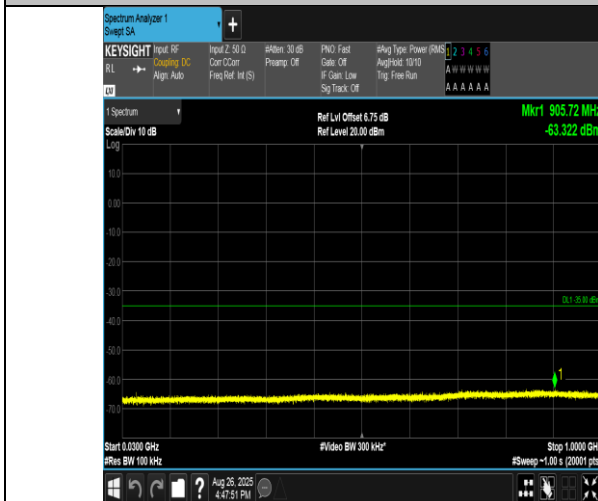
Band38-20MHz-QPSK-38150-1RB#99-30~1000-PASS
