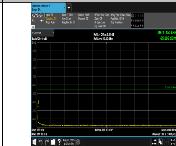
Band38-20MHz-QPSK-38150-1RB#0-0.15~30-PASS
