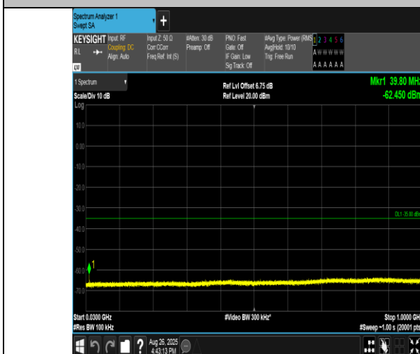
Band38-20MHz-QPSK-38150-1RB#0-30~1000-PASS
