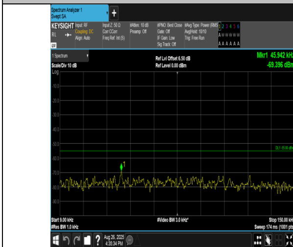
Band38-20MHz-16QAM-38000-1RB#99-0.009~0.15-PASS
