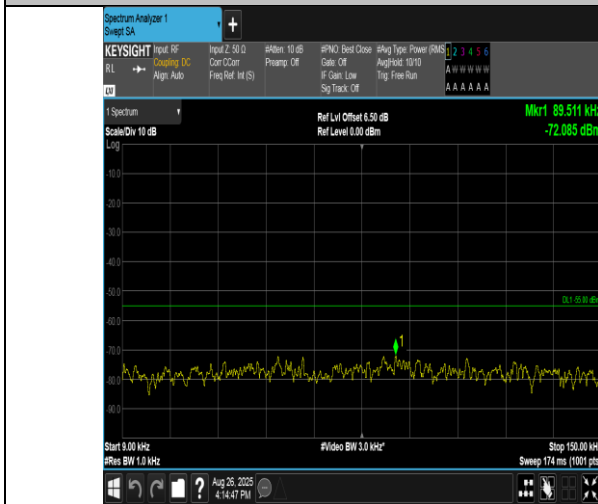
Band38-20MHz-QPSK-37850-1RB#0-0.009~0.15-PASS
