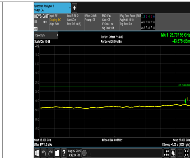
Band38-20MHz-16QAM-38000-100RB#0-18000~27000-PASS
