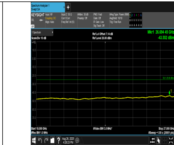
Band38-20MHz-16QAM-37850-100RB#0-18000~27000-PASS
