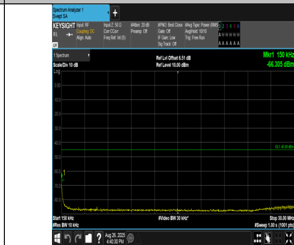
Band38-20MHz-16QAM-38000-100RB#0-0.15~30-PASS
