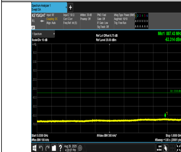
Band38-20MHz-QPSK-37850-1RB#99-30~1000-PASS
