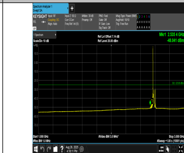
Band38-20MHz-16QAM-37850-1RB#0-1000~3000-PASS
