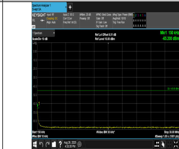
Band38-20MHz-QPSK-38000-1RB#99-0.15~30-PASS
