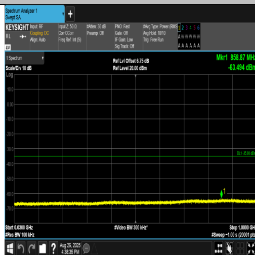
Band38-20MHz-QPSK-38000-100RB#0-30~1000-PASS
