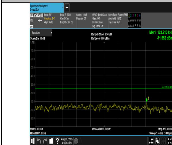
Band38-20MHz-16QAM-38000-1RB#0-0.009~0.15-PASS
