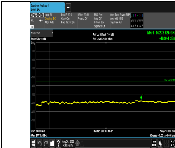
Band38-20MHz-16QAM-38000-100RB#0-3000~18000-PASS
