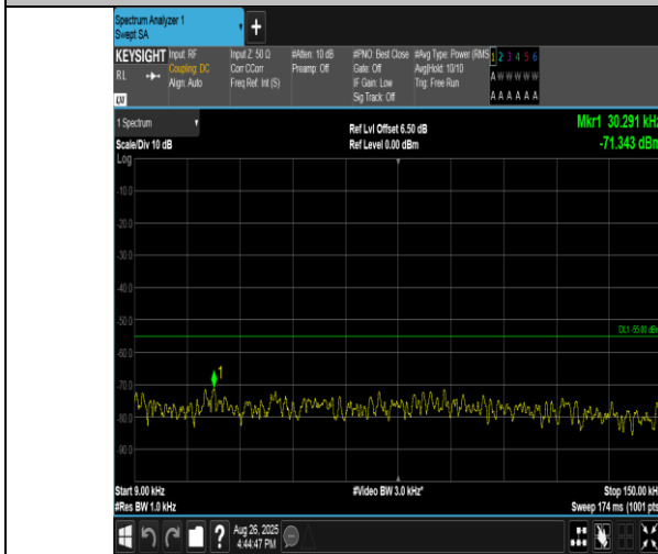
Band38-20MHz-16QAM-38150-1RB#0-0.009~0.15-PASS
