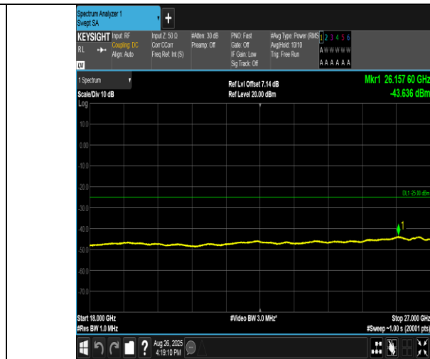
Band38-20MHz-16QAM-37850-1RB#0-18000~27000-PASS
