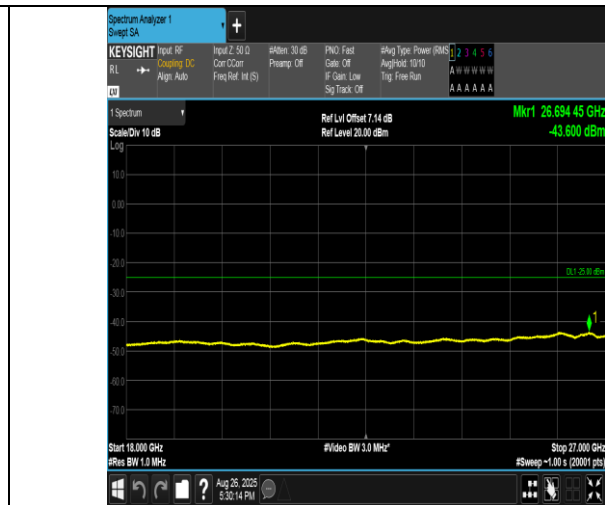
Band38-20MHz-QPSK-38150-100RB#0-18000~27000-PASS
