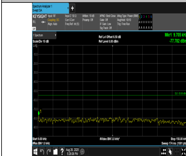
Band38-20MHz-QPSK-38150-100RB#0-0.009~0.15-PASS
