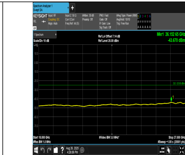
Band38-20MHz-QPSK-37850-100RB#0-18000~27000-PASS
