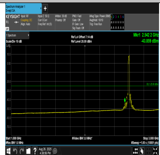
Band38-20MHz-QPSK-38000-100RB#0-1000~3000-PASS
