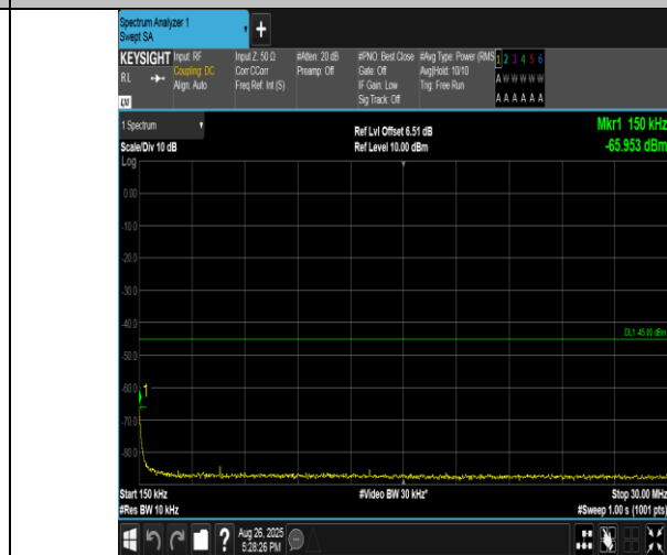
Band38-20MHz-QPSK-38150-100RB#0-0.15~30-PASS
