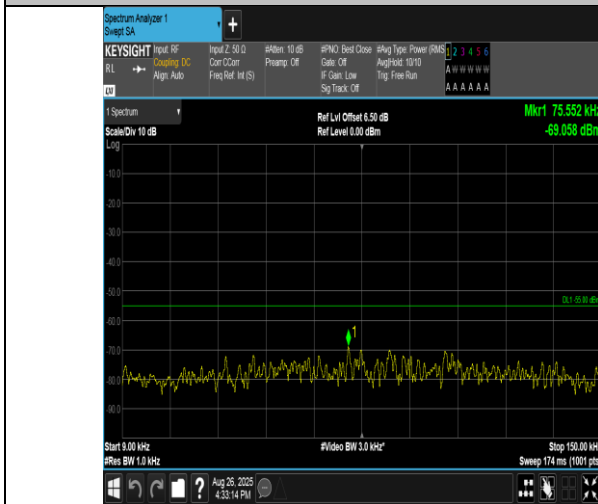
Band38-20MHz-QPSK-38000-1RB#99-0.009~0.15-PASS
