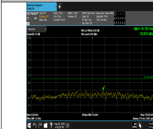
Band38-20MHz-QPSK-38150-1RB#0-0.009~0.15-PASS
