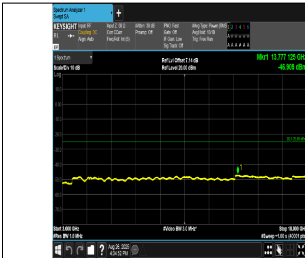
Band38-20MHz-QPSK-38000-1RB#99-3000~18000-PASS
