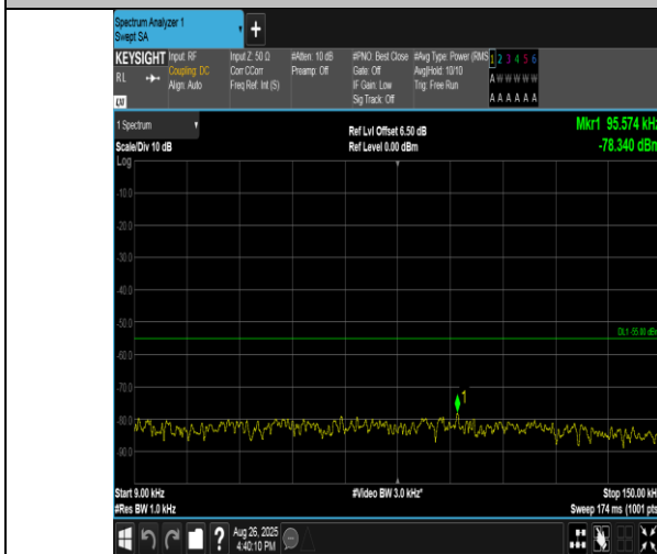
Band38-20MHz-16QAM-38000-100RB#0-0.009~0.15-PASS
