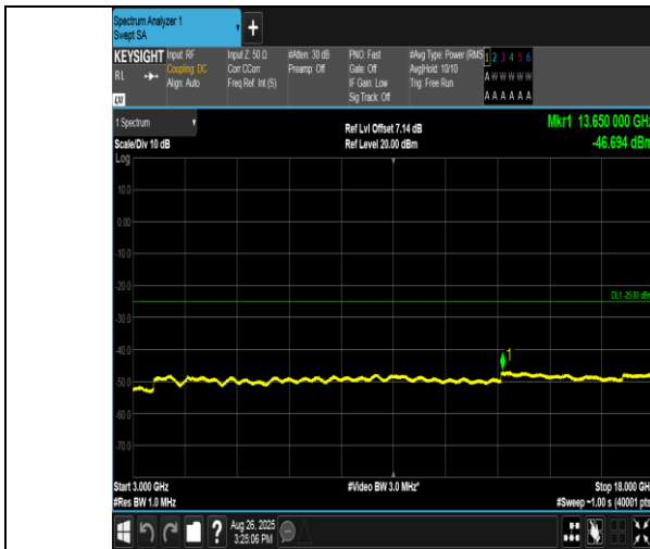
Band38-15MHz-16QAM-38175-75RB#0-3000~18000-PASS
