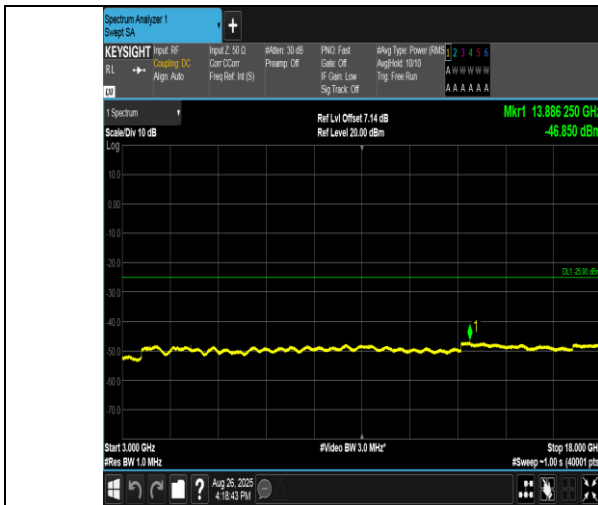
Band38-20MHz-16QAM-37850-1RB#0-3000~18000-PASS
