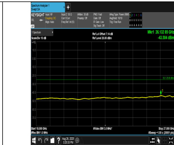
Band38-15MHz-16QAM-38175-75RB#0-18000~27000-PASS
