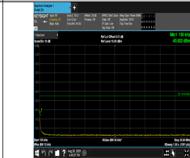
Band38-20MHz-16QAM-38150-1RB#0-0.15~30-PASS
