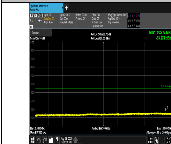
Band38-20MHz-QPSK-38150-100RB#0-30~1000-PASS
