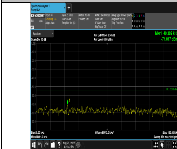
Band38-20MHz-16QAM-37850-1RB#99-0.009~0.15-PASS
