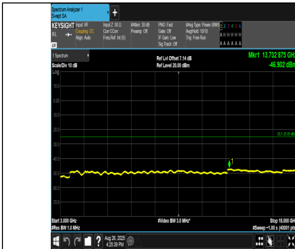
Band38-20MHz-QPSK-37850-100RB#0-3000~18000-PASS
