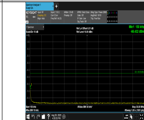
Band38-20MHz-16QAM-38000-1RB#99-0.15~30-PASS
