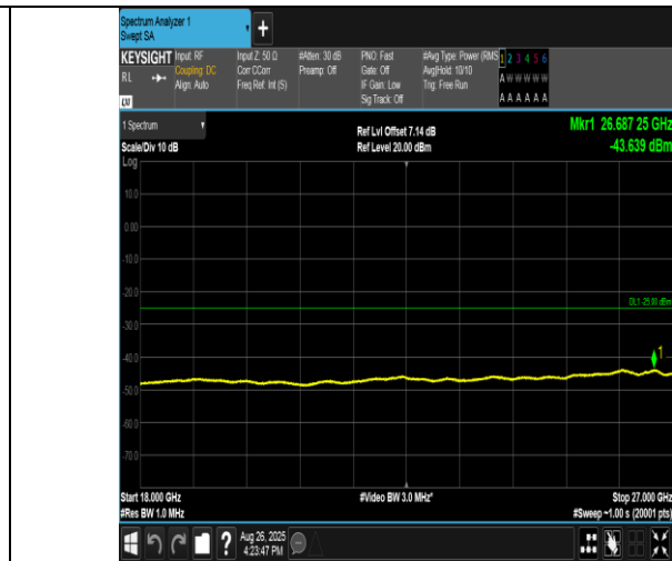
Band38-20MHz-16QAM-37850-1RB#99-18000~27000-PASS
