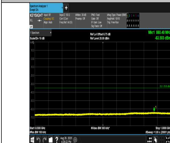
Band38-20MHz-QPSK-38000-1RB#0-30~1000-PASS
