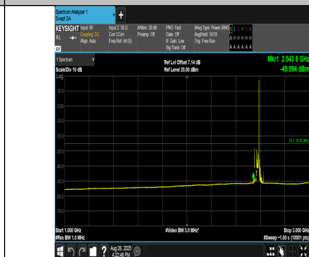
Band38-20MHz-16QAM-37850-1RB#99-1000~3000-PASS
