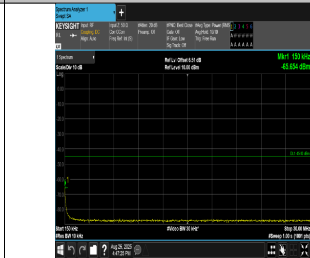
Band38-20MHz-QPSK-38150-1RB#99-0.15~30-PASS
