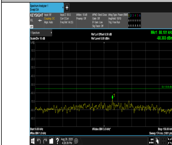
Band38-20MHz-QPSK-38000-1RB#0-0.009~0.15-PASS
