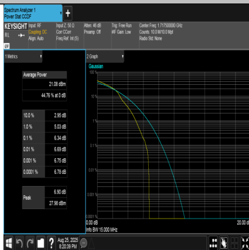
Band4-15MHz-16QAM-20025-1RB#0-PASS
