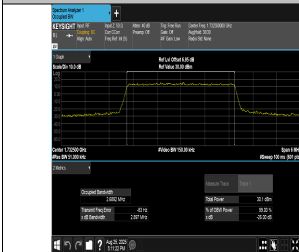
Band4-3MHz-QPSK-20175-15RB#0-PASS
