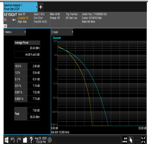
Band4-10MHz-16QAM-20000-50RB#0-PASS
