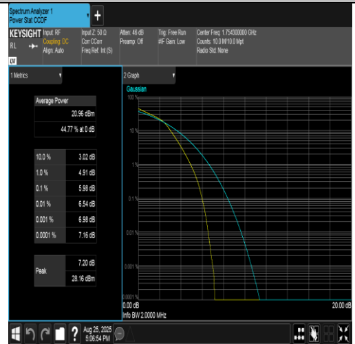
Band4-1.4MHz-16QAM-20393-6RB#0-PASS
