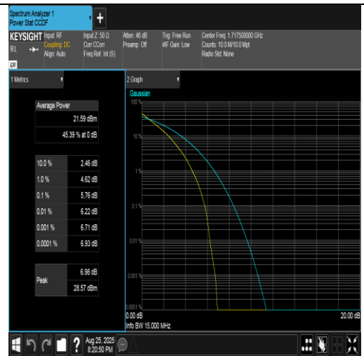
Band4-15MHz-QPSK-20025-75RB#0-PASS
