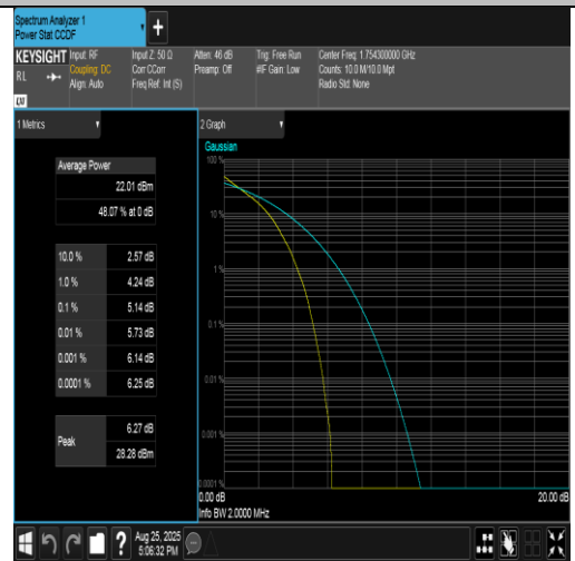
Band4-1.4MHz-QPSK-20393-6RB#0-PASS
