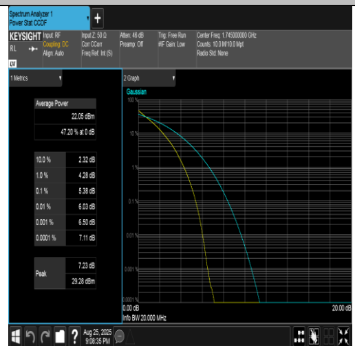
Band4-20MHz-QPSK-20300-100RB#0-PASS
