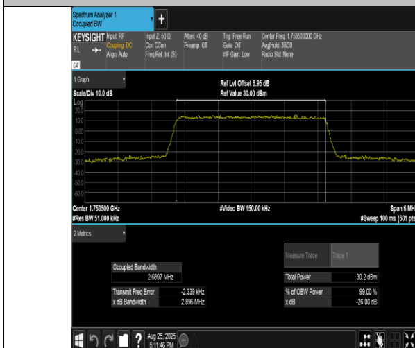
Band4-3MHz-QPSK-20385-15RB#0-PASS
