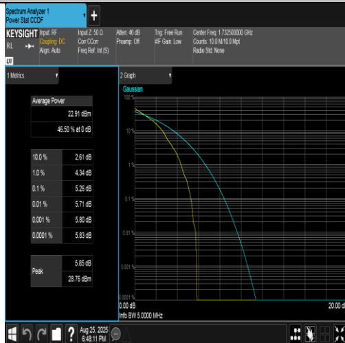
Band4-5MHz-QPSK-20175-1RB#0-PASS
