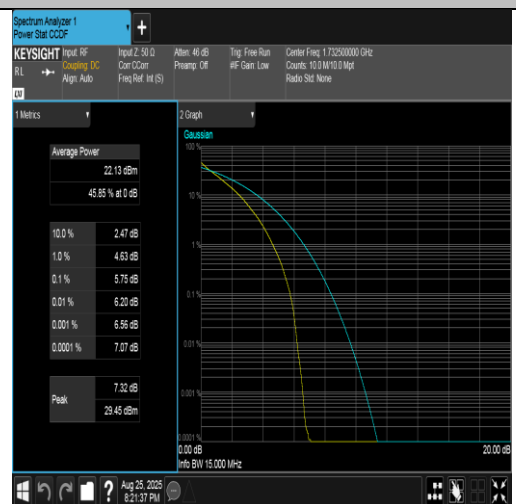
Band4-15MHz-QPSK-20175-75RB#0-PASS
