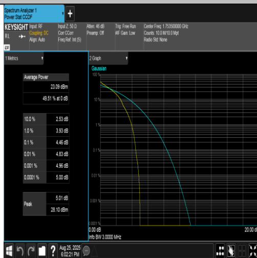
Band4-3MHz-QPSK-20385-1RB#0-PASS
