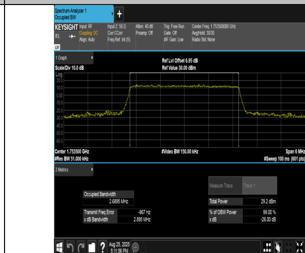
Band4-3MHz-16QAM-20385-15RB#0-PASS
