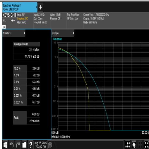
Band4-10MHz-16QAM-20000-1RB#0-PASS
