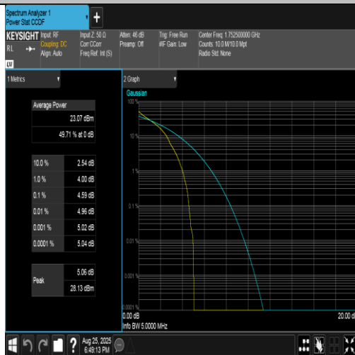
Band4-5MHz-QPSK-20375-1RB#0-PASS
