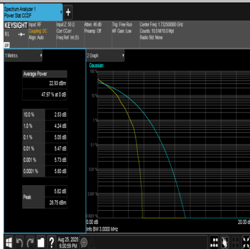
Band4-3MHz-QPSK-20175-1RB#0-PASS
