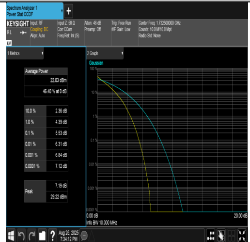
Band4-10MHz-QPSK-20175-50RB#0-PASS
