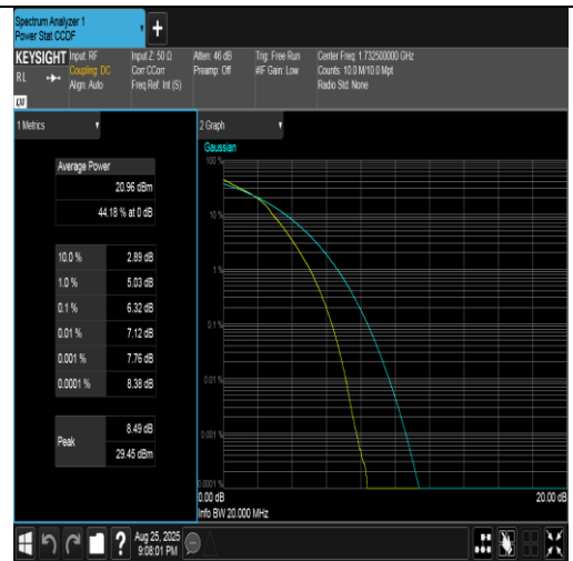
Band4-20MHz-16QAM-20175-100RB#0-PASS
