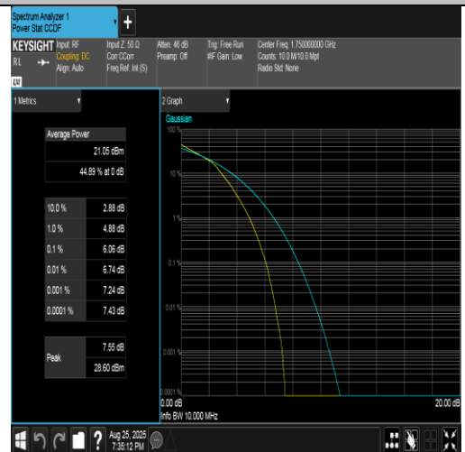
Band4-10MHz-16QAM-20350-50RB#0-PASS
