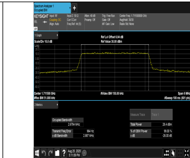
Band4-3MHz-16QAM-19965-15RB#0-PASS
