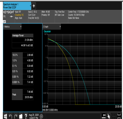
Band4-5MHz-16QAM-20375-25RB#0-PASS
