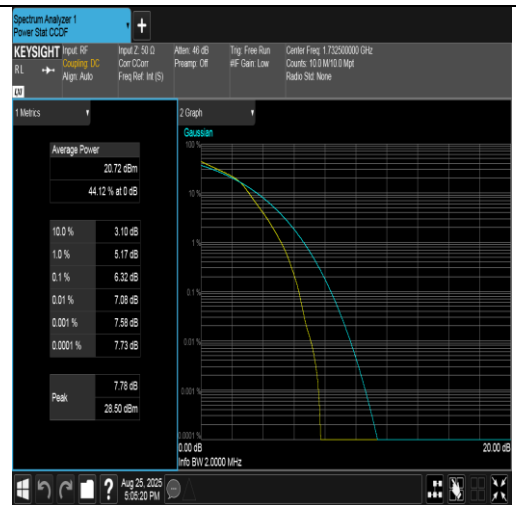
Band4-1.4MHz-16QAM-20175-6RB#0-PASS
