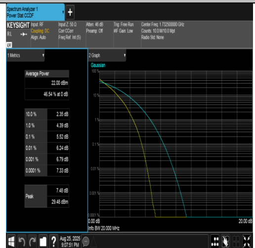
Band4-20MHz-QPSK-20175-100RB#0-PASS
