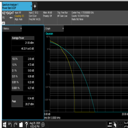
Band4-3MHz-16QAM-20385-1RB#0-PASS
