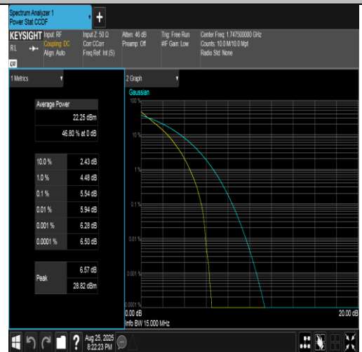
Band4-15MHz-QPSK-20325-75RB#0-PASS
