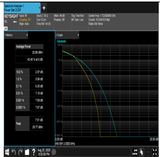
Band4-3MHz-16QAM-20175-15RB#0-PASS
