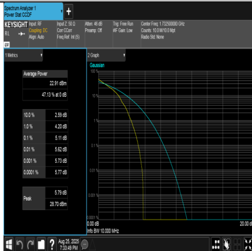
Band4-10MHz-QPSK-20175-1RB#0-PASS
