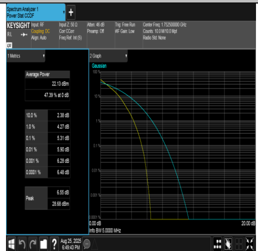
Band4-5MHz-QPSK-20375-25RB#0-PASS
