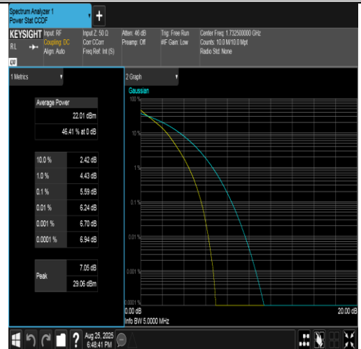
Band4-5MHz-QPSK-20175-25RB#0-PASS
