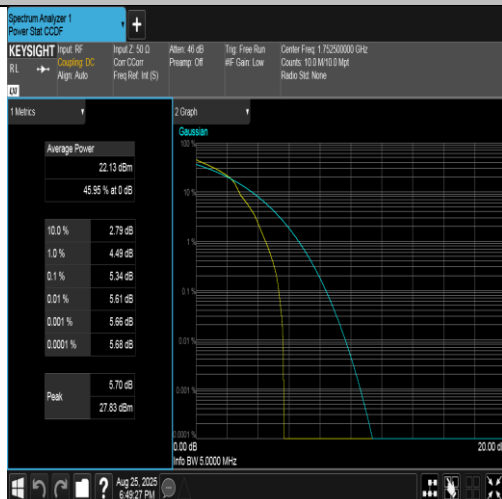
Band4-5MHz-16QAM-20375-1RB#0-PASS
