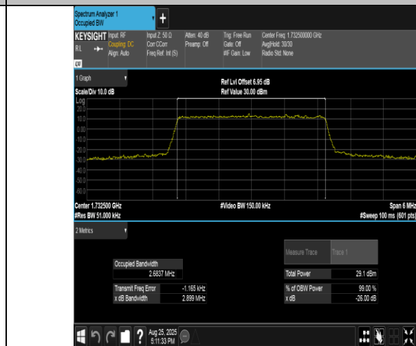
Band4-3MHz-16QAM-20175-15RB#0-PASS
