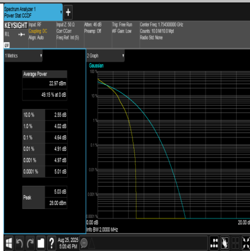
Band4-1.4MHz-QPSK-20393-1RB#0-PASS
