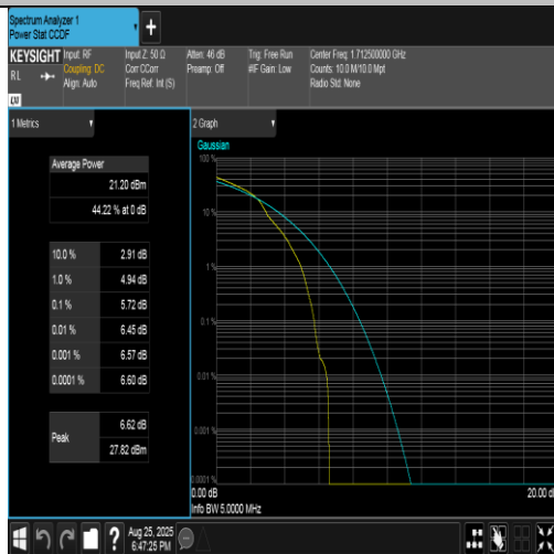
Band4-5MHz-16QAM-19975-1RB#0-PASS
