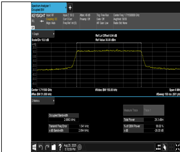
Band4-3MHz-QPSK-19965-15RB#0-PASS
