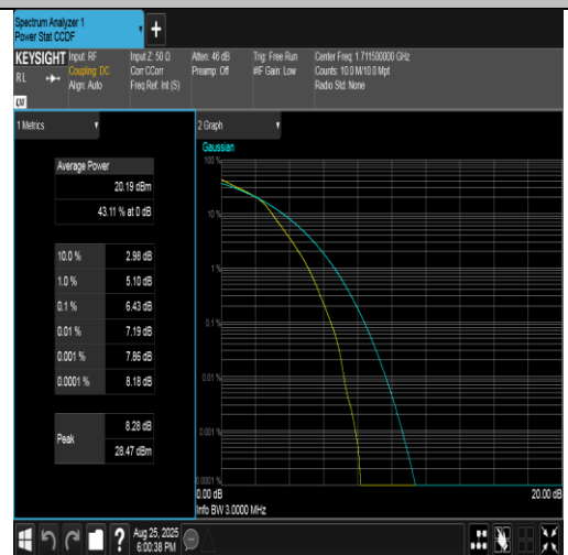
Band4-3MHz-16QAM-19965-15RB#0-PASS
