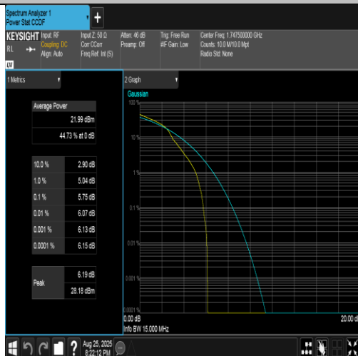
Band4-15MHz-16QAM-20325-1RB#0-PASS
