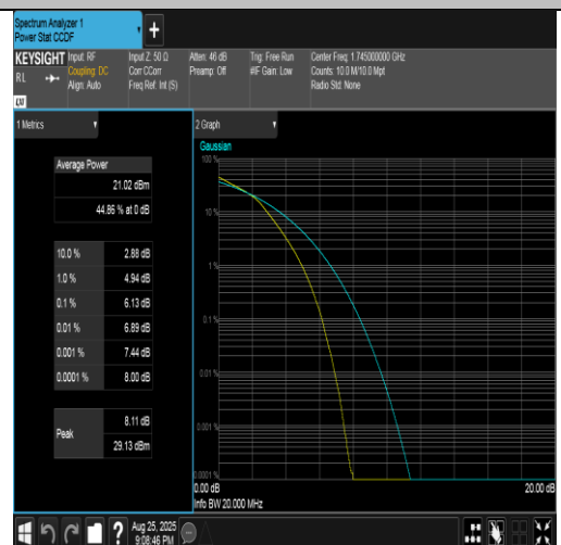
Band4-20MHz-16QAM-20300-100RB#0-PASS
