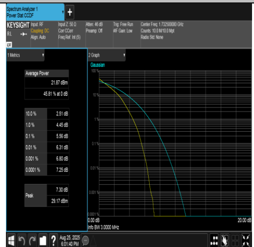
Band4-3MHz-QPSK-20175-15RB#0-PASS
