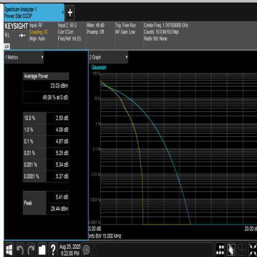
Band4-15MHz-QPSK-20325-1RB#0-PASS
