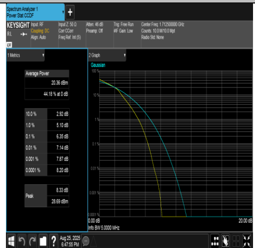
Band4-5MHz-16QAM-19975-25RB#0-PASS
