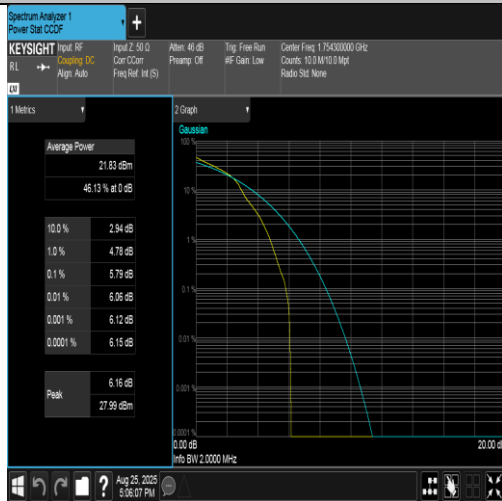
Band4-1.4MHz-16QAM-20393-1RB#0-PASS
