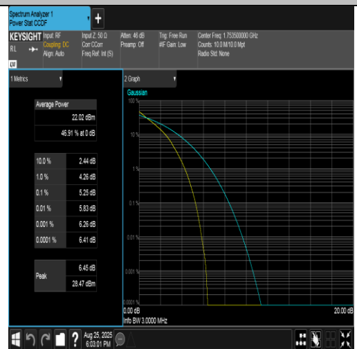
Band4-3MHz-QPSK-20385-15RB#0-PASS
