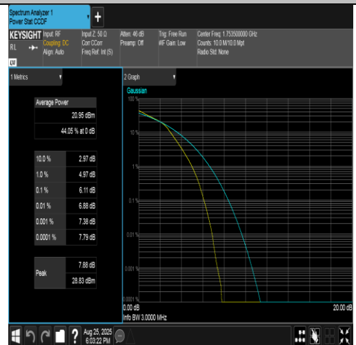
Band4-3MHz-16QAM-20385-15RB#0-PASS
