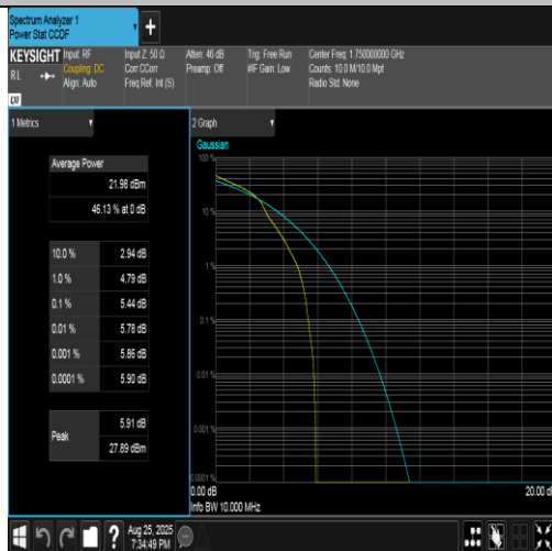
Band4-10MHz-16QAM-20350-1RB#0-PASS
