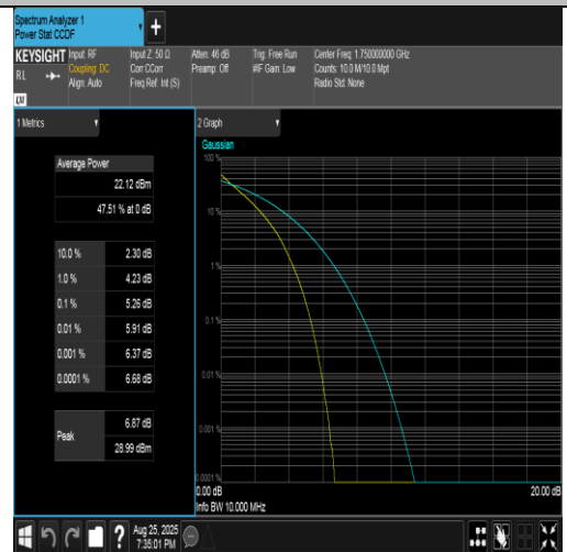
Band4-10MHz-QPSK-20350-50RB#0-PASS
