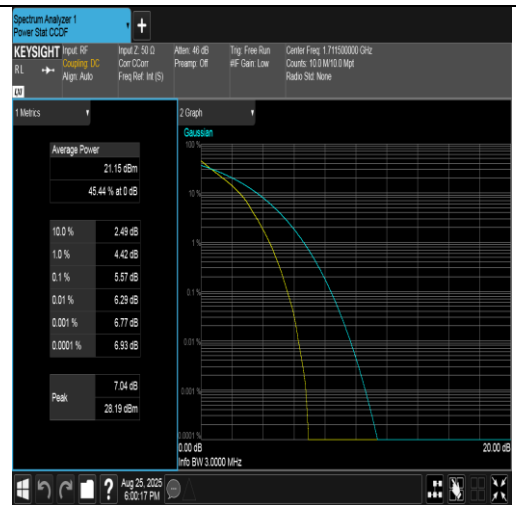
Band4-3MHz-QPSK-19965-15RB#0-PASS
