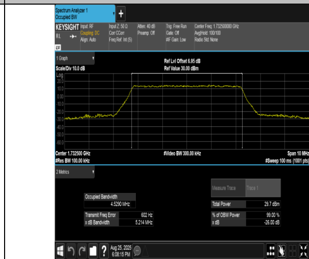
Band4-5MHz-16QAM-20175-25RB#0-PASS
