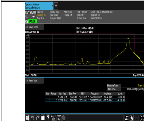
Band4-10MHz-16QAM-20350-1RB#49-PASS
