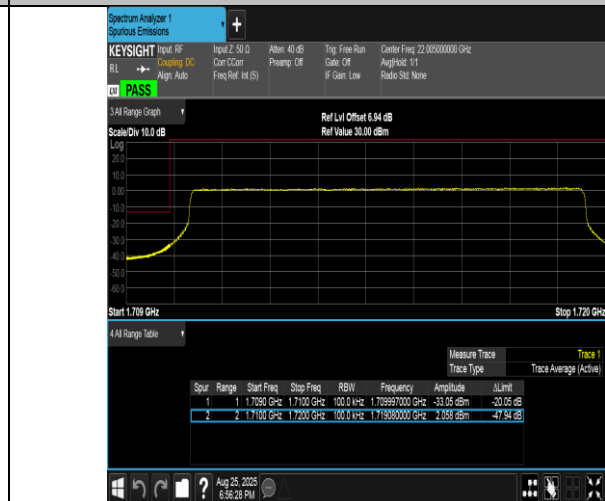
Band4-10MHz-16QAM-20000-50RB#0-PASS
