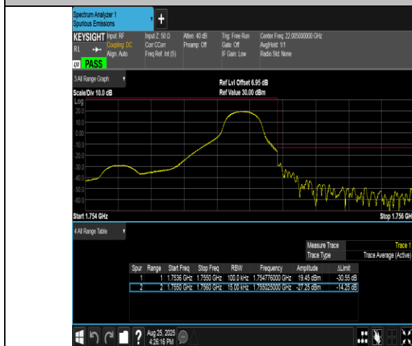
Band4-1.4MHz-16QAM-20393-1RB#5-PASS
