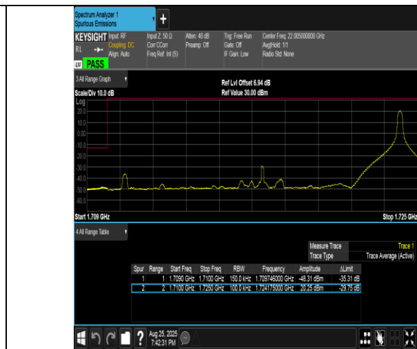
Band4-15MHz-QPSK-20025-1RB#74-PASS
