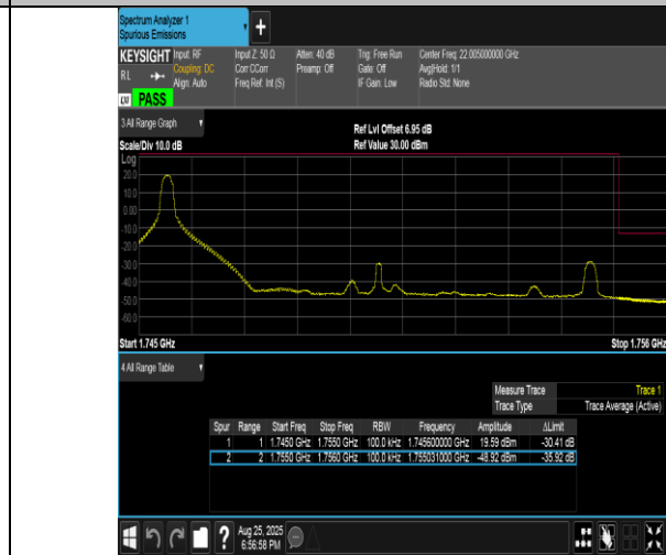
Band4-10MHz-16QAM-20350-1RB#0-PASS
