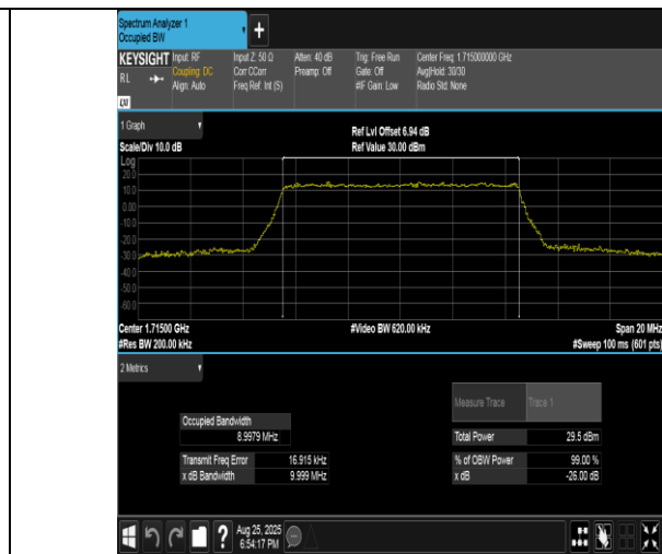
Band4-10MHz-16QAM-20000-50RB#0-PASS
