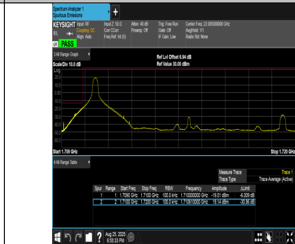
Band4-10MHz-16QAM-20000-1RB#0-PASS
