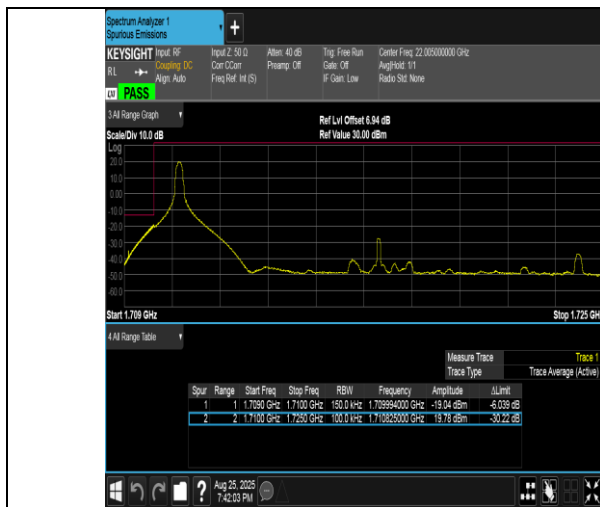
Band4-15MHz-QPSK-20025-1RB#0-PASS
