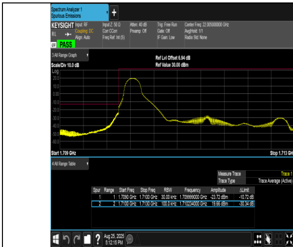
Band4-3MHz-QPSK-19965-1RB#0-PASS
