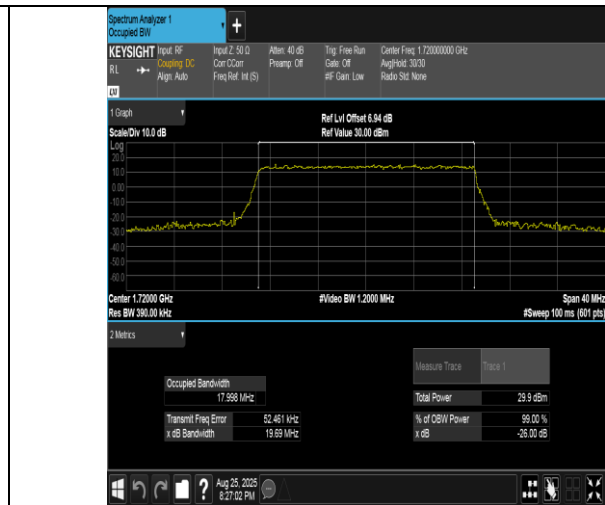
Band4-20MHz-16QAM-20050-100RB#0-PASS
