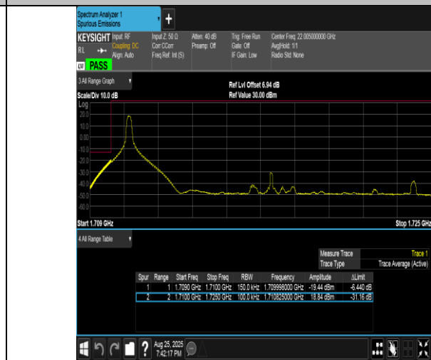
Band4-15MHz-16QAM-20025-1RB#0-PASS
