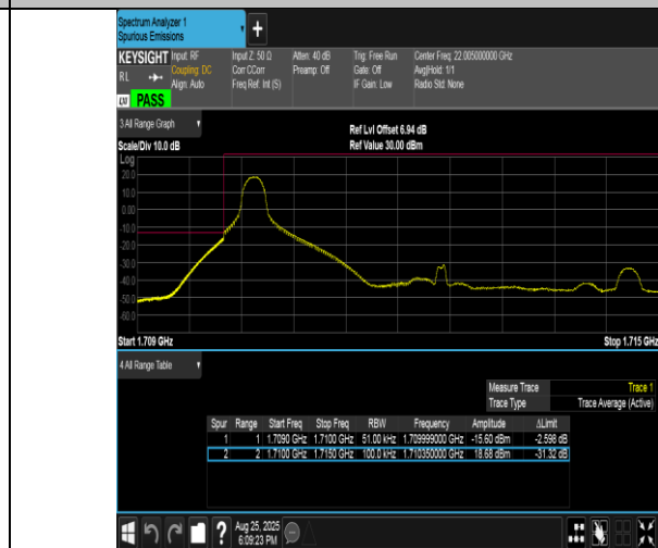
Band4-5MHz-16QAM-19975-1RB#0-PASS
