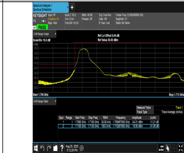
Band4-3MHz-16QAM-19965-1RB#0-PASS
