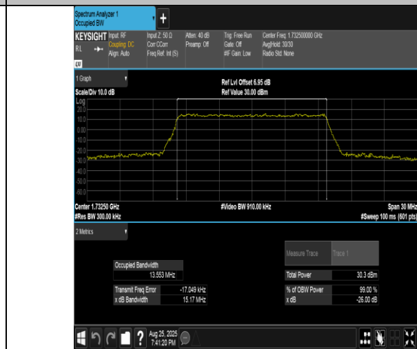
Band4-15MHz-16QAM-20175-75RB#0-PASS
