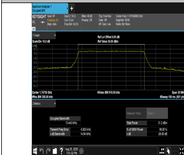
Band4-15MHz-QPSK-20325-75RB#0-PASS
