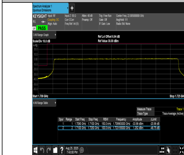
Band4-15MHz-QPSK-20025-75RB#0-PASS
