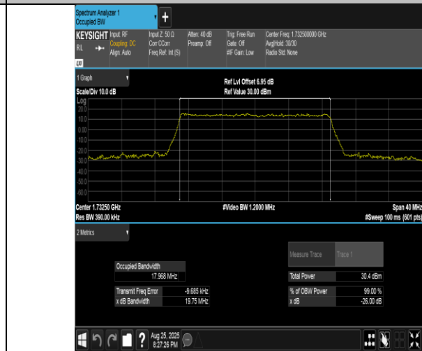
Band4-20MHz-16QAM-20175-100RB#0-PASS
