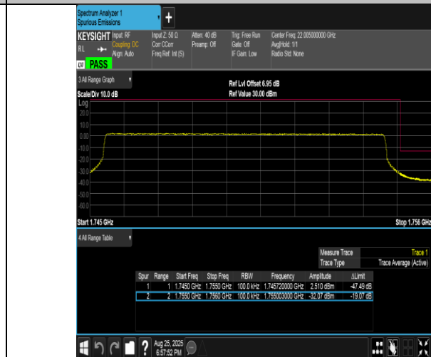
Band4-10MHz-16QAM-20350-50RB#0-PASS
