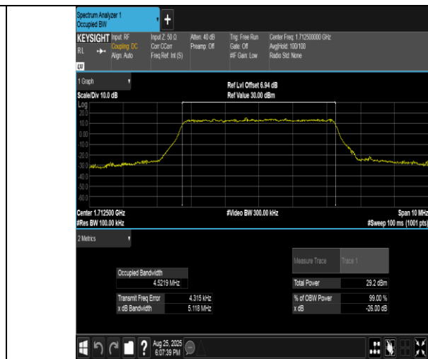
Band4-5MHz-16QAM-19975-25RB#0-PASS
