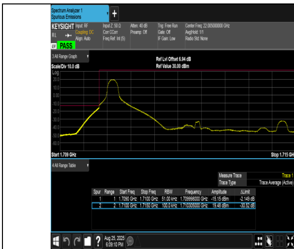
Band4-5MHz-QPSK-19975-1RB#0-PASS
