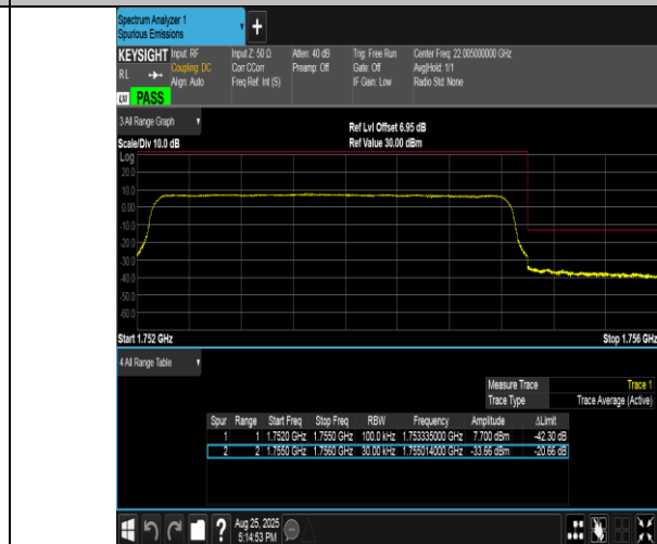
Band4-3MHz-16QAM-20385-15RB#0-PASS
