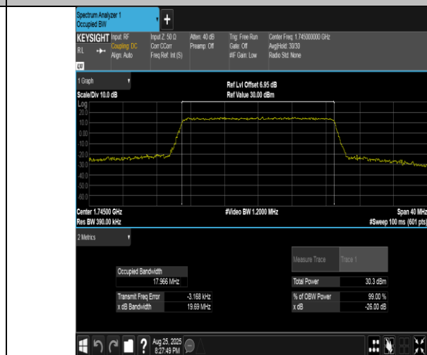
Band4-20MHz-16QAM-20300-100RB#0-PASS
