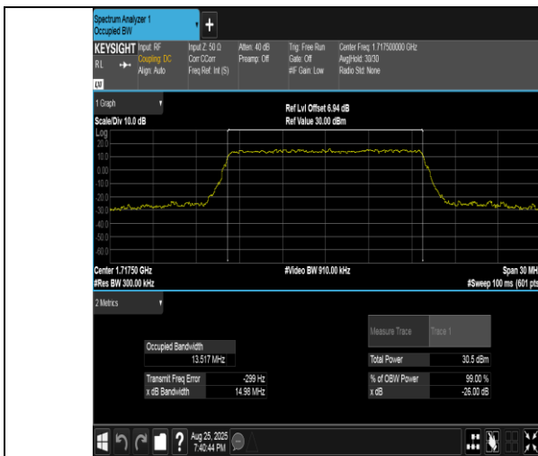
Band4-15MHz-QPSK-2025-75RB#0-PASS
