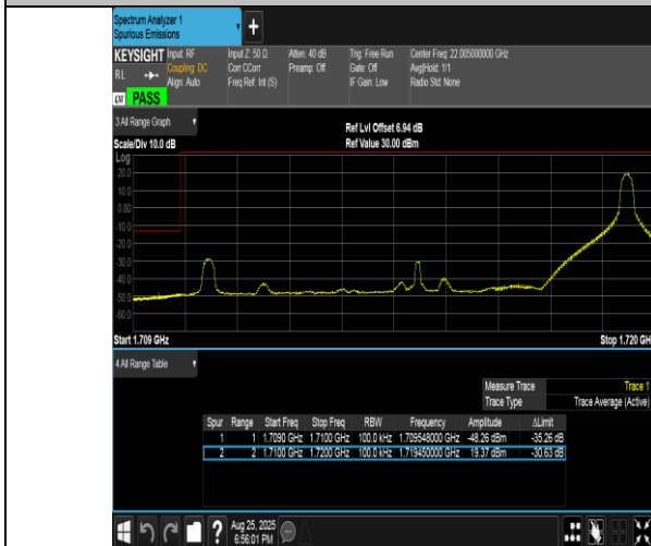
Band4-10MHz-16QAM-20000-1RB#49-PASS
