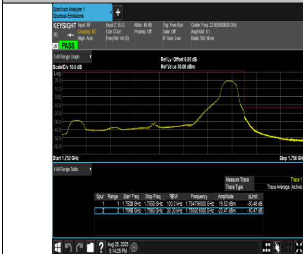
Band4-3MHz-16QAM-20385-1RB#14-PASS
