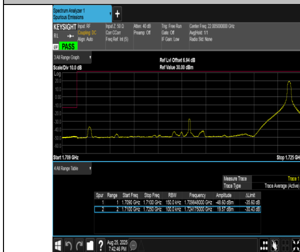
Band4-15MHz-16QAM-20025-1RB#74-PASS
