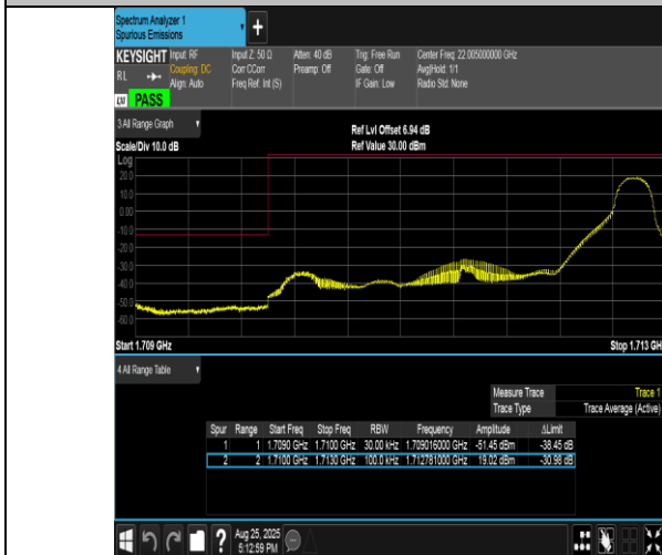
Band4-3MHz-16QAM-19965-1RB#14-PASS
