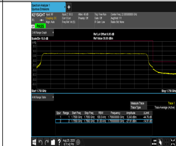
Band4-5MHz-16QAM-20375-25RB#0-PASS
