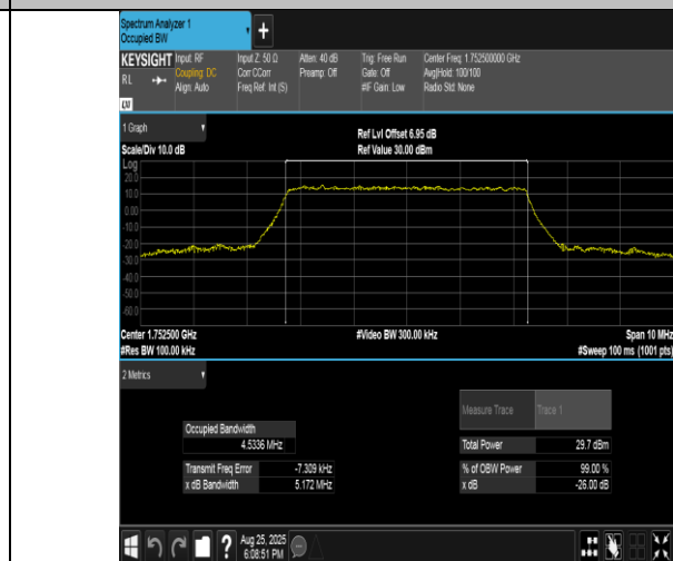
Band4-5MHz-16QAM-20375-25RB#0-PASS
