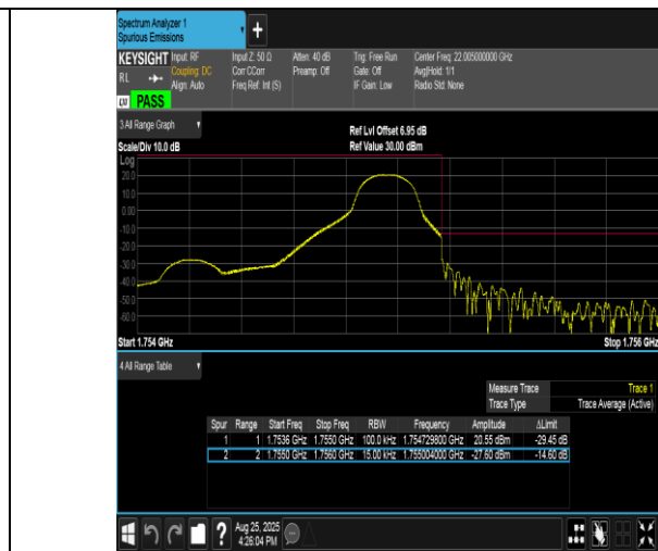
Band4-1.4MHz-QPSK-20393-1RB#5-PASS
