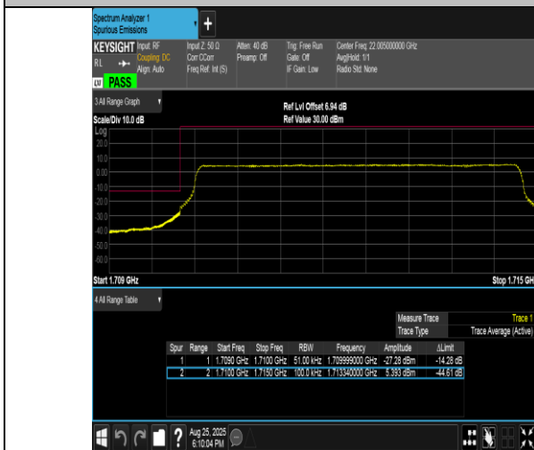
Band4-5MHz-QPSK-19975-25RB#0-PASS
