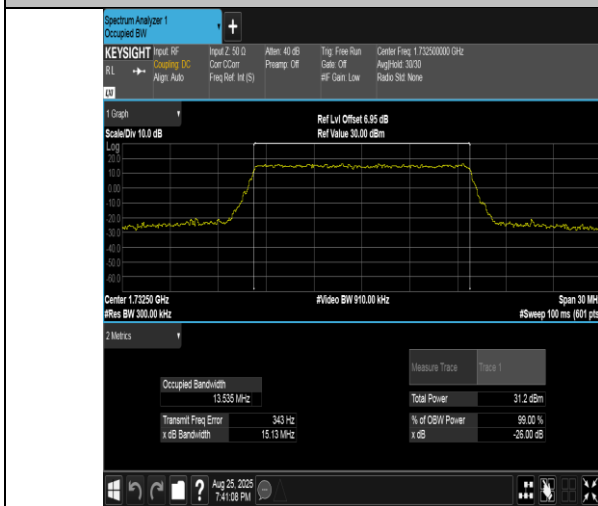
Band4-15MHz-QPSK-20175-75RB#0-PASS
