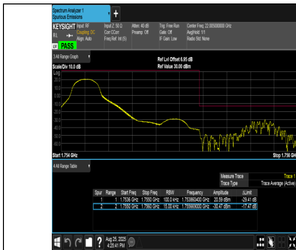
Band4-1.4MHz-QPSK-20393-1RB#0-PASS
