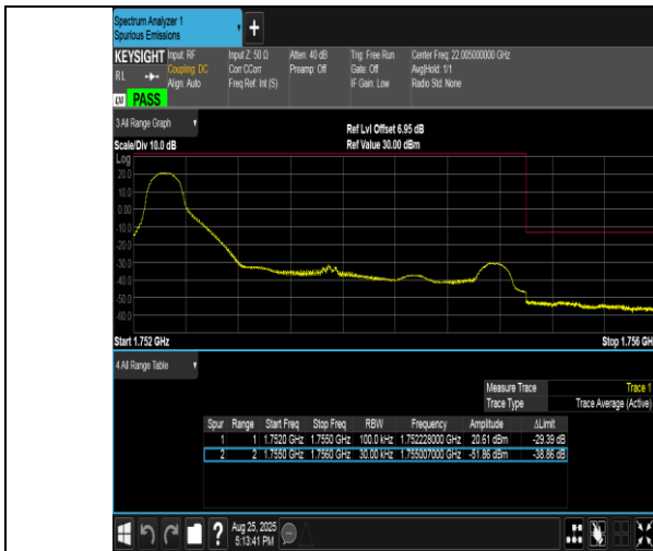
Band4-3MHz-QPSK-20385-1RB#0-PASS
