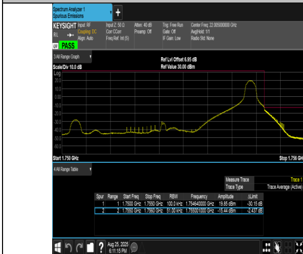
Band4-5MHz-16QAM-20375-1RB#24-PASS
