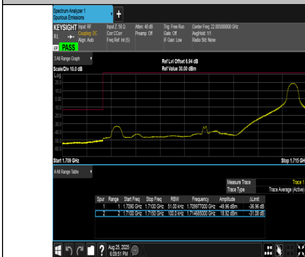
Band4-5MHz-16QAM-19975-1RB#24-PASS
