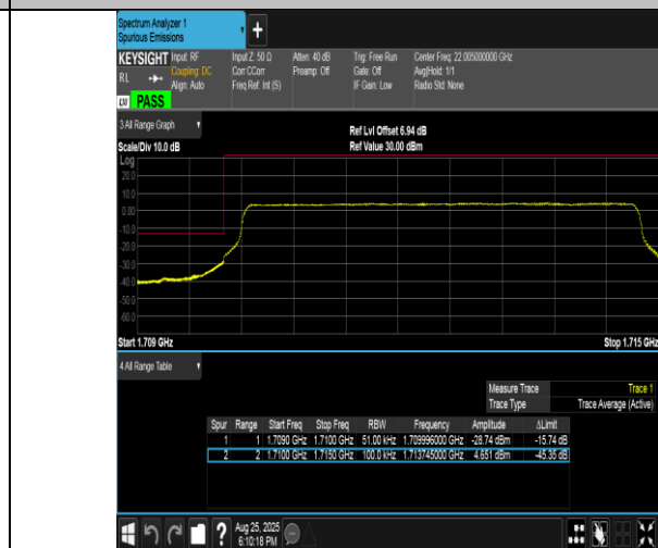
Band4-5MHz-16QAM-19975-25RB#0-PASS
