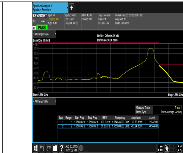
Band4-5MHz-QPSK-20375-1RB#24-PASS
