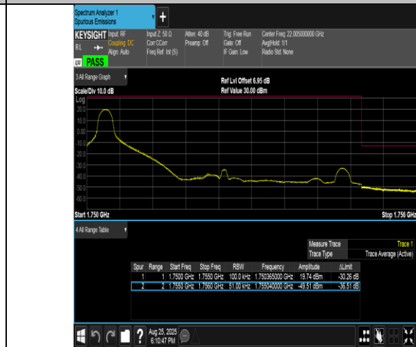
Band4-5MHz-16QAM-20375-1RB#0-PASS
