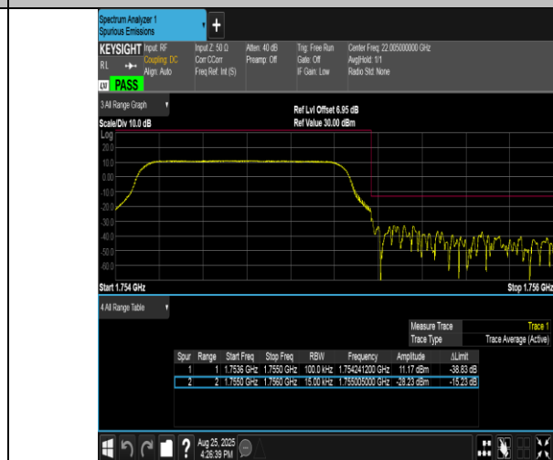
Band4-1.4MHz-16QAM-20393-6RB#0-PASS
