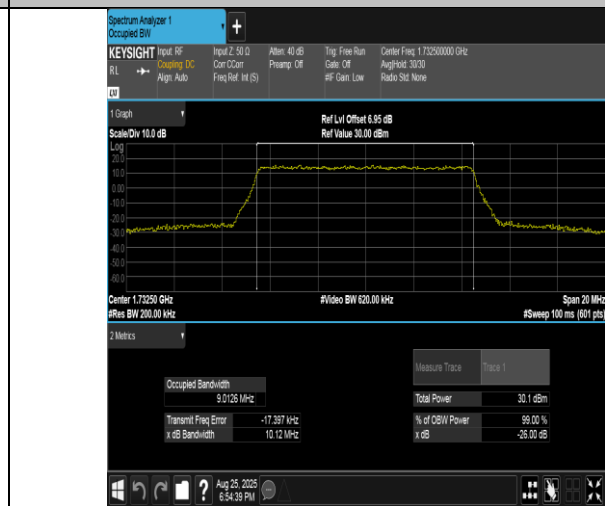
Band4-10MHz-16QAM-20175-50RB#0-PASS
