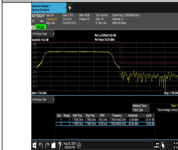
Band4-1.4MHz-QPSK-20393-6RB#0-PASS
