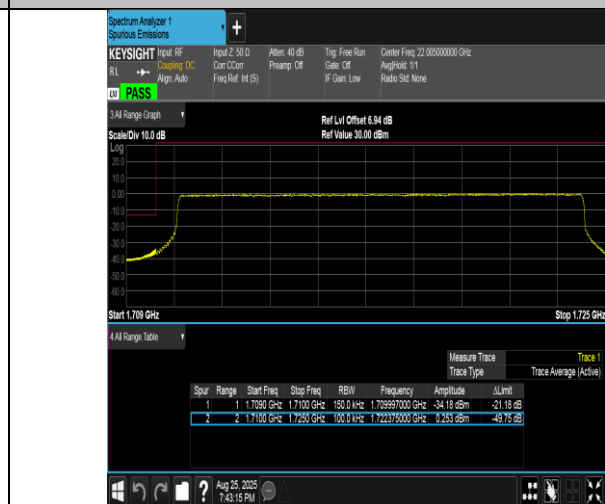
Band4-15MHz-16QAM-20025-75RB#0-PASS
