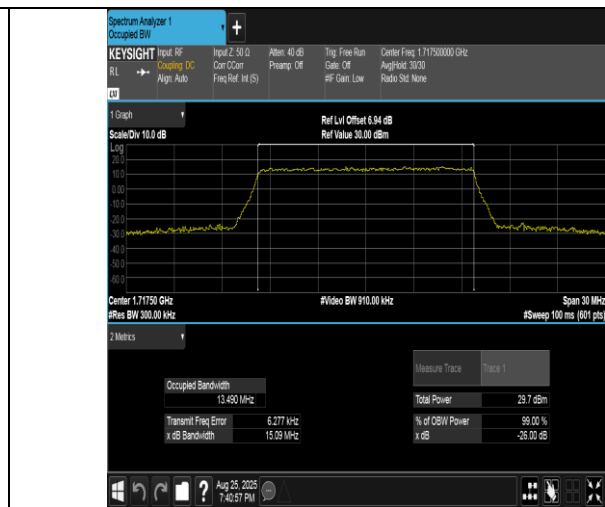
Band4-15MHz-16QAM-2025-75RB#0-PASS
