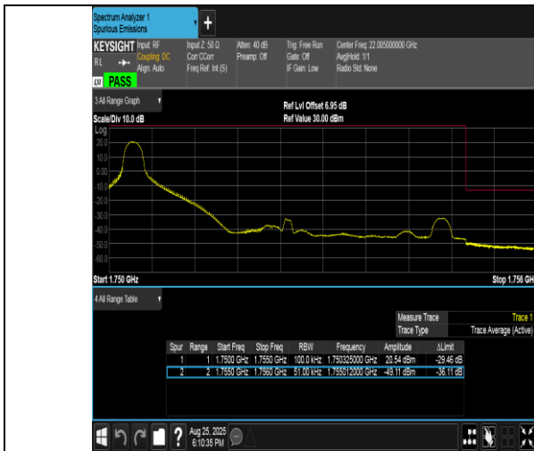
Band4-5MHz-QPSK-20375-1RB#0-PASS
