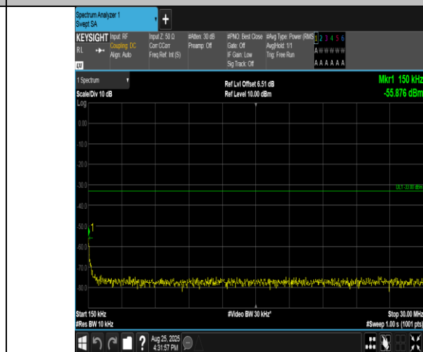
Band4-1.4MHz-QPSK-19957-6RB#0-0.15~30-PASS
