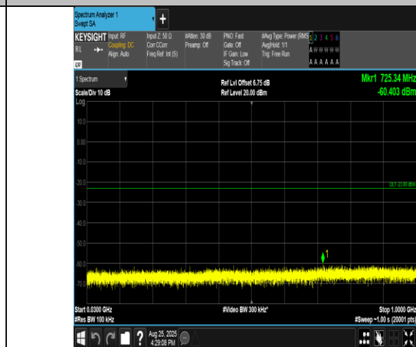
Band4-1.4MHz-16QAM-19957-1RB#0-30~1000-PASS
