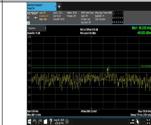
Band4-1.4MHz-16QAM-19957-1RB#0-0.009~0.15-PASS
