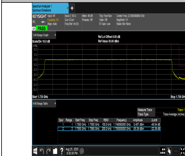
Band4-20MHz-QPSK-20300-100RB#0-PASS
