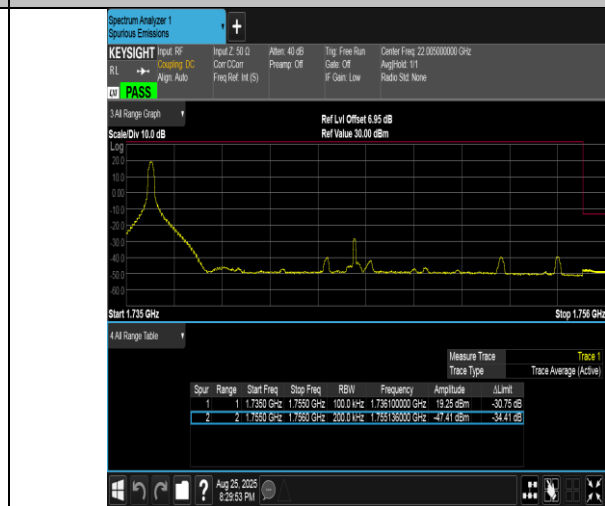
Band4-20MHz-16QAM-20300-1RB#0-PASS
