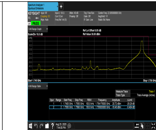
Band4-15MHz-QPSK-20325-1RB#74-PASS
