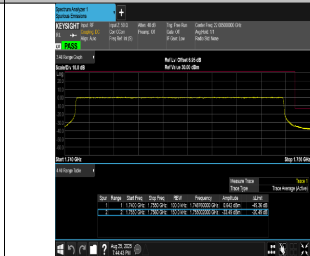
Band4-15MHz-16QAM-20325-75RB#0-PASS
