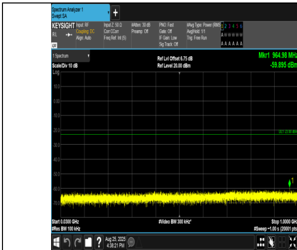
Band4-1.4MHz-QPSK-20175-6RB#0-30~1000-PASS
