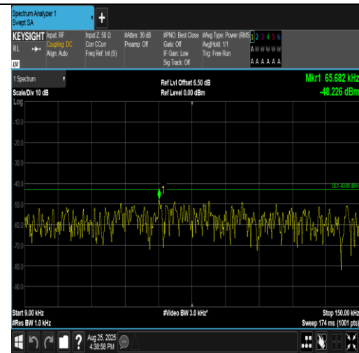
Band4-1.4MHz-16QAM-20175-6RB#0-0.009~0.15-PASS
