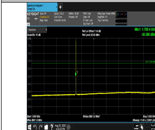
Band4-1.4MHz-16QAM-19957-6RB#0-1000~3000-PASS
