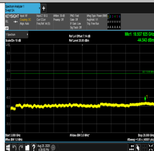
Band4-1.4MHz-16QAM-20175-6RB#0-3000~20000-PASS
