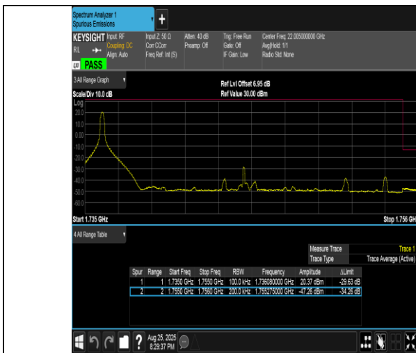
Band4-20MHz-QPSK-20300-1RB#0-PASS
