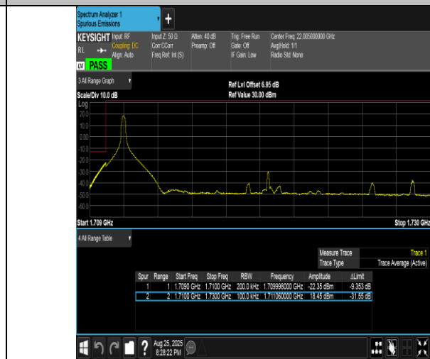
Band4-20MHz-16QAM-20050-1RB#0-PASS
