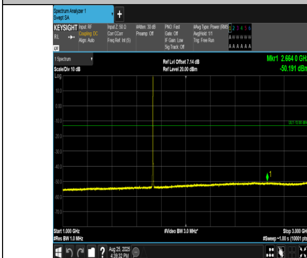
Band4-1.4MHz-16QAM-20175-6RB#0-1000~3000-PASS
