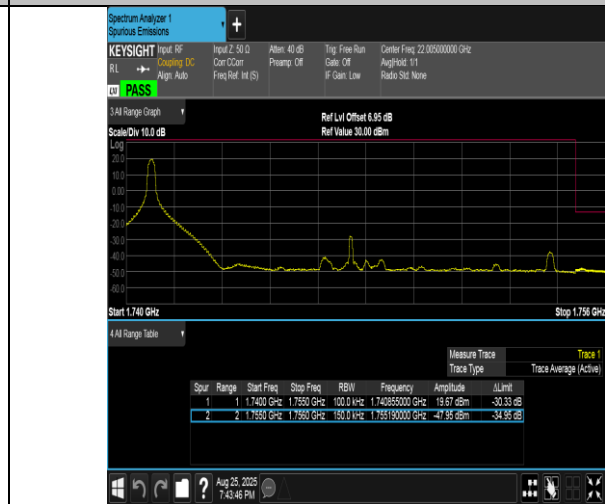
Band4-15MHz-16QAM-20325-1RB#0-PASS
