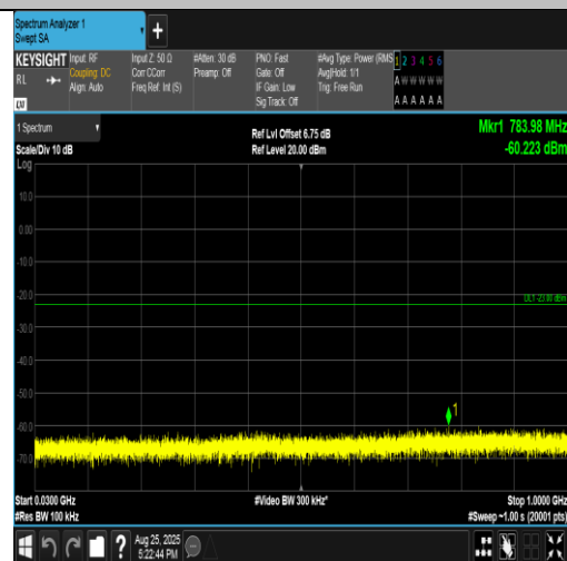
Band4-3MHz-16QAM-20175-1RB#0-30~1000-PASS
