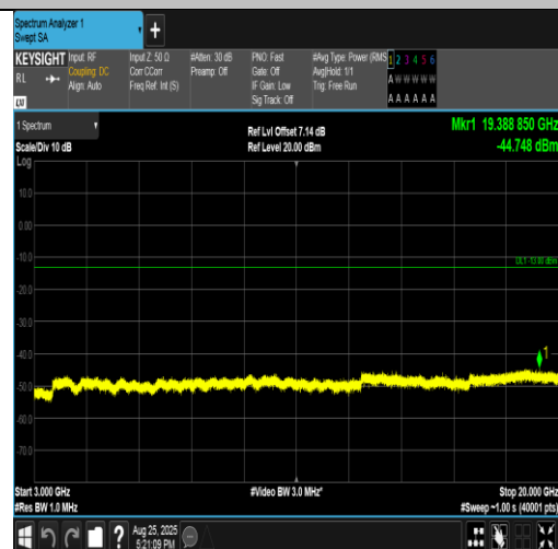
Band4-3MHz-16QAM-19965-15RB#0-3000~20000-PASS
