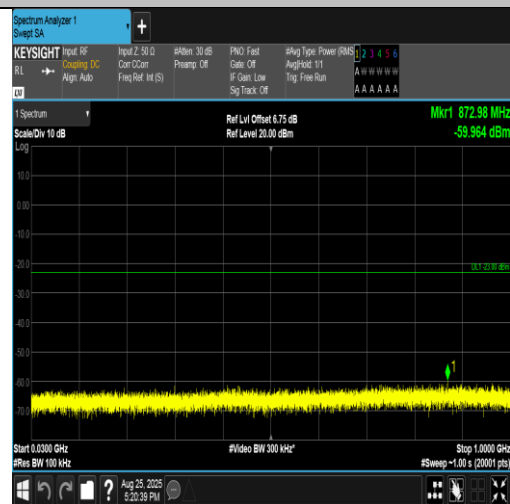
Band4-3MHz-16QAM-19965-15RB#0-30~1000-PASS
