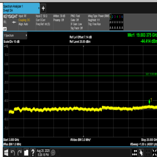
Band4-3MHz-QPSK-20175-15RB#0-3000~20000-PASS
