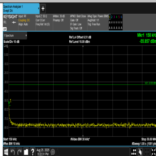
Band4-3MHz-16QAM-20175-1RB#0-0.15~30-PASS
