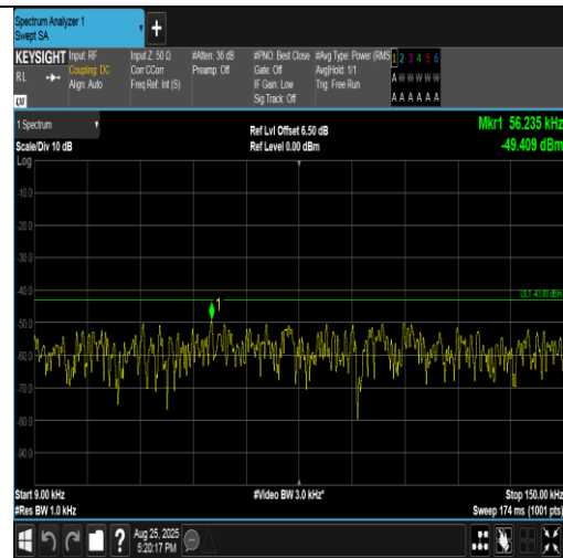
Band4-3MHz-16QAM-19965-15RB#0-0.009~0.15-PASS
