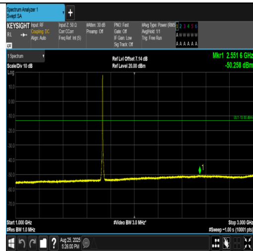
Band4-3MHz-QPSK-20175-15RB#0-1000~3000-PASS
