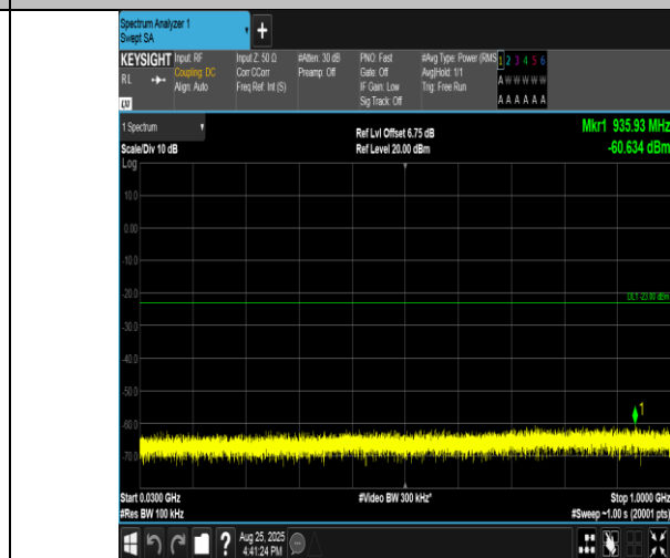
Band4-1.4MHz-16QAM-20393-1RB#0-30~1000-PASS
