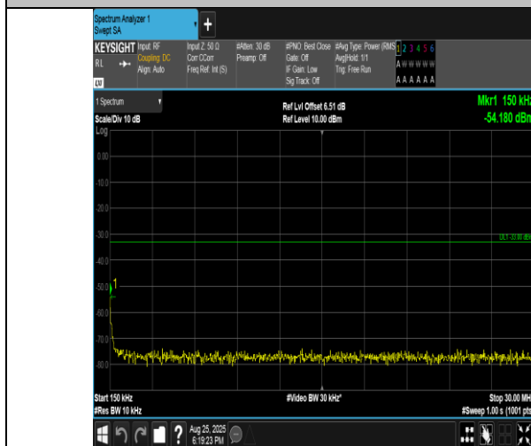
Band4-5MHz-16QAM-20175-1RB#0-0.15~30-PASS
