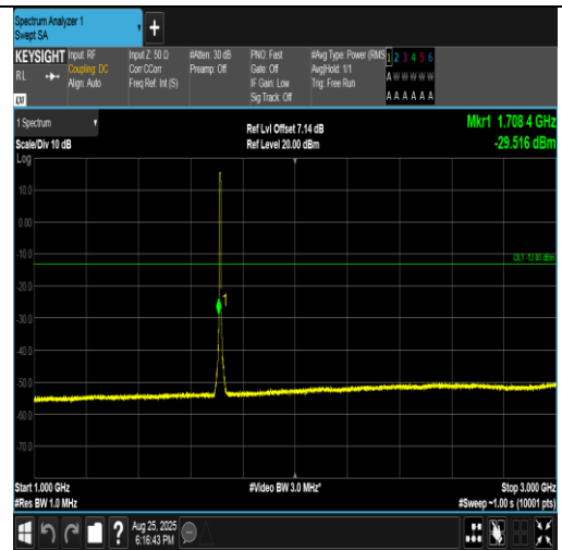
Band4-5MHz-QPSK-19975-25RB#0-1000~3000-PASS
