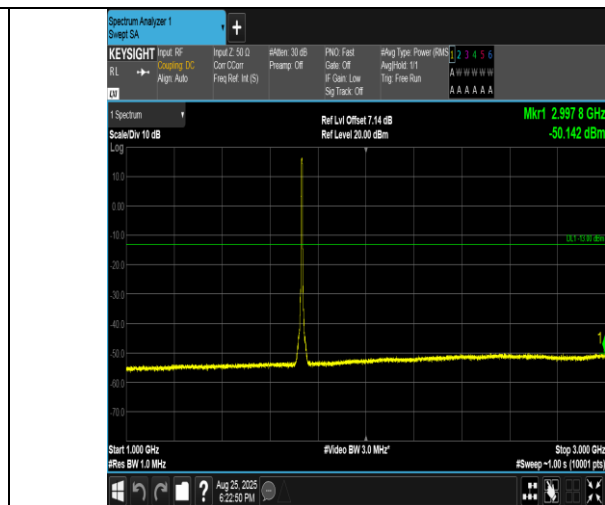
Band4-5MHz-QPSK-20175-25RB#0-1000~3000-PASS
