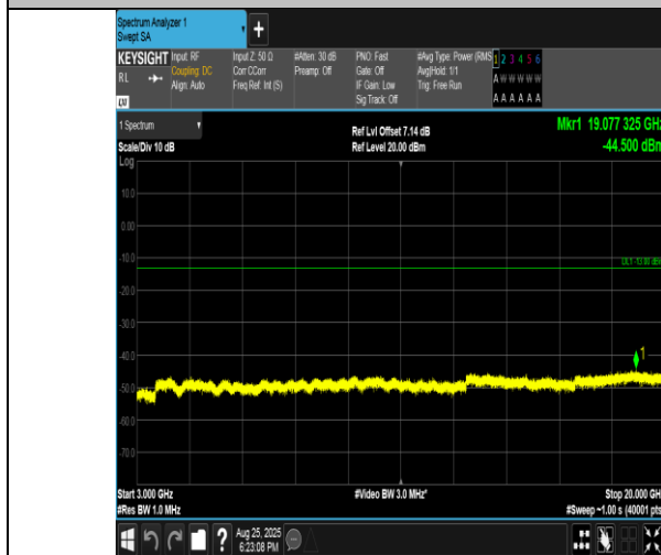
Band4-5MHz-QPSK-20175-25RB#0-3000~20000-PASS
