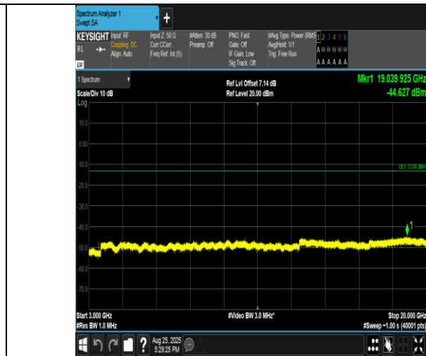
Band4-3MHz-16QAM-20385-1RB#0-3000~20000-PASS
