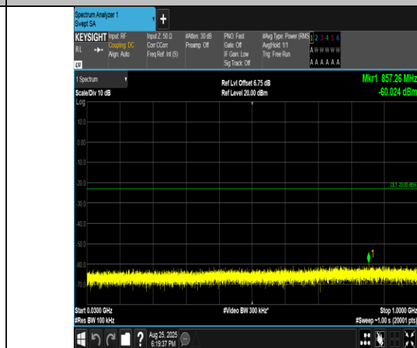
Band4-5MHz-16QAM-20175-1RB#0-30~1000-PASS
