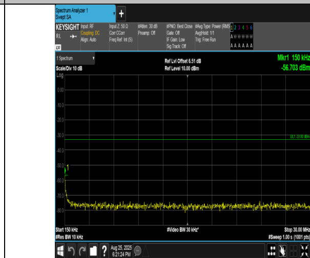
Band4-5MHz-16QAM-20175-1RB#24-0.15~30-PASS
