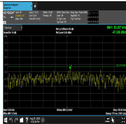
Band4-3MHz-16QAM-20385-15RB#0-0.009~0.15-PASS
