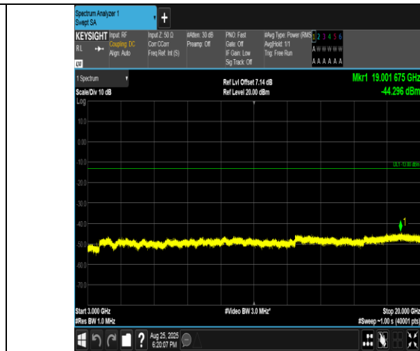
Band4-5MHz-16QAM-20175-1RB#0-3000~20000-PASS
