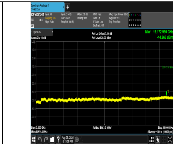
Band4-5MHz-16QAM-19975-1RB#0-3000~20000-PASS
