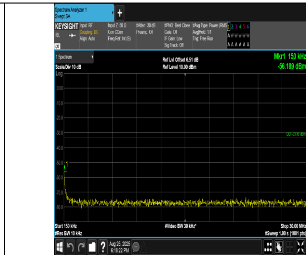
Band4-5MHz-QPSK-20175-1RB#0-0.15~30-PASS
