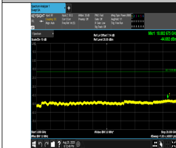
Band4-5MHz-QPSK-19975-1RB#0-3000~20000-PASS
