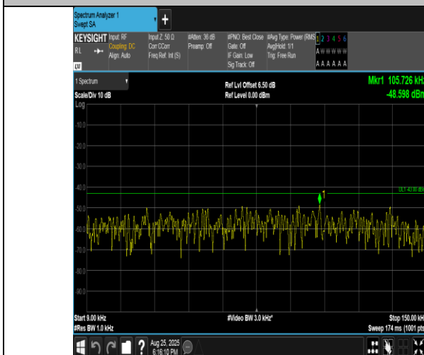
Band4-5MHz-QPSK-19975-25RB#0-0.009~0.15-PASS
