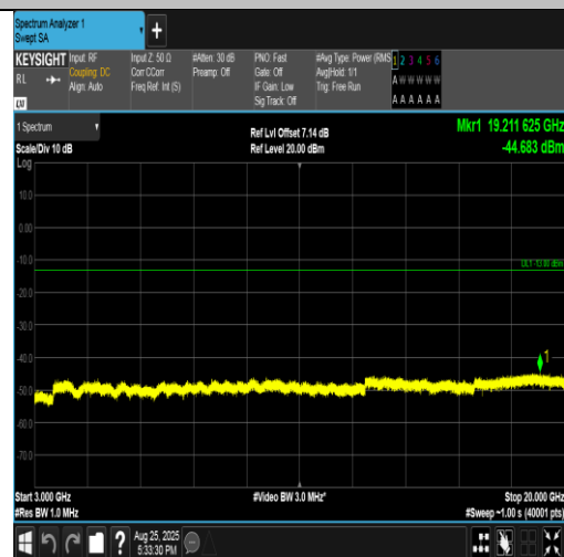
Band4-3MHz-16QAM-20385-15RB#0-3000~20000-PASS
