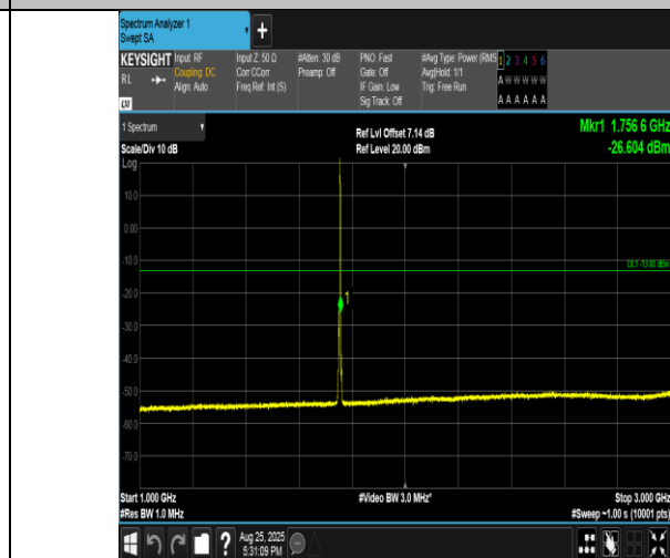
Band4-3MHz-16QAM-20385-1RB#14-1000~3000-PASS
