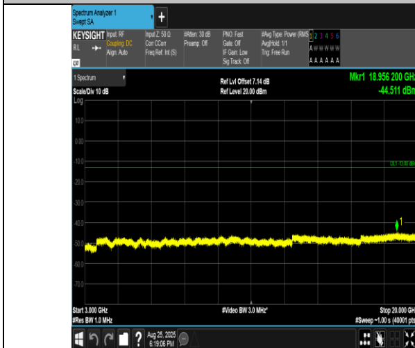
Band4-5MHz-QPSK-20175-1RB#0-3000~20000-PASS
