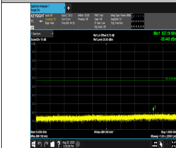
Band4-3MHz-16QAM-20385-1RB#14-30~1000-PASS
