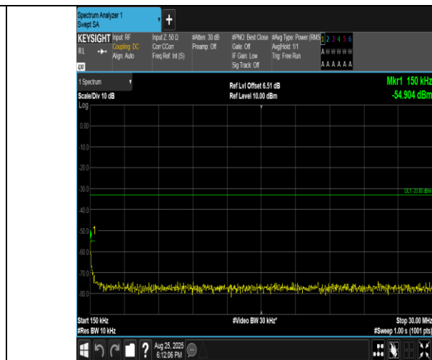
Band4-5MHz-QPSK-19975-1RB#0-0.15~30-PASS
