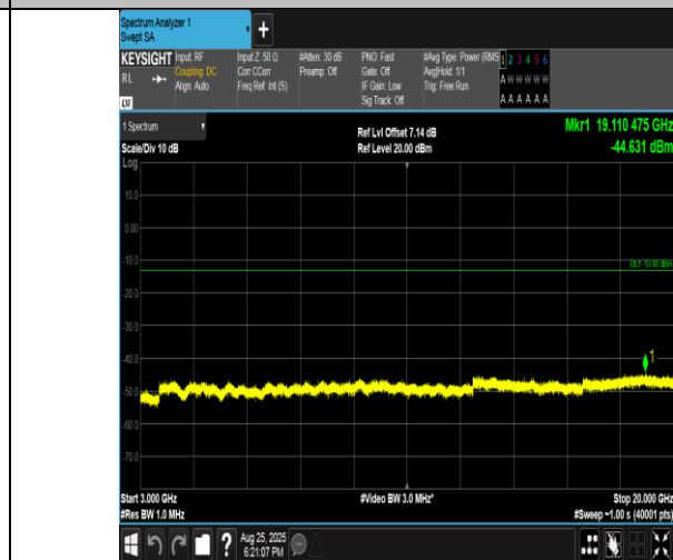
Band4-5MHz-QPSK-20175-1RB#24-3000~20000-PASS
