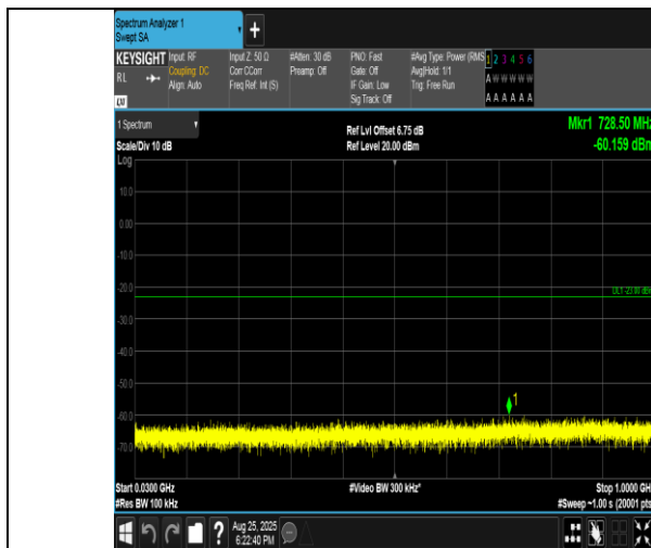
Band4-5MHz-QPSK-20175-25RB#0-30~1000-PASS
