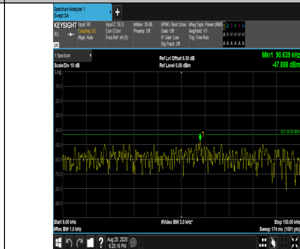
Band4-5MHz-QPSK-20175-1RB#24-0.009~0.15-PASS
