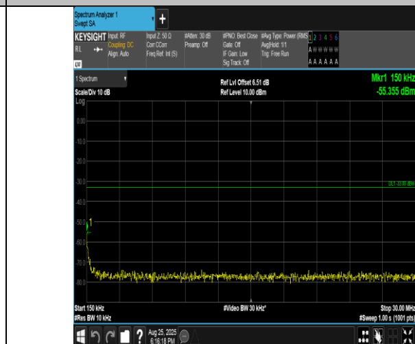
Band4-5MHz-QPSK-19975-25RB#0-0.15~30-PASS
