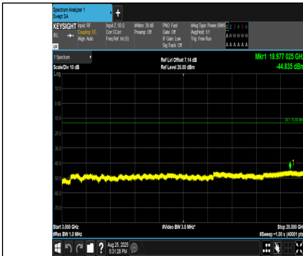
Band4-3MHz-16QAM-20385-1RB#14-3000~20000-PASS
