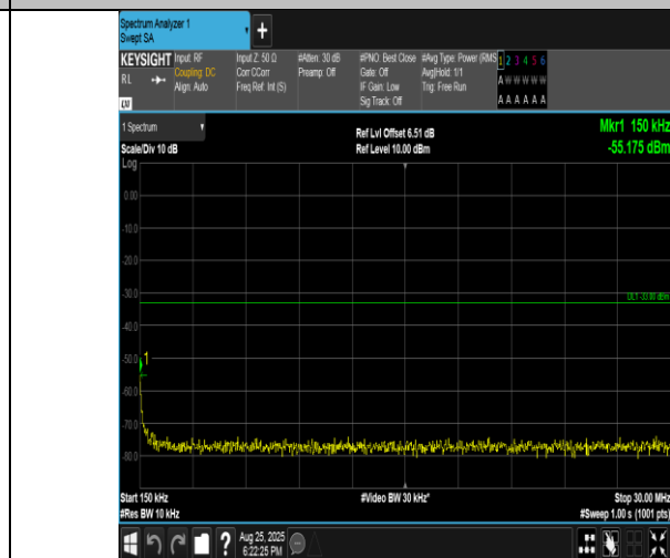
Band4-5MHz-QPSK-20175-25RB#0-0.15~30-PASS
