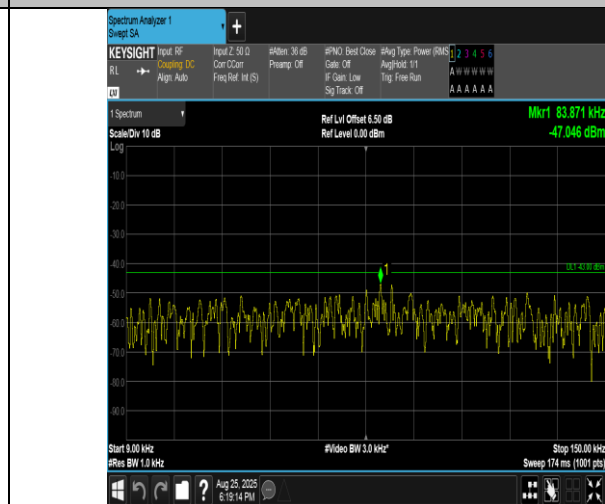
Band4-5MHz-16QAM-20175-1RB#0-0.009~0.15-PASS
