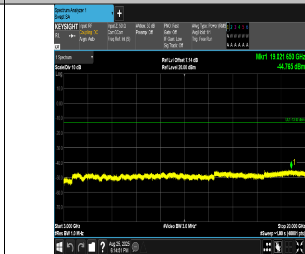
Band4-5MHz-QPSK-19975-1RB#24-3000~20000-PASS
