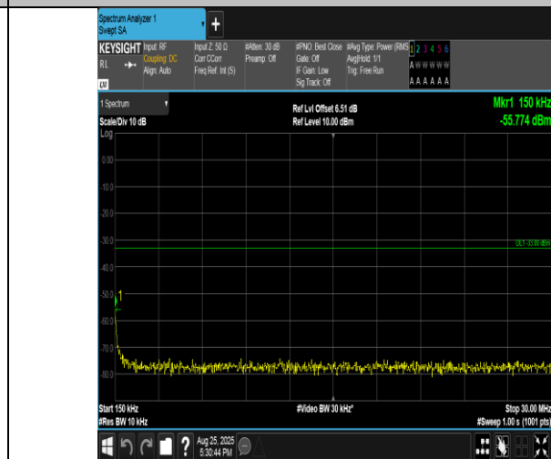
Band4-3MHz-16QAM-20385-1RB#14-0.15~30-PASS
