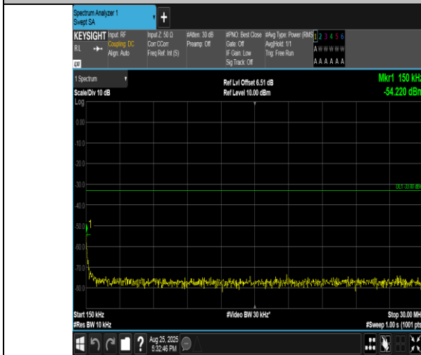
Band4-3MHz-16QAM-20385-15RB#0-0.15~30-PASS
