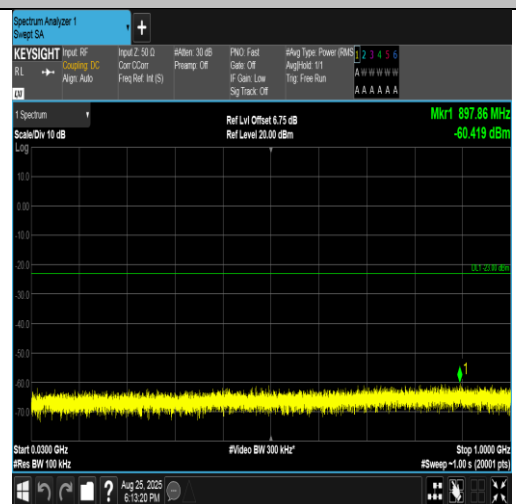
Band4-5MHz-16QAM-19975-1RB#0-30~1000-PASS
