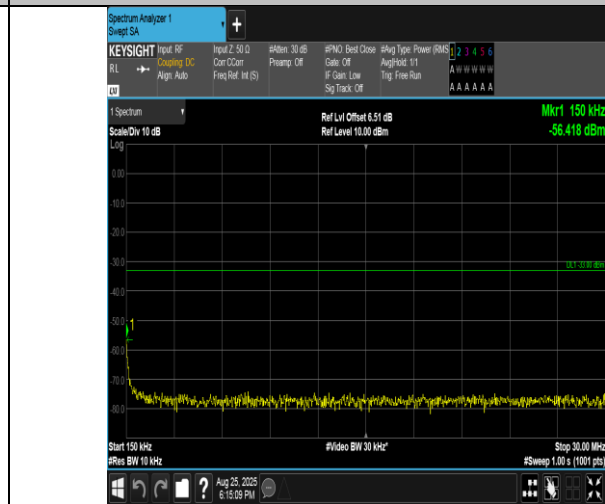
Band4-5MHz-16QAM-19975-1RB#24-0.15~30-PASS
