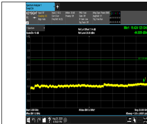
Band4-5MHz-16QAM-19975-1RB#24-3000~20000-PASS
