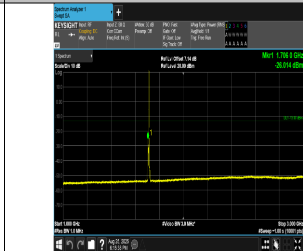
Band4-5MHz-16QAM-19975-1RB#24-1000~3000-PASS
