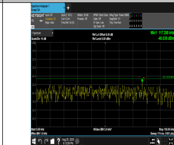
Band4-5MHz-QPSK-19975-1RB#24-0.009~0.15-PASS
