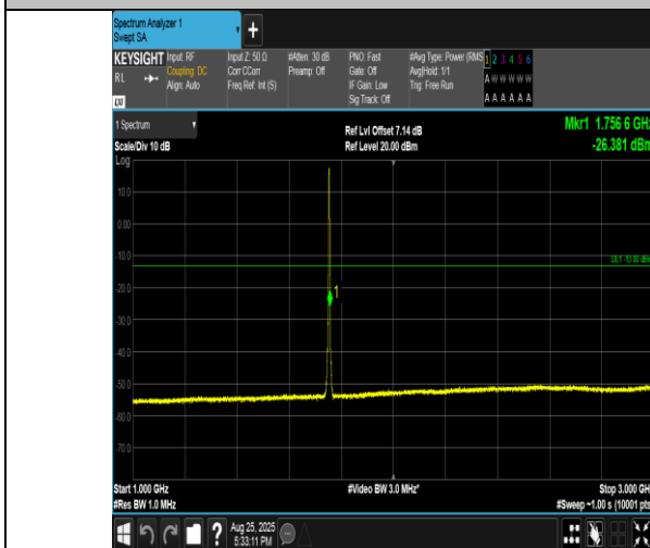
Band4-3MHz-16QAM-20385-15RB#0-1000~3000-PASS
