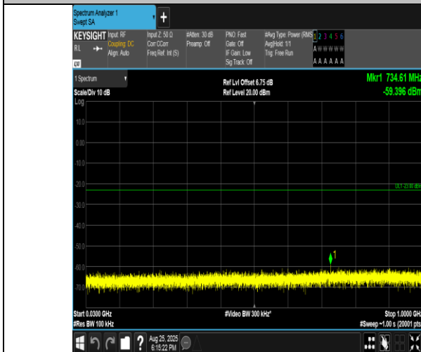
Band4-5MHz-16QAM-19975-1RB#24-30~1000-PASS
