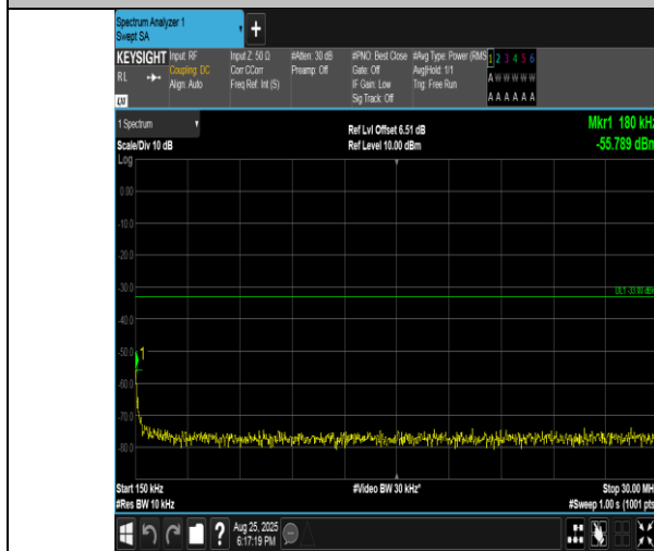
Band4-5MHz-16QAM-19975-25RB#0-0.15~30-PASS
