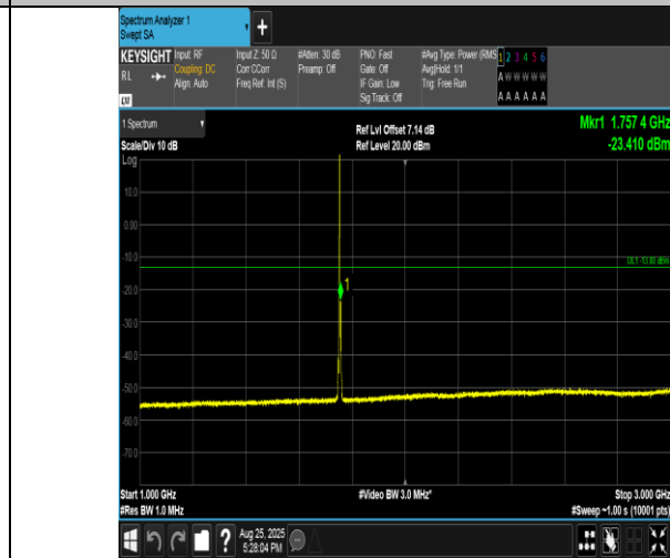
Band4-3MHz-QPSK-20385-1RB#0-1000~3000-PASS
