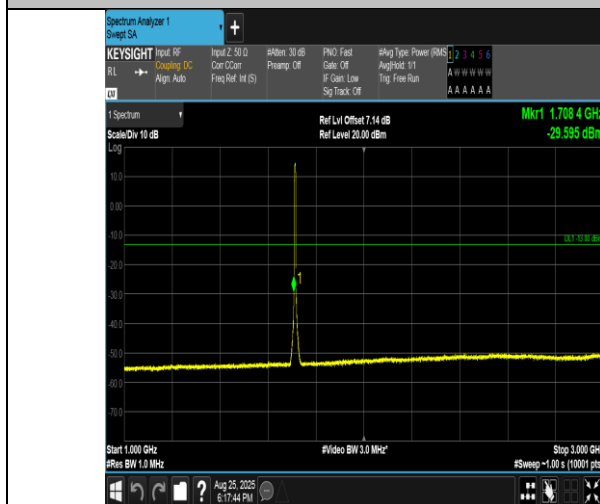
Band4-5MHz-16QAM-19975-25RB#0-1000~3000-PASS
