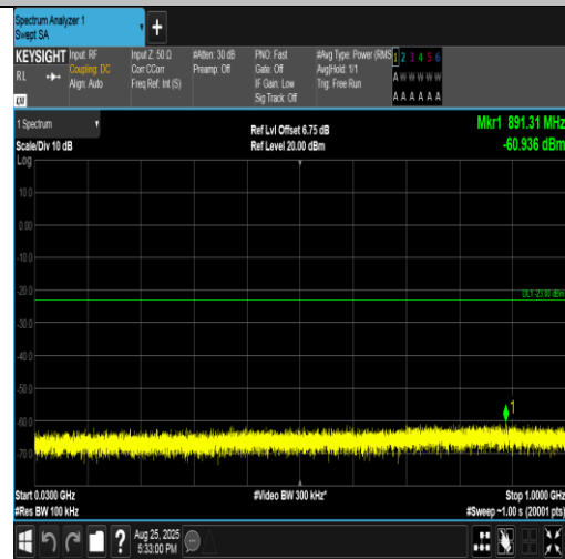
Band4-3MHz-16QAM-20385-15RB#0-30~1000-PASS
