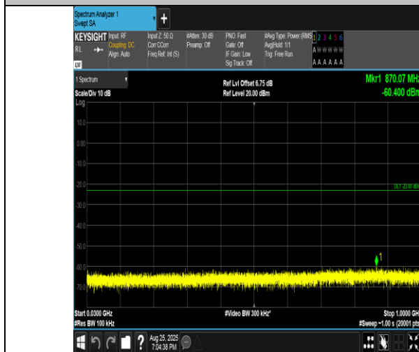
Band4-10MHz-QPSK-20175-1RB#0-30~1000-PASS
