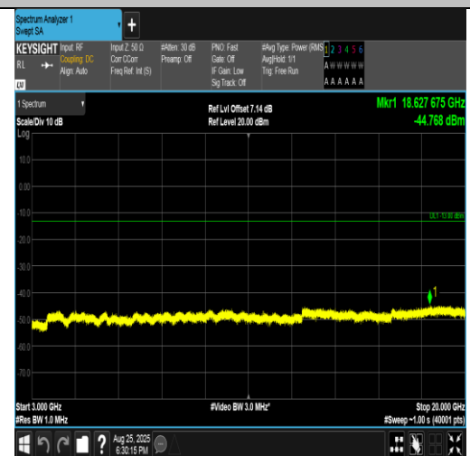
Band4-5MHz-16QAM-20375-25RB#0-3000~20000-PASS
