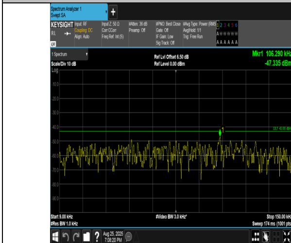
Band4-10MHz-QPSK-20175-50RB#0-0.009~0.15-PASS
