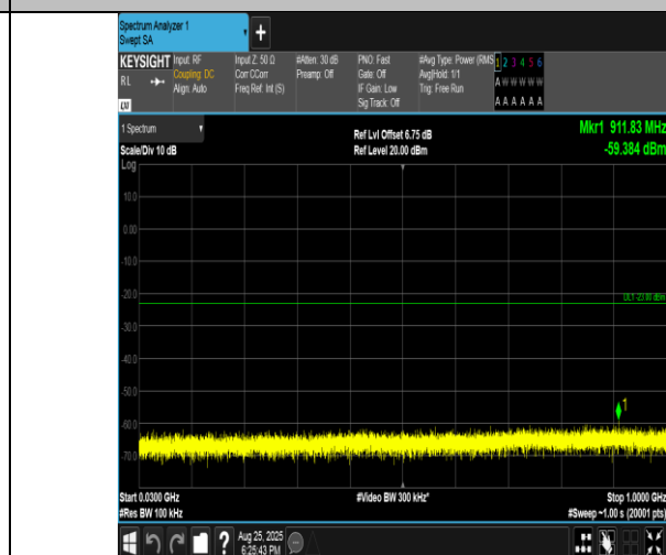
Band4-5MHz-16QAM-20375-1RB#0-30~1000-PASS
