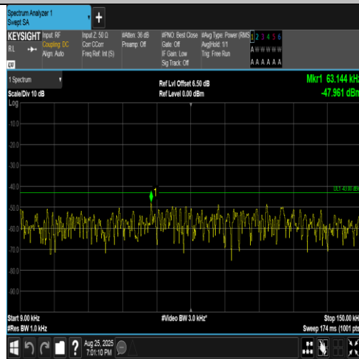
Band4-10MHz-16QAM-20000-1RB#49-0.009~0.15-PASS
