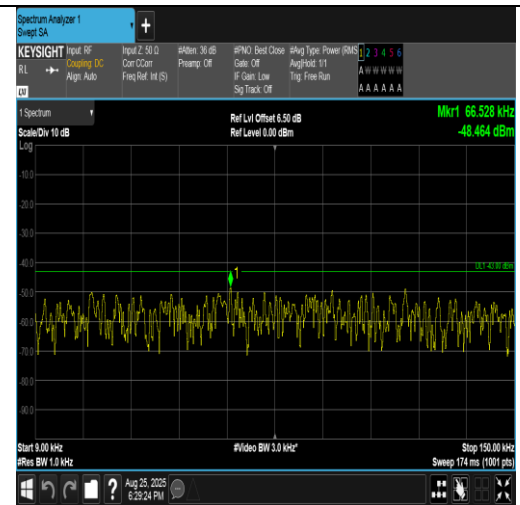
Band4-5MHz-16QAM-20375-25RB#0-0.009~0.15-PASS
