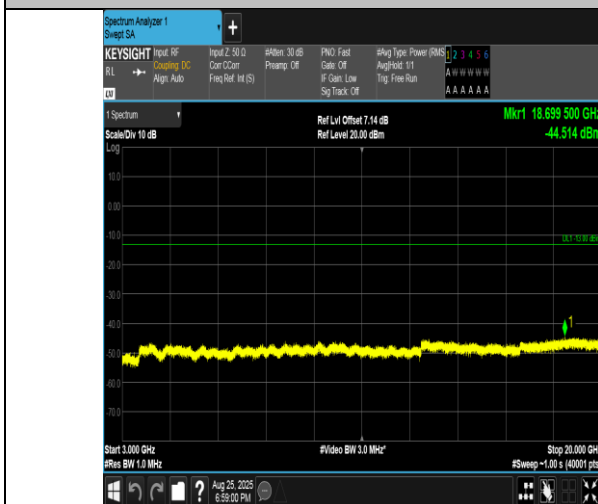
Band4-10MHz-QPSK-20000-1RB#0-3000~20000-PASS
