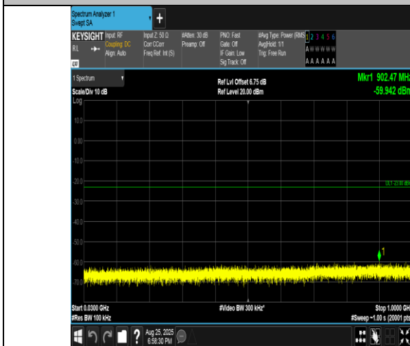
Band4-10MHz-QPSK-20000-1RB#0-30~1000-PASS
