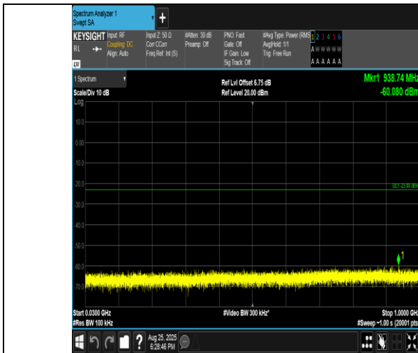
Band4-5MHz-QPSK-20375-25RB#0-30~1000-PASS
