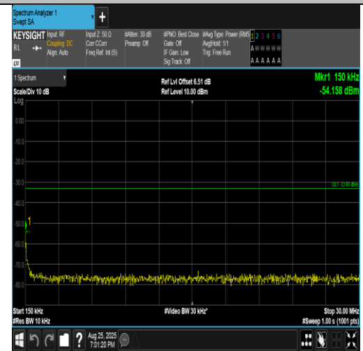
Band4-10MHz-16QAM-20000-1RB#49-0.15~30-PASS
