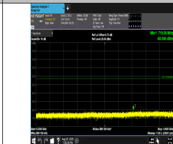
Band4-10MHz-16QAM-20175-1RB#0-30~1000-PASS
