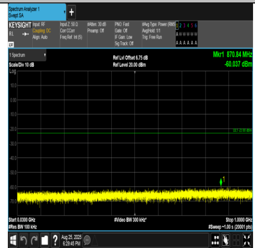
Band4-5MHz-16QAM-20375-25RB#0-30~1000-PASS
