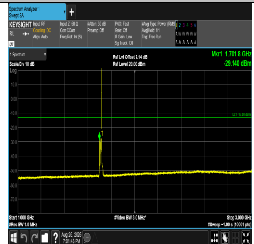
Band4-10MHz-16QAM-20000-1RB#49-1000~3000-PASS
