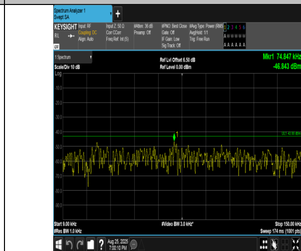
Band4-10MHz-QPSK-20000-1RB#49-0.009~0.15-PASS
