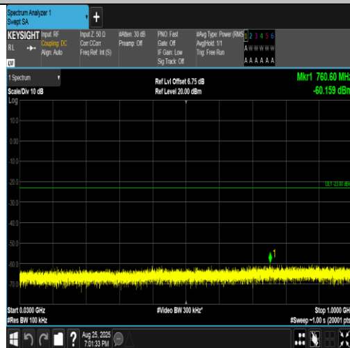
Band4-10MHz-16QAM-20000-1RB#49-30~1000-PASS
