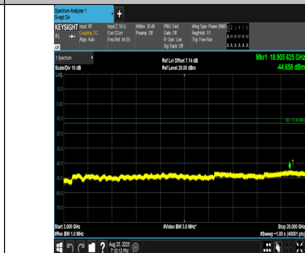
Band4-10MHz-16QAM-20175-50RB#0-3000~20000-PASS
