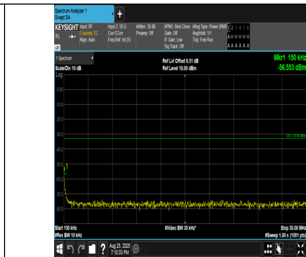
Band4-10MHz-QPSK-20350-1RB#0-0.15~30-PASS
