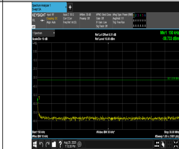
Band4-10MHz-16QAM-20350-1RB#49-0.15~30-PASS
