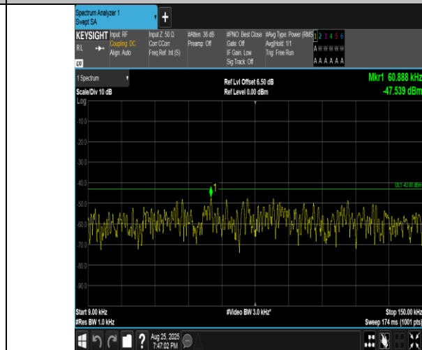
Band4-15MHz-QPSK-2025-1RB#74-0.009~0.15-PASS
