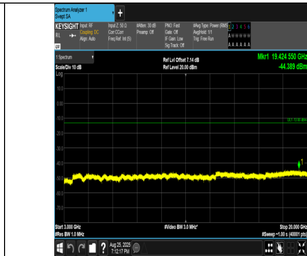
Band4-10MHz-16QAM-20350-1RB#0-3000~20000-PASS
