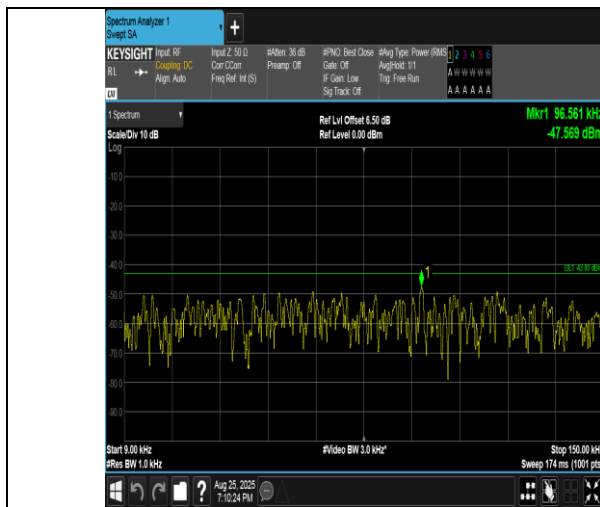
Band4-10MHz-QPSK-20350-1RB#0-0.009~0.15-PASS
