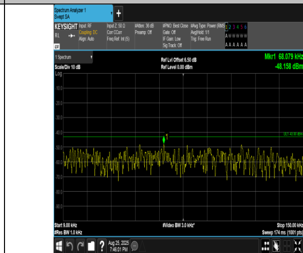
Band4-15MHz-16QAM-20025-1RB#0-0.009~0.15-PASS
