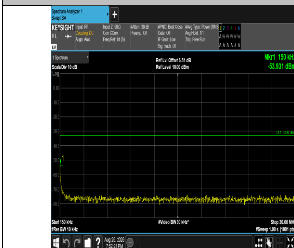
Band4-15MHz-16QAM-20175-1RB#0-0.15~30-PASS
