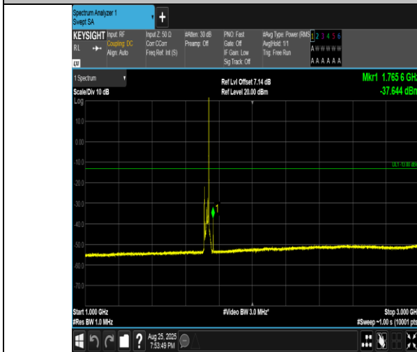
Band4-15MHz-QPSK-20175-1RB#74-1000~3000-PASS
