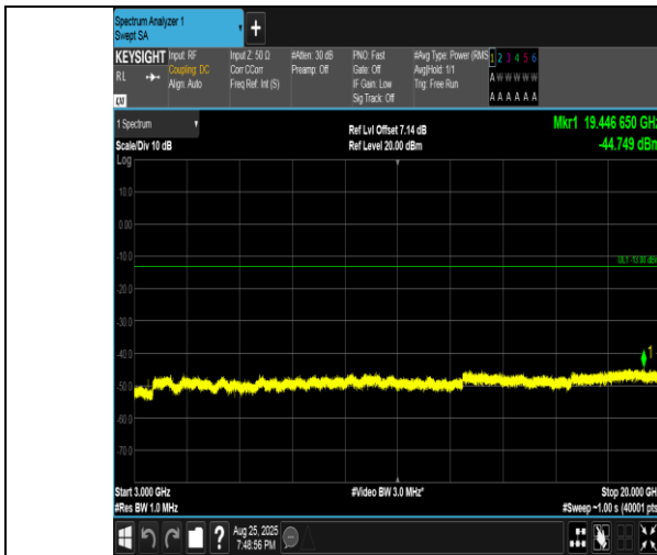
Band4-15MHz-16QAM-2025-1RB#74-3000~20000-PASS
