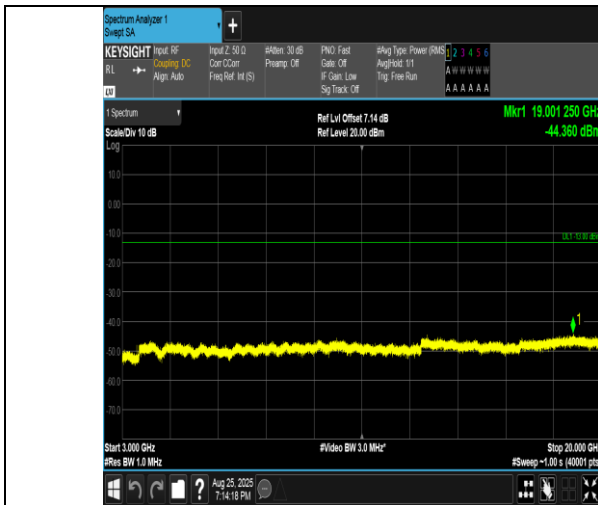
Band4-10MHz-16QAM-20350-1RB#49-3000~20000-PASS
