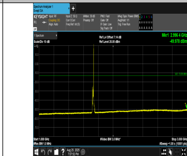
Band4-10MHz-16QAM-20175-1RB#49-1000~3000-PASS
