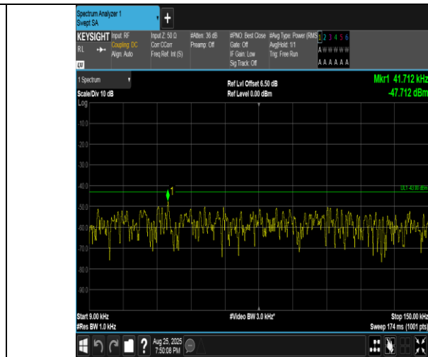
Band4-15MHz-16QAM-2025-75RB#0-0.009~0.15-PASS
