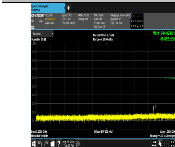
Band4-15MHz-16QAM-20025-1RB#74-30~1000-PASS
