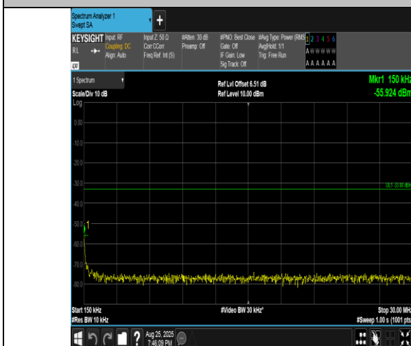
Band4-15MHz-16QAM-20025-1RB#0-0.15~30-PASS
