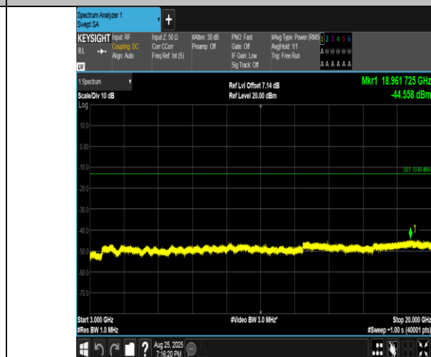
Band4-10MHz-16QAM-20350-50RB#0-3000~20000-PASS
