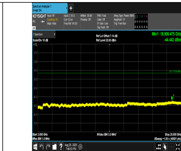
Band4-15MHz-16QAM-20025-1RB#0-3000~20000-PASS
