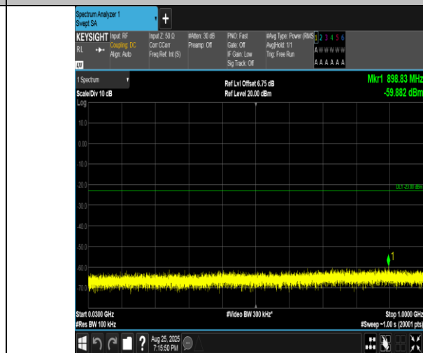
Band4-10MHz-16QAM-20350-50RB#0-30~1000-PASS
