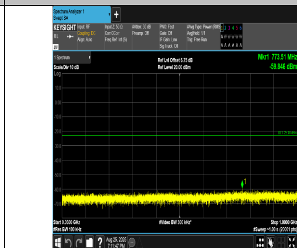
Band4-10MHz-16QAM-20350-1RB#0-30~1000-PASS
