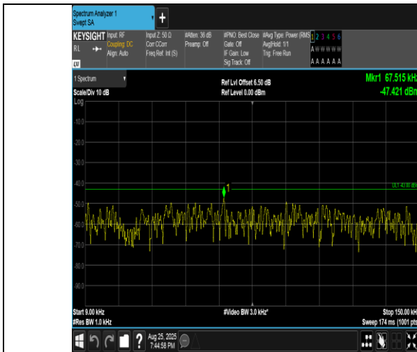
Band4-15MHz-QPSK-2025-1RB#0-0.009~0.15-PASS
