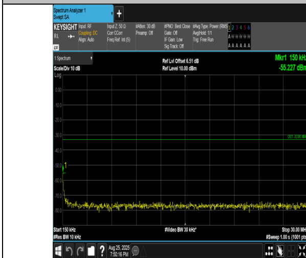
Band4-15MHz-16QAM-2025-75RB#0-0.15~30-PASS
