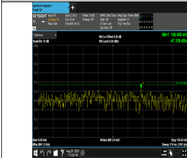
Band4-10MHz-16QAM-20350-1RB#49-0.009~0.15-PASS
