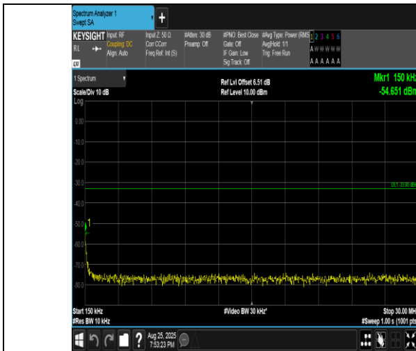
Band4-15MHz-QPSK-20175-1RB#74-0.15~30-PASS
