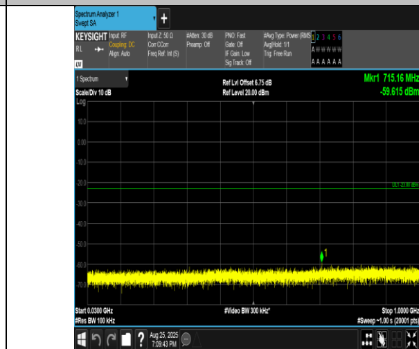
Band4-10MHz-16QAM-20175-50RB#0-30~1000-PASS
