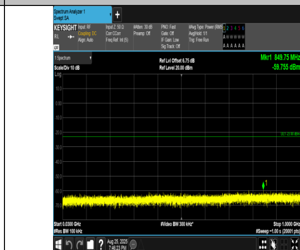
Band4-15MHz-16QAM-20025-1RB#0-30~1000-PASS
