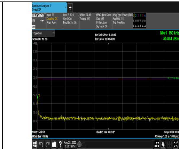
Band4-15MHz-QPSK-20175-1RB#0-0.15~30-PASS
