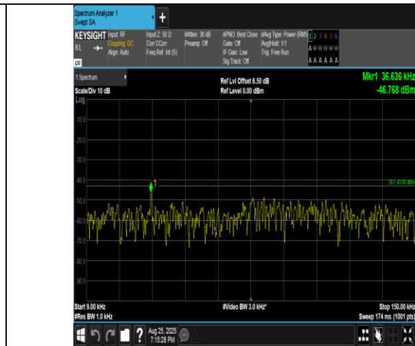
Band4-10MHz-16QAM-20350-50RB#0-0.009~0.15-PASS
