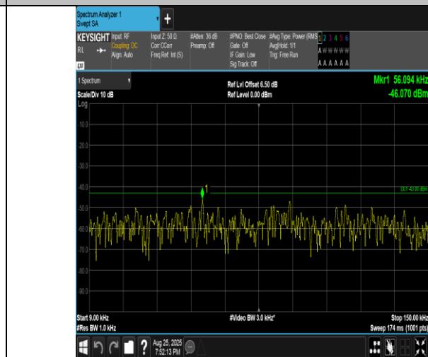
Band4-15MHz-16QAM-20175-1RB#0-0.009~0.15-PASS
