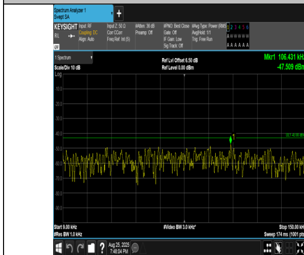
Band4-15MHz-16QAM-20025-1RB#74-0.009~0.15-PASS
