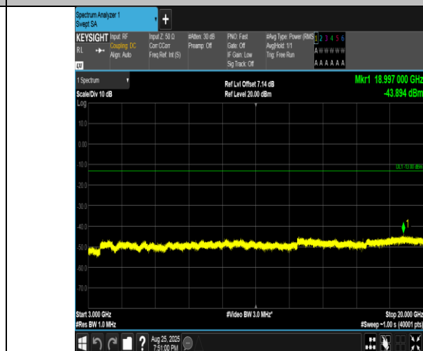
Band4-15MHz-16QAM-2025-75RB#0-3000~20000-PASS
