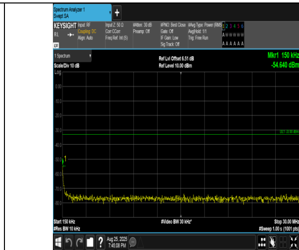
Band4-15MHz-QPSK-2025-1RB#0-0.15~30-PASS
