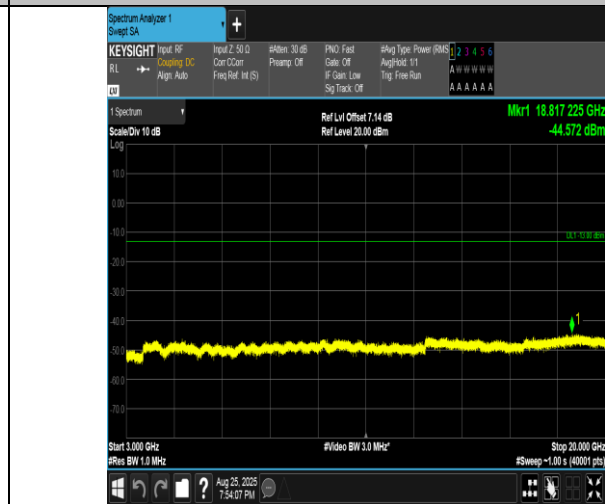
Band4-15MHz-QPSK-20175-1RB#74-3000~20000-PASS
