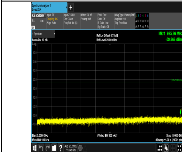
Band4-10MHz-16QAM-20350-1RB#49-30~1000-PASS
