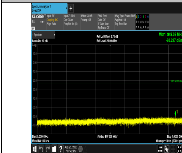
Band4-10MHz-16QAM-20175-1RB#49-30~1000-PASS
