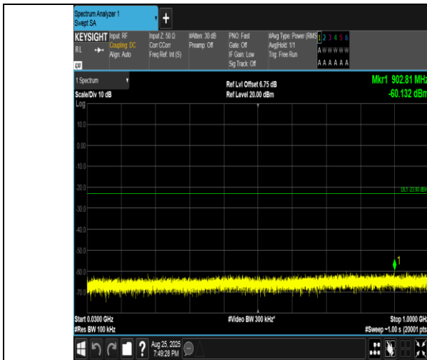
Band4-15MHz-QPSK-20025-75RB#0-30~1000-PASS
