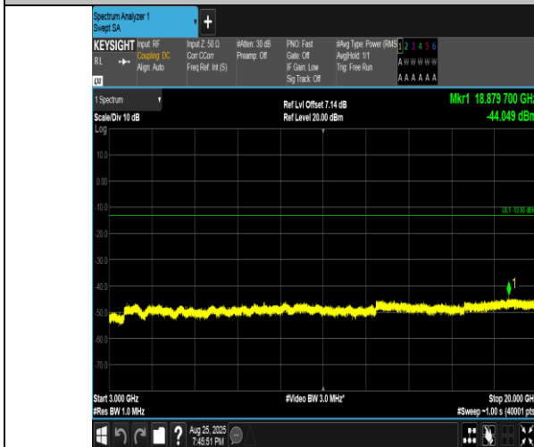
Band4-15MHz-QPSK-2025-1RB#0-3000~20000-PASS
