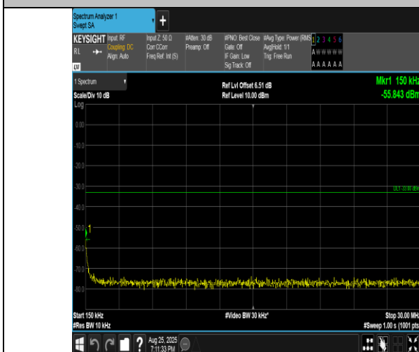
Band4-10MHz-16QAM-20350-1RB#0-0.15~30-PASS
