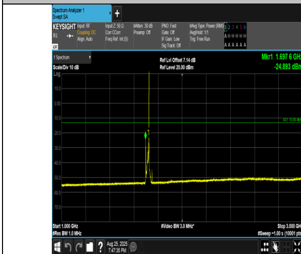
Band4-15MHz-QPSK-2025-1RB#74-1000~3000-PASS
