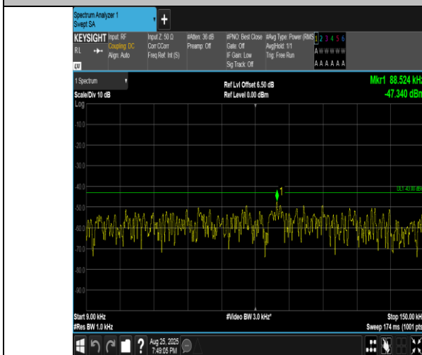
Band4-15MHz-QPSK-2025-75RB#0-0.009~0.15-PASS
