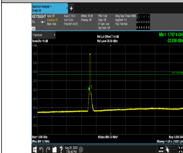
Band4-15MHz-16QAM-2025-75RB#0-1000~3000-PASS
