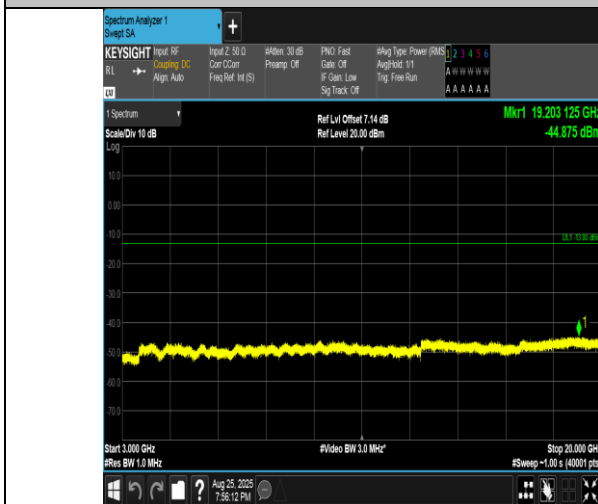
Band4-15MHz-QPSK-20175-75RB#0-3000~20000-PASS
