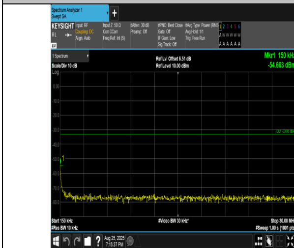
Band4-10MHz-16QAM-20350-50RB#0-0.15~30-PASS
