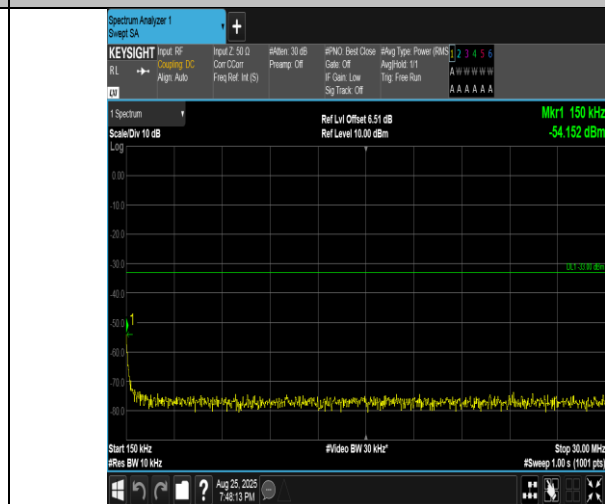
Band4-15MHz-16QAM-20025-1RB#74-0.15~30-PASS
