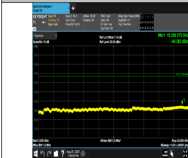
Band4-15MHz-QPSK-20025-75RB#0-3000~20000-PASS
