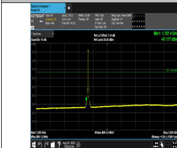
Band4-10MHz-16QAM-20175-50RB#0-1000~3000-PASS
