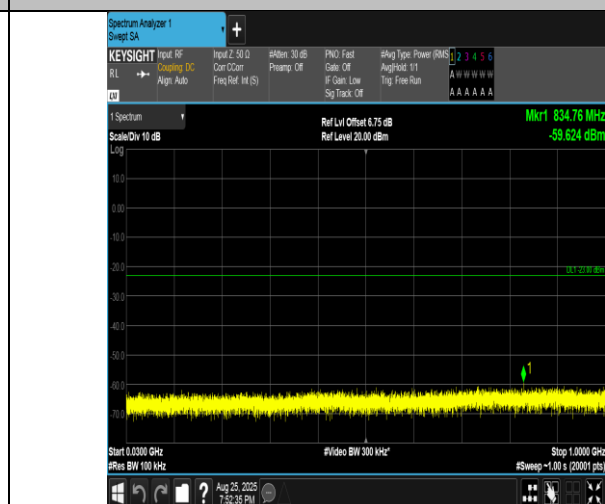
Band4-15MHz-16QAM-20175-1RB#0-30~1000-PASS
