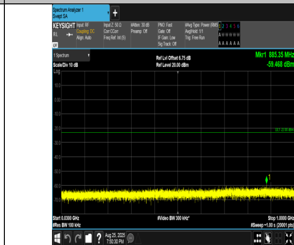
Band4-15MHz-16QAM-2025-75RB#0-30~1000-PASS
