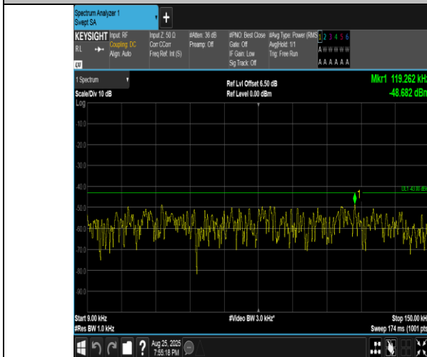
Band4-15MHz-QPSK-20175-75RB#0-0.009~0.15-PASS
