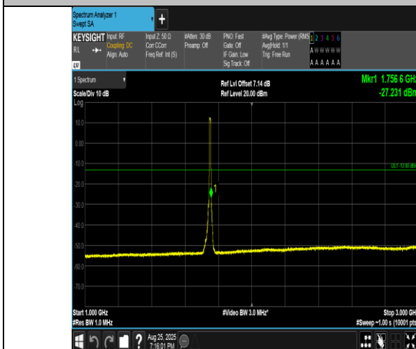
Band4-10MHz-16QAM-20350-50RB#0-1000~3000-PASS
