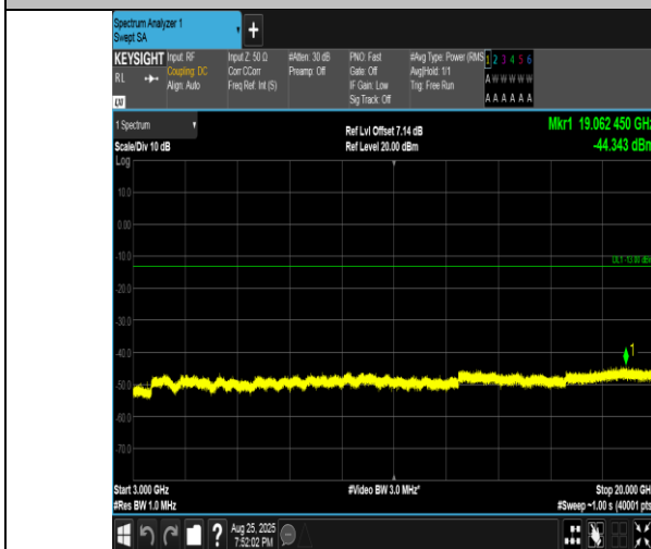
Band4-15MHz-QPSK-20175-1RB#0-3000~20000-PASS
