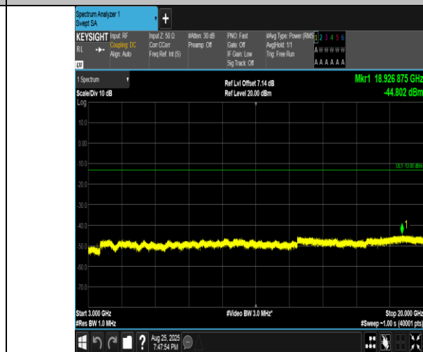
Band4-15MHz-QPSK-2025-1RB#74-3000~20000-PASS
