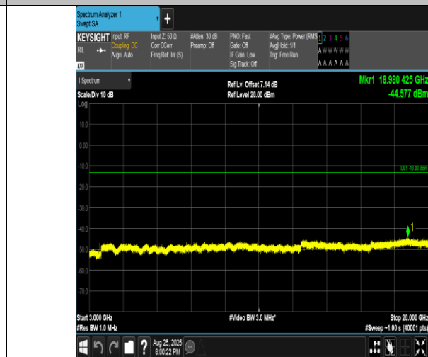
Band4-15MHz-QPSK-20325-1RB#74-3000~20000-PASS
