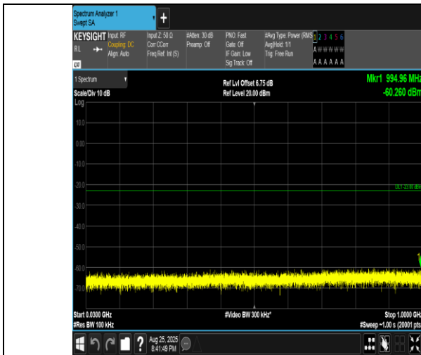
Band4-20MHz-QPSK-20175-100RB#0-30~1000-PASS
