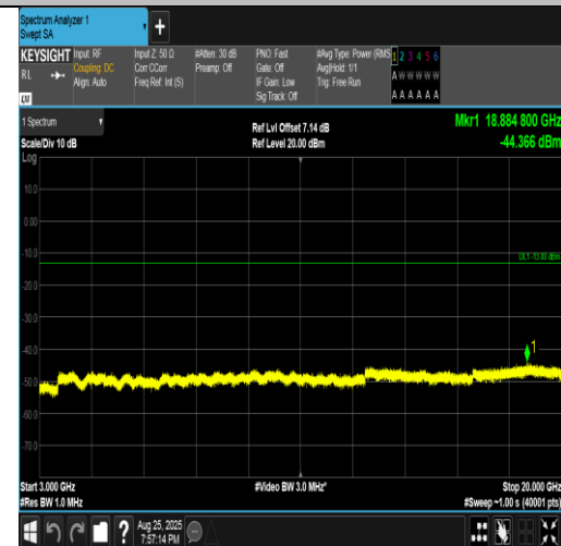
Band4-15MHz-16QAM-20175-75RB#0-3000~20000-PASS
