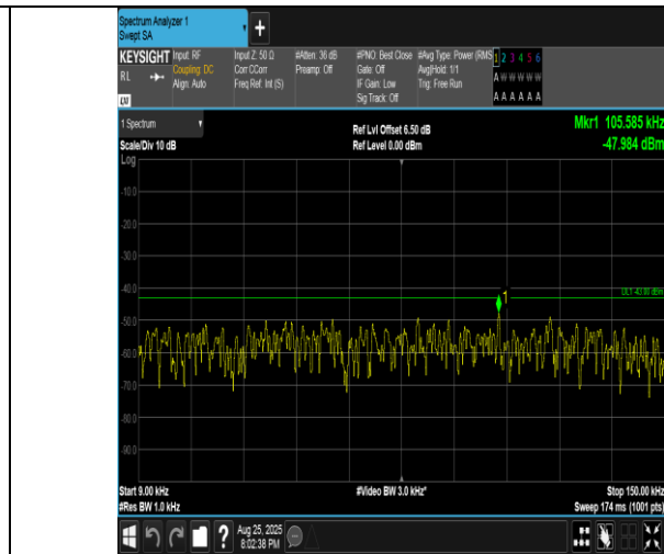
Band4-15MHz-16QAM-20325-75RB#0-0.009~0.15-PASS
