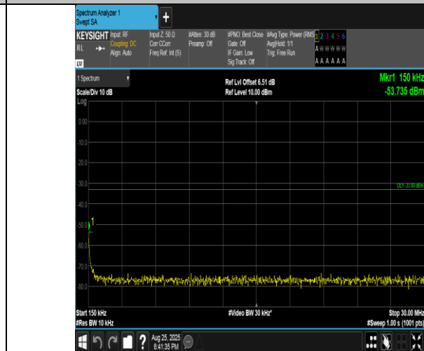
Band4-20MHz-QPSK-20175-100RB#0-0.15~30-PASS
