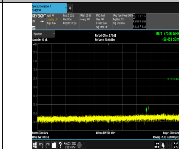
Band4-20MHz-16QAM-20050-1RB#0-30~1000-PASS
