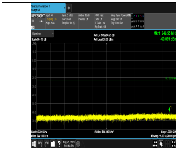
Band4-15MHz-QPSK-20325-75RB#0-30~1000-PASS
