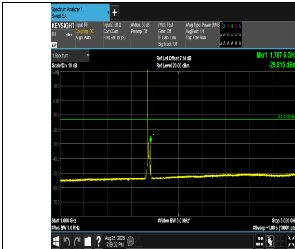
Band4-15MHz-16QAM-20325-1RB#0-1000~3000-PASS
