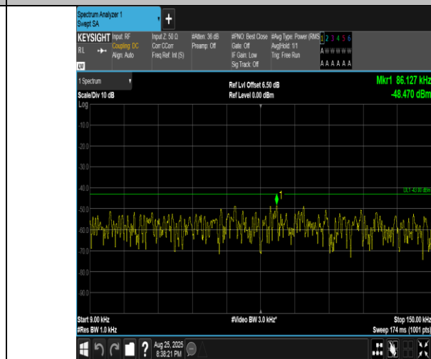
Band4-20MHz-16QAM-20175-1RB#0-0.009~0.15-PASS
