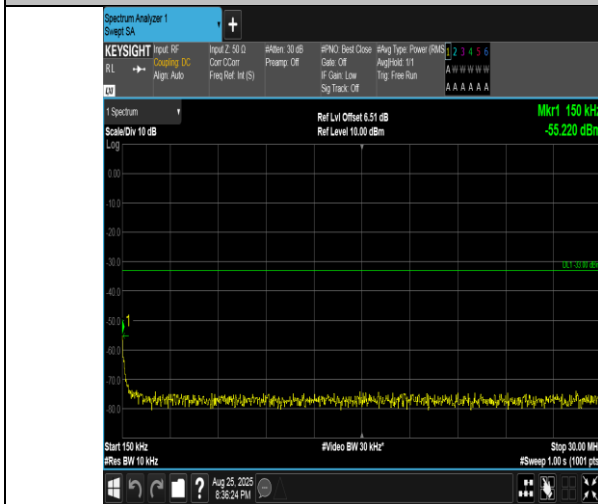
Band4-20MHz-16QAM-20050-100RB#0-0.15~30-PASS
