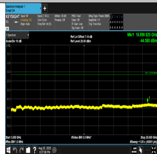
Band4-20MHz-16QAM-20050-100RB#0-3000~20000-PASS
