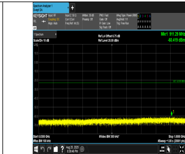
Band4-20MHz-QPSK-20175-1RB#99-30~1000-PASS
