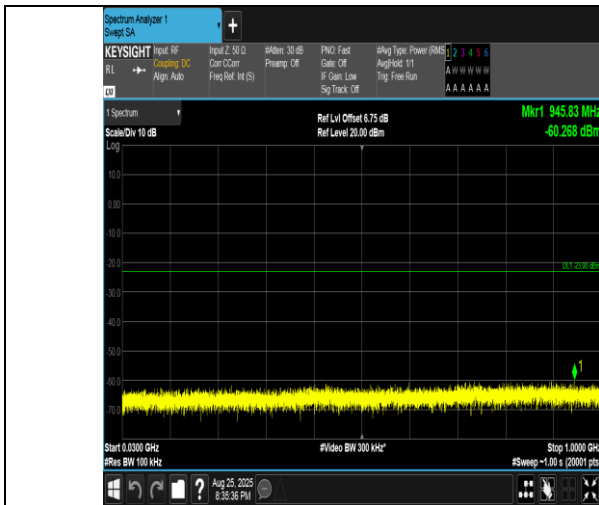
Band4-20MHz-QPSK-20050-100RB#0-30~1000-PASS
