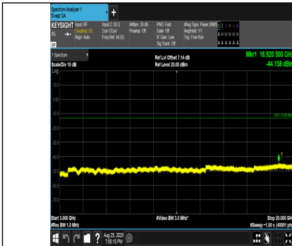
Band4-15MHz-16QAM-20175-1RB#74-3000~20000-PASS
