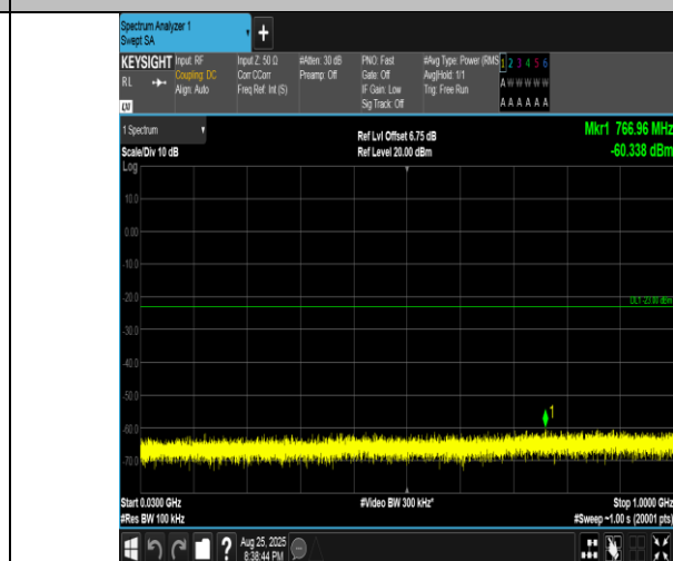
Band4-20MHz-16QAM-20175-1RB#0-30~1000-PASS
