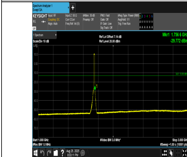
Band4-15MHz-16QAM-20325-75RB#0-1000~3000-PASS
