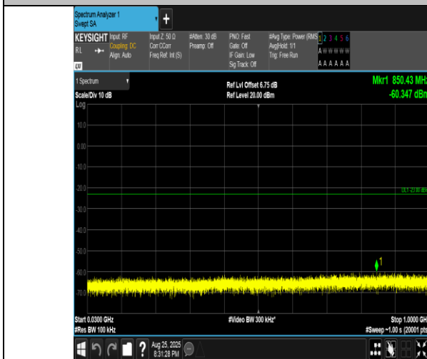
Band4-20MHz-QPSK-20050-1RB#0-30~1000-PASS
