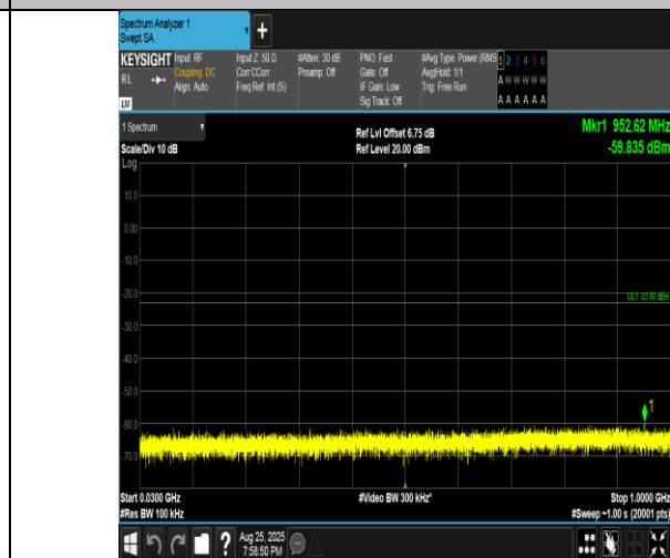
Band4-15MHz-16QAM-20325-1RB#0-30~1000-PASS
