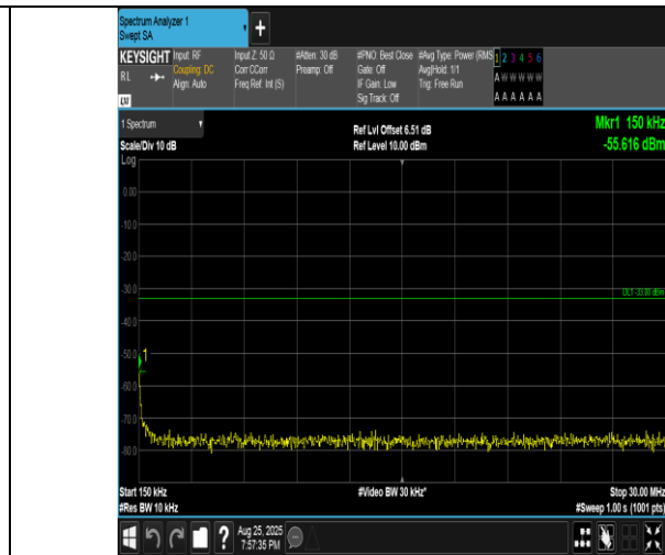
Band4-15MHz-QPSK-20325-1RB#0-0.15~30-PASS
