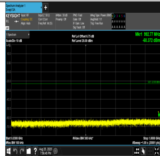
Band4-15MHz-16QAM-20175-75RB#0-30~1000-PASS
