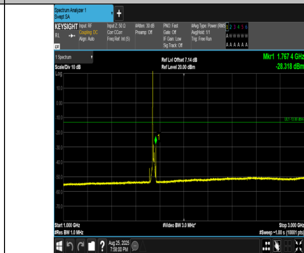
Band4-15MHz-QPSK-20325-1RB#0-1000~3000-PASS
