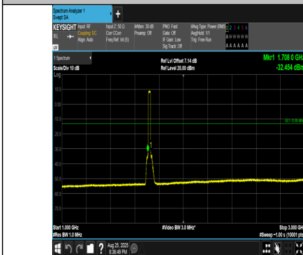
Band4-20MHz-16QAM-20050-100RB#0-1000~3000-PASS
