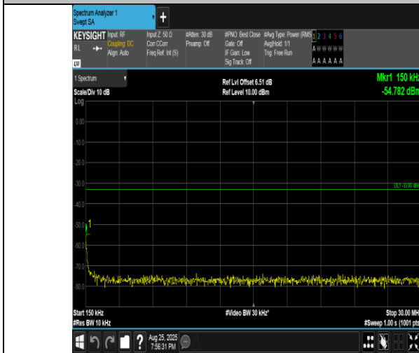
Band4-15MHz-16QAM-20175-75RB#0-0.15~30-PASS
