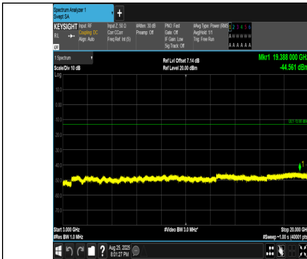
Band4-15MHz-16QAM-20325-1RB#74-3000~20000-PASS
