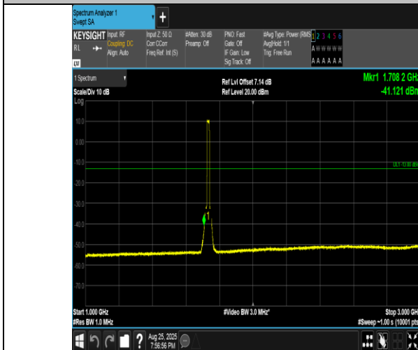
Band4-15MHz-16QAM-20175-75RB#0-1000~3000-PASS
