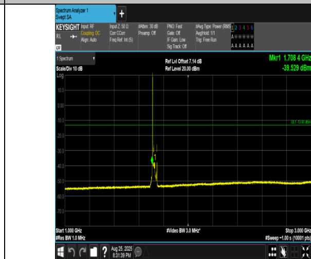
Band4-20MHz-QPSK-20050-1RB#0-1000~3000-PASS
