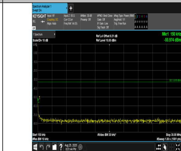
Band4-15MHz-QPSK-20325-75RB#0-0.15~30-PASS
