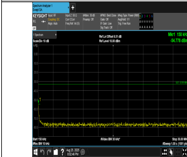
Band4-15MHz-16QAM-20325-75RB#0-0.15~30-PASS
