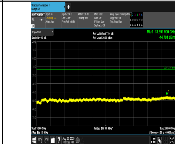
Band4-15MHz-16QAM-20325-75RB#0-3000~20000-PASS
