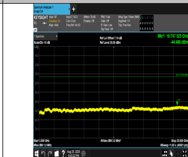
Band4-20MHz-16QAM-20175-100RB#0-3000~20000-PASS
