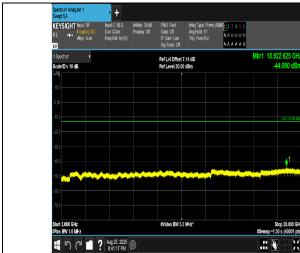
Band4-20MHz-16QAM-20175-1RB#99-3000~20000-PASS
