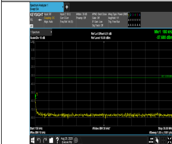
Band4-20MHz-16QAM-20300-1RB#0-0.15~30-PASS
