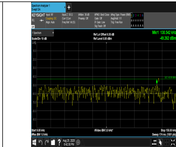
Band4-20MHz-16QAM-20175-100RB#0-0.009~0.15-PASS
