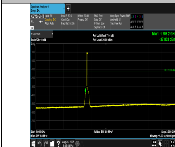
Band4-20MHz-16QAM-20175-100RB#0-1000~3000-PASS
