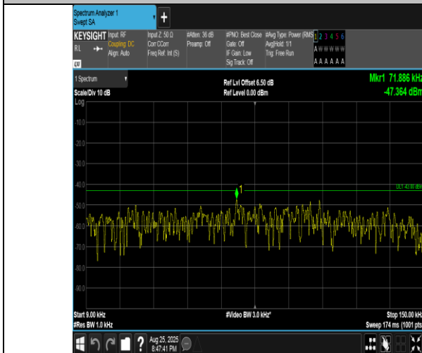
Band4-20MHz-QPSK-20300-100RB#0-0.009~0.15-PASS
