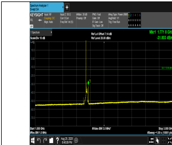
Band4-20MHz-16QAM-20300-1RB#0-1000~3000-PASS
