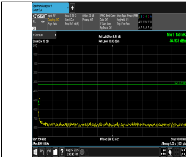
Band4-20MHz-QPSK-20300-1RB#99-0.15~30-PASS
