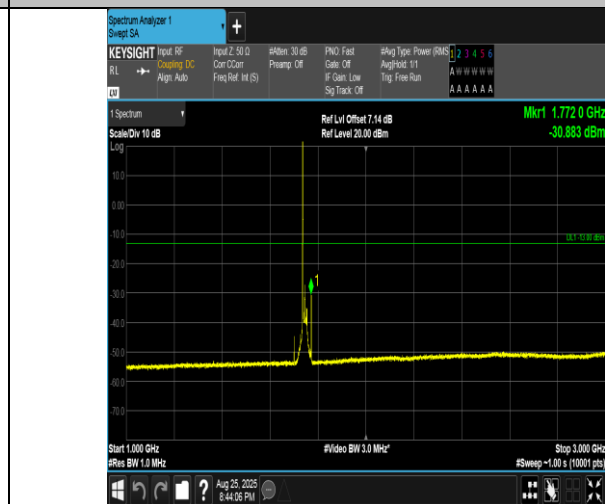
Band4-20MHz-QPSK-20300-1RB#0-1000~3000-PASS
