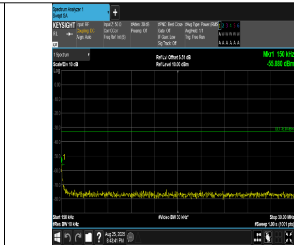
Band4-20MHz-QPSK-20300-1RB#0-0.15~30-PASS
