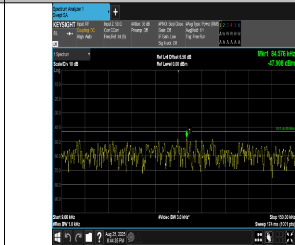
Band4-20MHz-16QAM-20300-1RB#0-0.009~0.15-PASS
