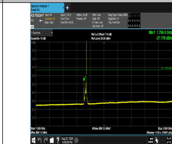
Band4-20MHz-16QAM-20175-1RB#99-1000~3000-PASS
