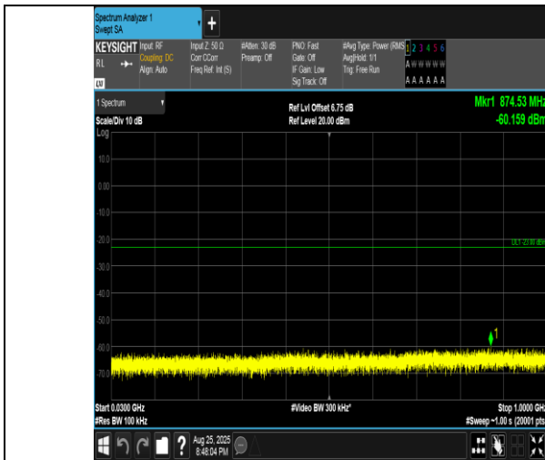
Band4-20MHz-QPSK-20300-100RB#0-30~1000-PASS
