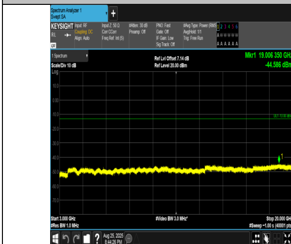
Band4-20MHz-QPSK-20300-1RB#0-3000~20000-PASS
