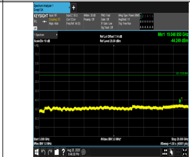
Band4-20MHz-QPSK-20300-1RB#99-3000~20000-PASS
