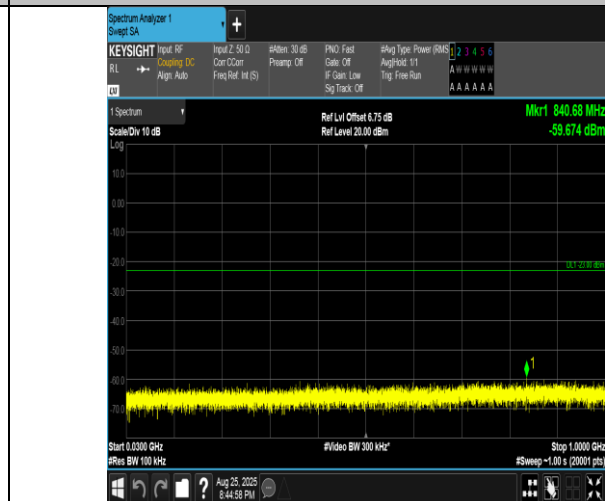
Band4-20MHz-16QAM-20300-1RB#0-30~1000-PASS
