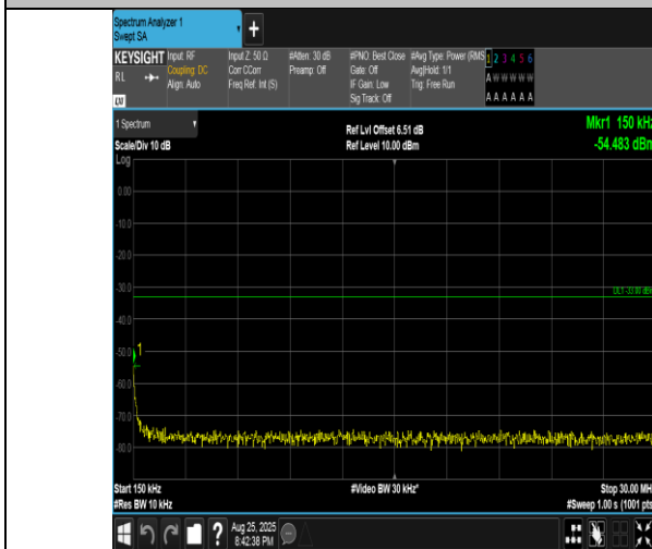
Band4-20MHz-16QAM-20175-100RB#0-0.15~30-PASS
