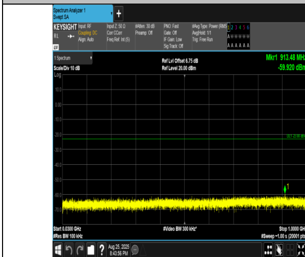
Band4-20MHz-QPSK-20300-1RB#0-30~1000-PASS
