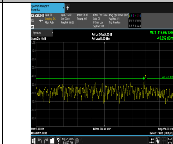
Band4-20MHz-QPSK-20300-1RB#99-0.009~0.15-PASS
