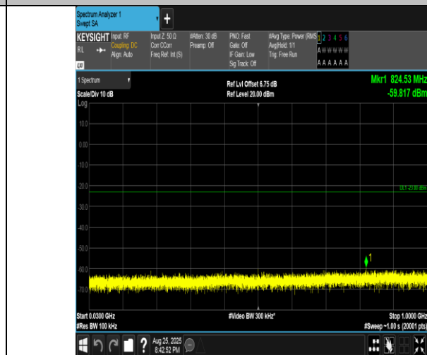
Band4-20MHz-16QAM-20175-100RB#0-30~1000-PASS
