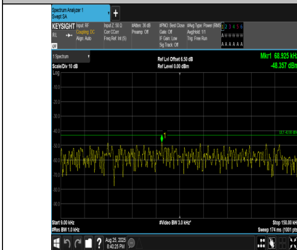
Band4-20MHz-16QAM-20175-1RB#99-0.009~0.15-PASS
