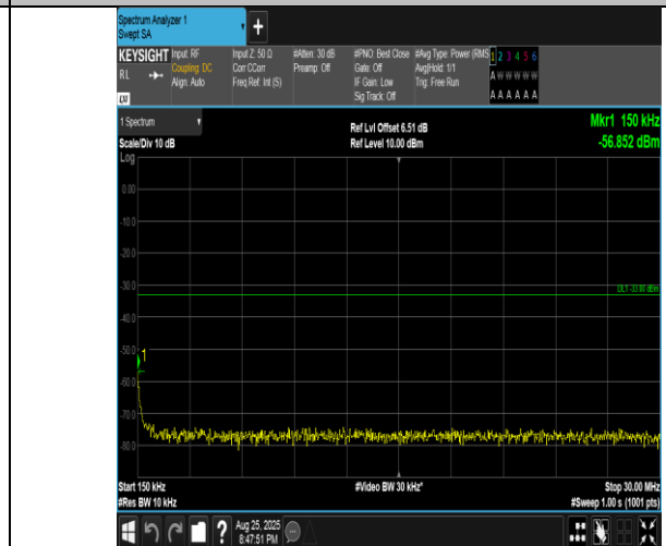
Band4-20MHz-QPSK-20300-100RB#0-0.15~30-PASS
