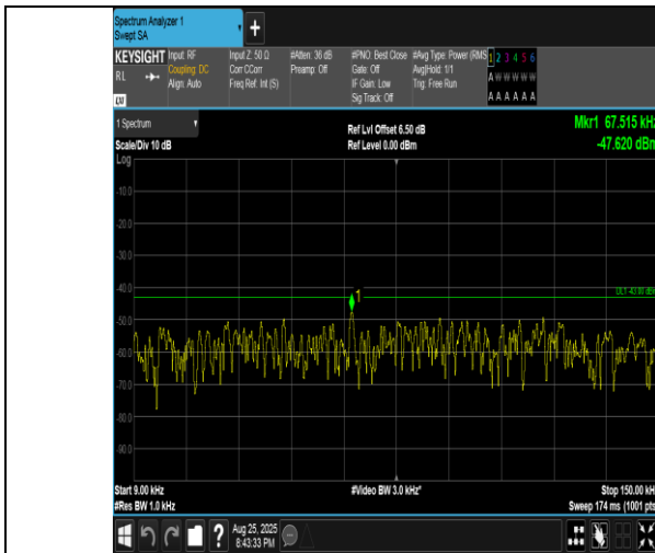
Band4-20MHz-QPSK-20300-1RB#0-0.009~0.15-PASS
