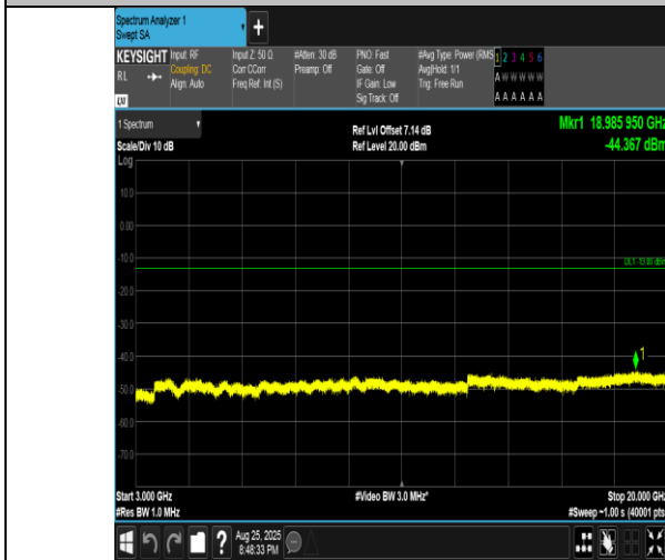
Band4-20MHz-QPSK-20300-100RB#0-3000~20000-PASS
