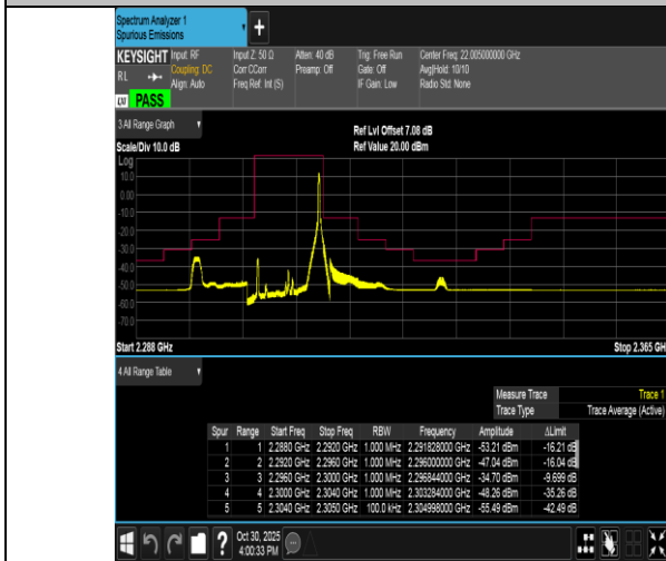
Band40(2305-2315)-10MHz-16QAM-38750-1RB#49-PASS
