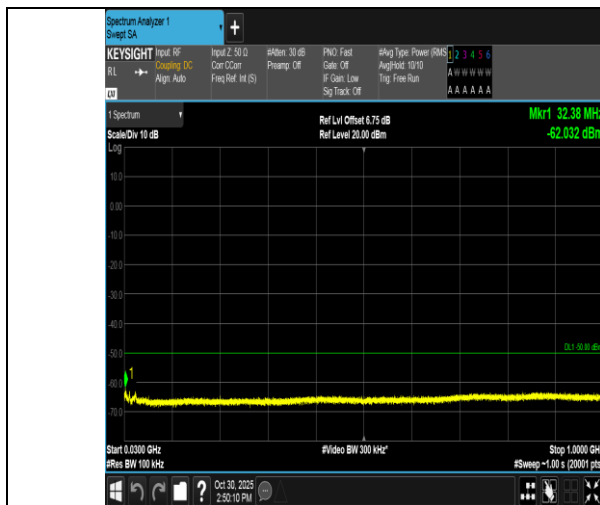
Band40(2305-2315)-5MHz-16QAM-38725-1RB#24-30~1000-PASS
