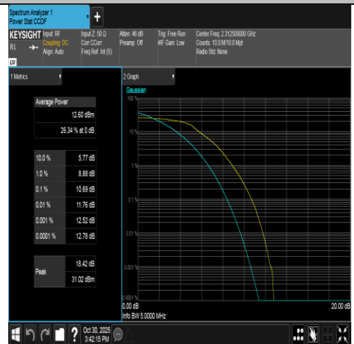
Band40(2305-2315)-5MHz-QPSK-38775-25RB#0-PASS
