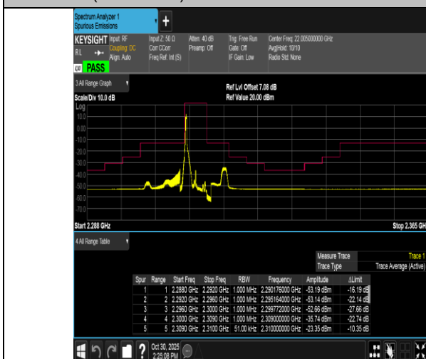
Band40(2305-2315)-5MHz-QPSK-38775-1RB#0-PASS
