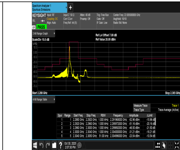
Band40(2305-2315)-5MHz-16QAM-38725-1RB#0-PASS
