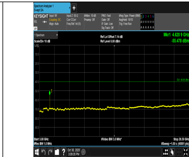
Band40(2305-2315)-5MHz-QPSK-38775-1RB#0-3000~26500-PASS
