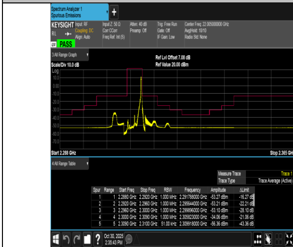
Band40(2305-2315)-5MHz-16QAM-38775-1RB#24-PASS
