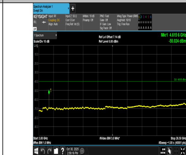
Band40(2305-2315)-5MHz-16QAM-38750-1RB#0-3000~26500-PASS
