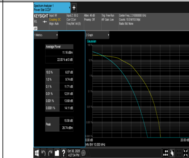
Band40(2305-2315)-10MHz-16QAM-38750-50RB#0-PASS
