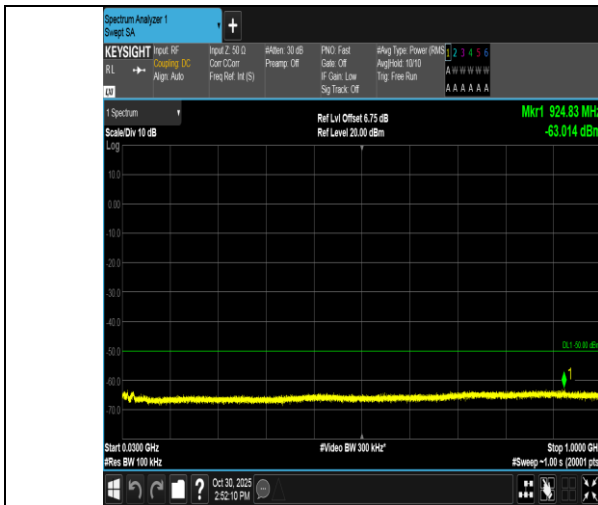
Band40(2305-2315)-5MHz-QPSK-38725-25RB#0-30~1000-PASS
