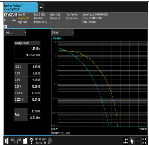
Band40(2305-2315)-5MHz-16QAM-38750-25RB#0-PASS
