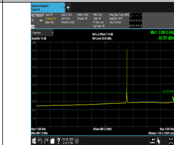
Band40(2305-2315)-5MHz-QPSK-38775-1RB#24-1000~3000-PASS
