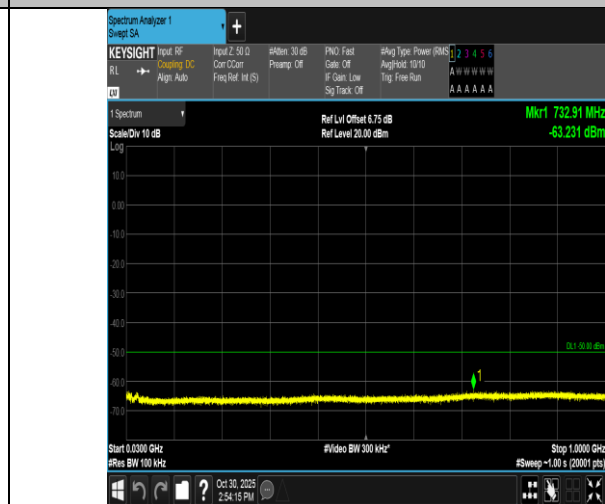
Band40(2305-2315)-5MHz-16QAM-38725-25RB#0-30~1000-PASS
