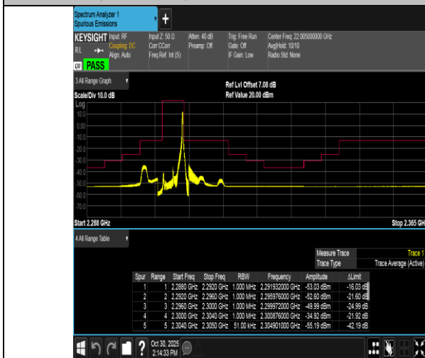
Band40(2305-2315)-5MHz-16QAM-38725-1RB#24-PASS
