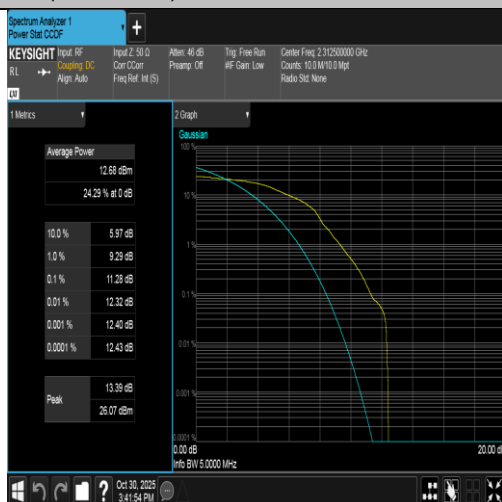
Band40(2305-2315)-5MHz-16QAM-38775-1RB#0-PASS
