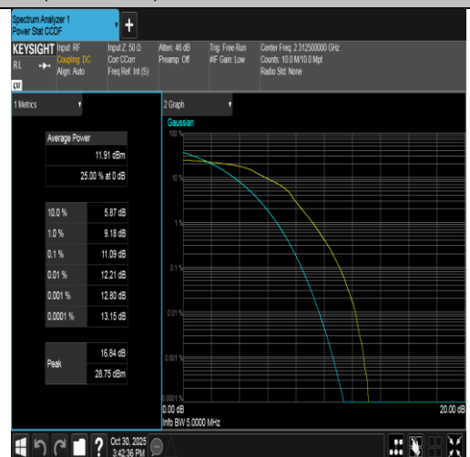
Band40(2305-2315)-5MHz-16QAM-38775-25RB#0-PASS
