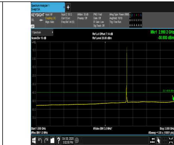
Band40(2305-2315)-5MHz-16QAM-38750-1RB#24-1000~3000-PASS
