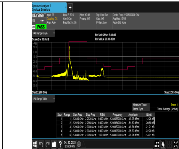
Band40(2305-2315)-10MHz-16QAM-38750-1RB#0-PASS
