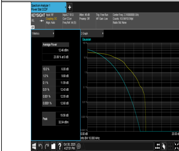
Band40(2305-2315)-10MHz-16QAM-38750-1RB#0-PASS
