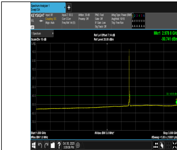
Band40(2305-2315)-5MHz-QPSK-38775-1RB#0-1000~3000-PASS
