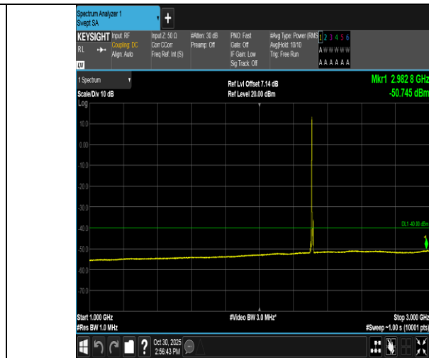
Band40(2305-2315)-5MHz-QPSK-38750-1RB#0-1000~3000-PASS
