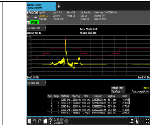
Band40(2305-2315)-5MHz-16QAM-38775-1RB#0-PASS
