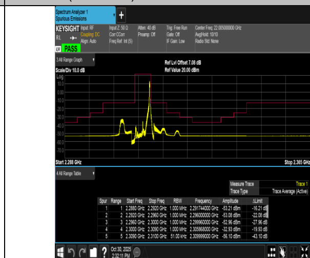
Band40(2305-2315)-5MHz-QPSK-38775-1RB#24-PASS
