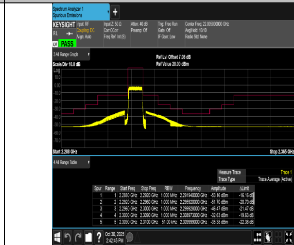
Band40(2305-2315)-5MHz-16QAM-38775-25RB#0-PASS
