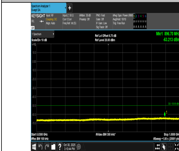
Band40(2305-2315)-5MHz-16QAM-38775-1RB#0-30~1000-PASS
