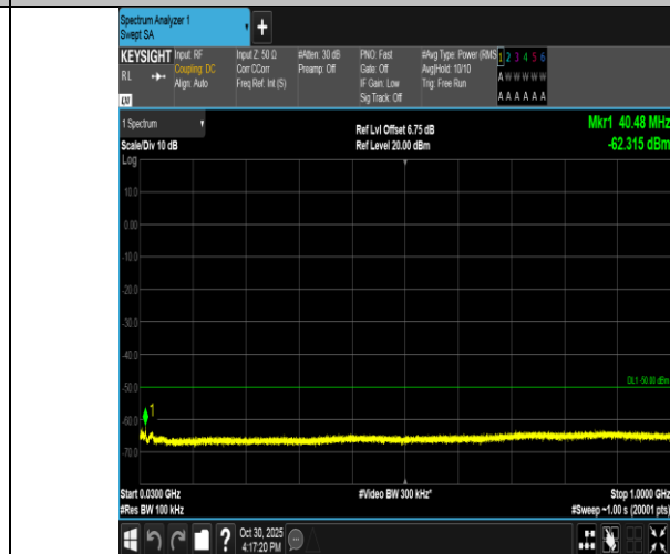
Band40(2305-2315)-10MHz-QPSK-38750-50RB#0-30~1000-PASS
