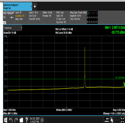
Band40(2305-2315)-5MHz-16QAM-38775-25RB#0-1000~3000-PASS
