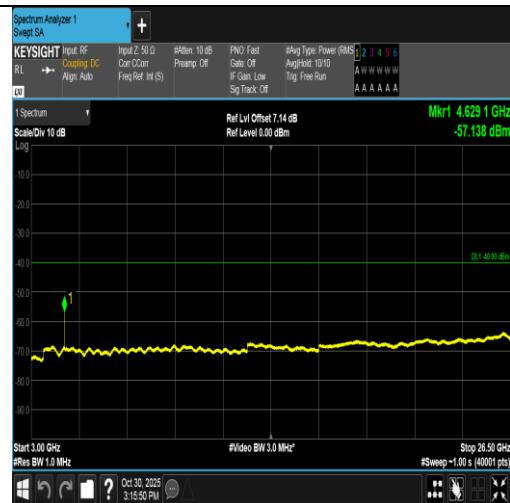
Band40(2305-2315)-5MHz-16QAM-38775-1RB#24-3000~26500-PASS
