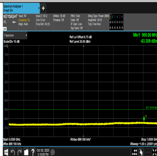
Band40(2305-2315)-5MHz-16QAM-38775-25RB#0-30~1000-PASS
