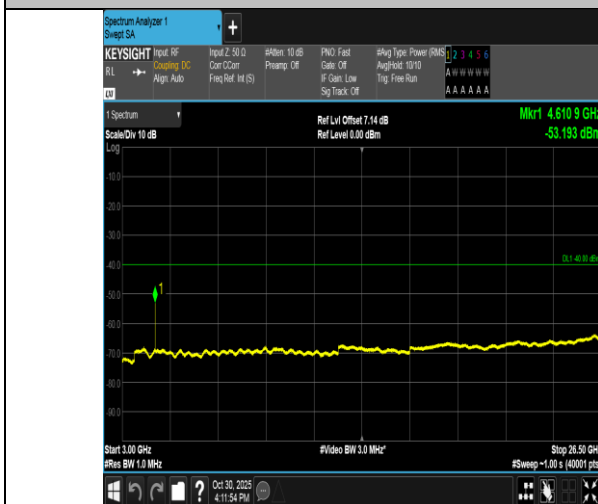
Band40(2305-2315)-10MHz-16QAM-38750-1RB#0-3000~26500-PASS
