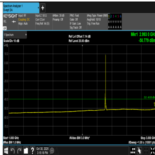
Band40(2305-2315)-5MHz-16QAM-38775-1RB#24-1000~3000-PASS
