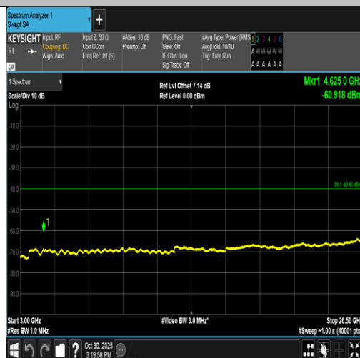
Band40(2305-2315)-5MHz-16QAM-38775-25RB#0-3000~26500-PASS
