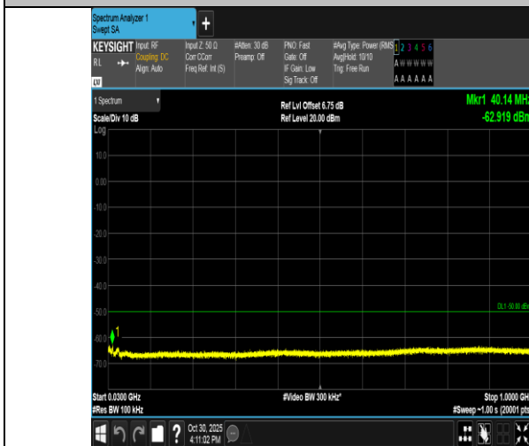
Band40(2305-2315)-10MHz-16QAM-38750-1RB#0-30~1000-PASS
