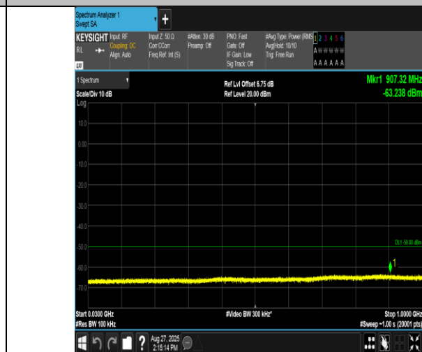
Band40(2350-2360)-5MHz-16QAM-39200-1RB#0-30~1000-PASS
