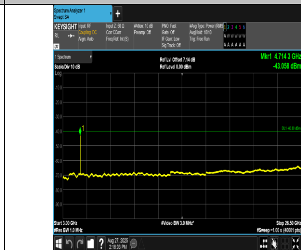
Band40(2350-2360)-5MHz-QPSK-39200-1RB#24-3000~26500-PASS
