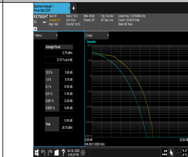
Band40(2350-2360)-5MHz-QPSK-39225-25RB#0-PASS
