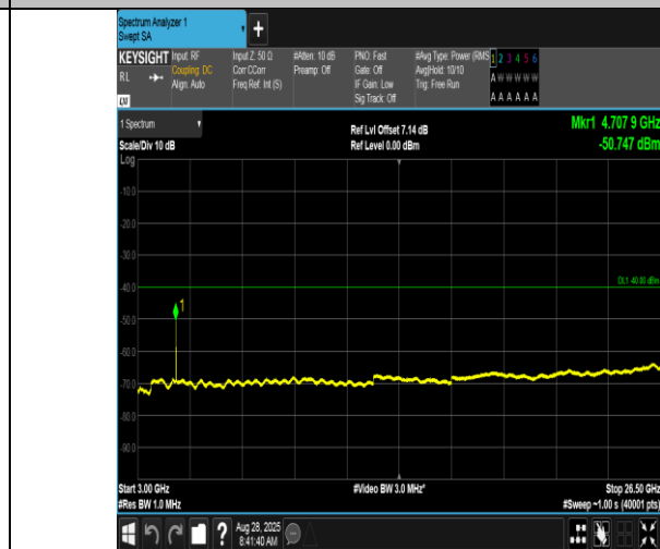
Band40(2350-2360)-5MHz-QPSK-39200-25RB#0-3000~26500-PASS
