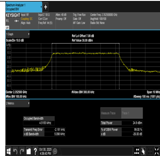
Band40(2350-2360)-5MHz-16QAM-39175-25RB#0-PASS
