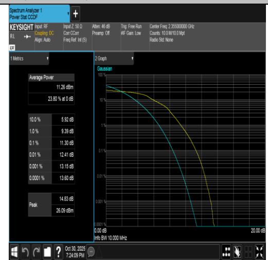
Band40(2350-2360)-10MHz-16QAM-39200-50RB#0-PASS
