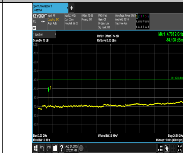
Band40(2350-2360)-5MHz-16QAM-39175-25RB#0-3000~26500-PASS
