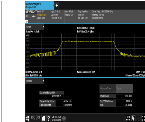
Band40(2350-2360)-5MHz-QPSK-39175-25RB#0-PASS
