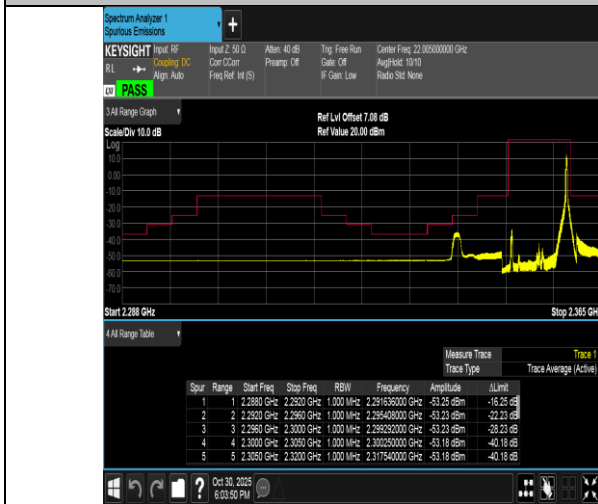
Band40(2350-2360)-10MHz-16QAM-39200-1RB#49-PASS
