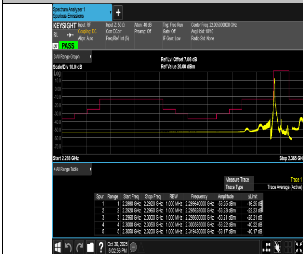
Band40(2350-2360)-5MHz-QPSK-39225-1RB#0-PASS
