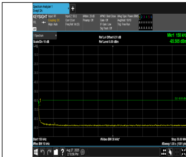
Band40(2350-2360)-5MHz-16QAM-39175-25RB#0-0.15~30-PASS
