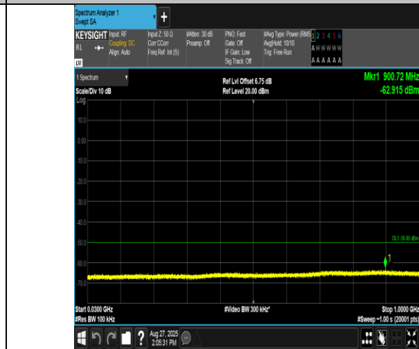
Band40(2350-2360)-5MHz-QPSK-39175-1RB#24-30~1000-PASS
