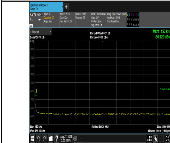
Band40(2350-2360)-5MHz-QPSK-39175-1RB#24-0.15~30-PASS
