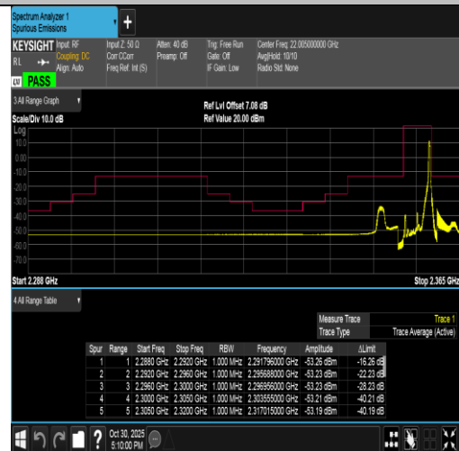
Band40(2350-2360)-5MHz-QPSK-39225-1RB#24-PASS
