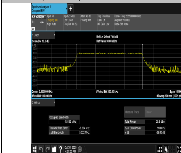
Band40(2350-2360)-5MHz-QPSK-39200-25RB#0-PASS
