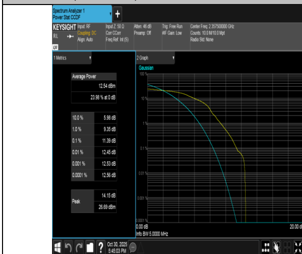
Band40(2350-2360)-5MHz-16QAM-39225-1RB#0-PASS
