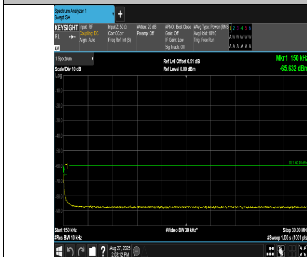
Band40(2350-2360)-5MHz-16QAM-39175-1RB#0-0.15~30-PASS
