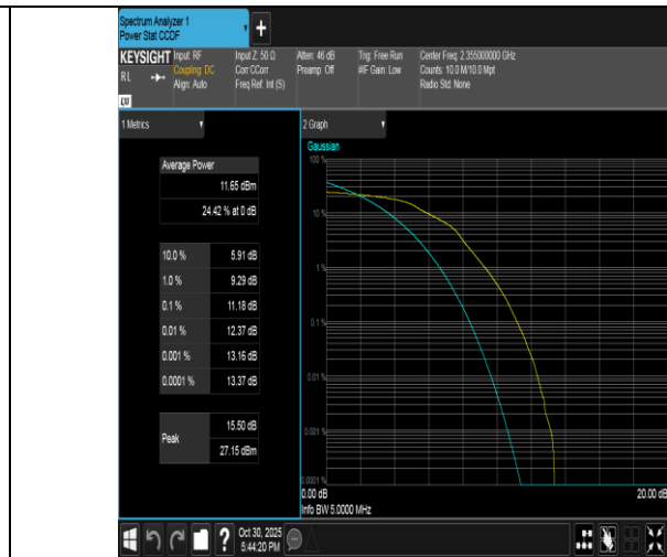
Band40(2350-2360)-5MHz-16QAM-39200-25RB#0-PASS
