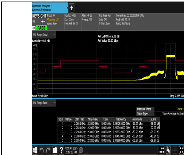
Band40(2350-2360)-5MHz-QPSK-39225-25RB#0-PASS
