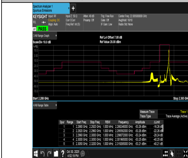
Band40(2350-2360)-5MHz-16QAM-39175-1RB#24-PASS
