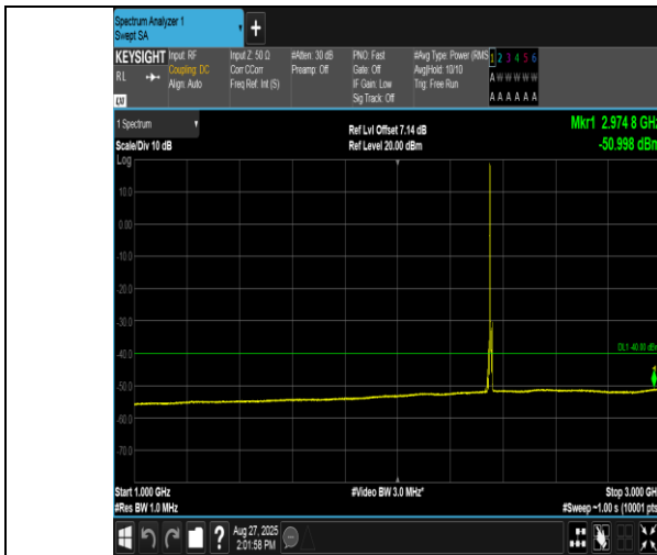
Band40(2350-2360)-5MHz-QPSK-39175-1RB#0-1000~3000-PASS
