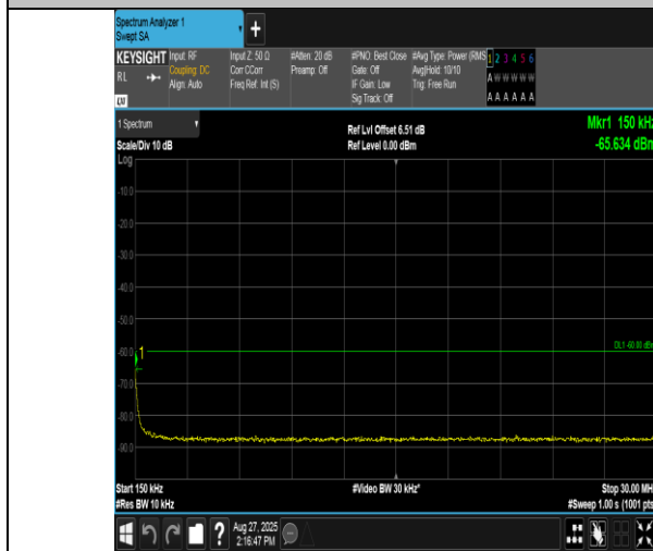
Band40(2350-2360)-5MHz-QPSK-39200-1RB#24-0.15~30-PASS
