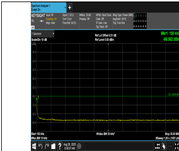
Band40(2350-2360)-5MHz-QPSK-39200-25RB#0-0.15~30-PASS
