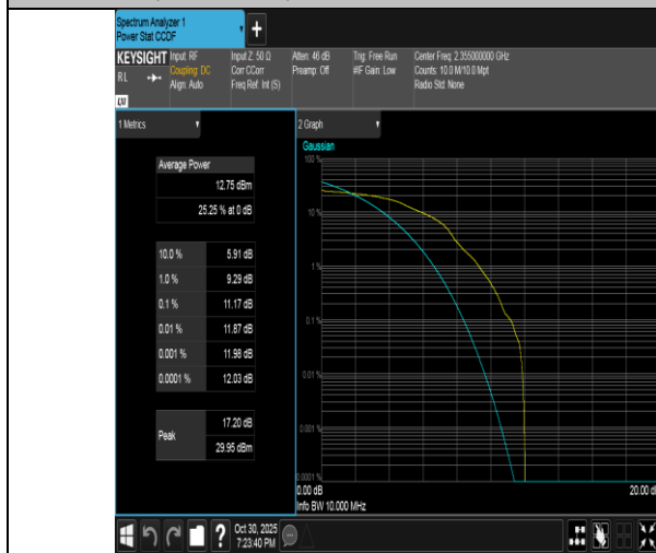
Band40(2350-2360)-10MHz-16QAM-39200-1RB#0-PASS
