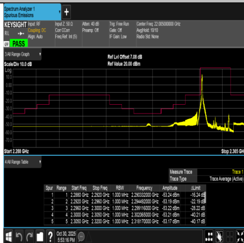
Band40(2350-2360)-10MHz-QPSK-39200-1RB#0-PASS
