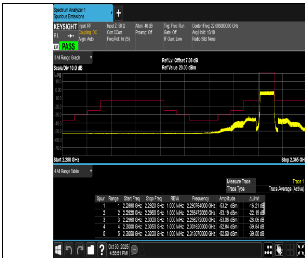
Band40(2350-2360)-5MHz-QPSK-39175-25RB#0-PASS
