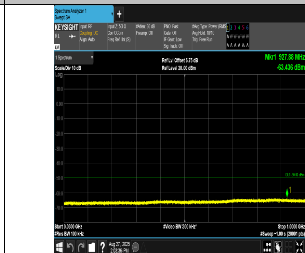
Band40(2350-2360)-5MHz-16QAM-39175-1RB#0-30~1000-PASS
