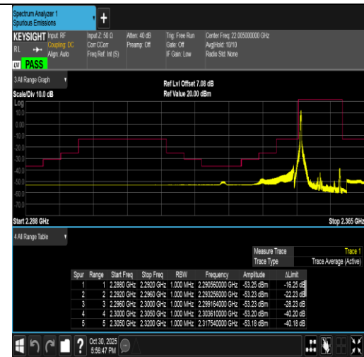
Band40(2350-2360)-10MHz-16QAM-39200-1RB#0-PASS
