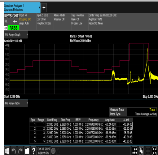
Band40(2350-2360)-10MHz-QPSK-39200-1RB#49-PASS
