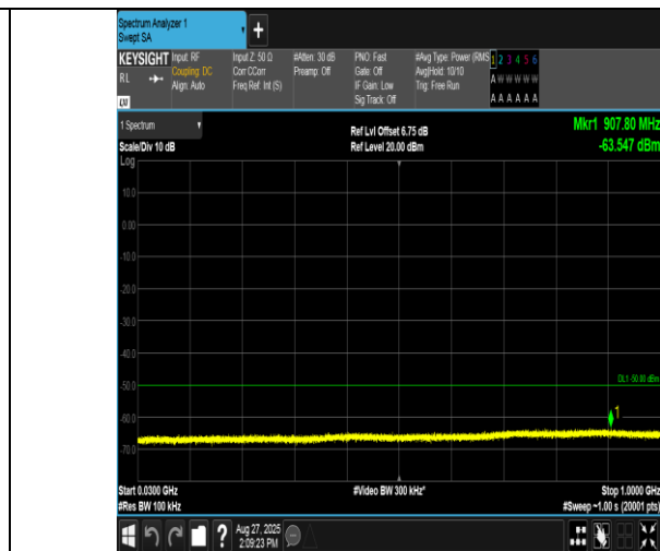
Band40(2350-2360)-5MHz-QPSK-39175-25RB#0-30~1000-PASS
