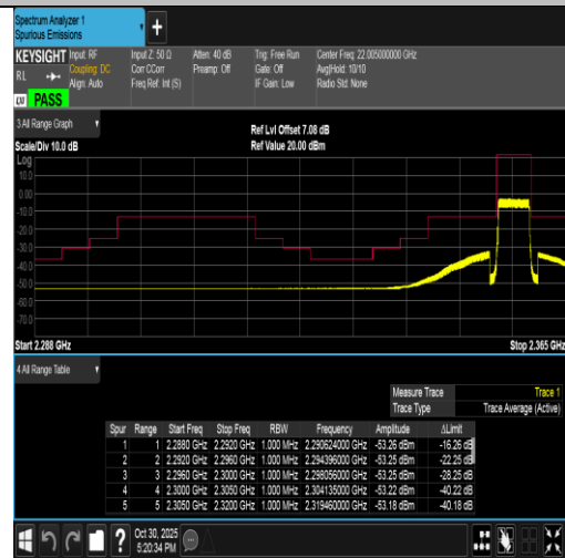
Band40(2350-2360)-5MHz-16QAM-39225-25RB#0-PASS
