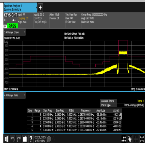
Band40(2350-2360)-5MHz-16QAM-39175-25RB#0-PASS
