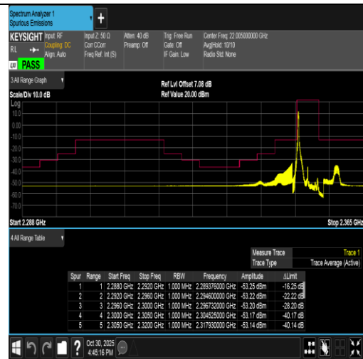
Band40(2350-2360)-5MHz-16QAM-39175-1RB#0-PASS
