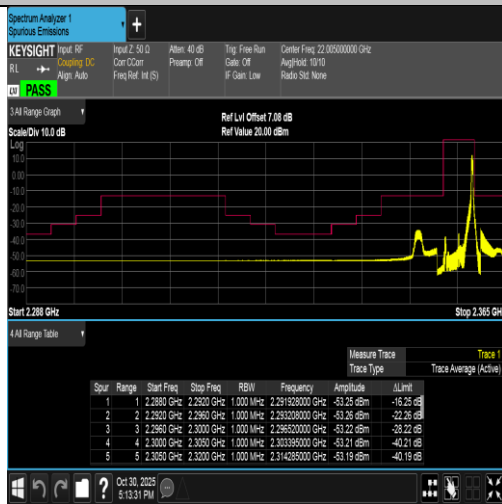
Band40(2350-2360)-5MHz-16QAM-39225-1RB#24-PASS
