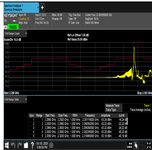
Band40(2350-2360)-5MHz-16QAM-39225-1RB#0-PASS
