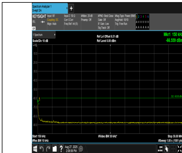
Band40(2350-2360)-5MHz-QPSK-39175-25RB#0-0.15~30-PASS
