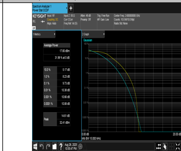
Band41(2555-2655)-15MHz-QPSK-40690-75RB#0-PASS
