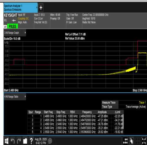
Band41(2555-2655)-5MHz-16QAM-40265-25RB#0-PASS
