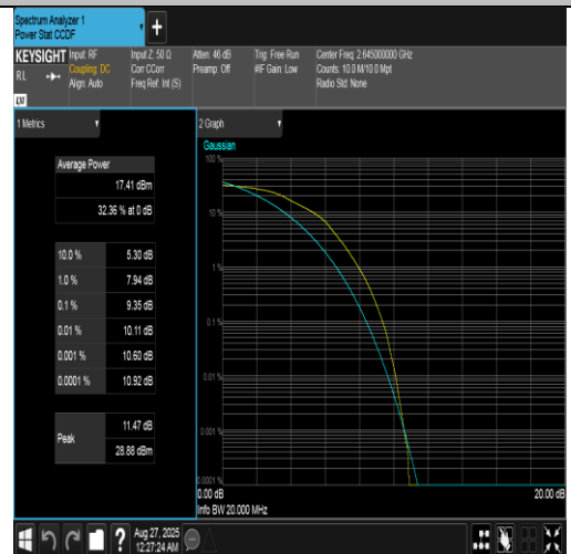
Band41(2555-2655)-20MHz-16QAM-41140-100RB#0-PASS
