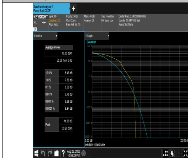
Band41(2555-2655)-15MHz-16QAM-41165-1RB#0-PASS
