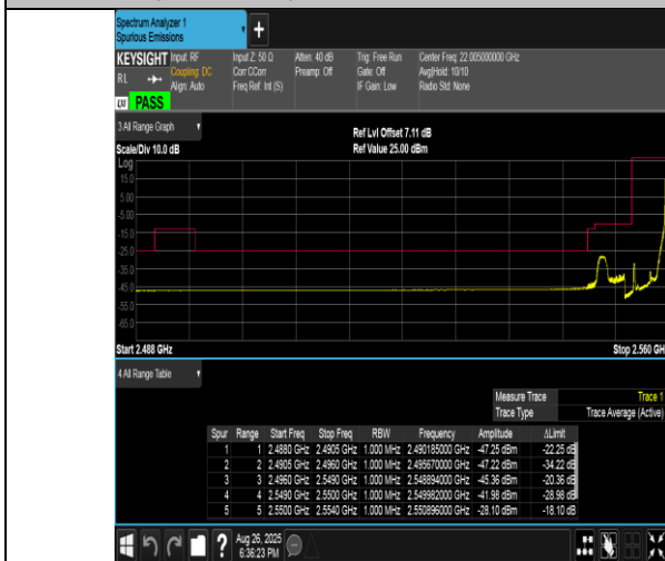
Band41(2555-2655)-5MHz-16QAM-40265-1RB#24-PASS
