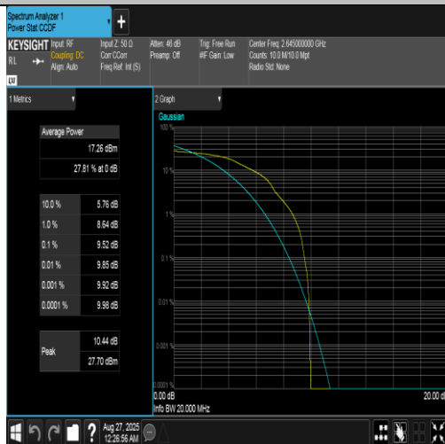
Band41(2555-2655)-20MHz-16QAM-41140-1RB#0-PASS
