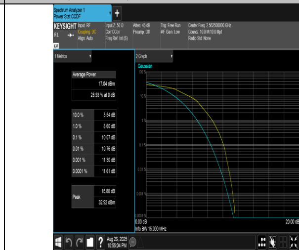
Band41(2555-2655)-15MHz-16QAM-40315-75RB#0-PASS
