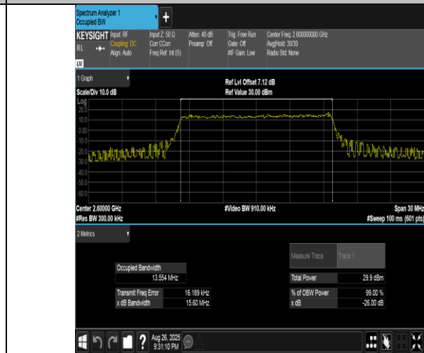
Band41(2555-2655)-15MHz-16QAM-40690-75RB#0-PASS
