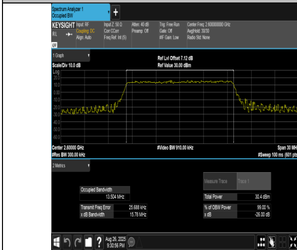
Band41(2555-2655)-15MHz-QPSK-40690-75RB#0-PASS
