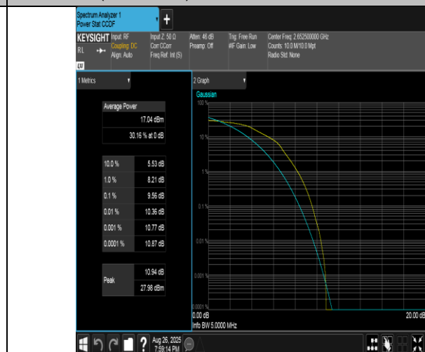
Band41(2555-2655)-5MHz-16QAM-41215-25RB#0-PASS
