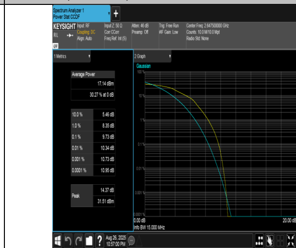
Band41(2555-2655)-15MHz-16QAM-41165-75RB#0-PASS
