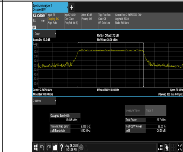
Band41(2555-2655)-15MHz-16QAM-41165-75RB#0-PASS
