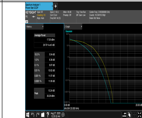
Band41(2555-2655)-20MHz-16QAM-40340-100RB#0-PASS
