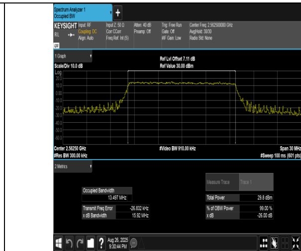
Band41(2555-2655)-15MHz-16QAM-40315-75RB#0-PASS
